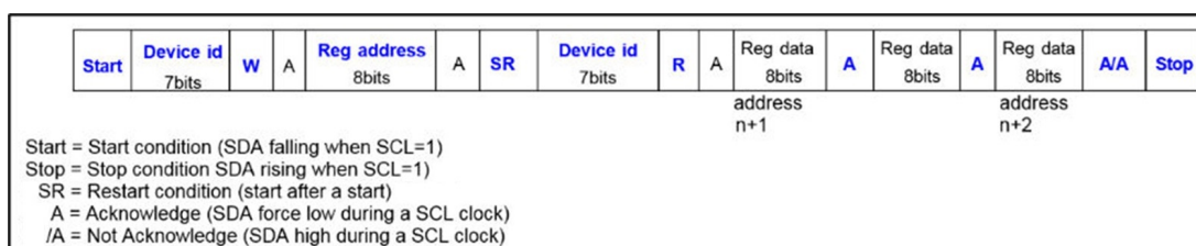
Figure 20. I 2 C read operation
