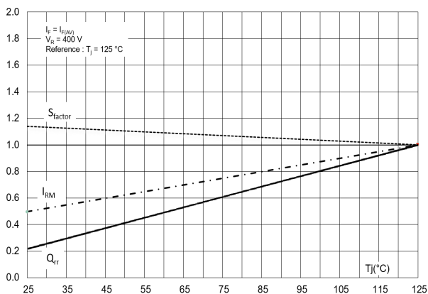
Figure 10. Relative variation of dynamic parameters versus junction temperature
