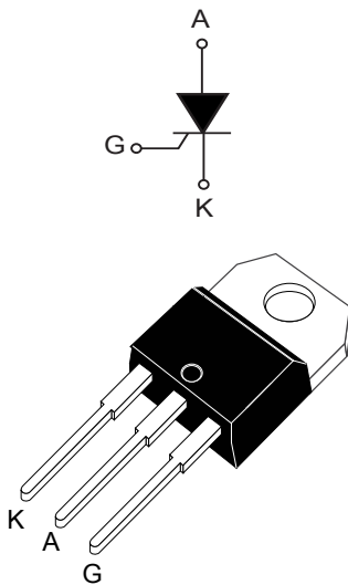
TO-220AB insulated
