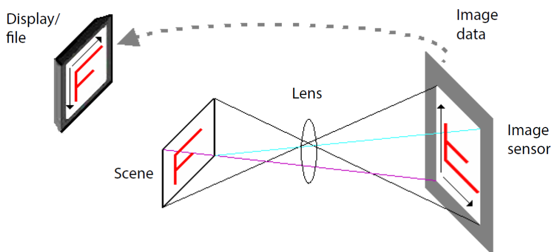
Figure 13. Image orientation
