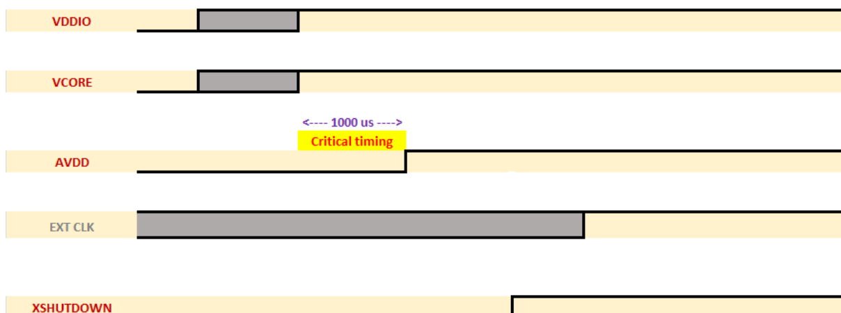
Figure 7. Powerup sequence
