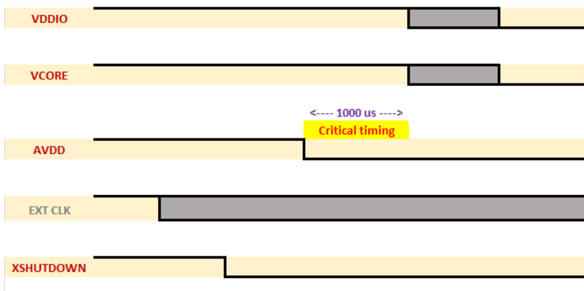
Figure 8. Powerdown sequence
