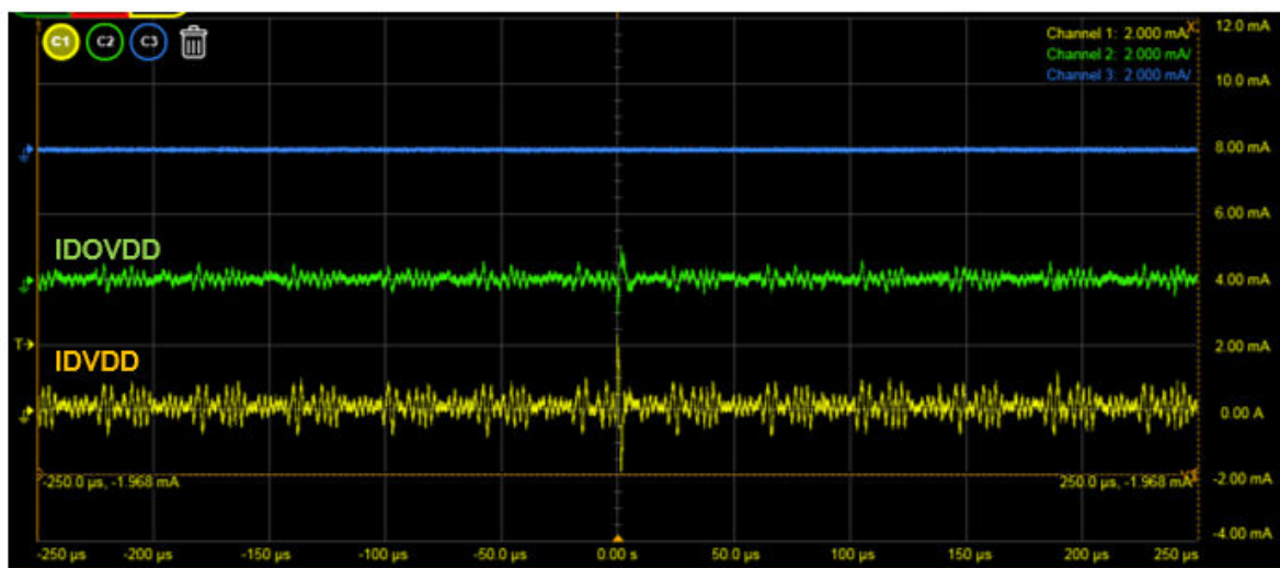
Figure 10. Start streaming
