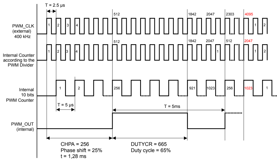
Figure 12. Resulting waveform 1
