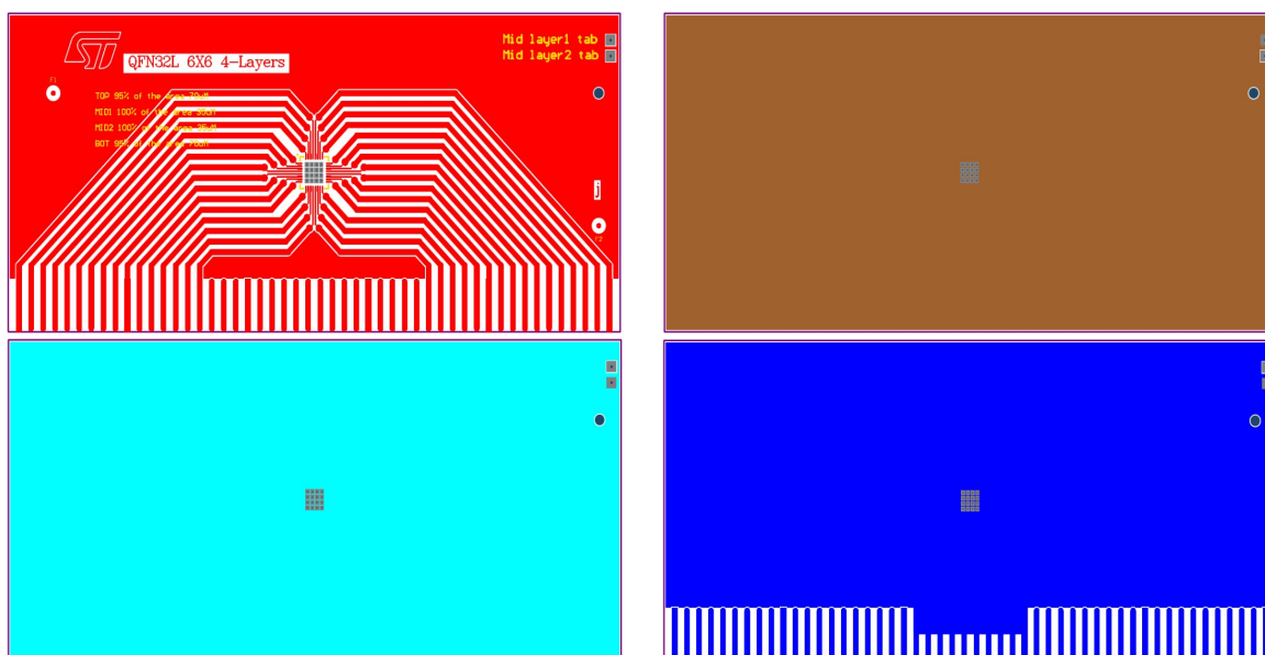
Figure 43. QFN 6x6 PCB 4 layers
