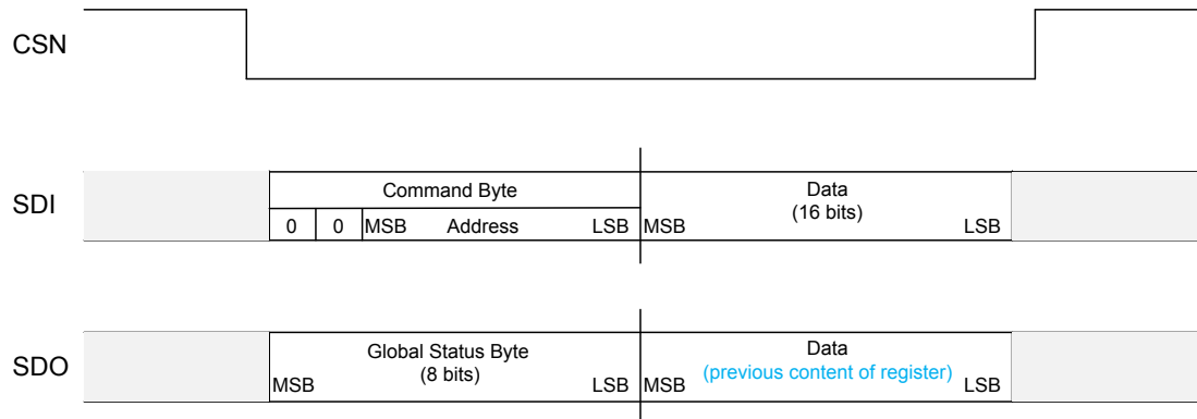
Figure 8. SPI write operation
