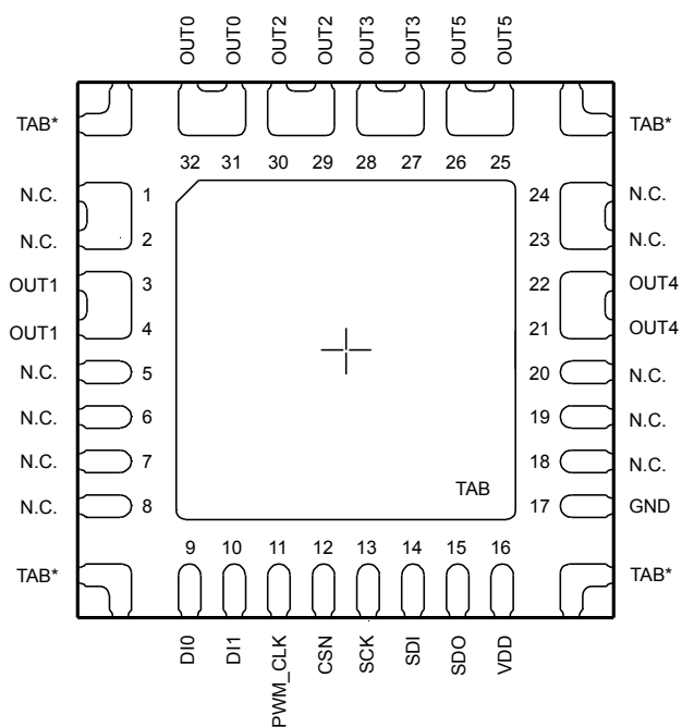
Figure 2. Connection diagram (top view)
