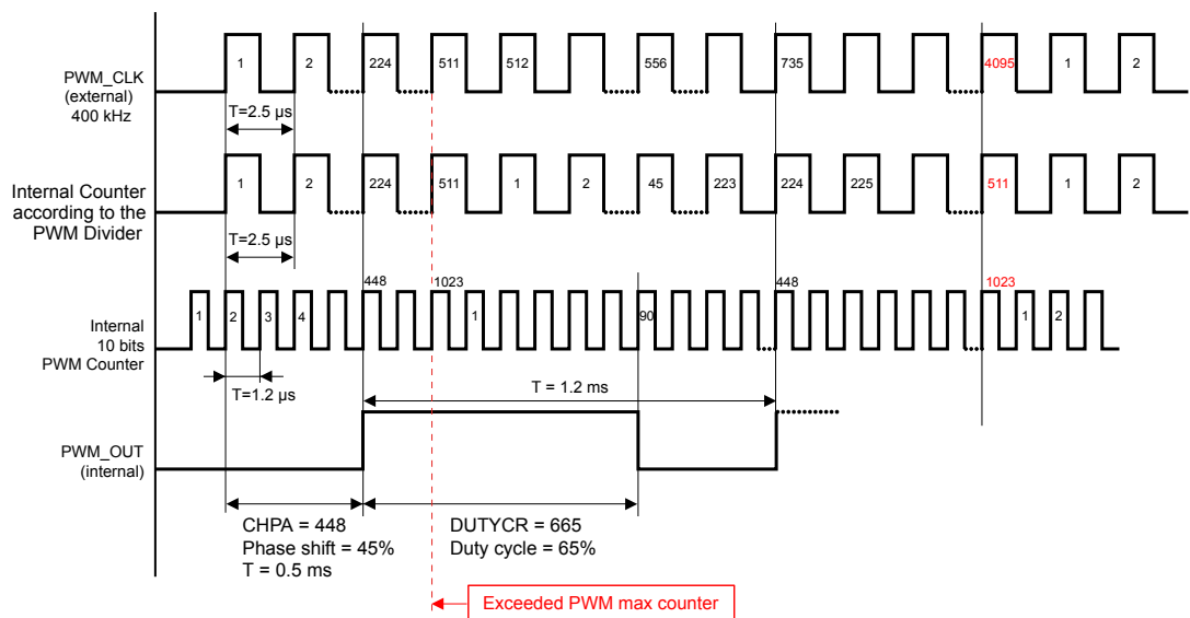
Figure 14. Resulting waveform 3
