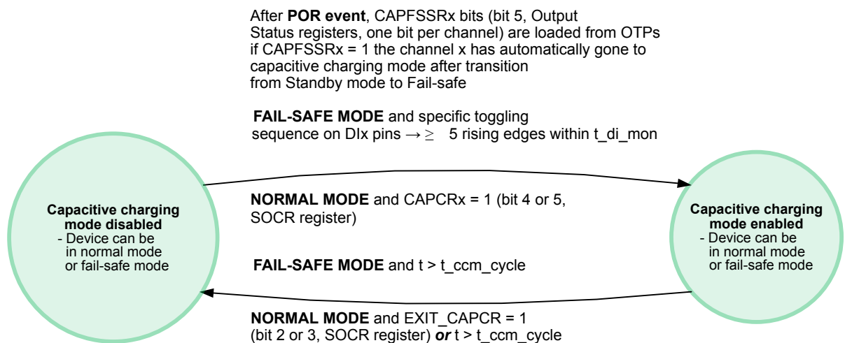
Figure 4. Channel state diagram
