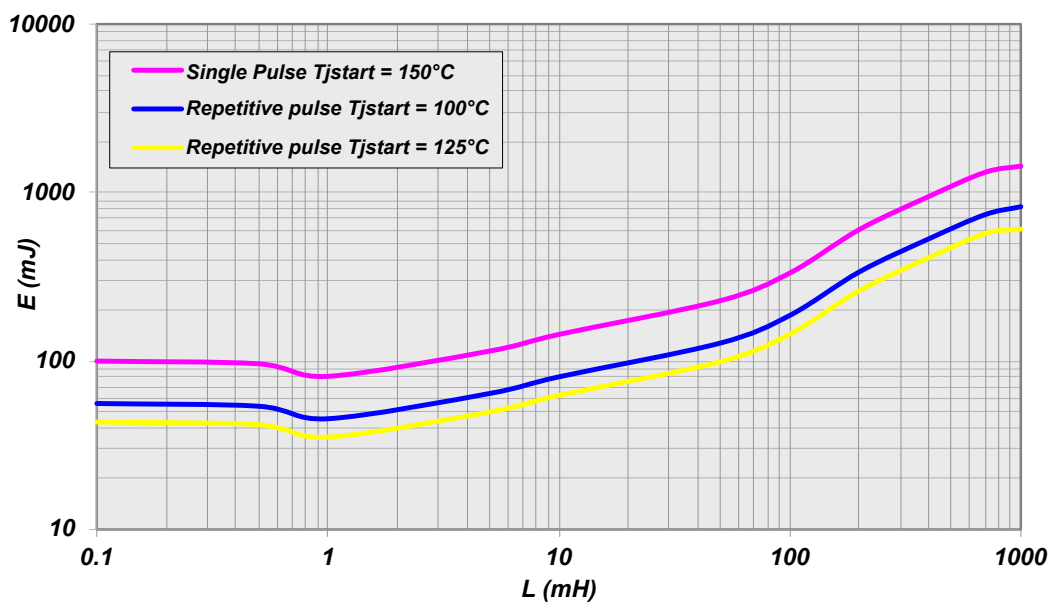
Figure 21. Maximum turn off energy versus inductance
