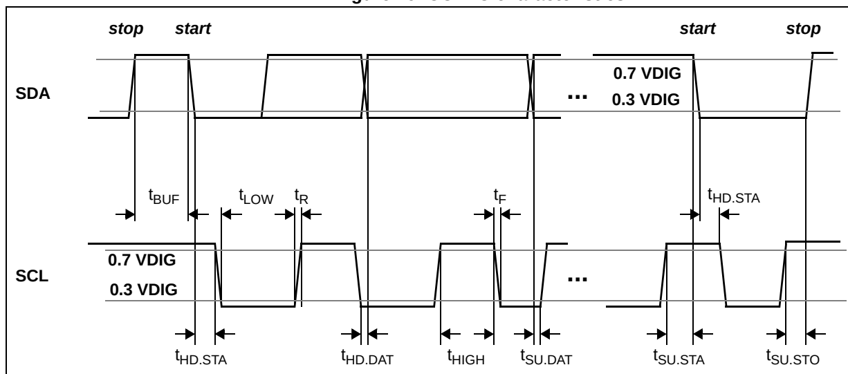
Figure 19. CCI AC characteristics
