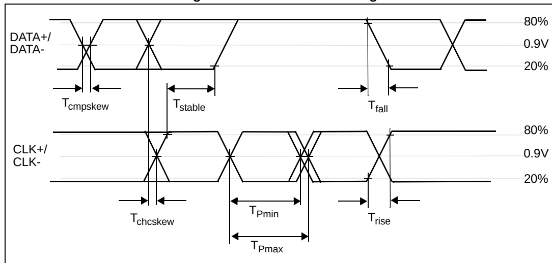
Figure 20. SubLVDS AC timing
