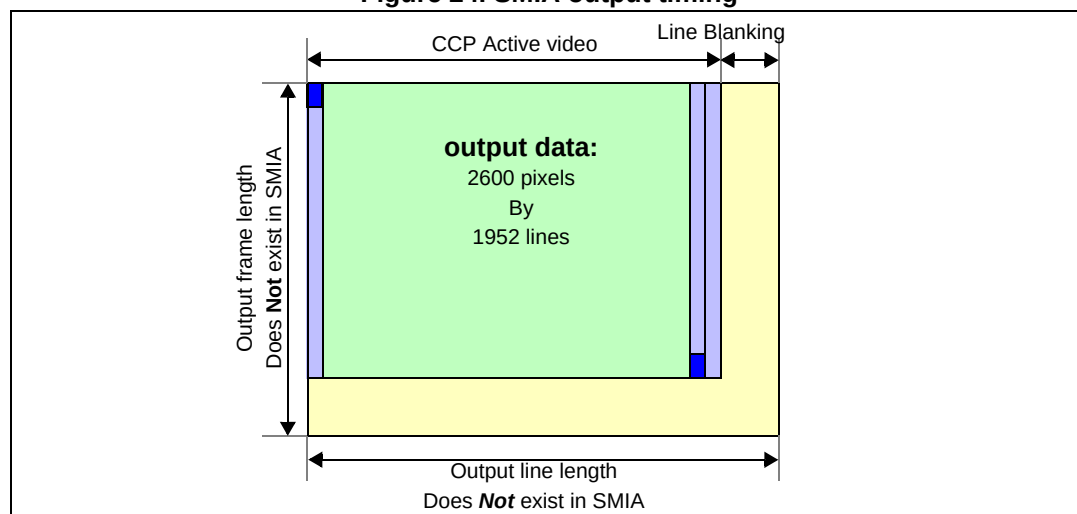
Figure 24. SMIA output timing
