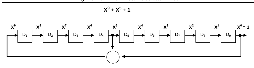
Figure 29. PN9 linear feedback filter
