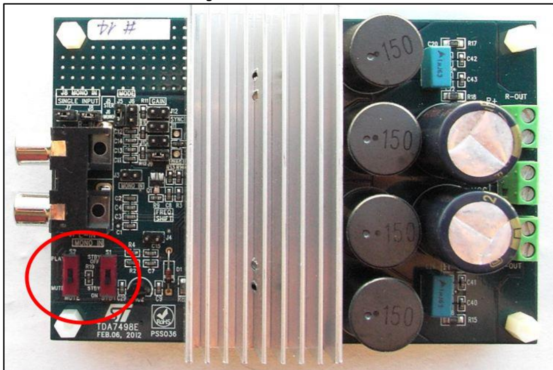
Figure 1: Board identification
