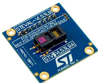
STEval: Order code: STEVAL-VL53L9
