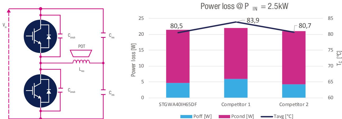
FIGURE 2: POWER LOSSES AND T_c EVALUATION
