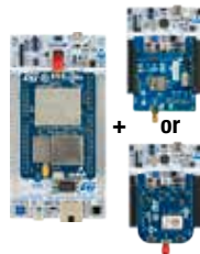
2 NUCLEO PACKS: GATEWAY + END-NODE P/N: P-NUCLEO-LRWAN2 a P/N: P-NUCLEO-LRWAN3 b (ST and USI®/RisingHF®)
