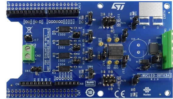
X-NUCLEO-OUT03A1
