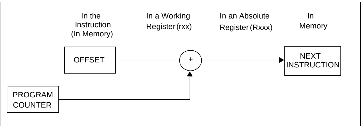
Figure 14. Program Memory Relative Addressing Mode
