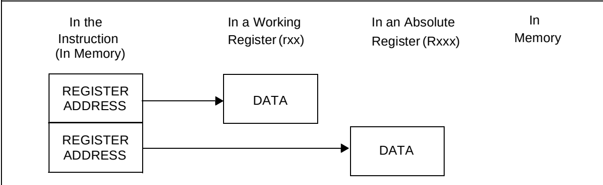
Figure 2. Register Direct Addressing Mode
