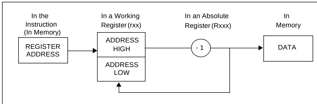
Figure 9. Memory Indirect Addressing Mode with Pre-Decrement
