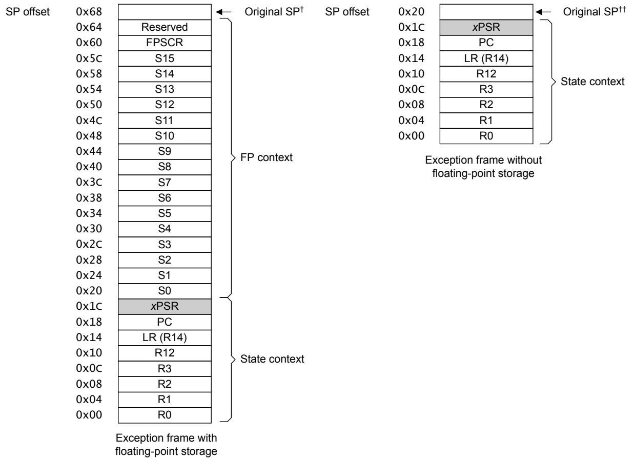
Figure 9. Stack frame when an interrupt or an exception is preserved on the stack with or without floating-point state
