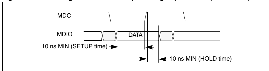
Figure 57. MII management interface: input timing requirements (PHY device)
