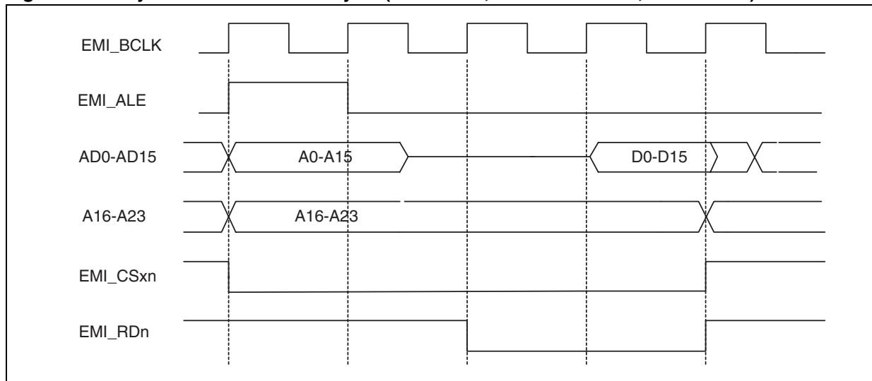
Figure 14. Asynchronous read bus cycle (mux mode, with WSTOE = 2, WSTRD = 3)
