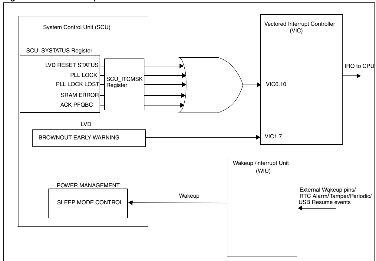
Figure 27. SCU Interrupts
