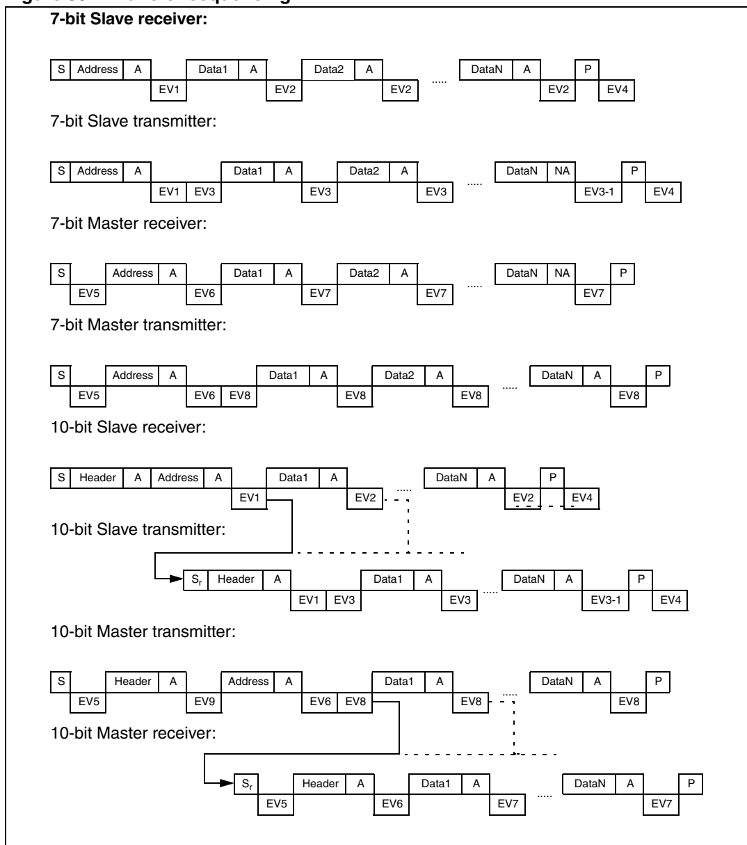
Figure 83. Transfer sequencing
