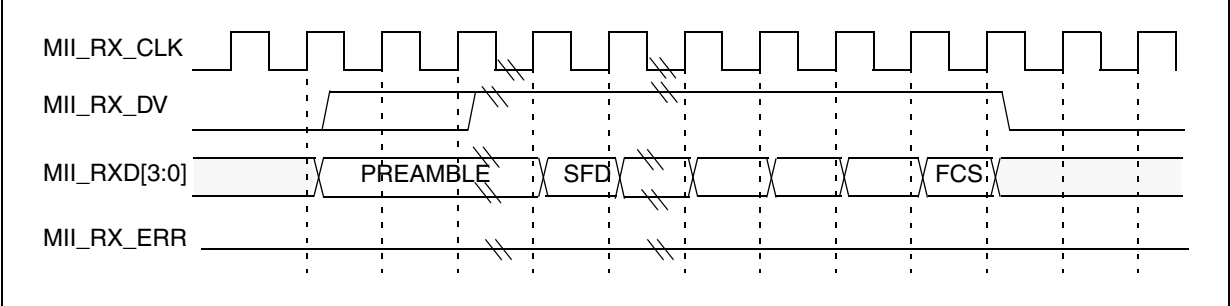
Figure 52. Reception with no errors
