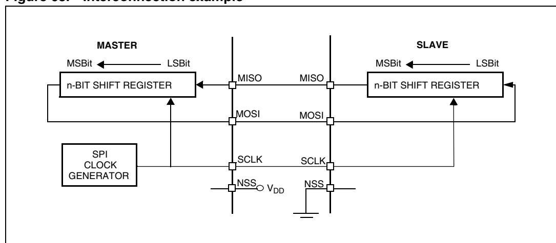
Figure 68. Interconnection example
