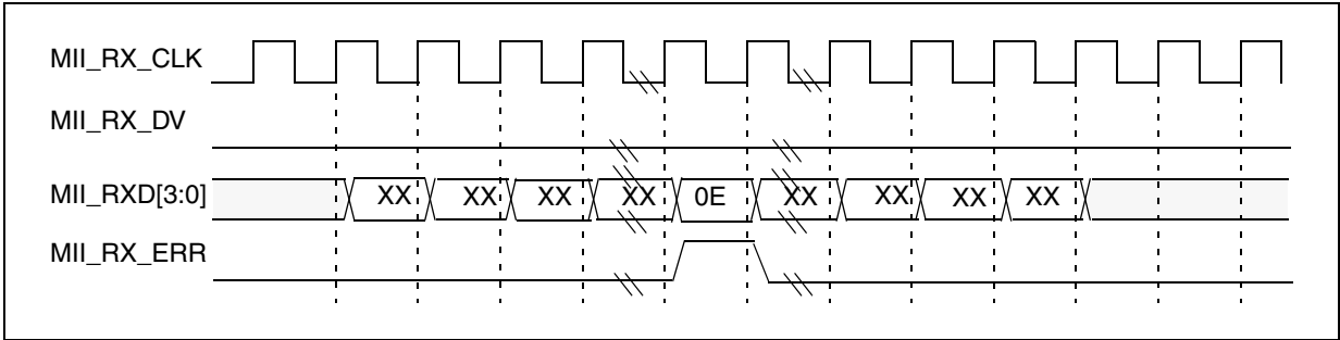
Figure 54. Reception with false carrier indication
