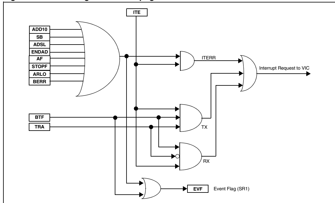
Figure 84. Event flags and interrupt generation
