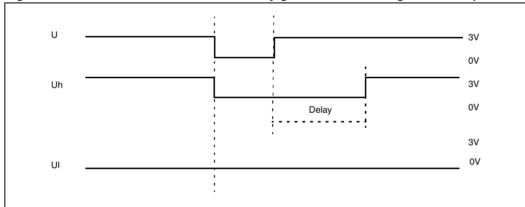
Figure 92. Dead time waveforms with delay greater than the negative PWM pulse
