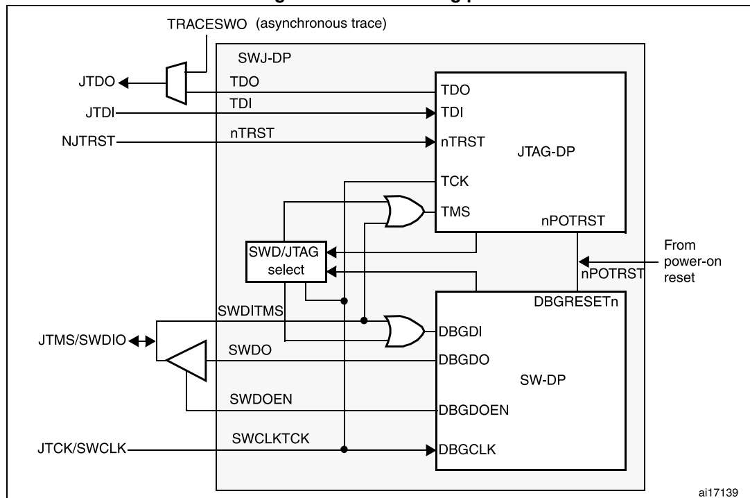
Figure 502. SWJ debug port
