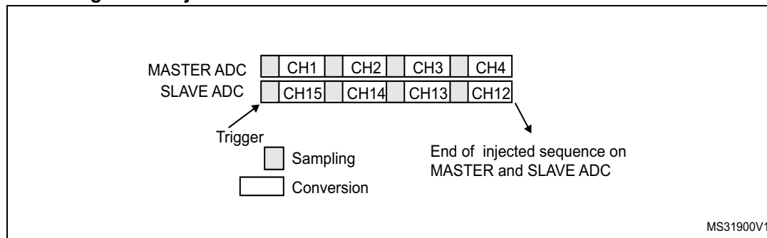
Figure 91. Injected simultaneous mode on 4 channels: dual ADC mode
