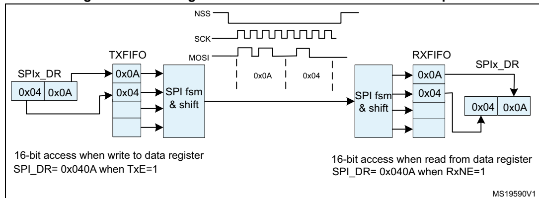
Figure 435. Packing data in FIFO for transmission and reception
