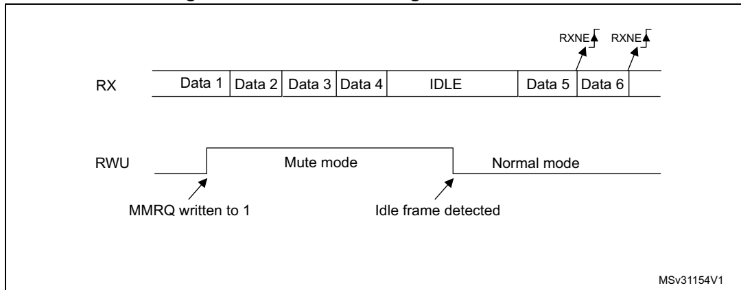
Figure 418. Mute mode using Idle line detection
