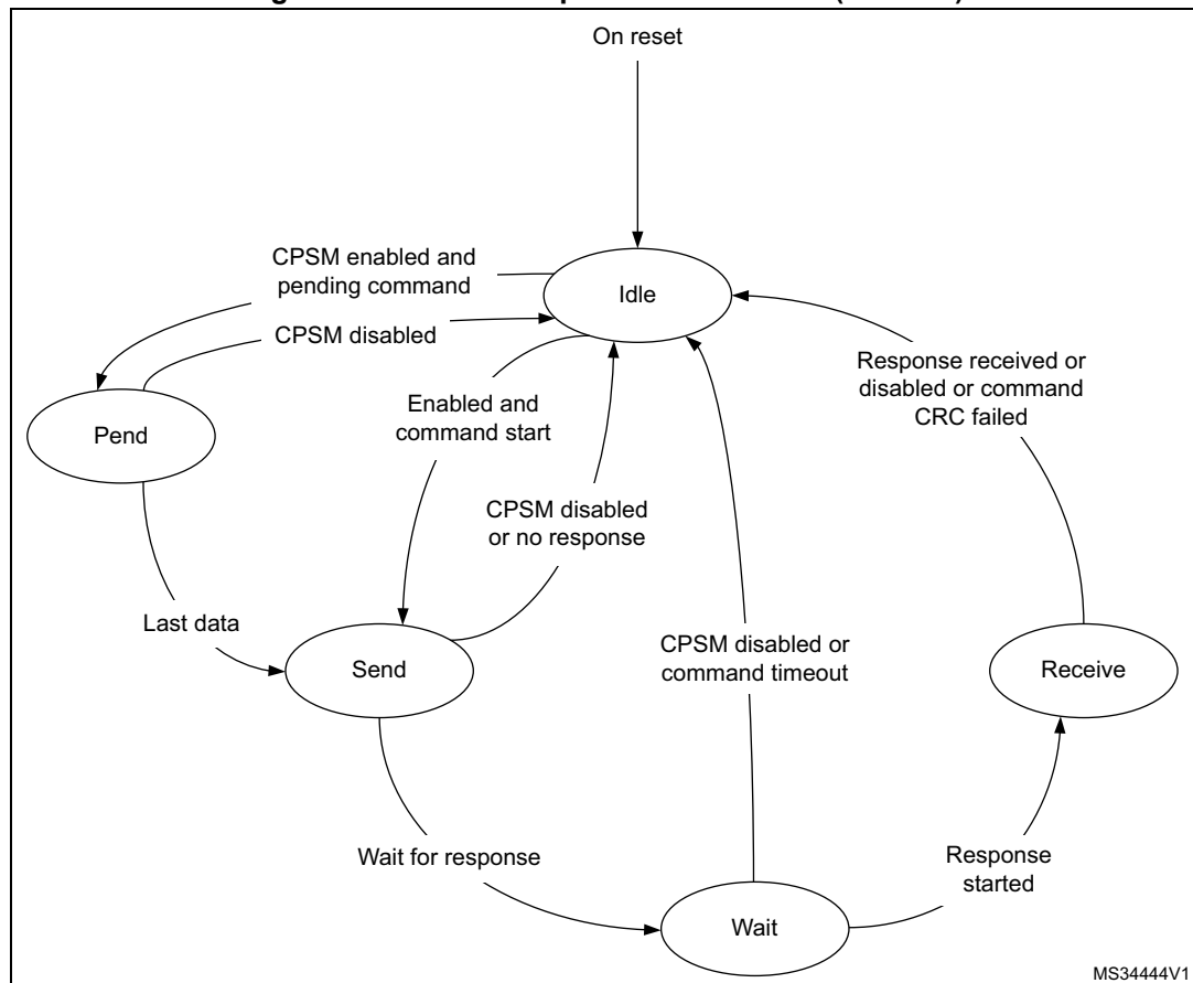
Figure 479. Command path state machine (SDMMC)
