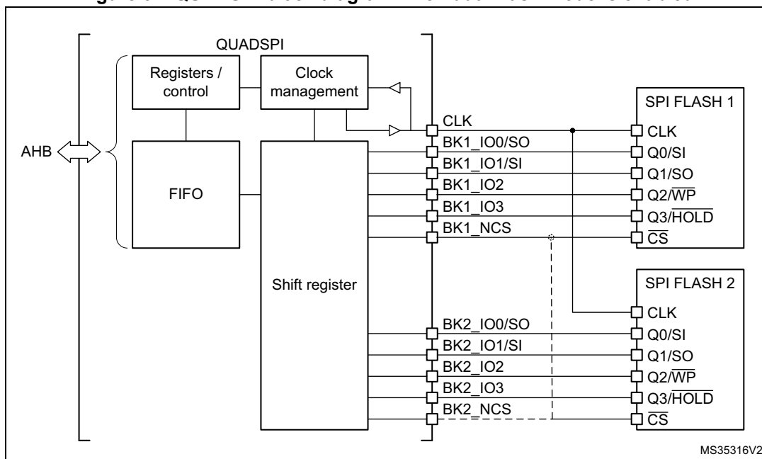
Figure 32. QUADSPI block diagram when dual-flash mode is enabled
