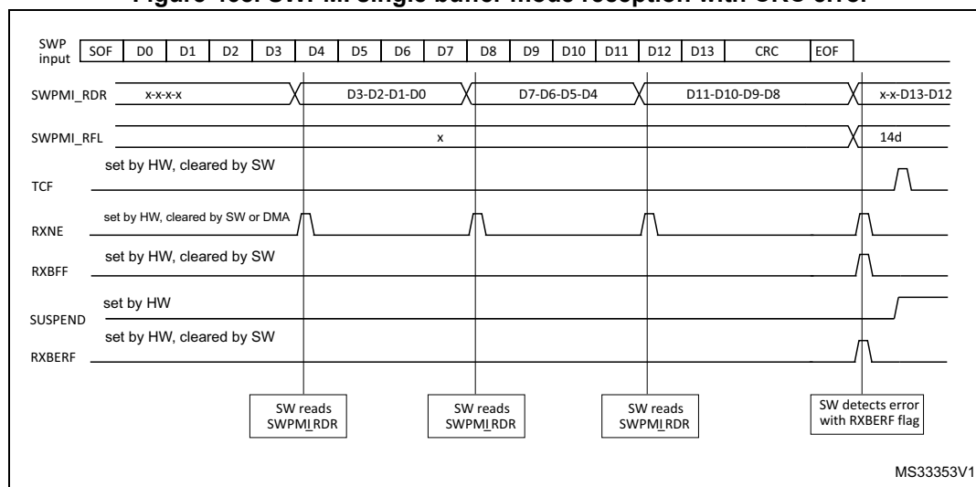
Figure 468. SWPMI single buffer mode reception with CRC error
