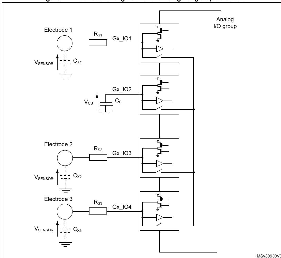
Figure 147. Surface charge transfer analog I/O group structure
