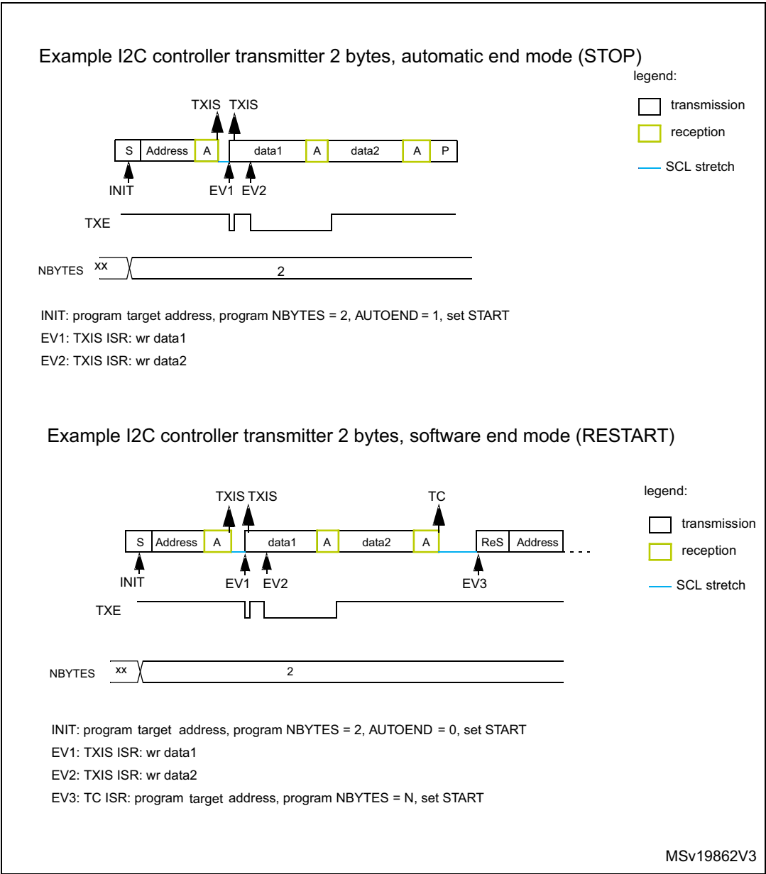
Figure 378. Transfer bus diagrams for I2C controller transmitter (mandatory events only)
