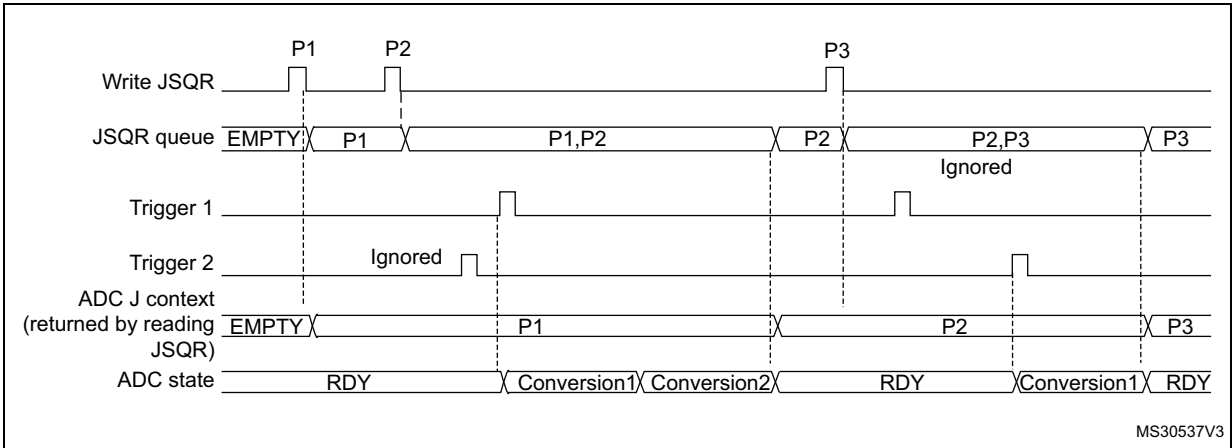
Figure 53. Example of JSQR queue of context (trigger change)
