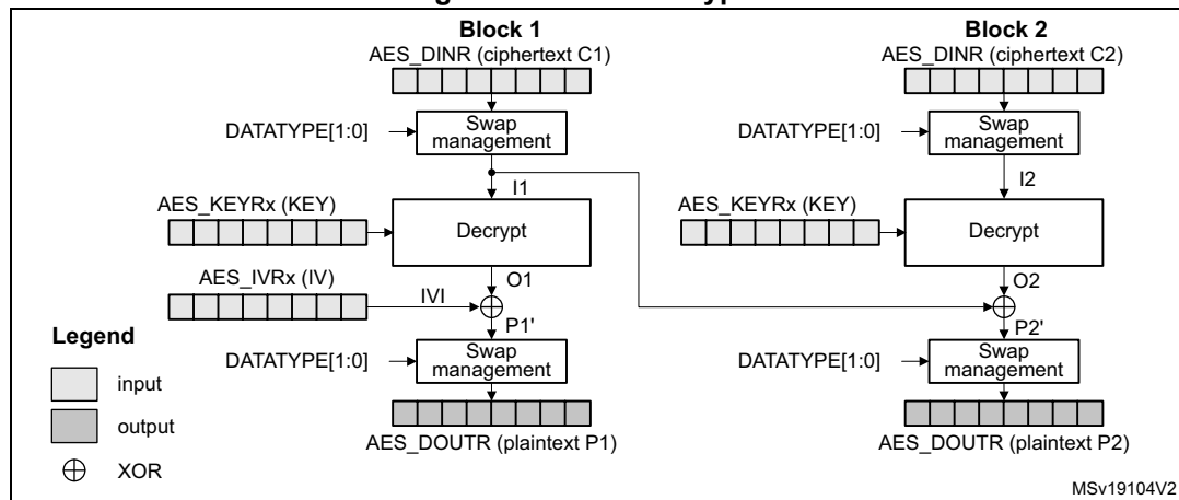
Figure 167. CBC decryption
