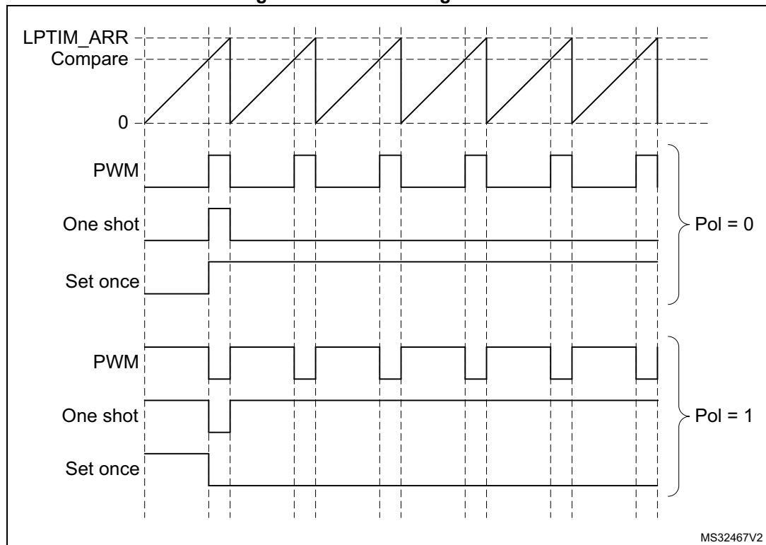
Figure 349. Waveform generation
