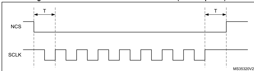
Figure 36. NCS when CKMODE = 1 in SDR mode (T = CLK period)
