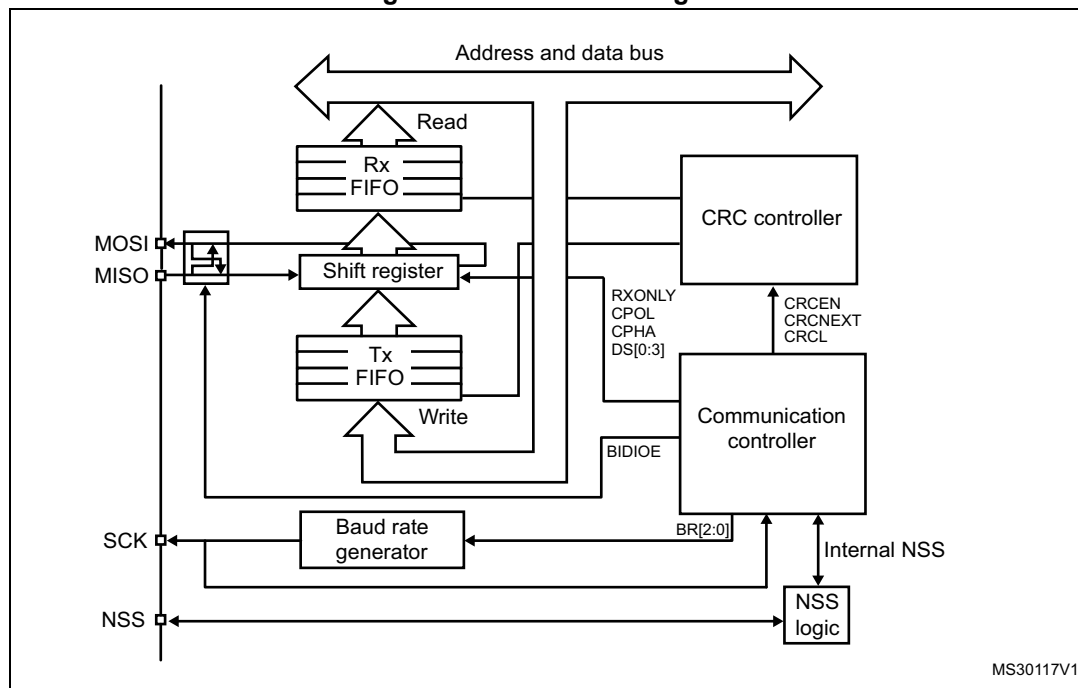
Figure 426. SPI block diagram
