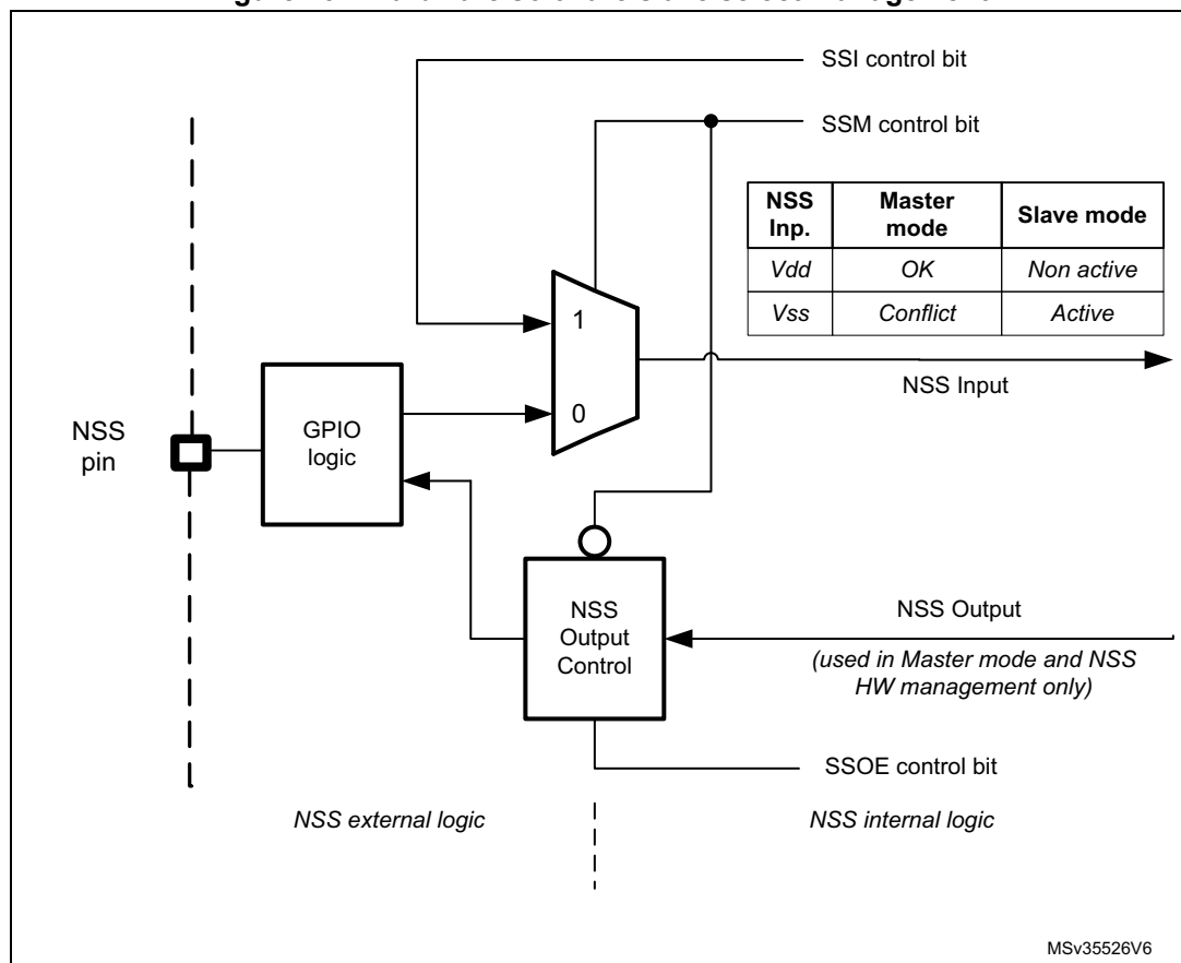
Figure 432. Hardware/software slave select management
