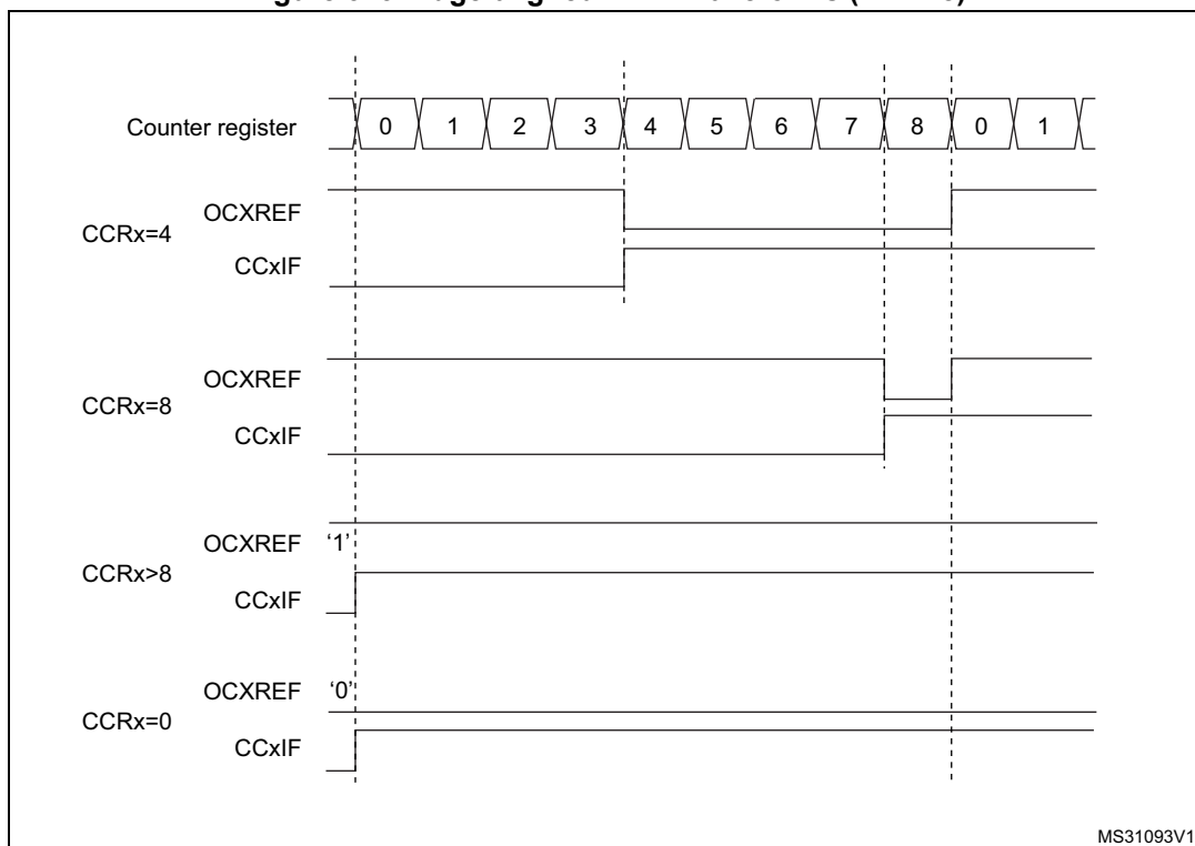
Figure 313. Edge-aligned PWM waveforms (ARR=8)
