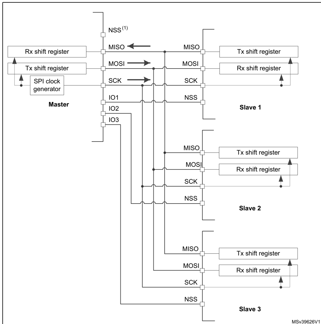
Figure 430. Master and three independent slaves
