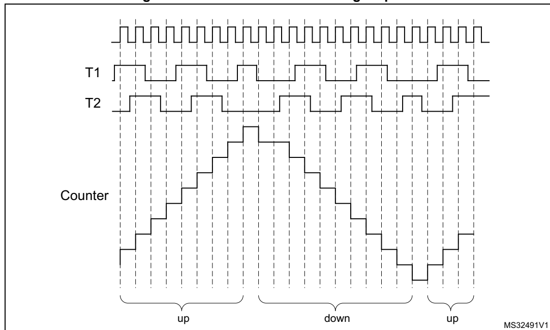
Figure 350. Encoder mode counting sequence
