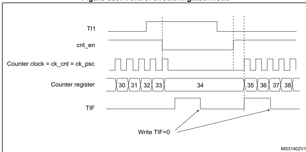
Figure 325. Control circuit in gated mode
