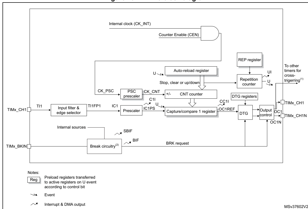
Figure 294. TIM16 block diagram
