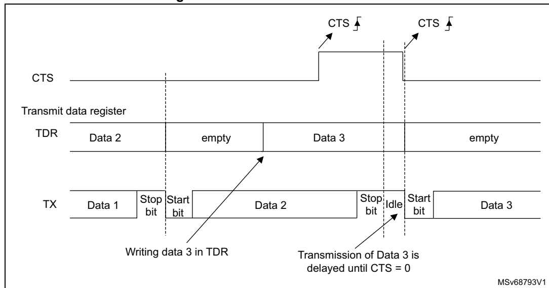
Figure 412. RS232 CTS flow control
