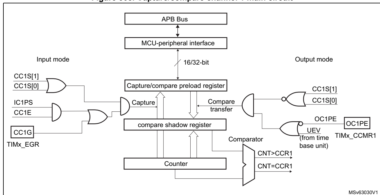
Figure 308. Capture/compare channel 1 main circuit
