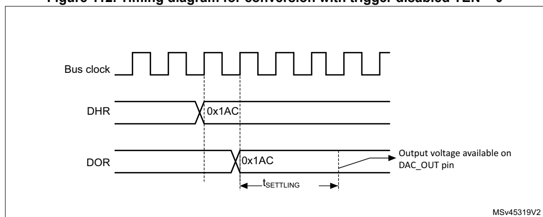
Figure 112. Timing diagram for conversion with trigger disabled TEN = 0
