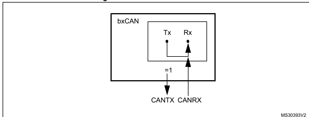
Figure 486. bxCAN in silent mode
