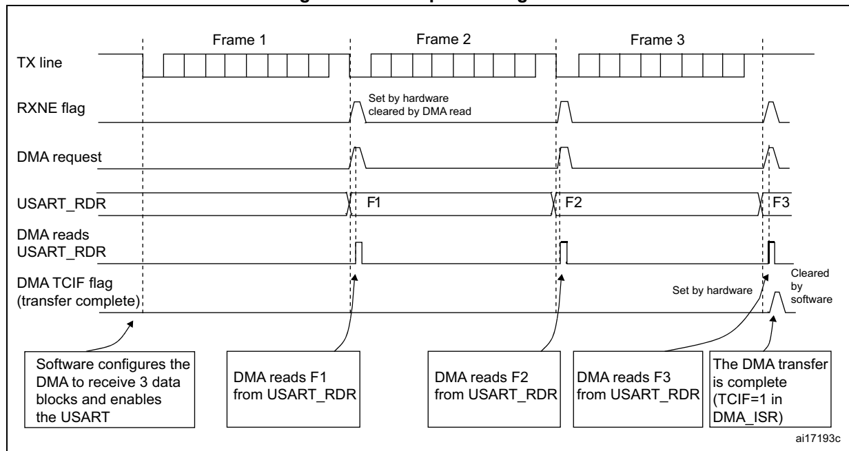
Figure 409. Reception using DMA
