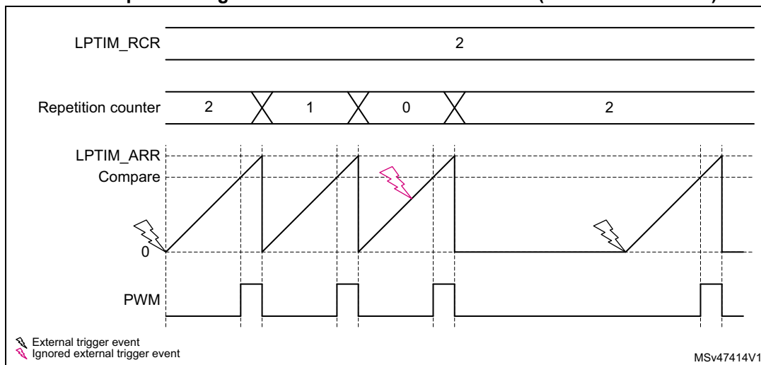
Figure 346. LPTIM output waveform, single-counting mode configuration when repetition register content is different than zero (with PRELOAD = 1)
