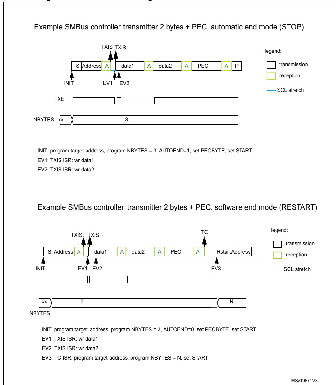
Figure 387. Bus transfer diagrams for SMBus controller transmitter
