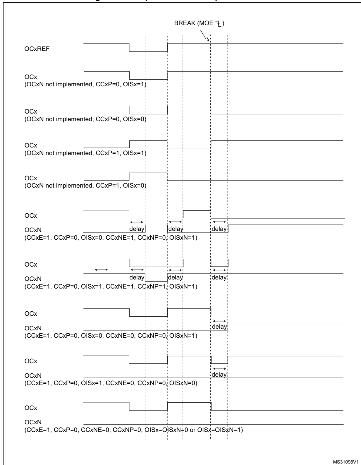
Figure 319. Output behavior in response to a break
