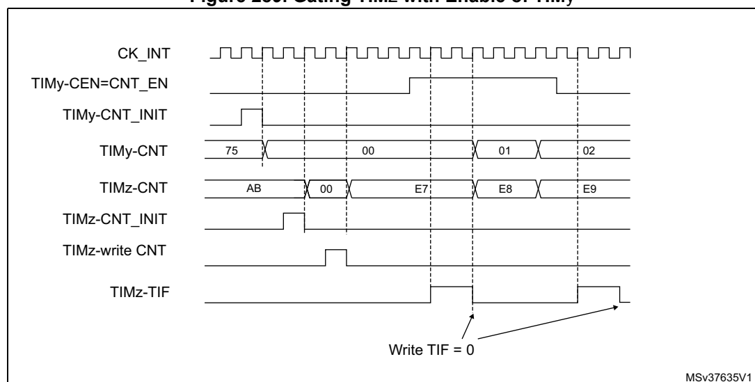
Figure 289. Gating TIMz with Enable of TIMy
