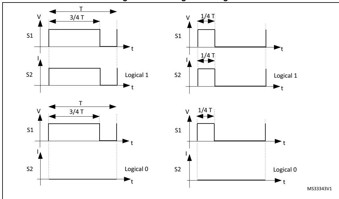
Figure 458. S2 signal coding
