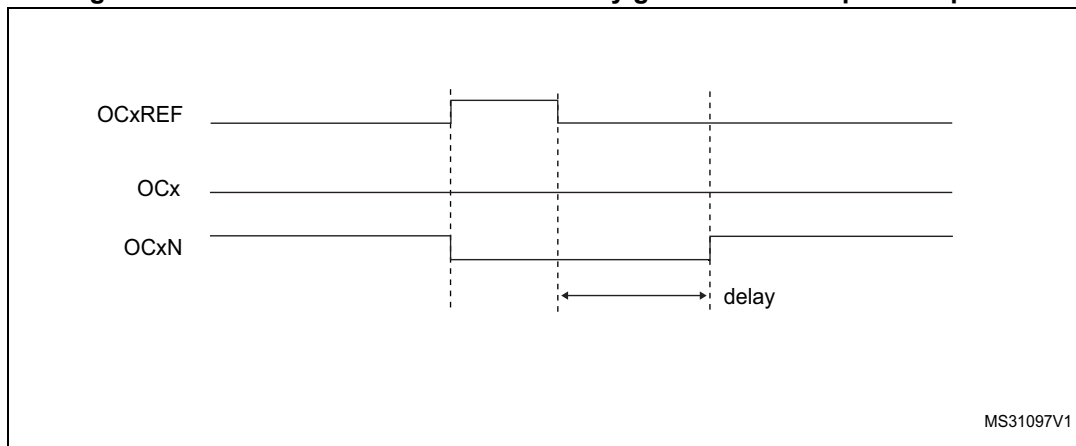
Figure 317. Dead-time waveforms with delay greater than the positive pulse.
