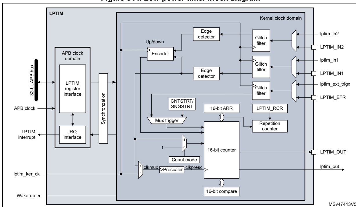
Figure 344. Low-power timer block diagram
