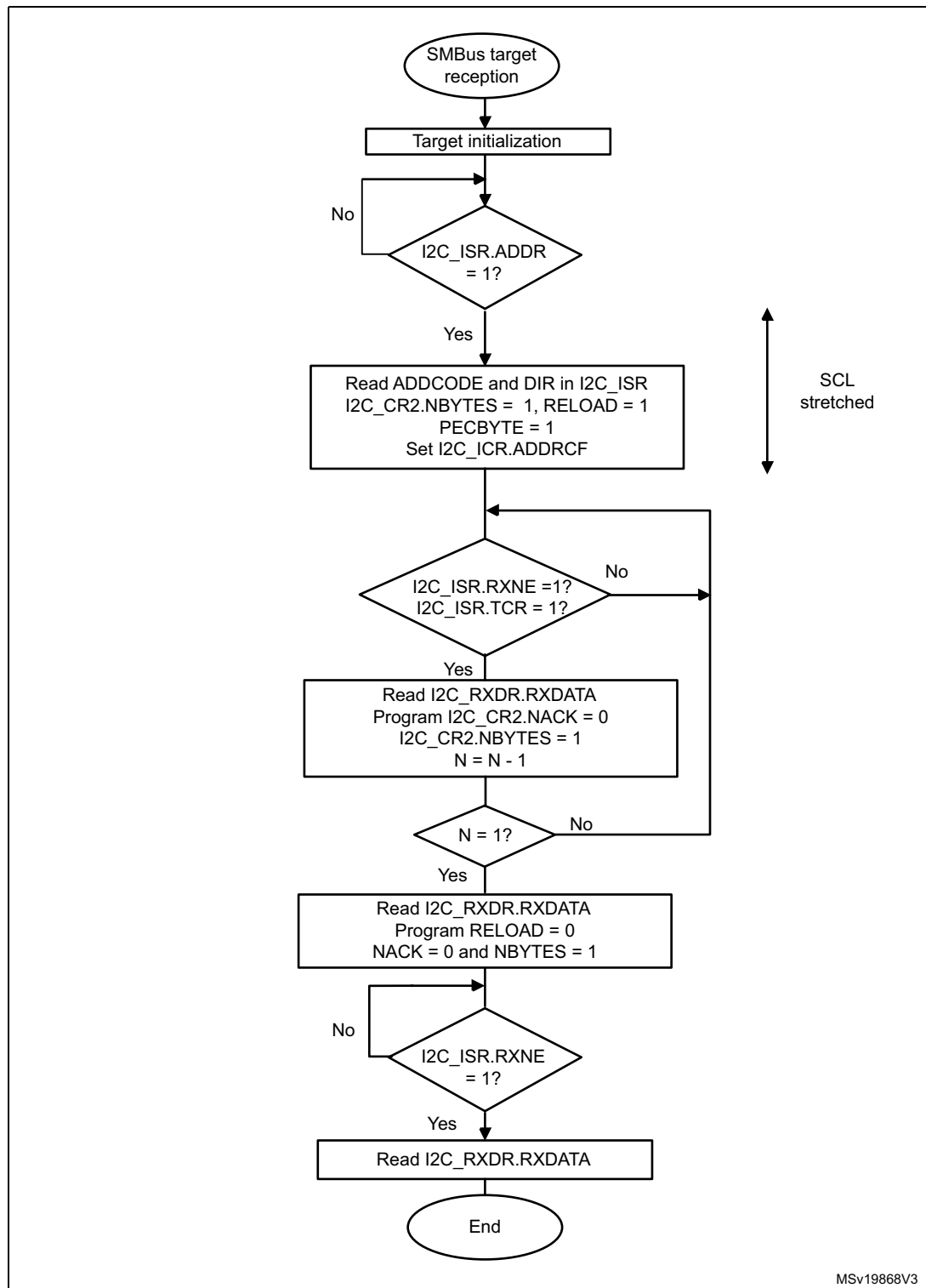
Figure 385. Transfer sequence flow for SMBus target receiver N bytes + PEC
