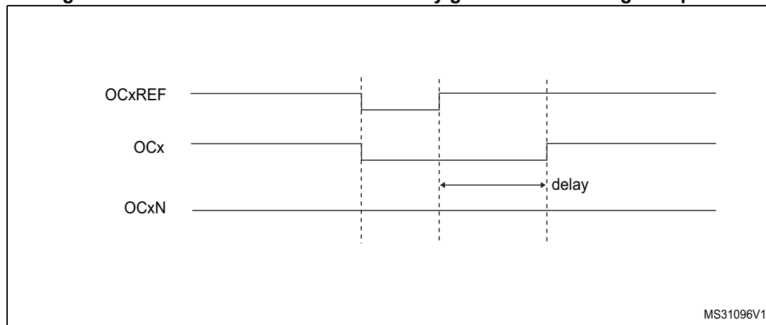
Figure 316. Dead-time waveforms with delay greater than the negative pulse.
