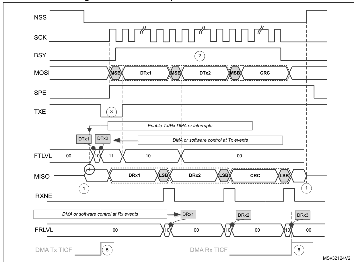
Figure 438. Master full-duplex communication with CRC
