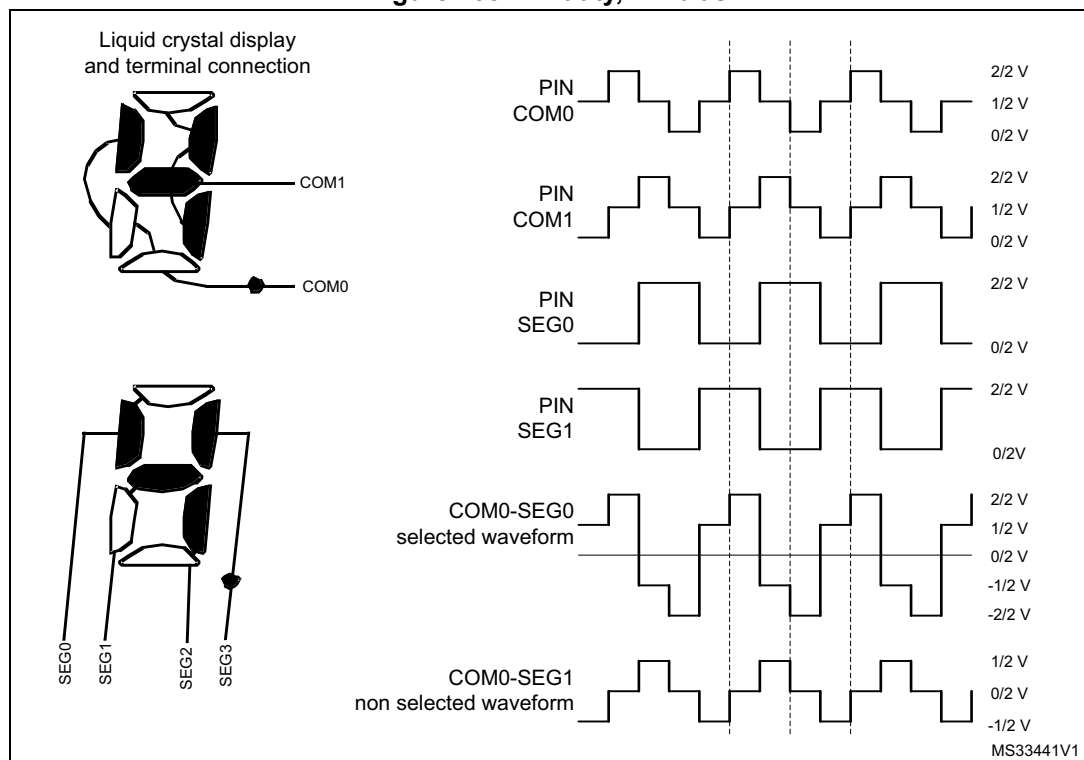
Figure 138. 1/2 duty, 1/2 bias
