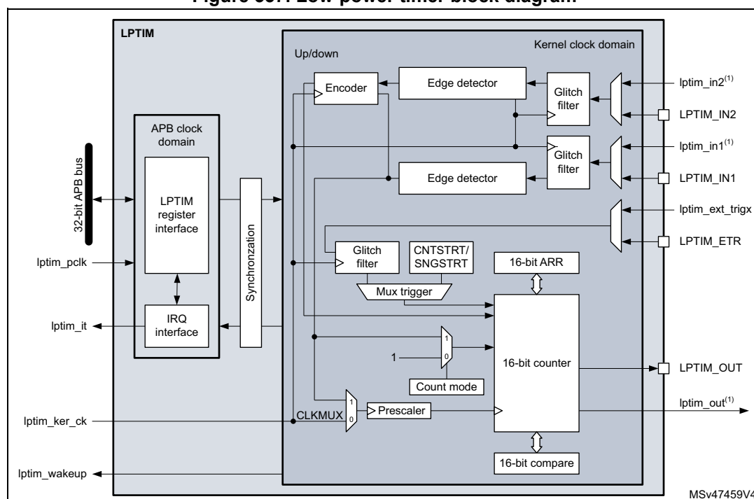
Figure 337. Low-power timer block diagram
