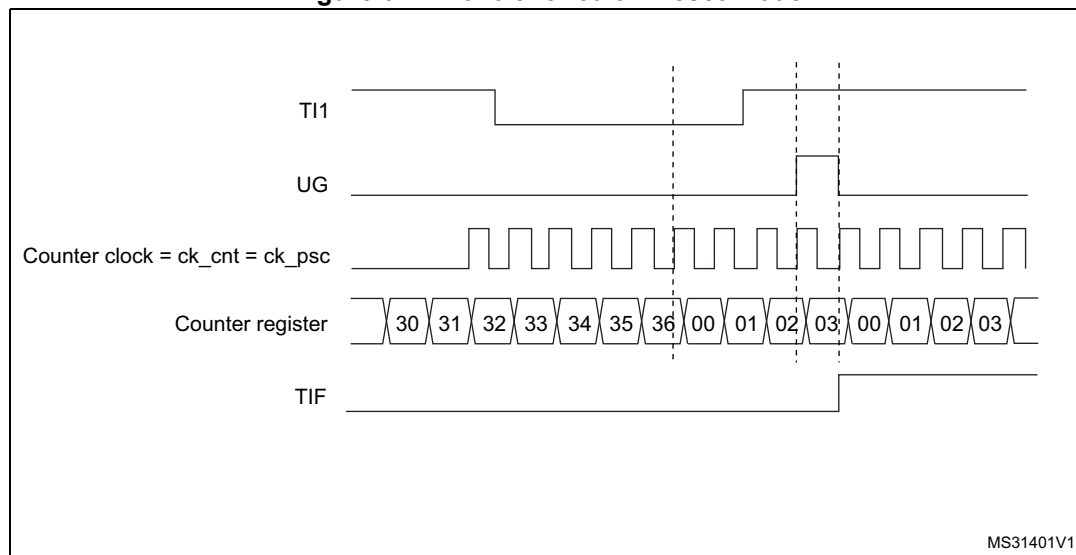
Figure 324. Control circuit in reset mode
