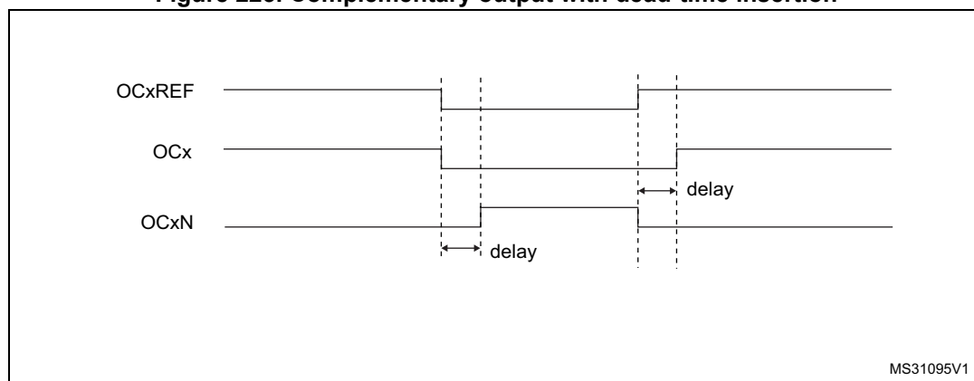
Figure 223. Complementary output with dead-time insertion
