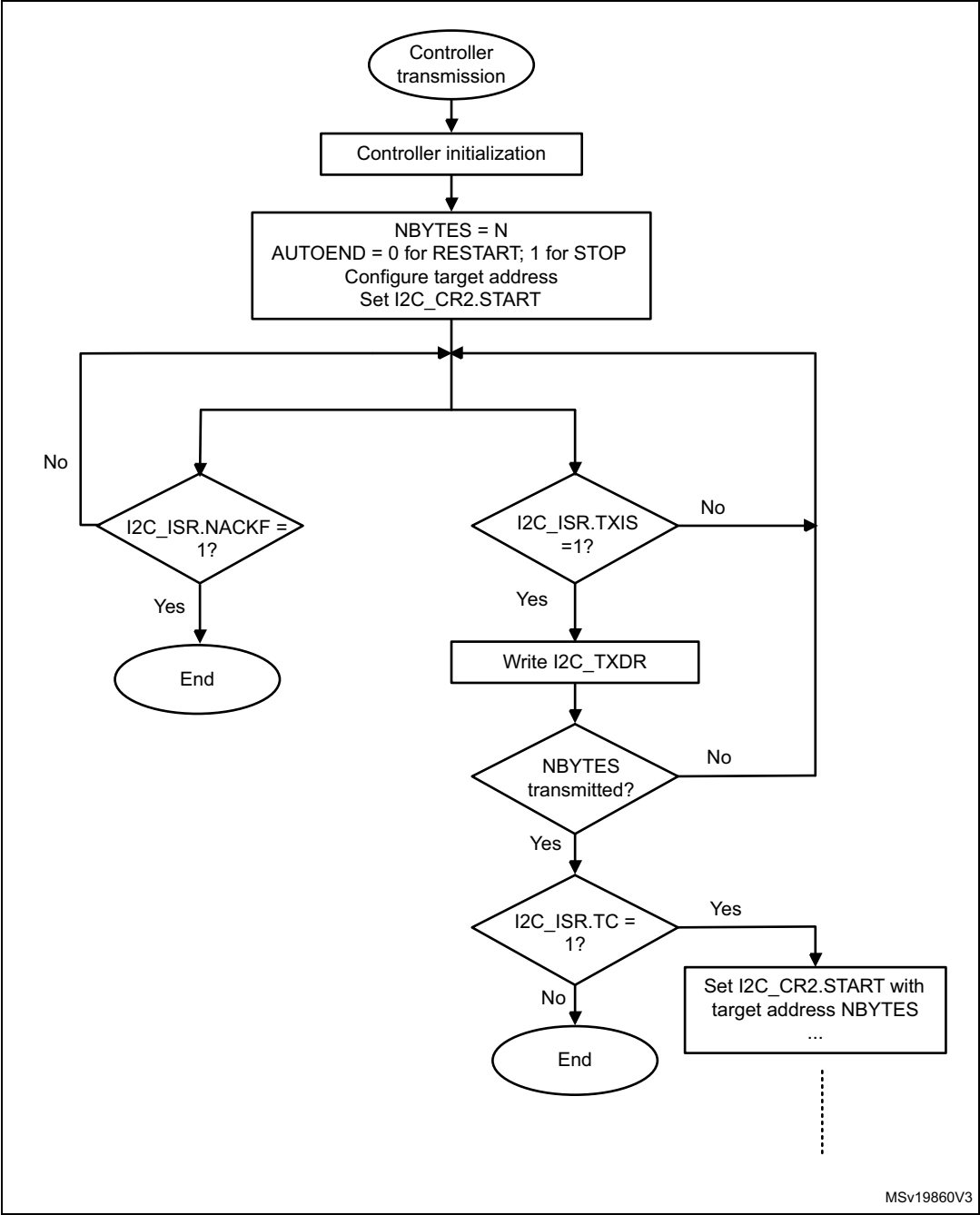
Figure 376. Transfer sequence flow for I2C controller transmitter, N \leq 255 bytes
