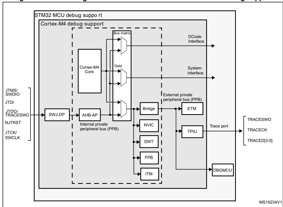
Figure 501. Block diagram of STM32 MCU and Cortex®-M4-level debug support
