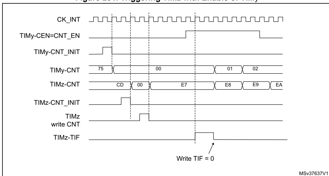
Figure 291. Triggering TIMz with Enable of TIMy
