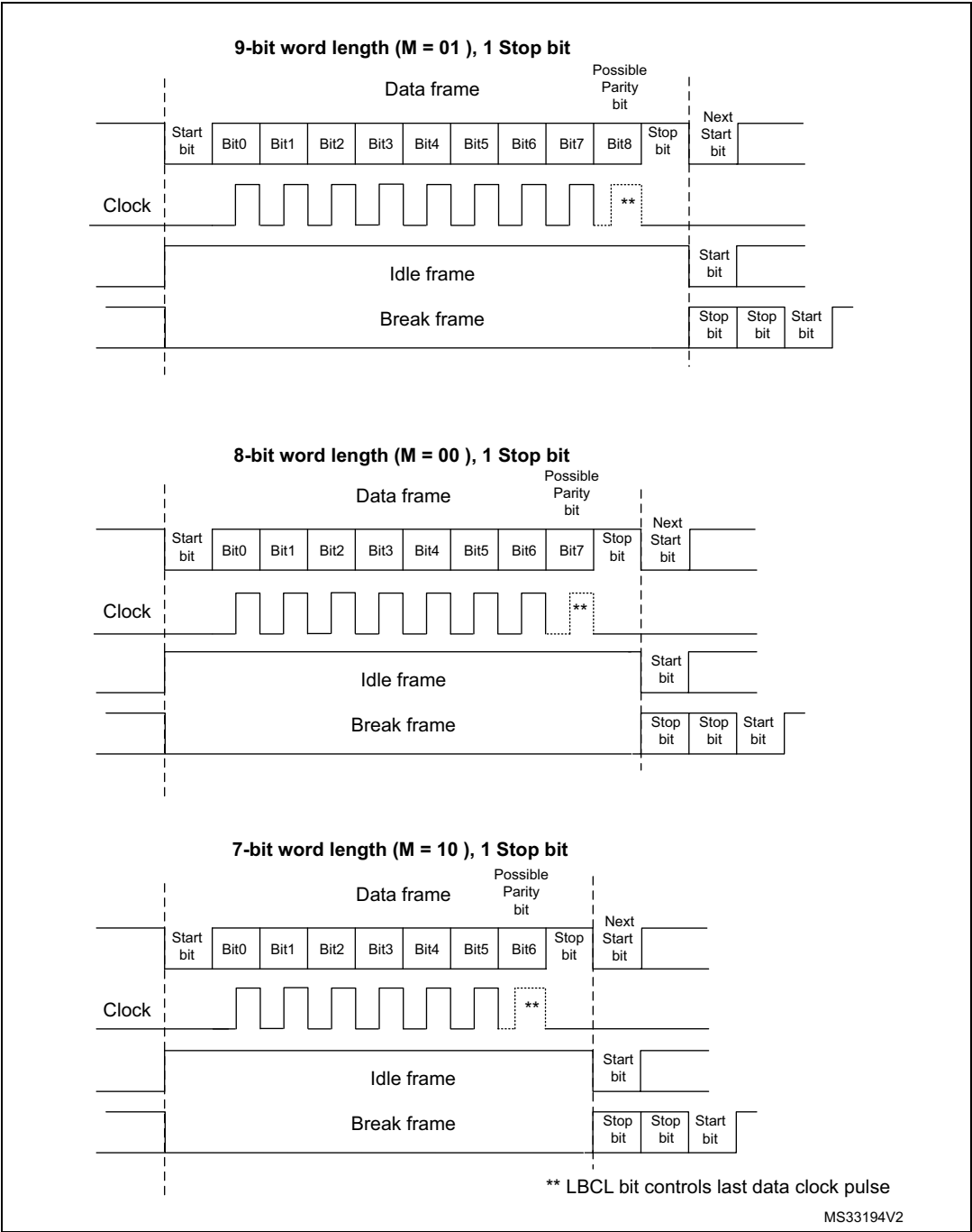
Figure 415. Word length programming
