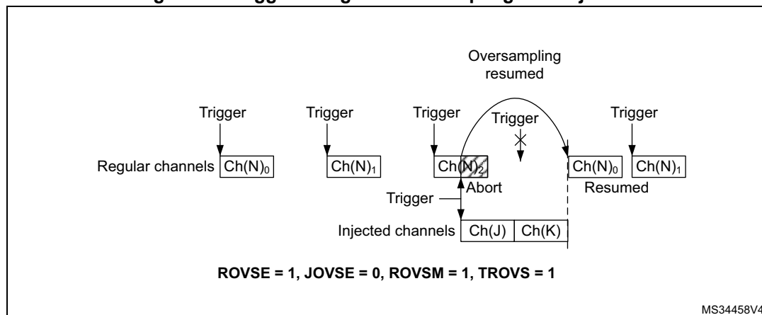
Figure 88. Triggered regular oversampling with injection
