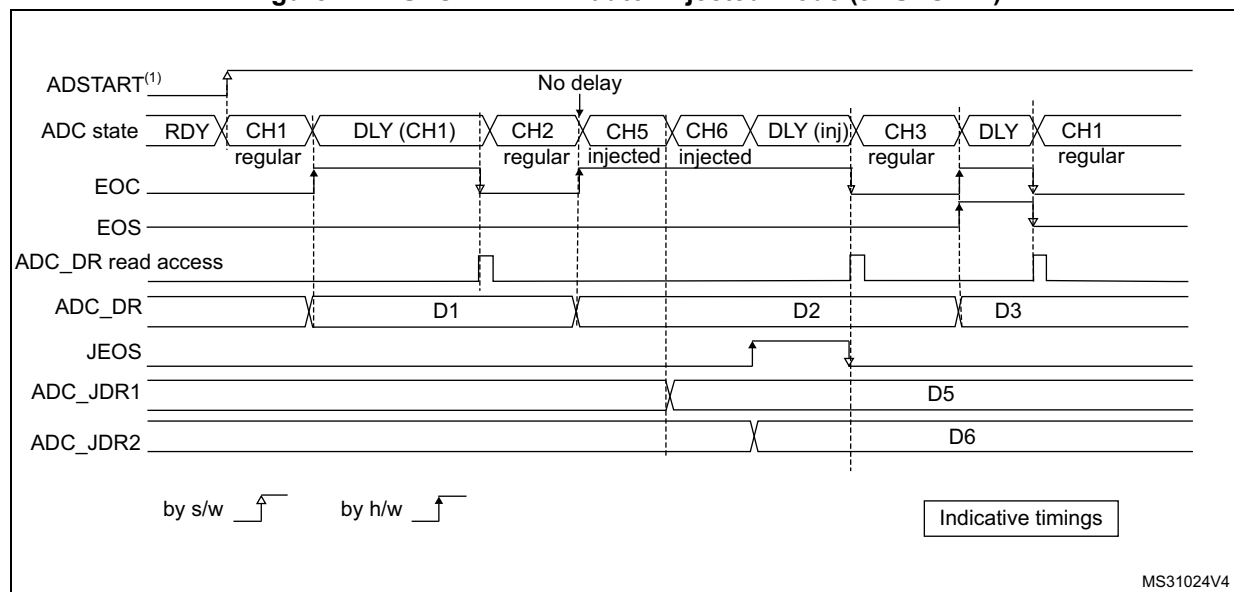
Figure 77. AUTODLY = 1 in auto-injected mode (JAUTO = 1)
