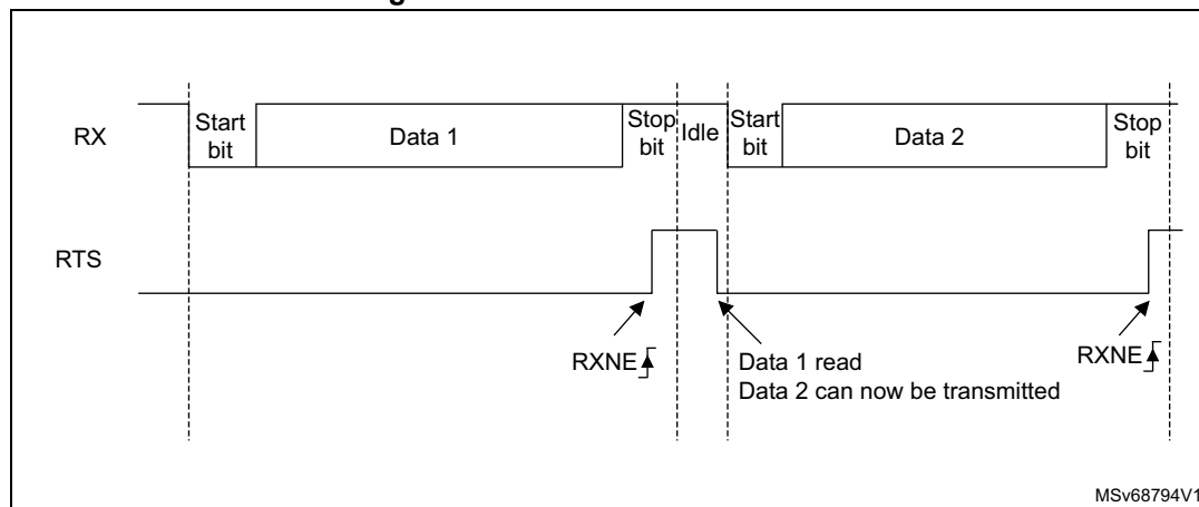
Figure 411. RS232 RTS flow control
