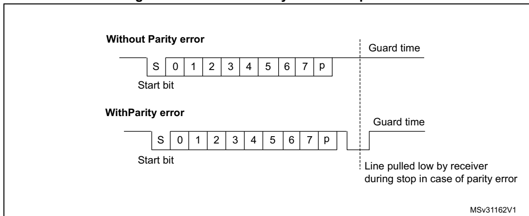
Figure 404. ISO 7816-3 asynchronous protocol
