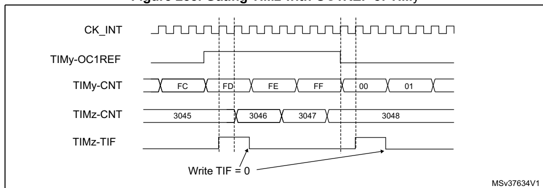
Figure 288. Gating TIMz with OC1REF of TIMy
