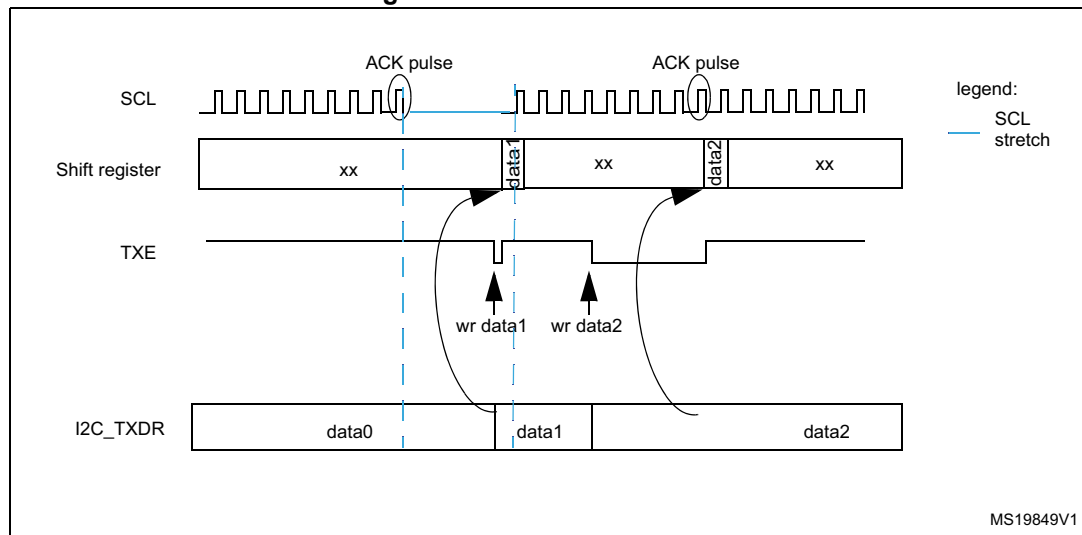
Figure 364. Data transmission
