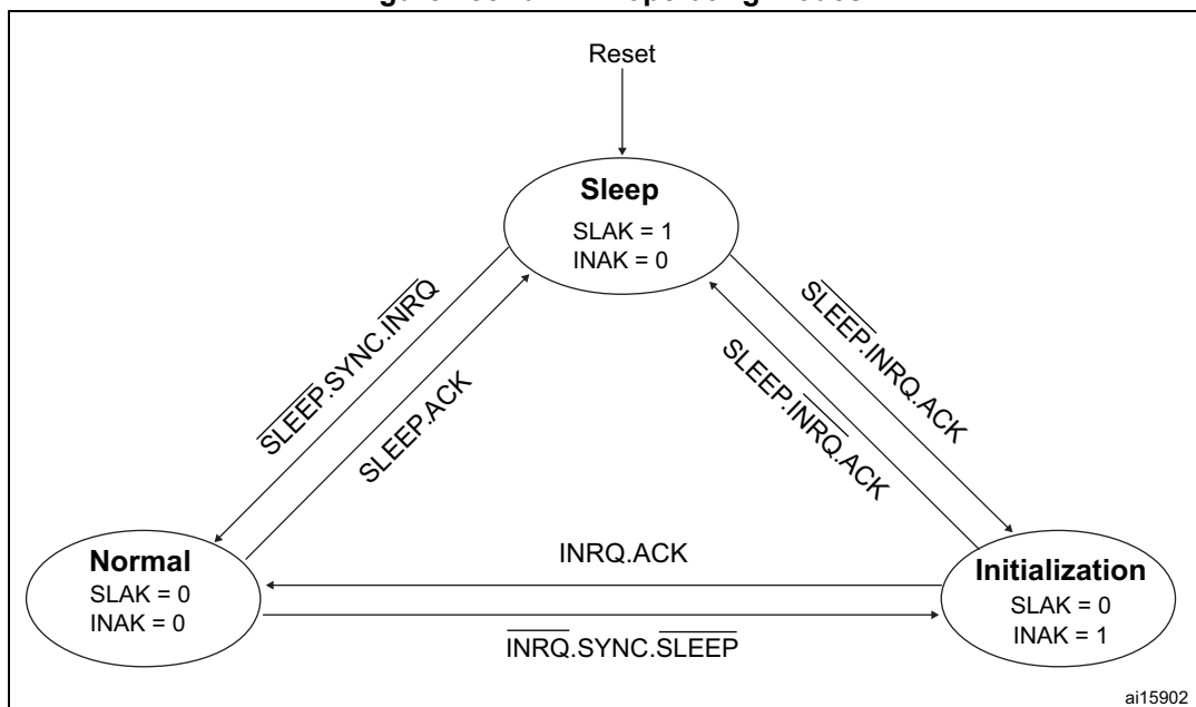
Figure 485. bxCAN operating modes
