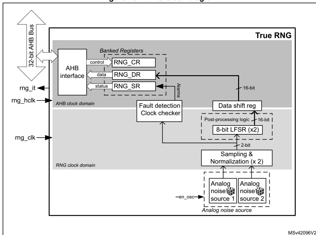
Figure 151. RNG block diagram
