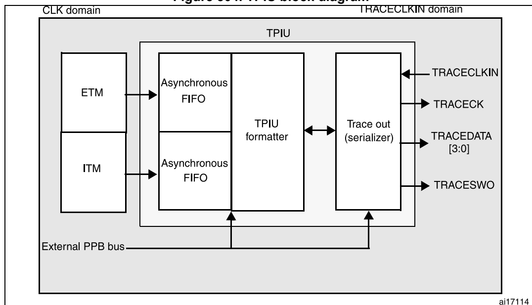
Figure 504. TPIU block diagram
