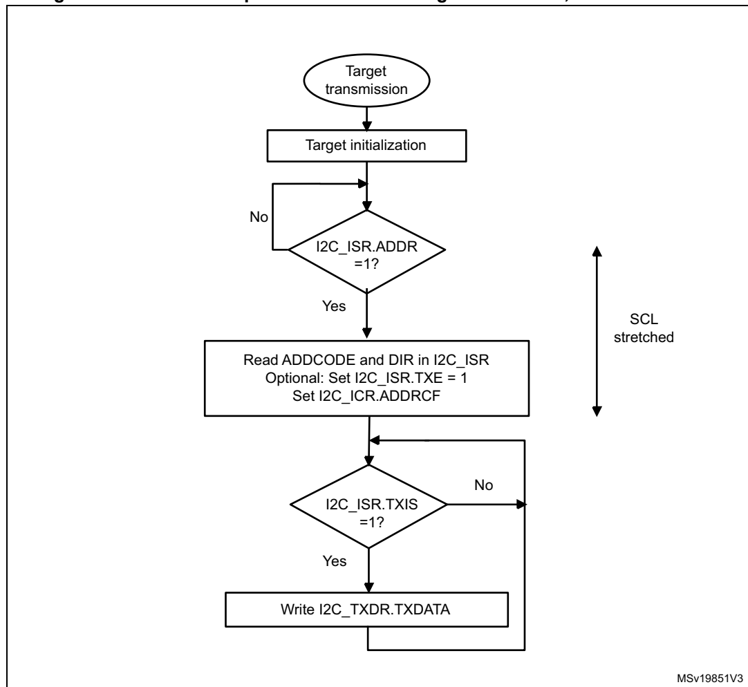
Figure 366. Transfer sequence flow for I2C target transmitter, NOSTRETCH = 0
