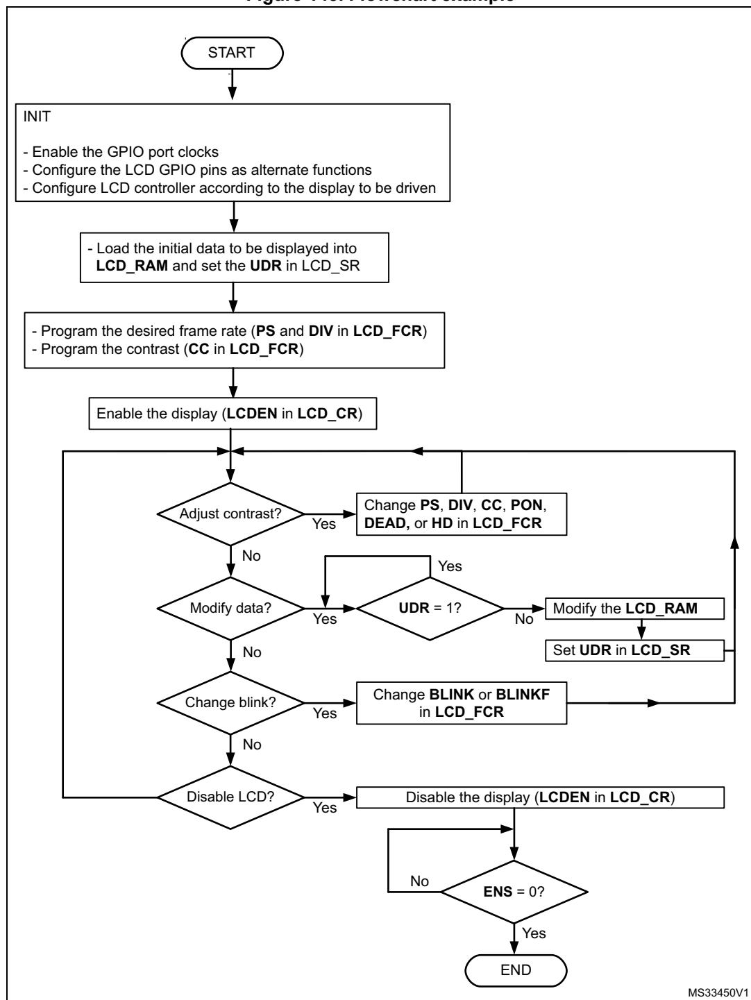
Figure 145. Flowchart example
