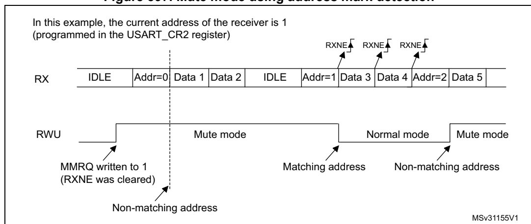
Figure 397. Mute mode using address mark detection
