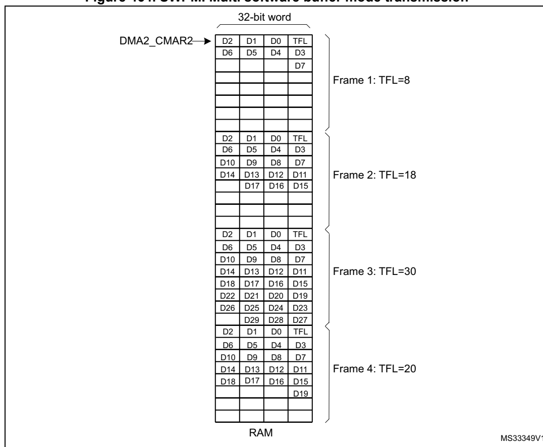
Figure 464. SWPMI Multi software buffer mode transmission
