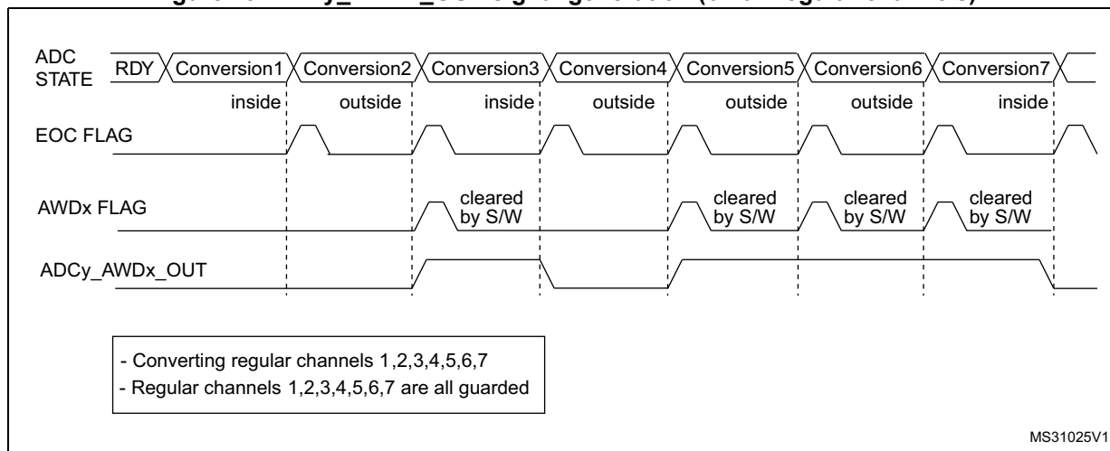
Figure 79. ADCy_AWDx_OUT signal generation (on all regular channels)
