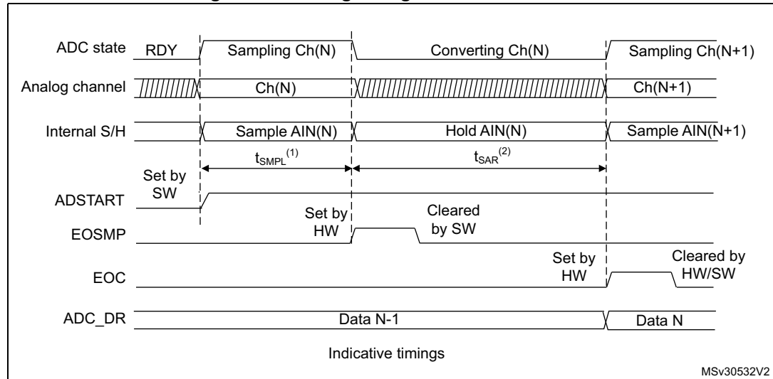
Figure 47. Analog-to-digital conversion time
