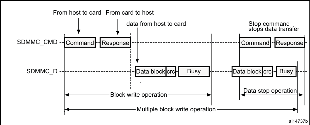
Figure 471. (Multiple) block write operation
