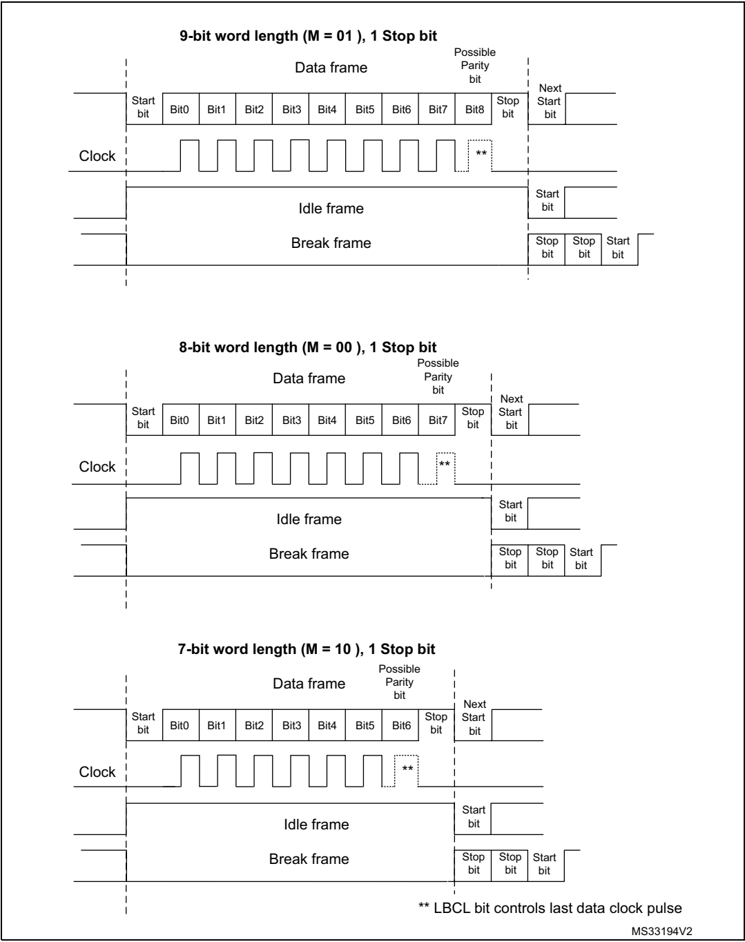
Figure 390. Word length programming
