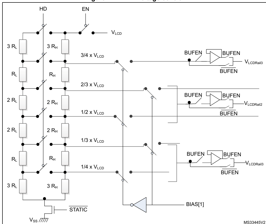
Figure 142. LCD voltage control
