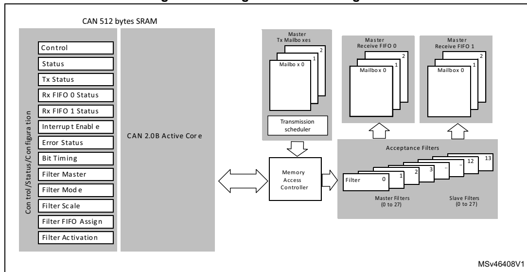
Figure 484. Single-CAN block diagram
