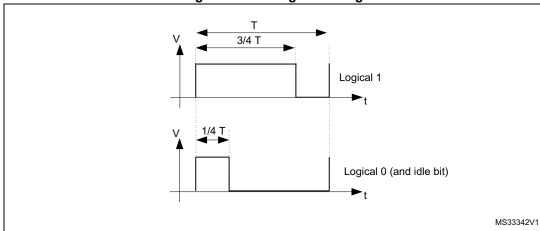
Figure 457. S1 signal coding
