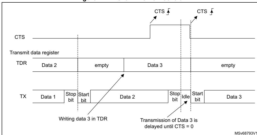
Figure 424. RS232 CTS flow control
