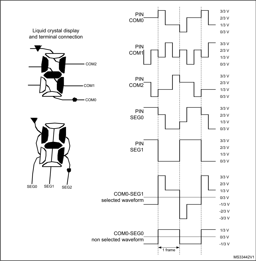
Figure 139. 1/3 duty, 1/3 bias
