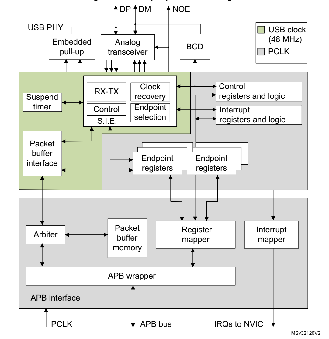
Figure 499. USB peripheral block diagram
