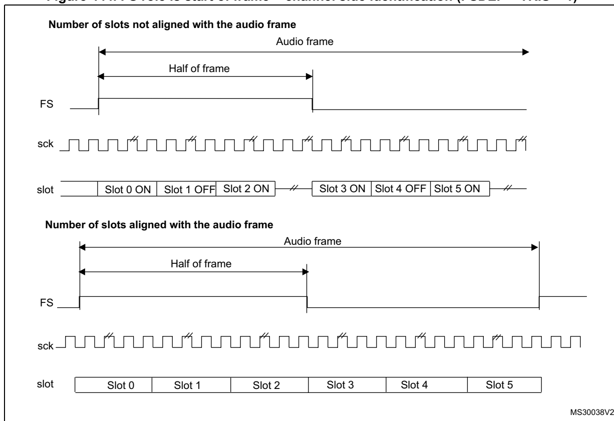
Figure 444. FS role is start of frame + channel side identification (FSDEF = TRIS = 1)
