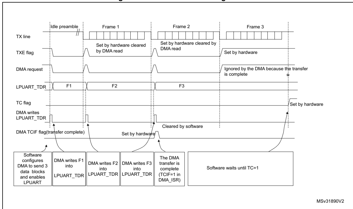
Figure 420. Transmission using DMA
