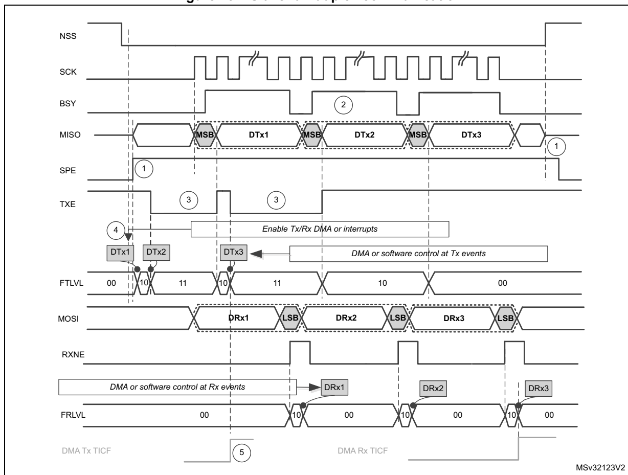
Figure 437. Slave full-duplex communication
