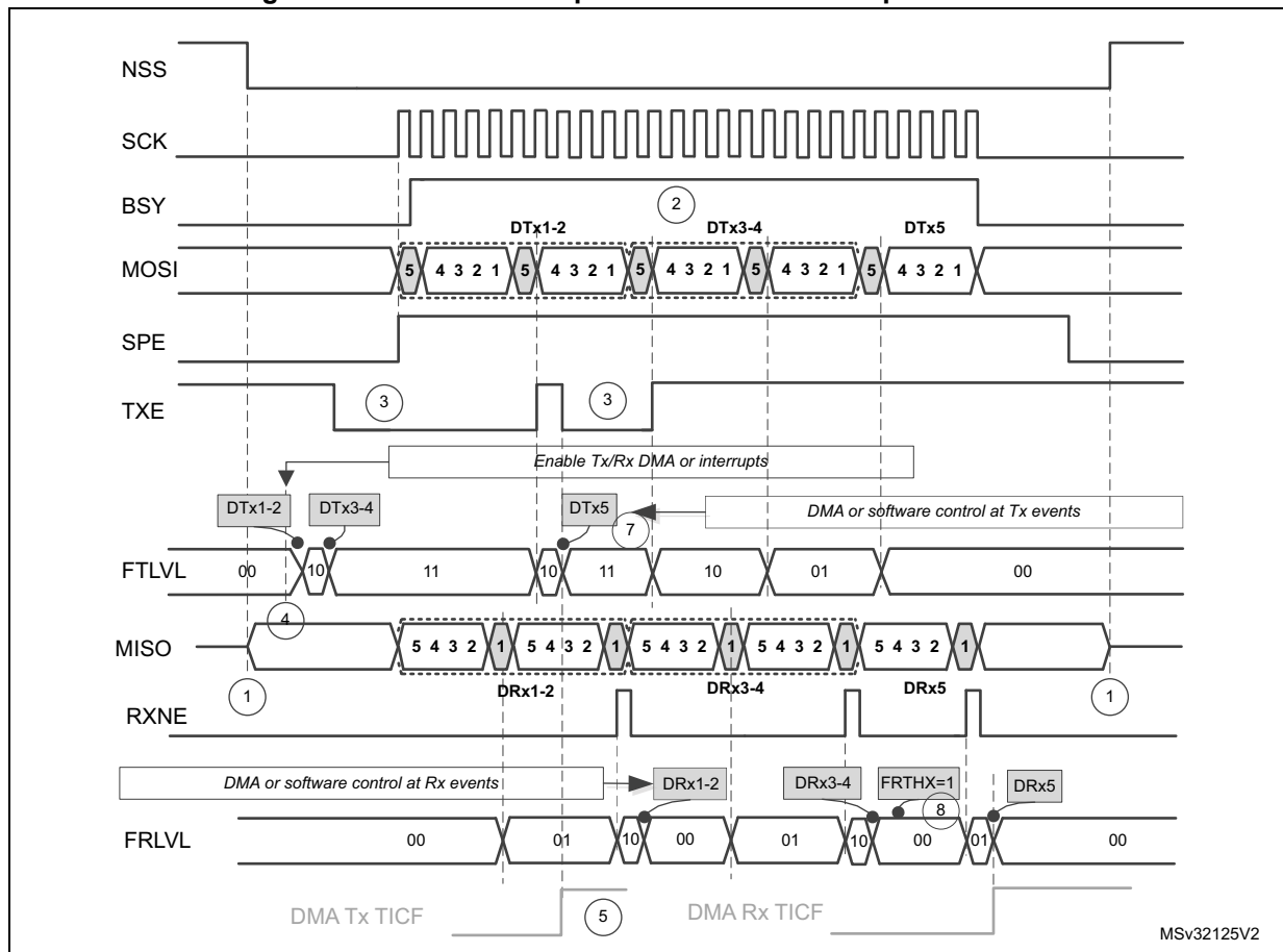
Figure 439. Master full-duplex communication in packed mode
