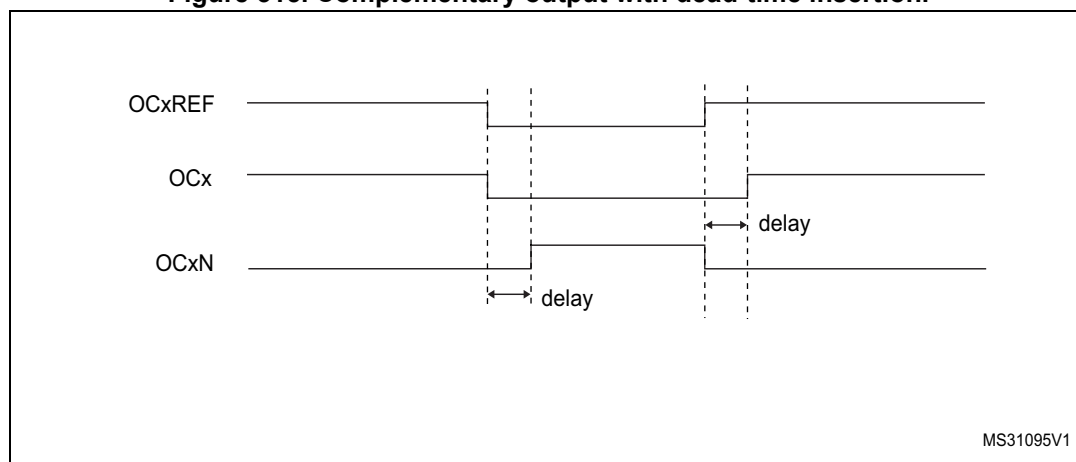
Figure 315. Complementary output with dead-time insertion.
