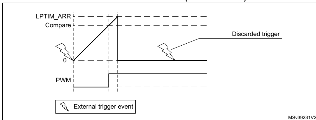
Figure 347. LPTIM output waveform, single-counting mode configuration and Set-once mode activated (WAVE bit is set)
