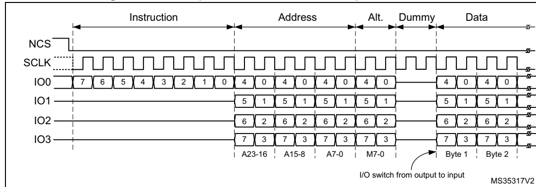
Figure 33. Example of read command in quad-SPI mode
