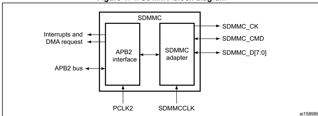
Figure 474. SDMMC block diagram
