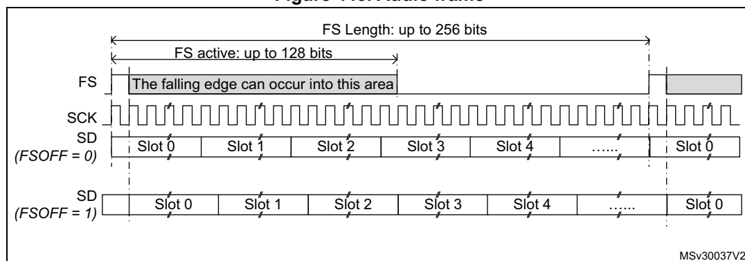
Figure 443. Audio frame
