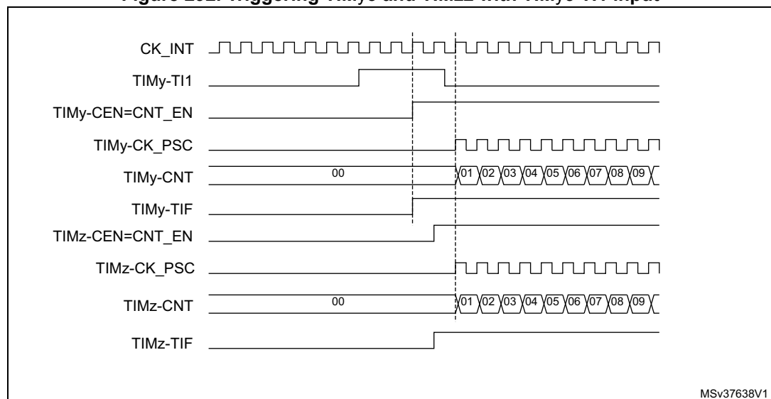
Figure 292. Triggering TIMy3 and TIMz2 with TIMy3 TI1 input
