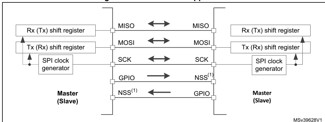
Figure 431. Multimaster application
