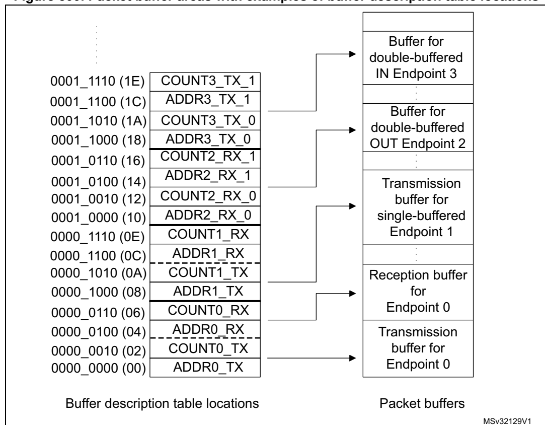
Figure 500. Packet buffer areas with examples of buffer description table locations
