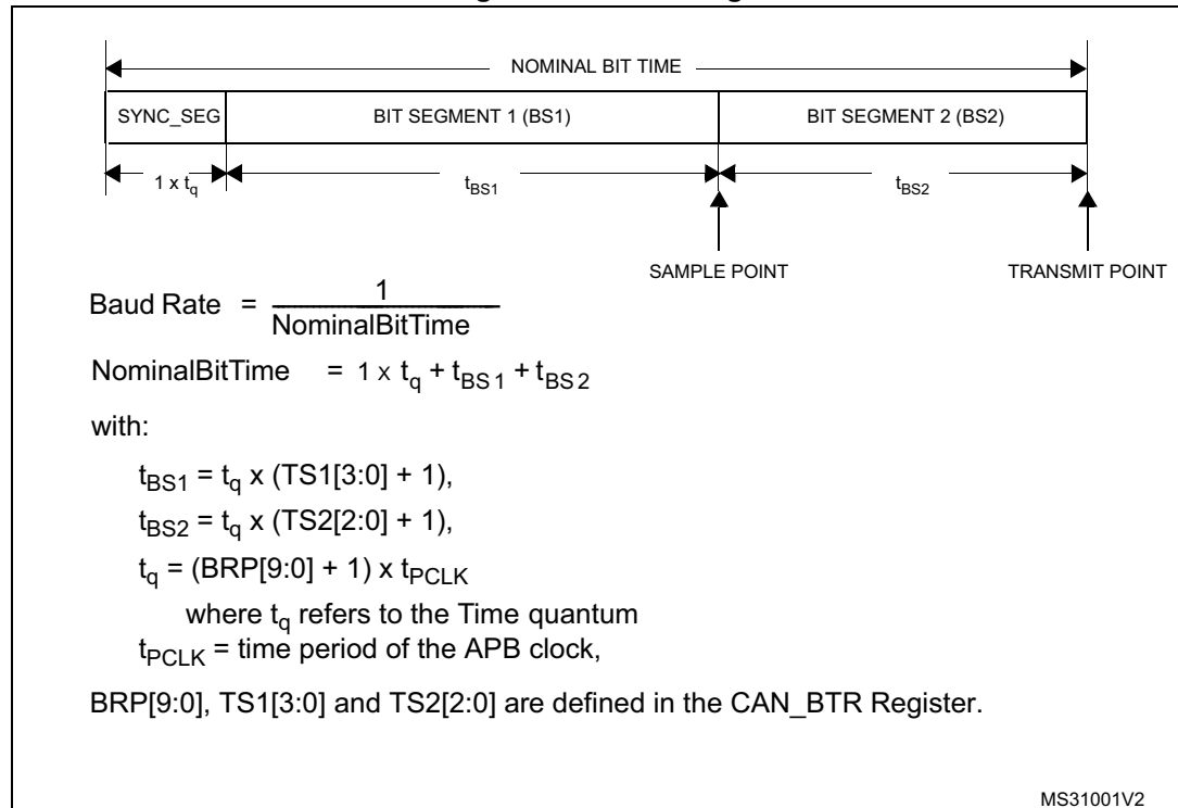
Figure 495. Bit timing
