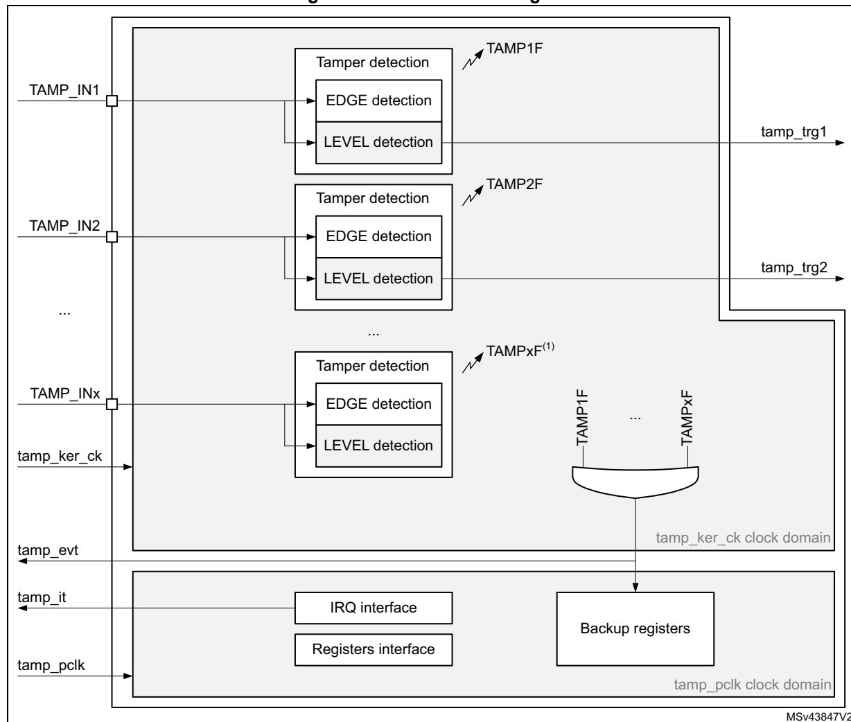
Figure 357. TAMP block diagram
