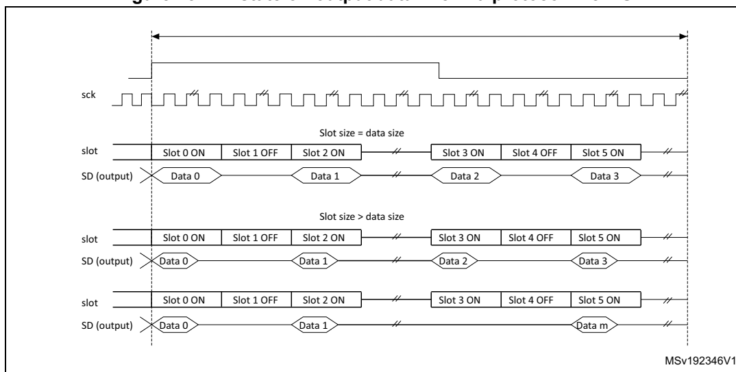
Figure 454. Tristate on output data line in a protocol like I2S
