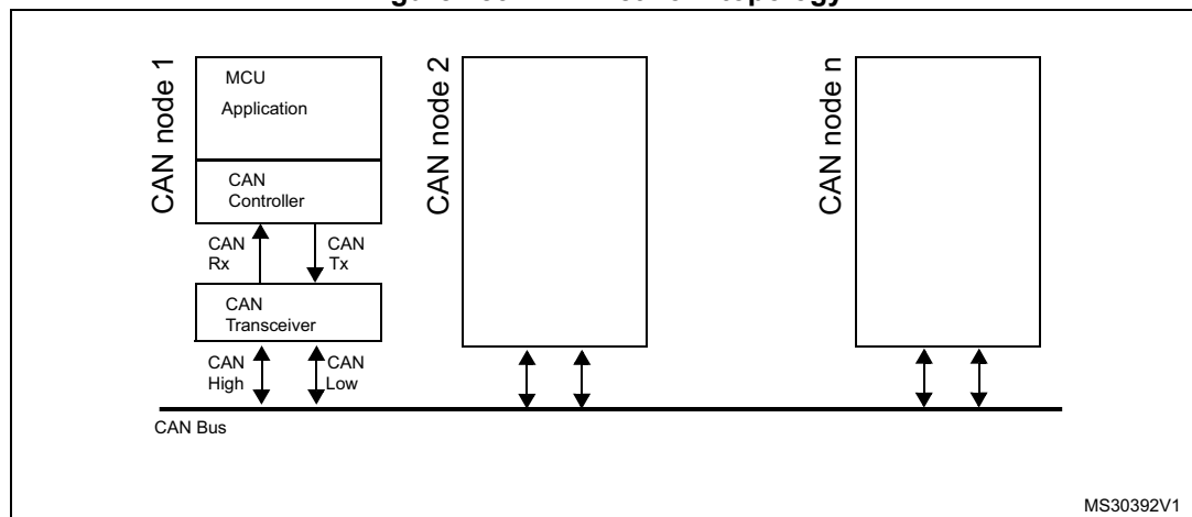
Figure 483. CAN network topology
