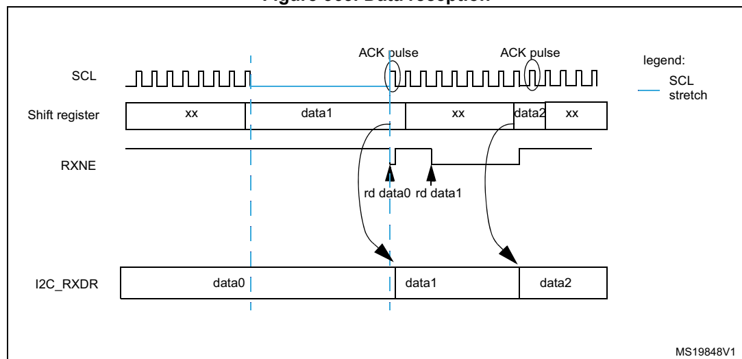
Figure 363. Data reception
