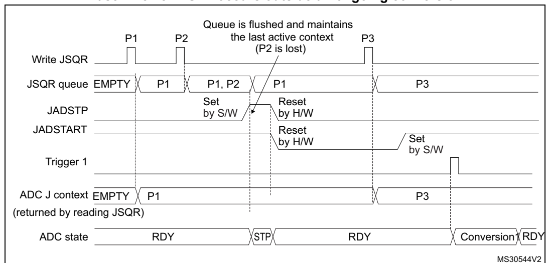
Figure 60. Flushing JSQR queue of context by setting JADSTP = 1 (JQM = 0) Case when JADSTP occurs outside an ongoing conversion
