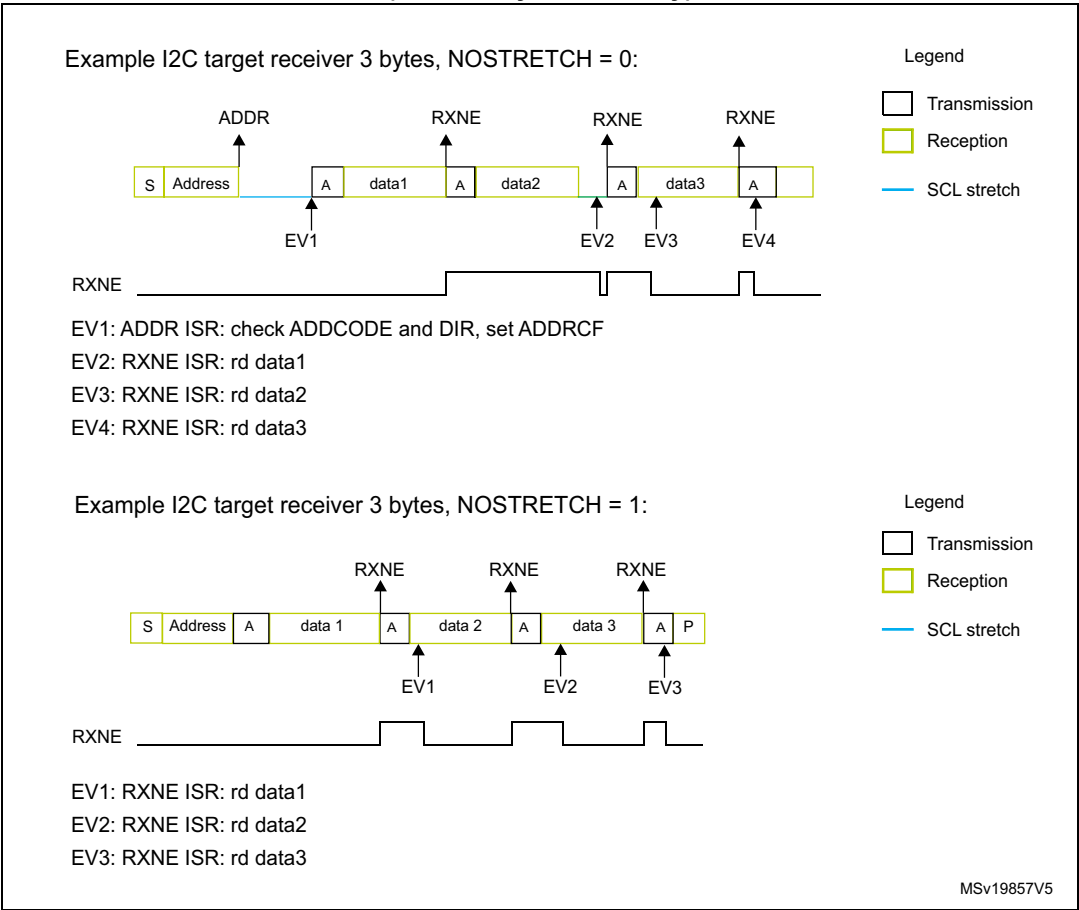
Figure 371. Transfer bus diagrams for I2C target receiver (mandatory events only)
