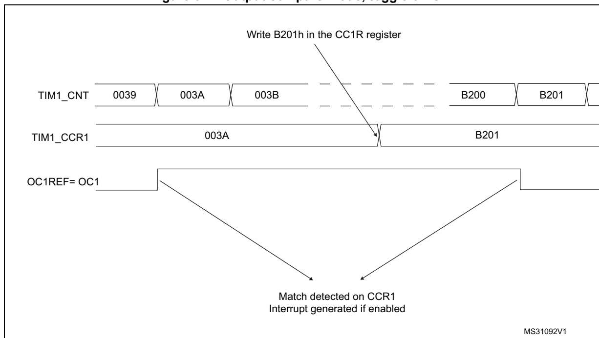
Figure 312. Output compare mode, toggle on OC1
