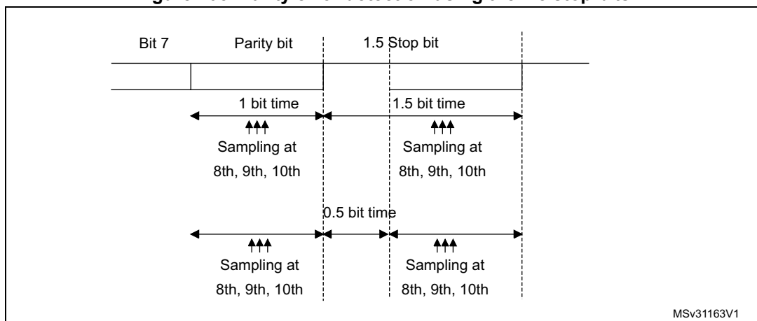
Figure 405. Parity error detection using the 1.5 stop bits
