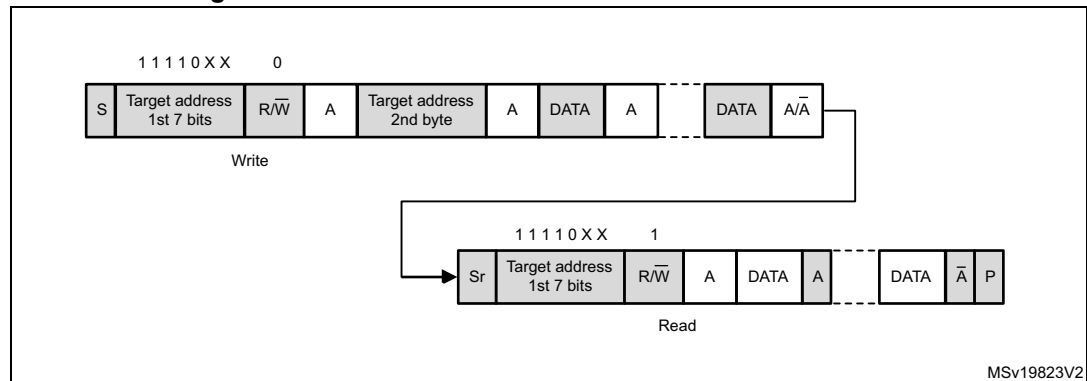
Figure 375. 10-bit address read access with HEAD10R = 1
