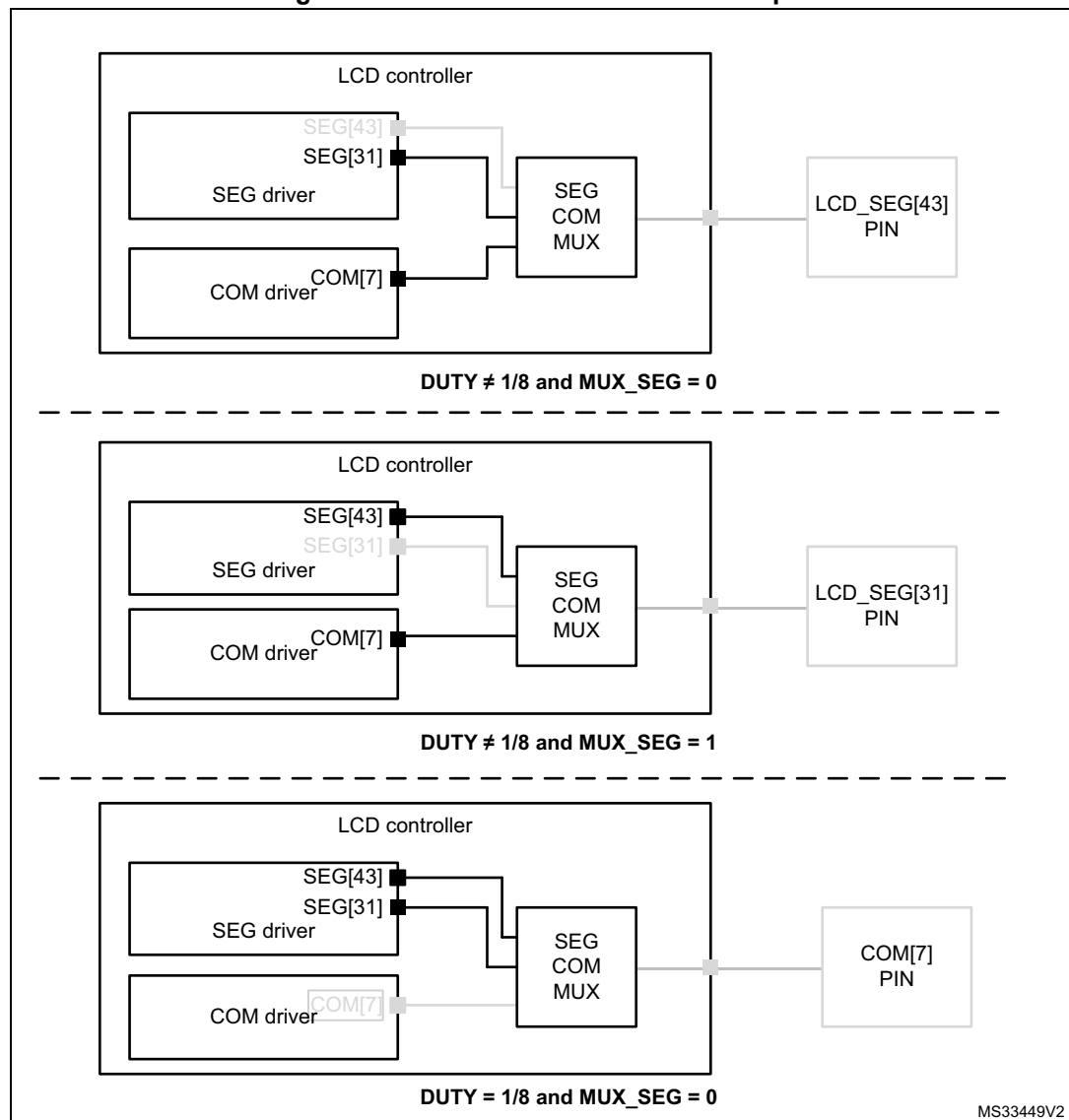
Figure 144. SEG/COM mux feature example
