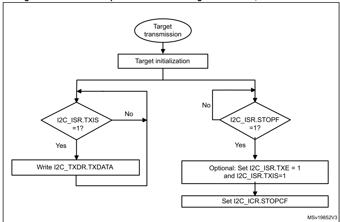
Figure 367. Transfer sequence flow for I2C target transmitter, NOSTRETCH = 1
