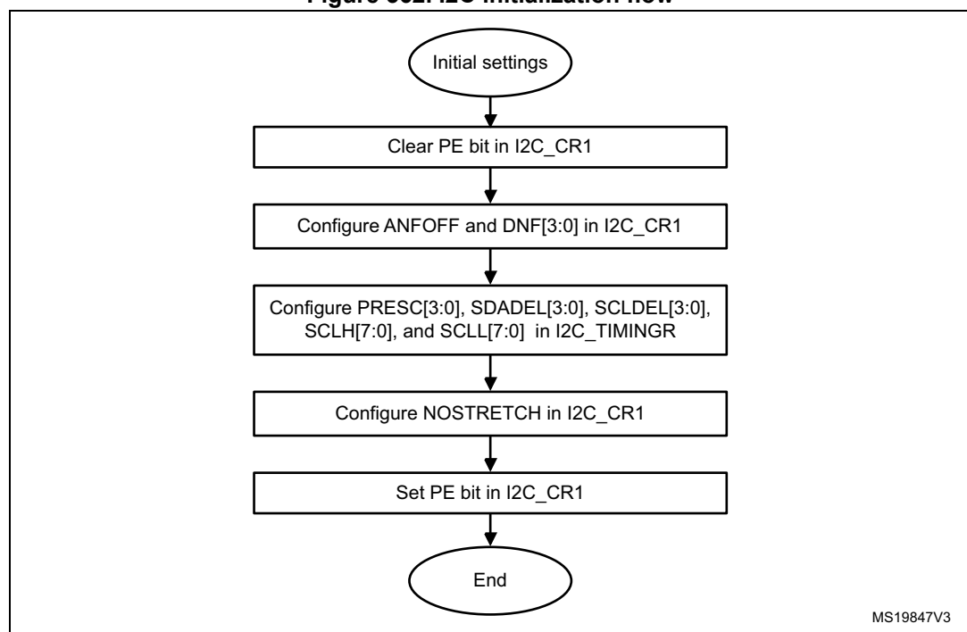
Figure 362. I2C initialization flow
