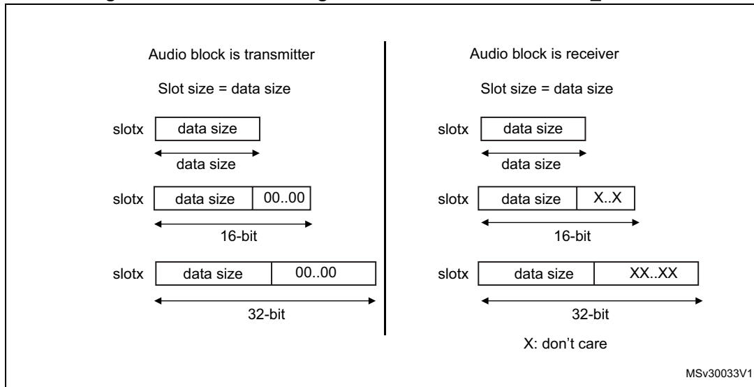
Figure 446. Slot size configuration with FBOFF = 0 in SAI_xSLOTR
