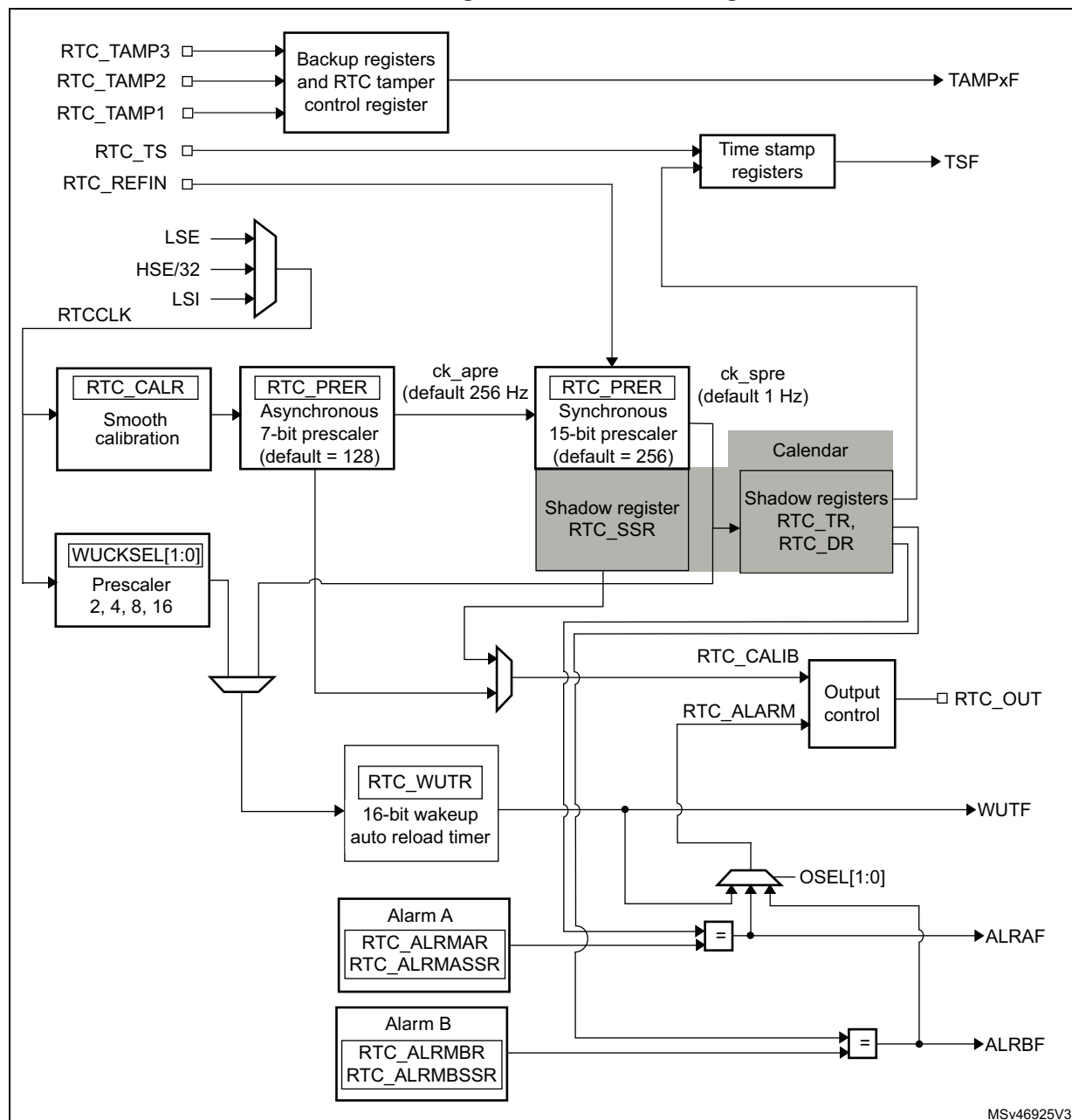
Figure 358. RTC block diagram
