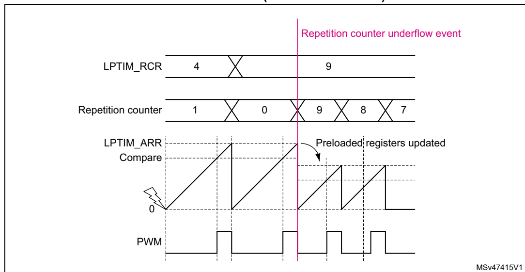
Figure 351. Continuous counting mode when repetition register LPTIM_RCR different from zero (with PRELOAD = 1)
