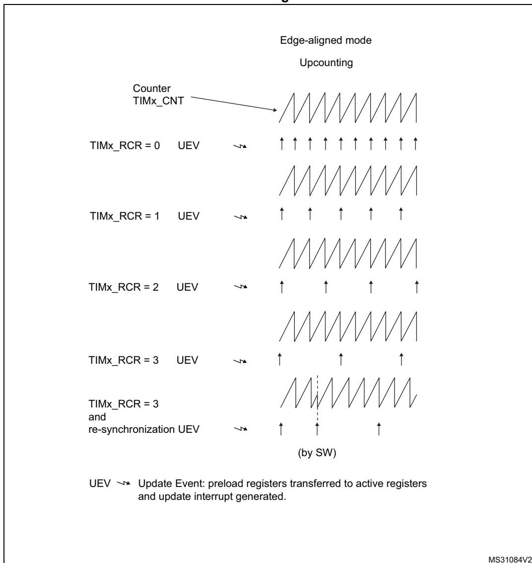
Figure 303. Update rate examples depending on mode and TIMx_RCR register settings
