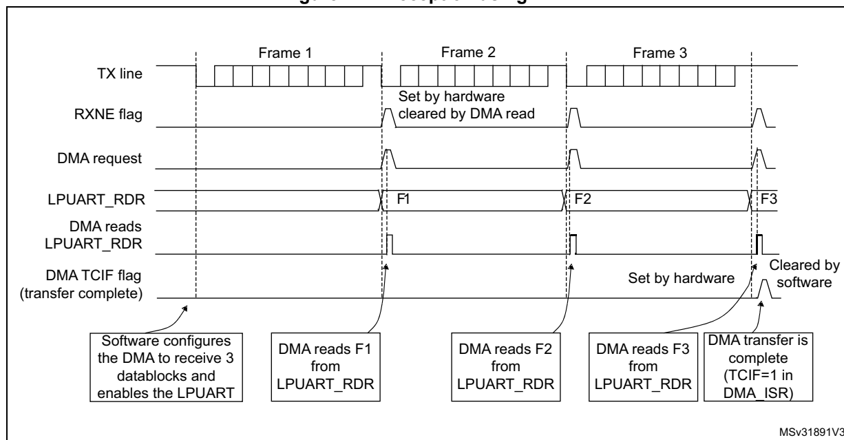
Figure 421. Reception using DMA
