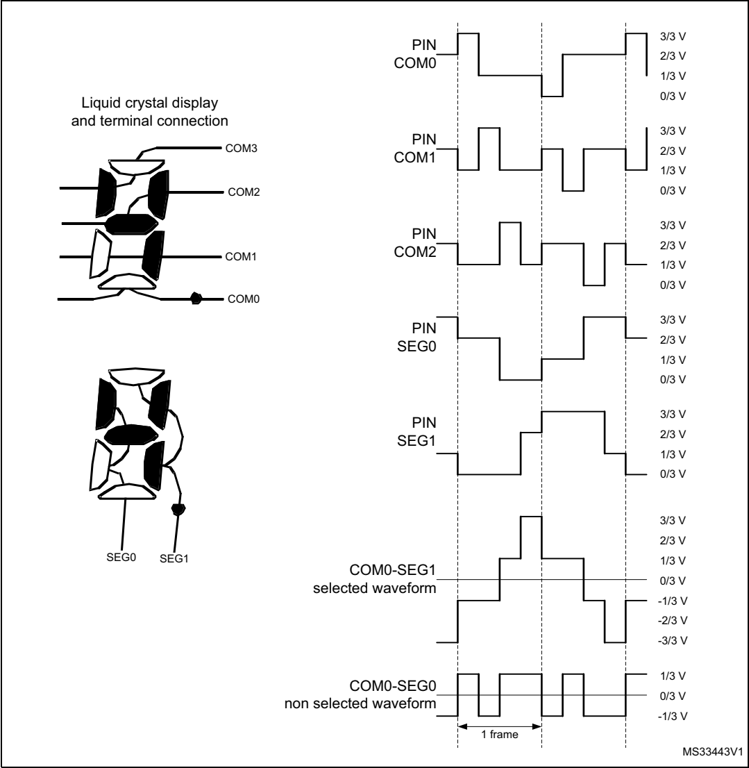
Figure 140. 1/4 duty, 1/3 bias
