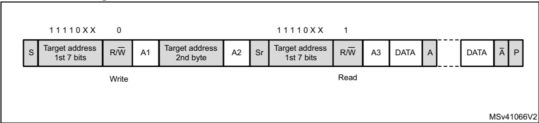
Figure 374. 10-bit address read access with HEAD10R = 0
