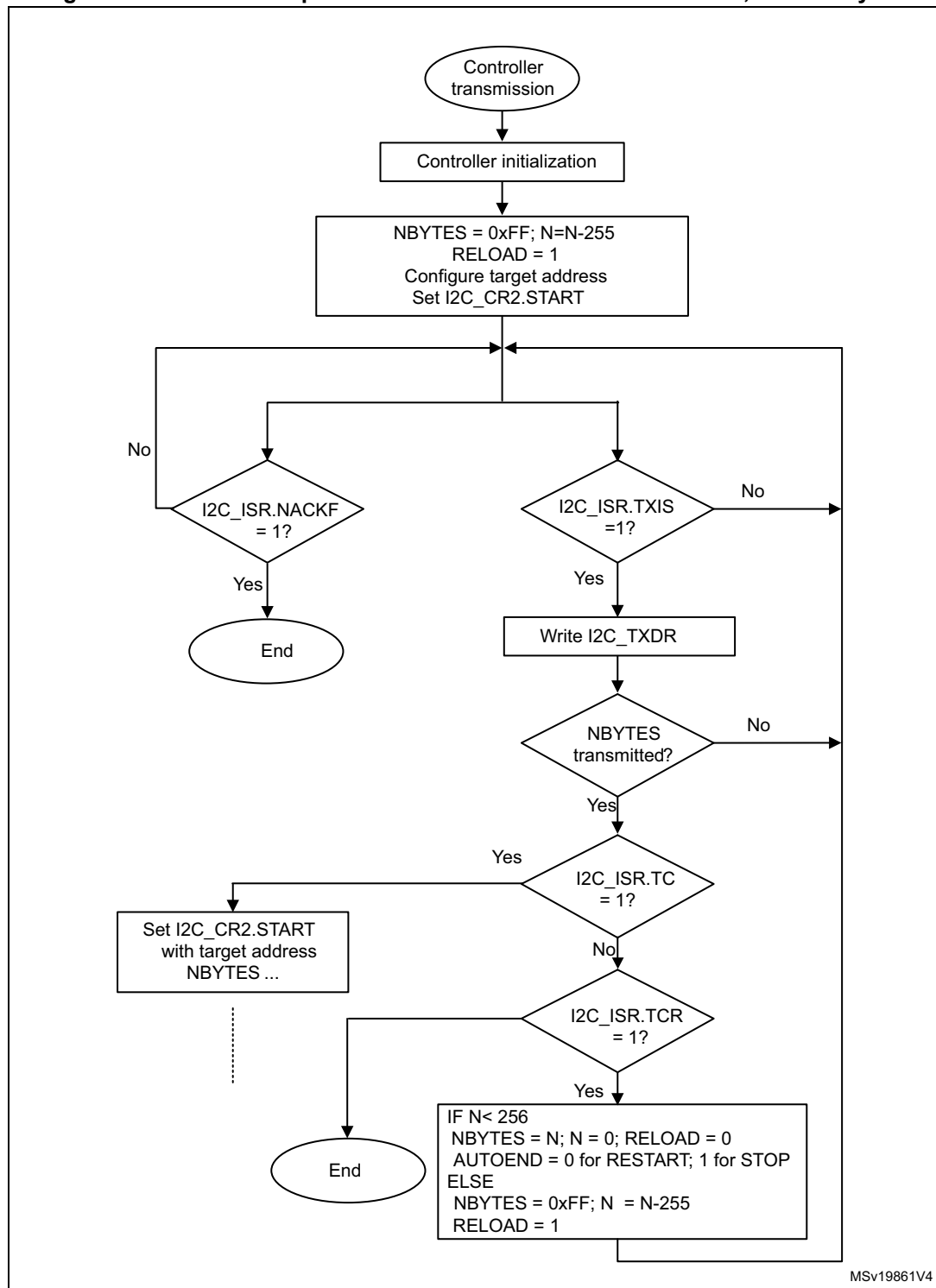
Figure 377. Transfer sequence flow for I2C controller transmitter, N > 255 bytes
