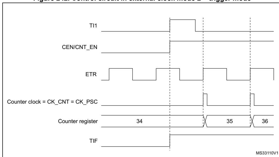
Figure 242. Control circuit in external clock mode 2 + trigger mode
