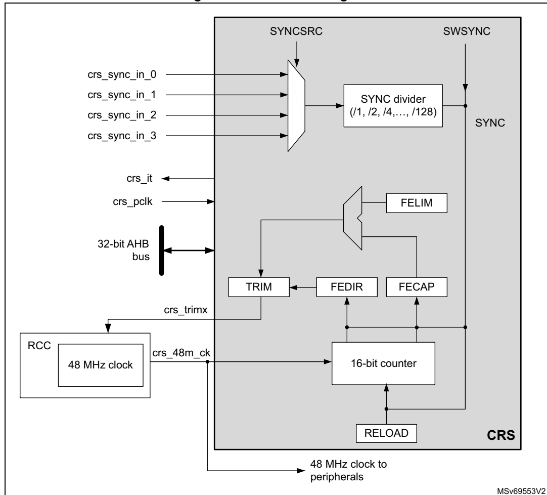
Figure 17. CRS block diagram
