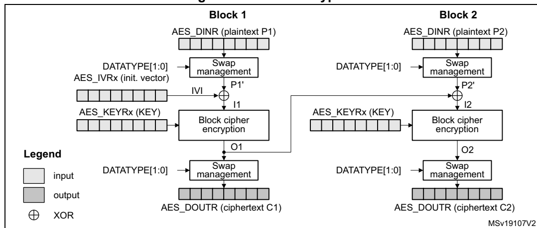
Figure 166. CBC encryption
