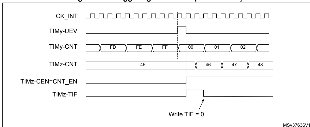
Figure 290. Triggering TIMz with update of TIMy
