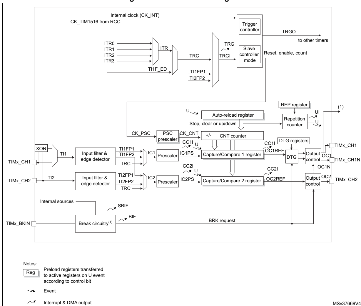
Figure 293. TIM15 block diagram
