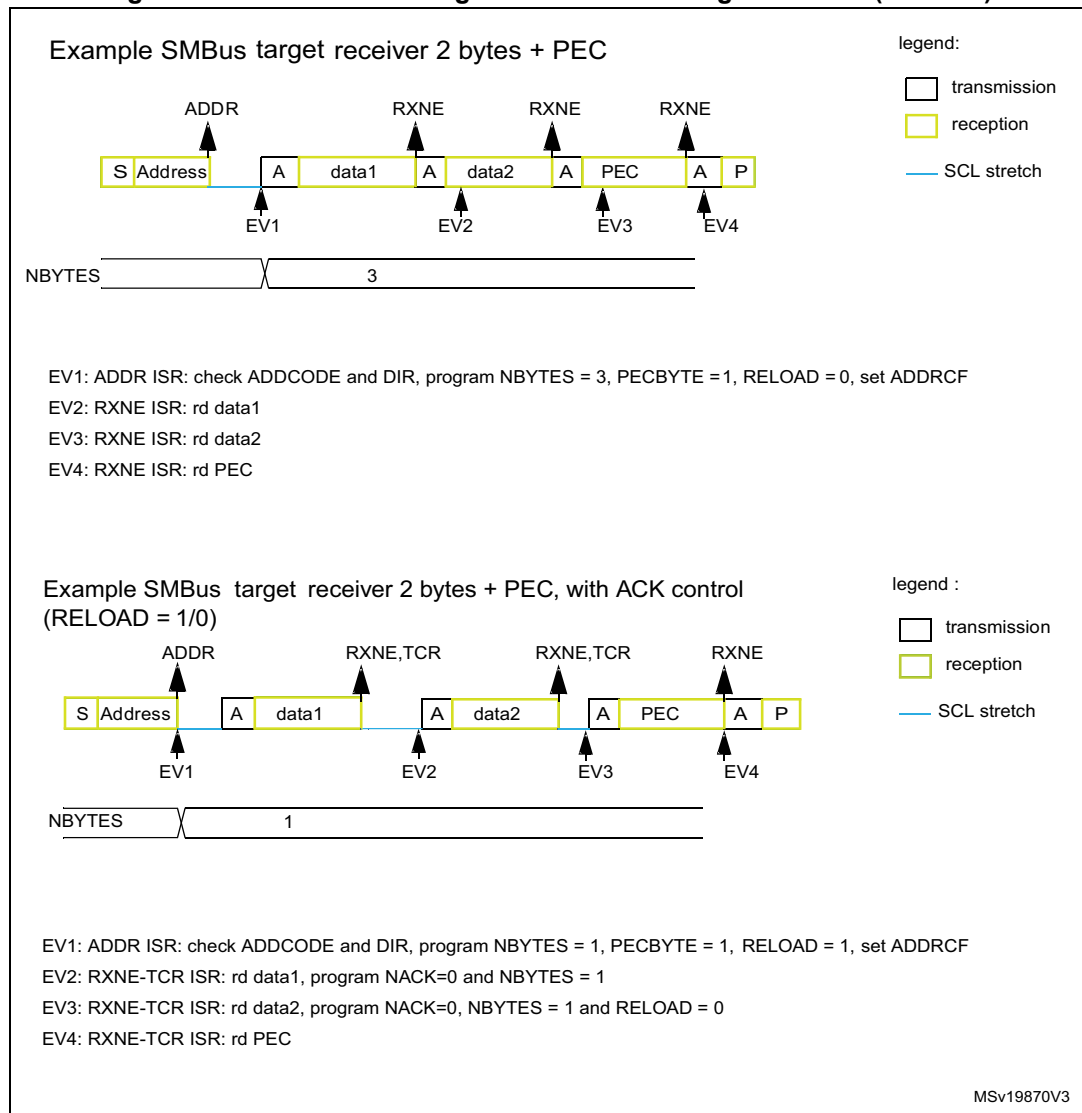
Figure 386. Bus transfer diagrams for SMBus target receiver (SBC = 1)
