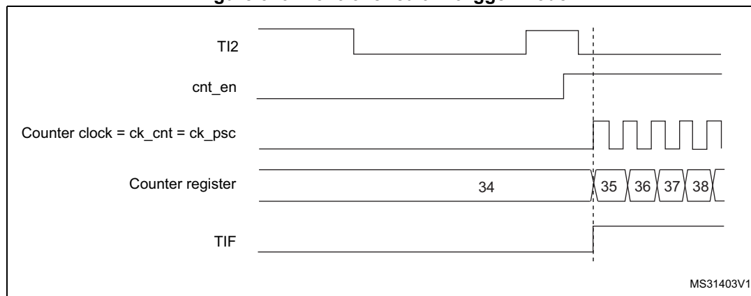
Figure 326. Control circuit in trigger mode
