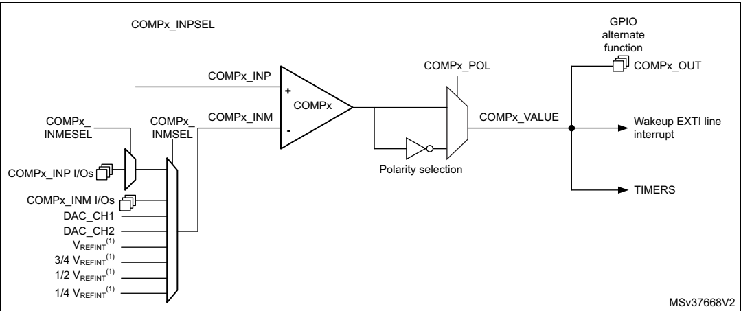
Figure 118. Comparator block diagram
