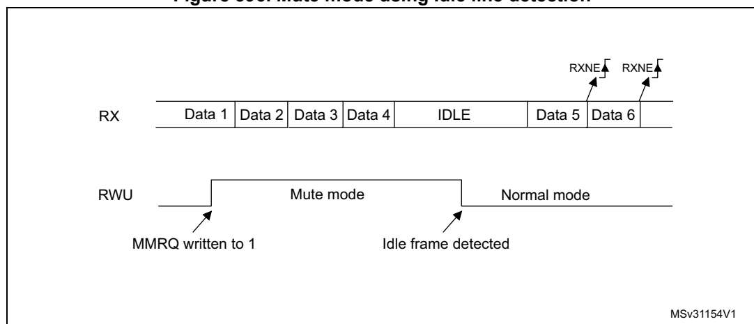
Figure 396. Mute mode using Idle line detection
