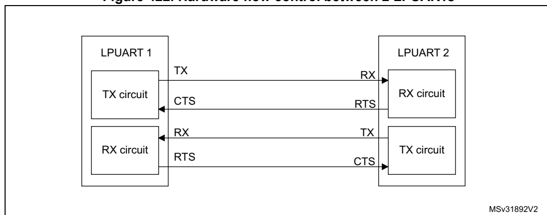
Figure 422. Hardware flow control between 2 LPUARTs
