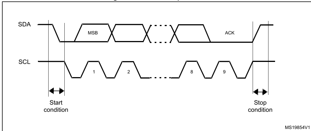
Figure 360. I 2 C-bus protocol
