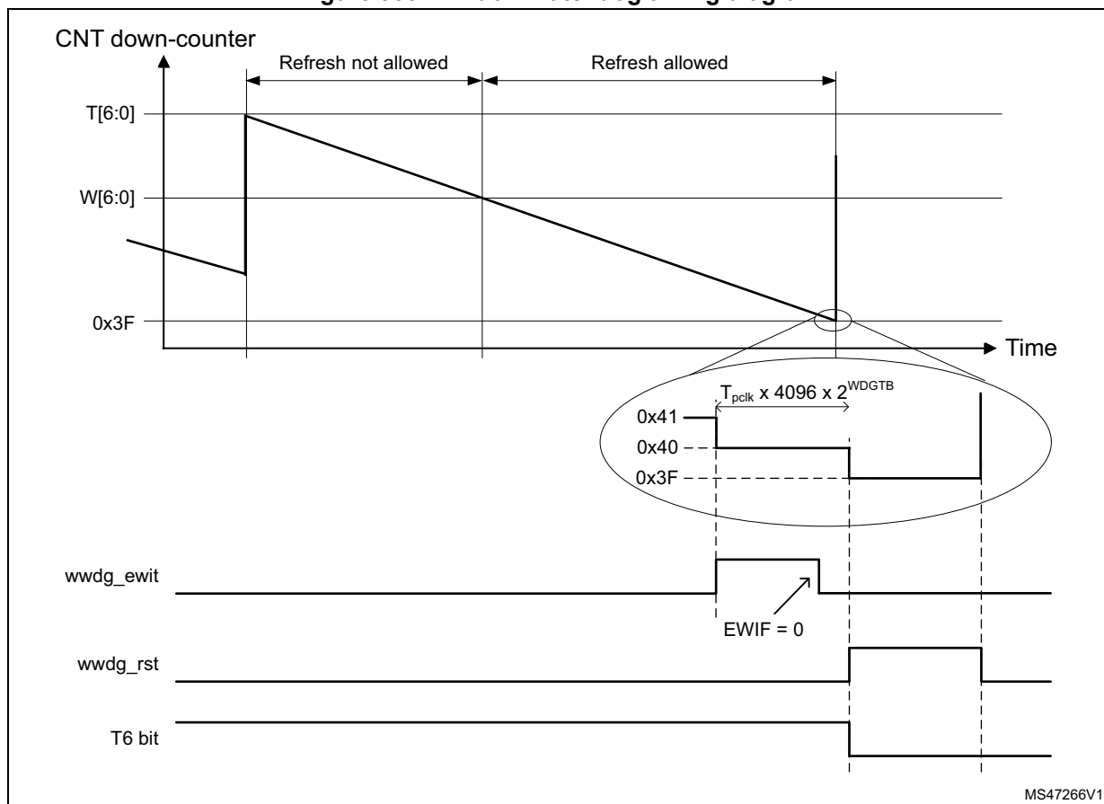
Figure 355. Window watchdog timing diagram
