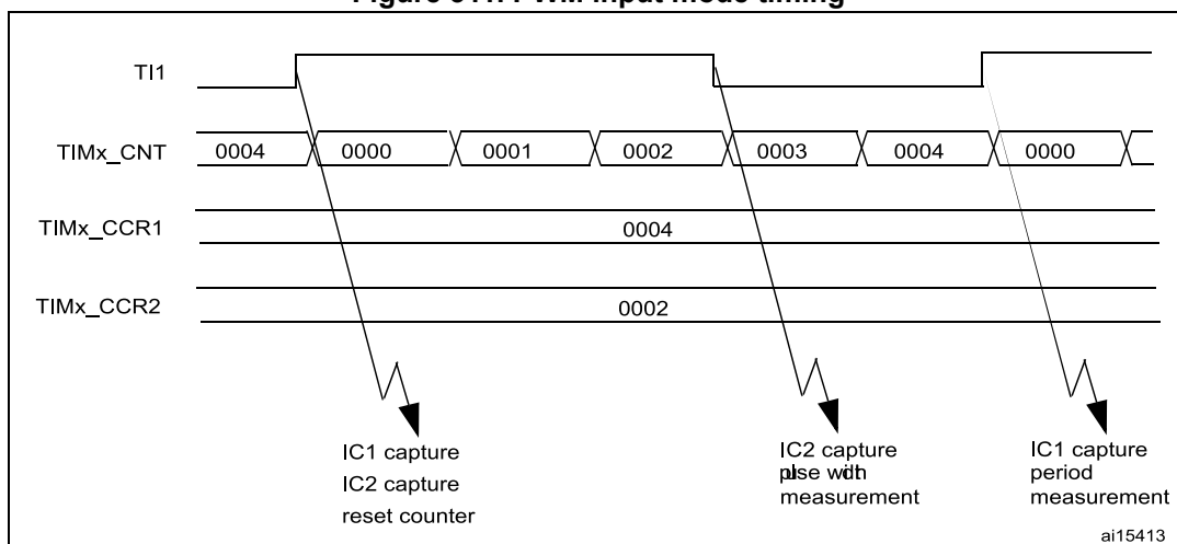
Figure 311. PWM input mode timing
