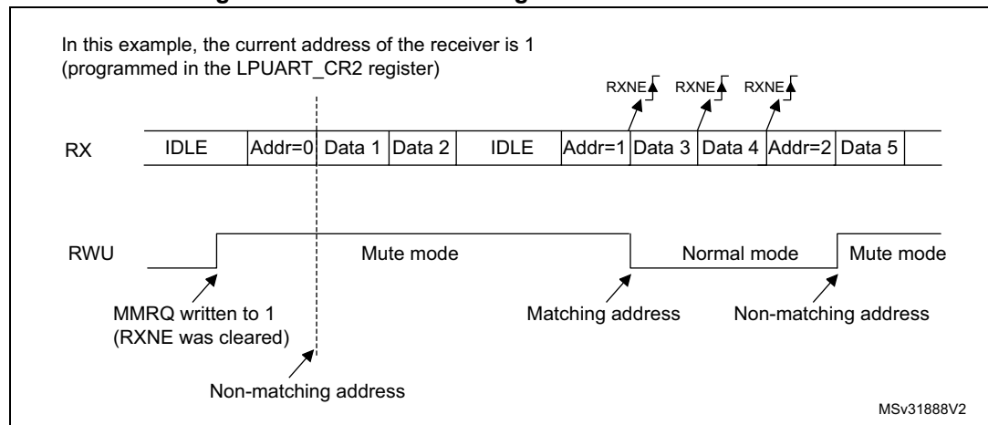
Figure 419. Mute mode using address mark detection
