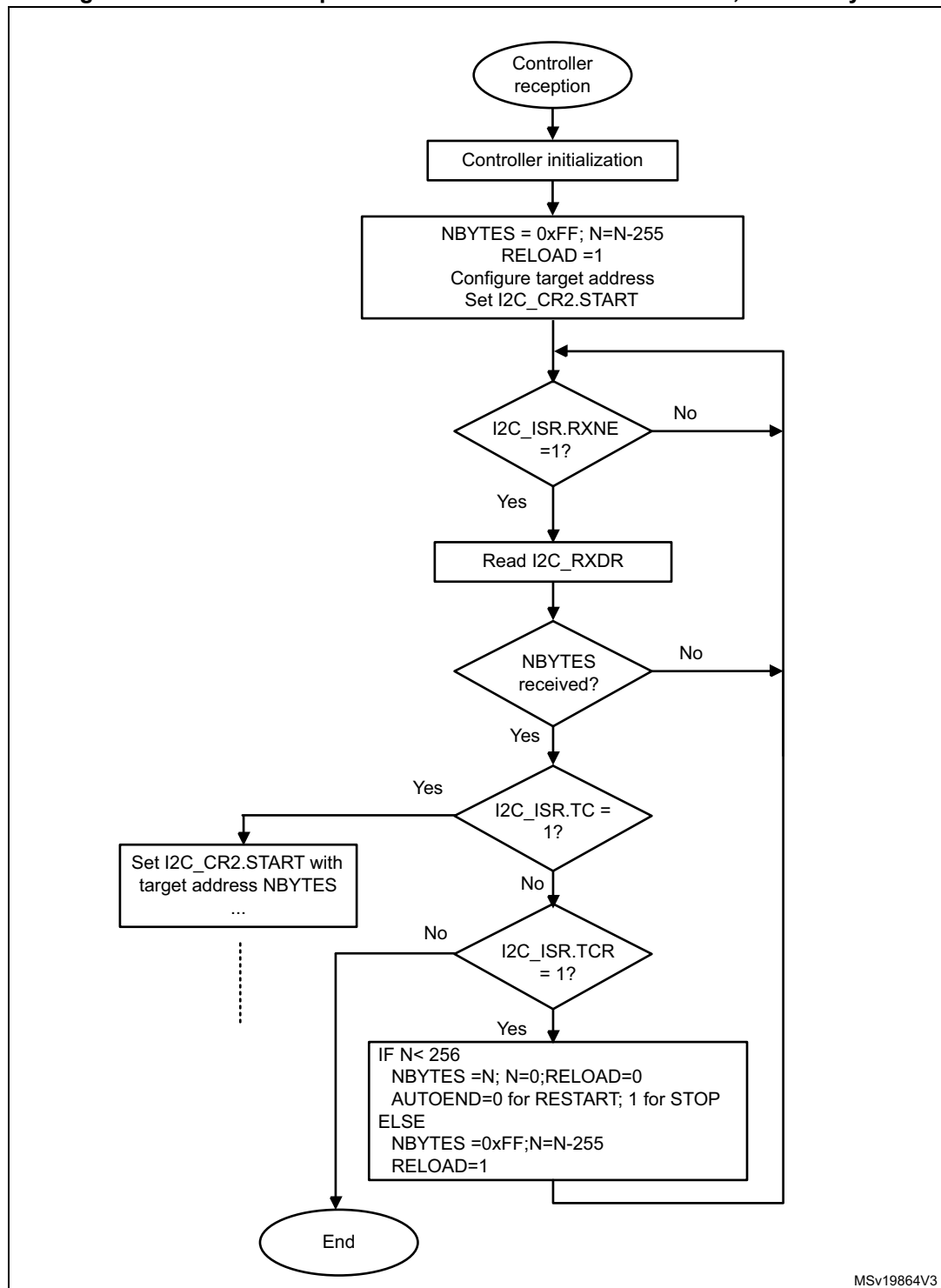
Figure 380. Transfer sequence flow for I2C controller receiver, N &gt; 255 bytes
