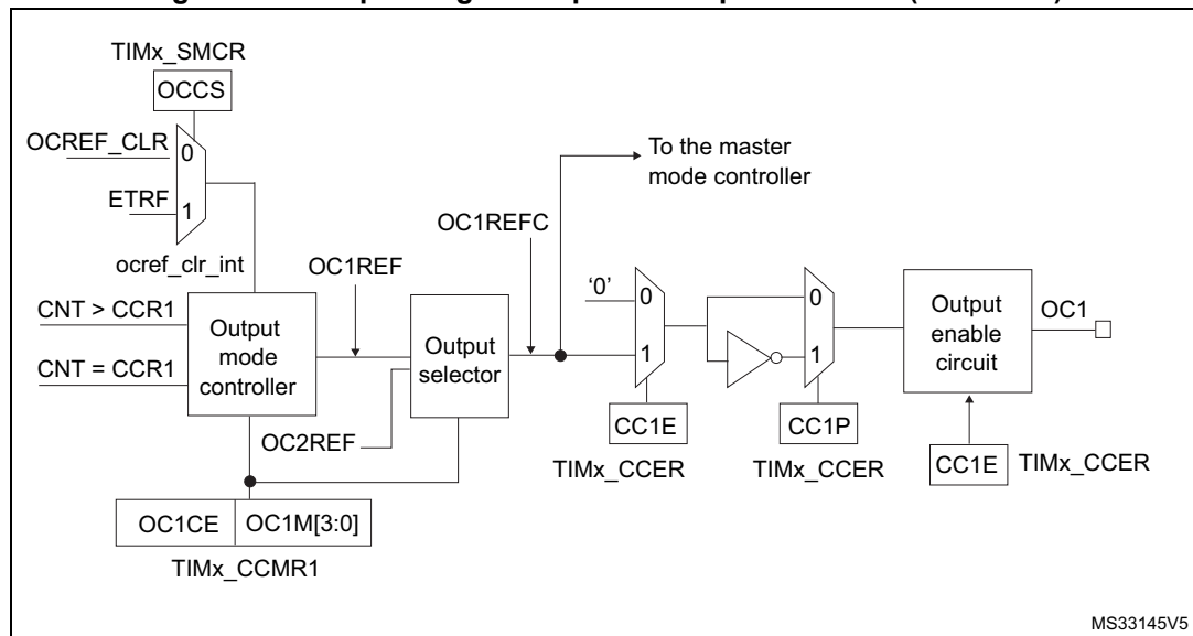
Figure 270. Output stage of Capture/Compare channel (channel 1)
