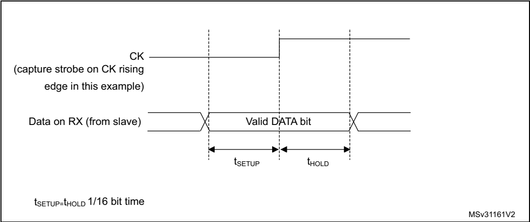
Figure 403. RX data setup/hold time
