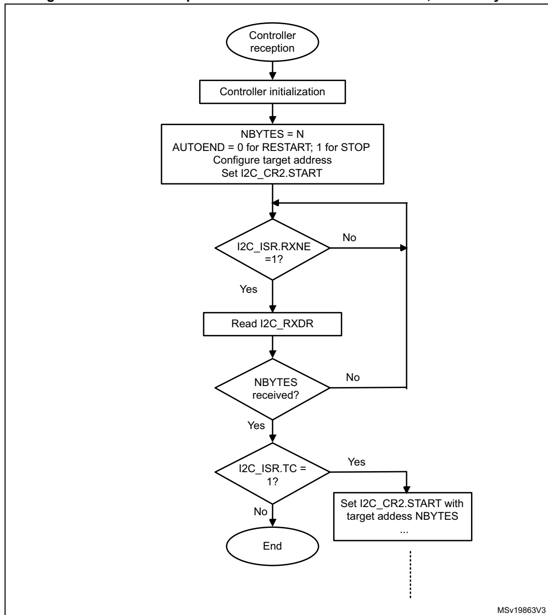
Figure 379. Transfer sequence flow for I2C controller receiver, N \leq 255 bytes
