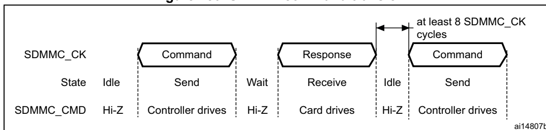
Figure 480. SDMMC command transfer
