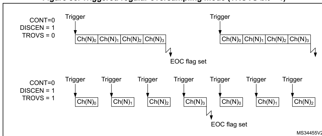
Figure 85. Triggered regular oversampling mode (TROVS bit = 1)
