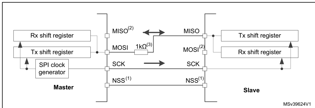
Figure 428. Half-duplex single master/ single slave application
