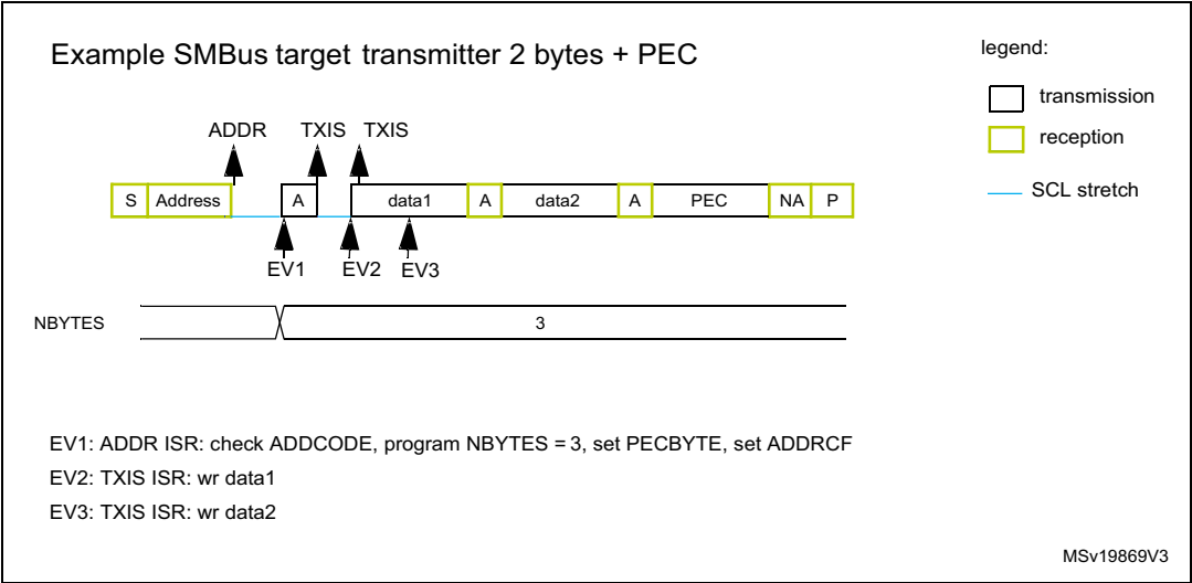
Figure 384. Transfer bus diagram for SMBus target transmitter (SBC = 1)
