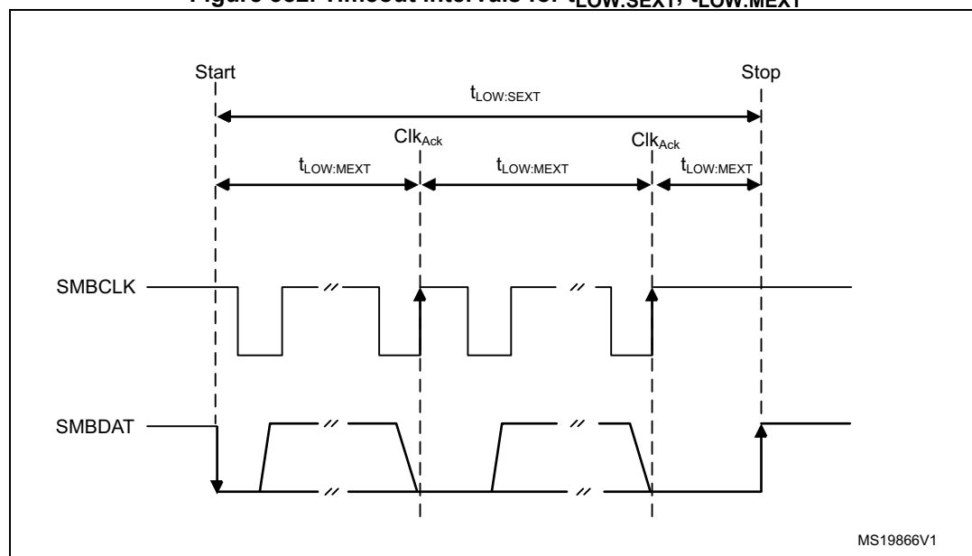
Figure 382. Timeout intervals for t_{\text{LOW:SEXT}} , t_{\text{LOW:MEXT}}
