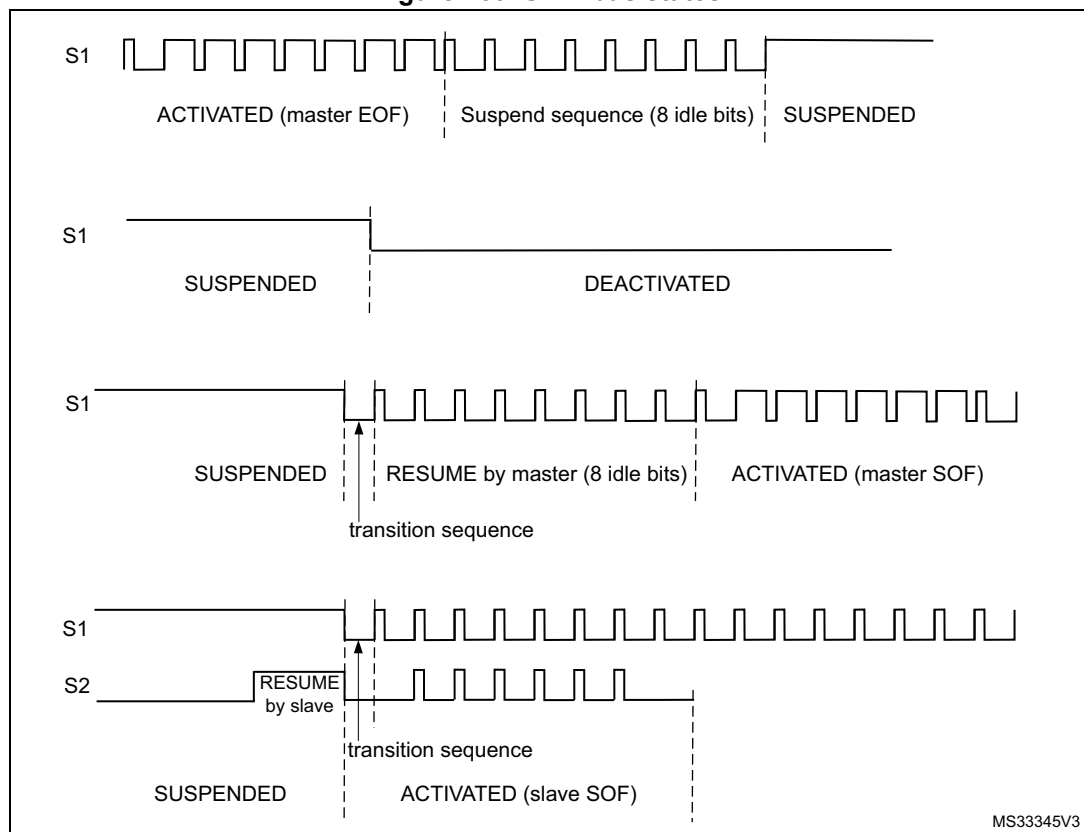
Figure 460. SWP bus states
