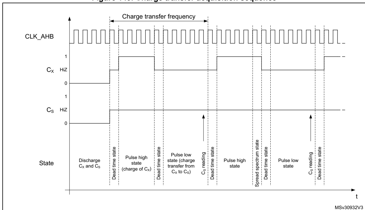
Figure 149. Charge transfer acquisition sequence
