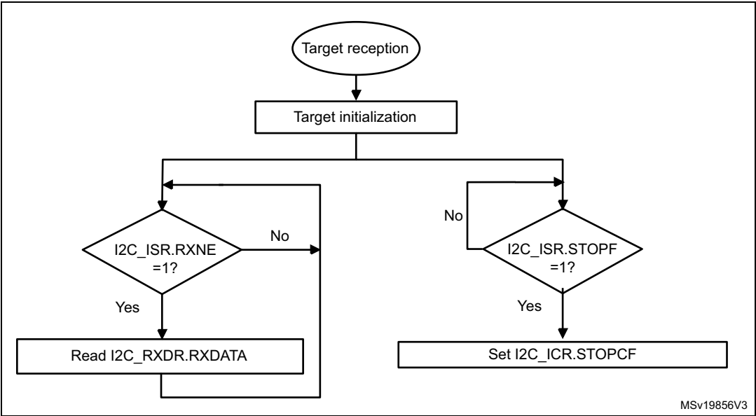
Figure 370. Transfer sequence flow for I2C target receiver, NOSTRETCH = 1
