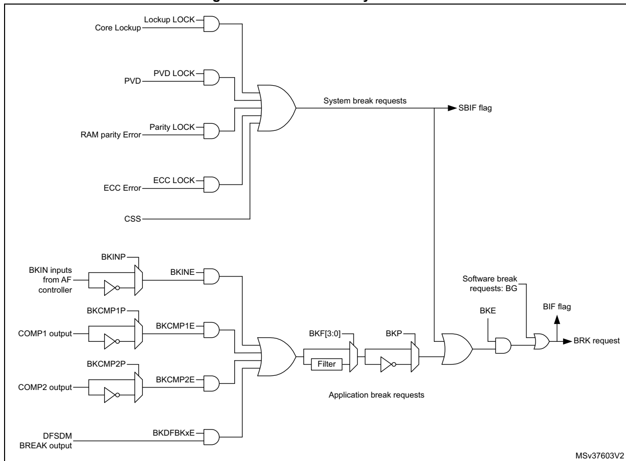
Figure 318. Break circuitry overview
