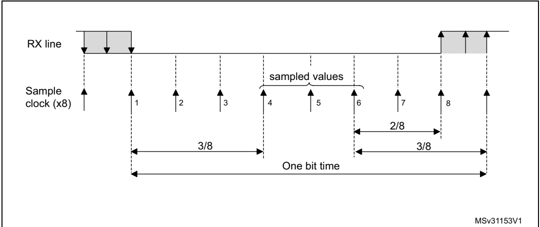
Figure 395. Data sampling when oversampling by 8
