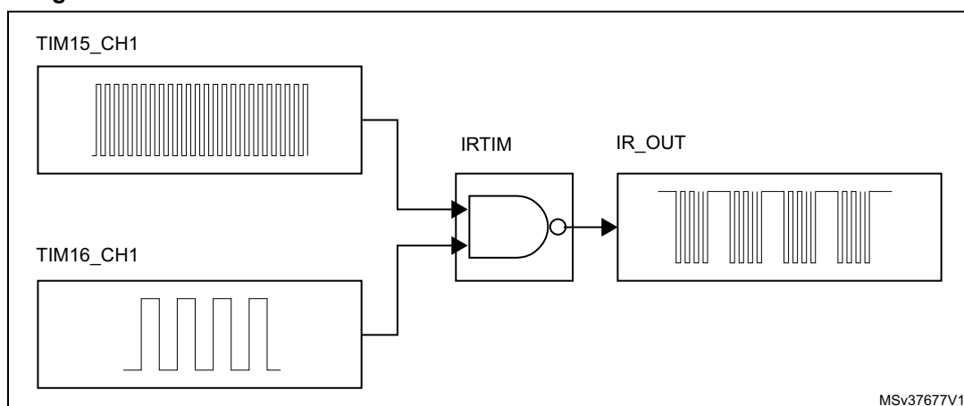
Figure 352. IRTIM internal hardware connections with TIM15 and TIM16 and TIM17
