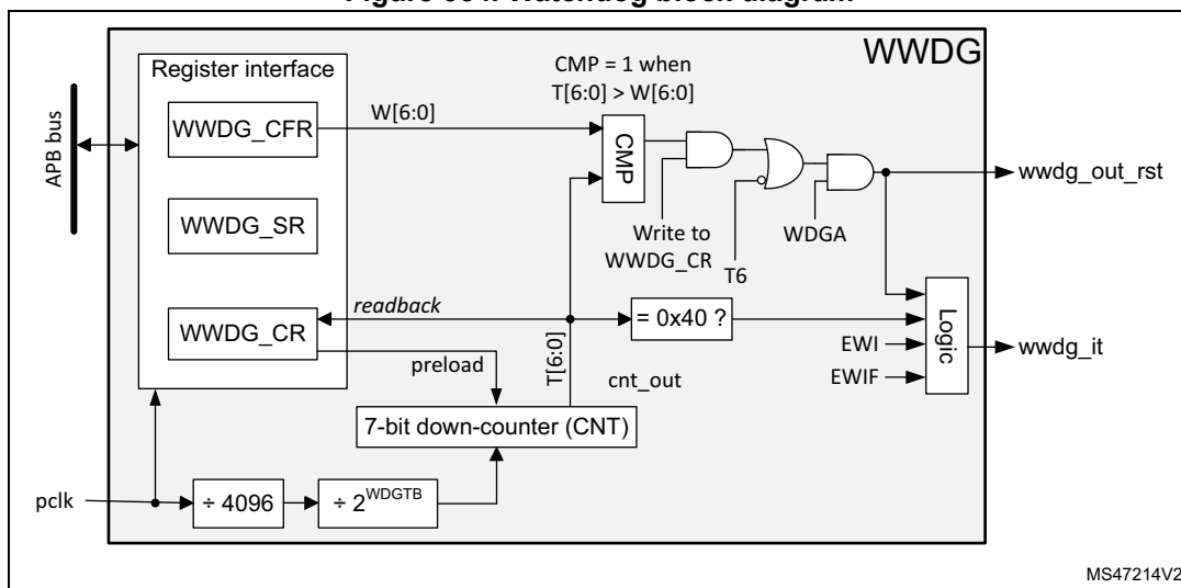
Figure 354. Watchdog block diagram
