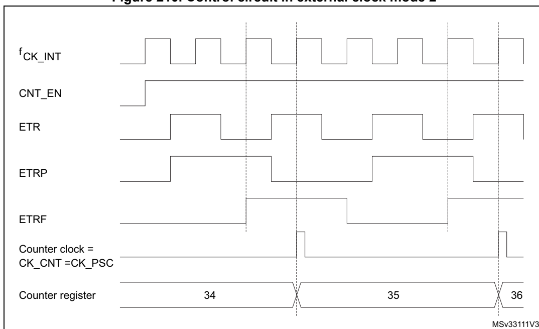
Figure 210. Control circuit in external clock mode 2
