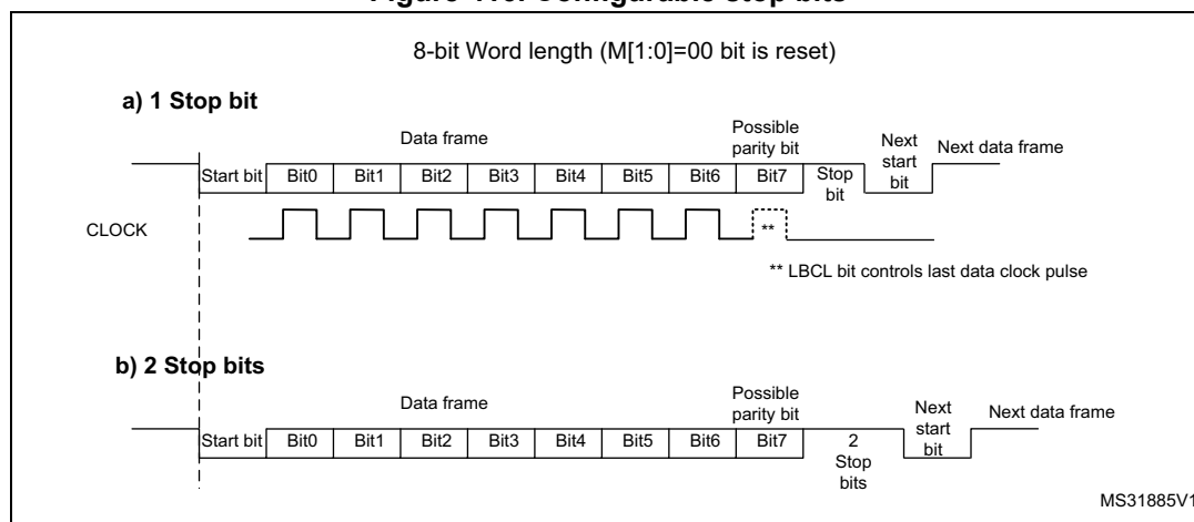
Figure 416. Configurable stop bits
