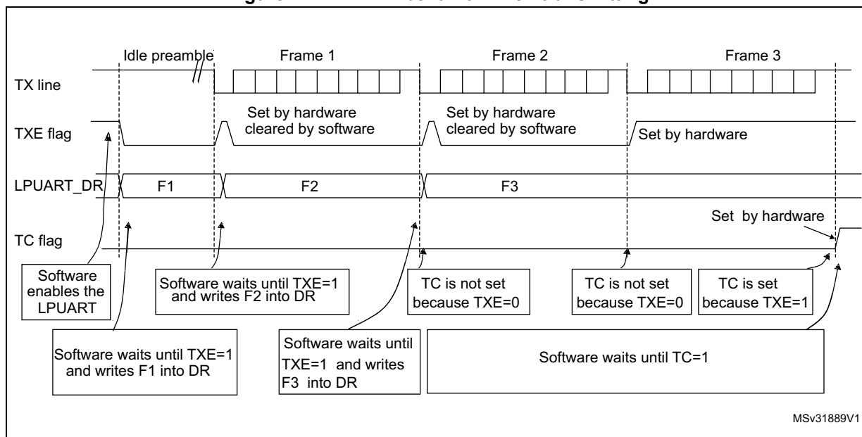
Figure 417. TC/TXE behavior when transmitting
