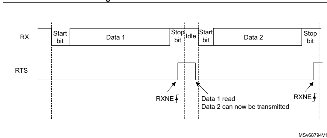
Figure 423. RS232 RTS flow control
