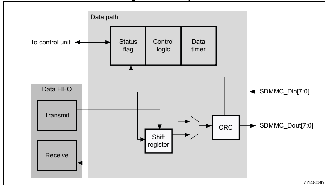
Figure 481. Data path
