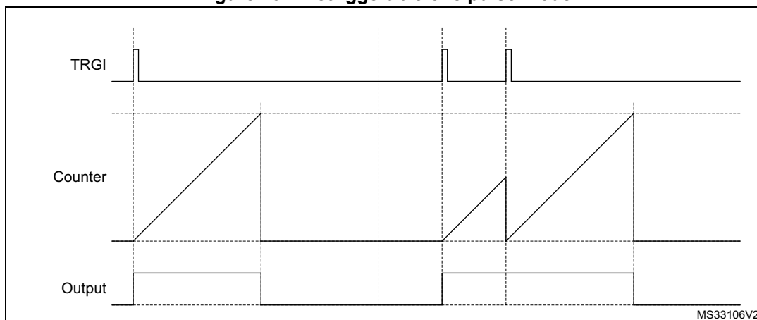
Figure 234. Retriggerable one pulse mode
