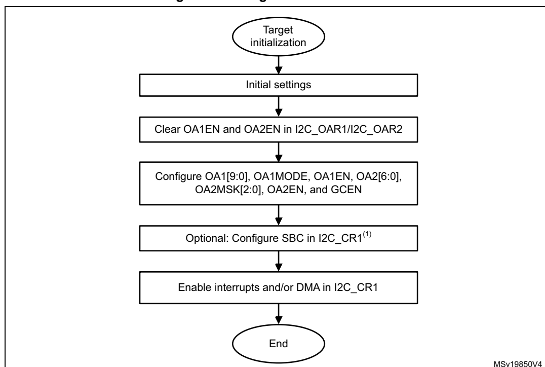
Figure 365. Target initialization flow
