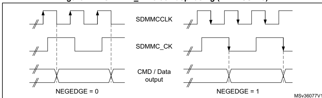
Figure 477. SDMMC_CK clock dephasing (BYPASS = 0)
