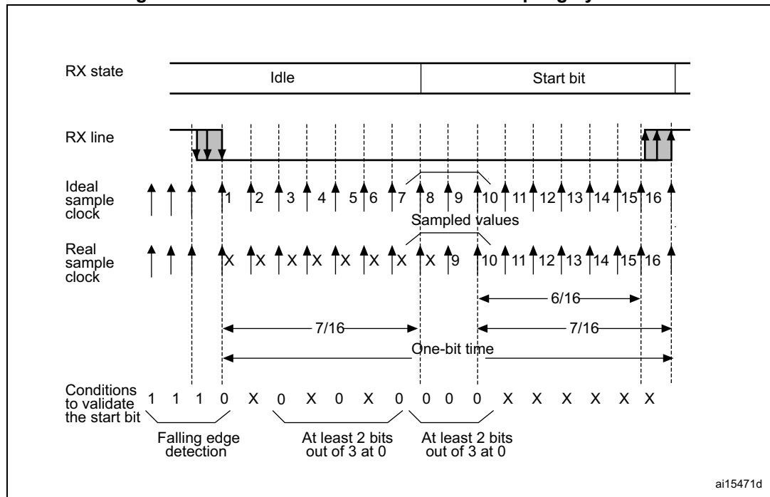
Figure 393. Start bit detection when oversampling by 16 or 8
