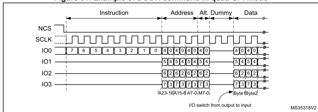
Figure 34. Example of a DDR command in quad-SPI mode
