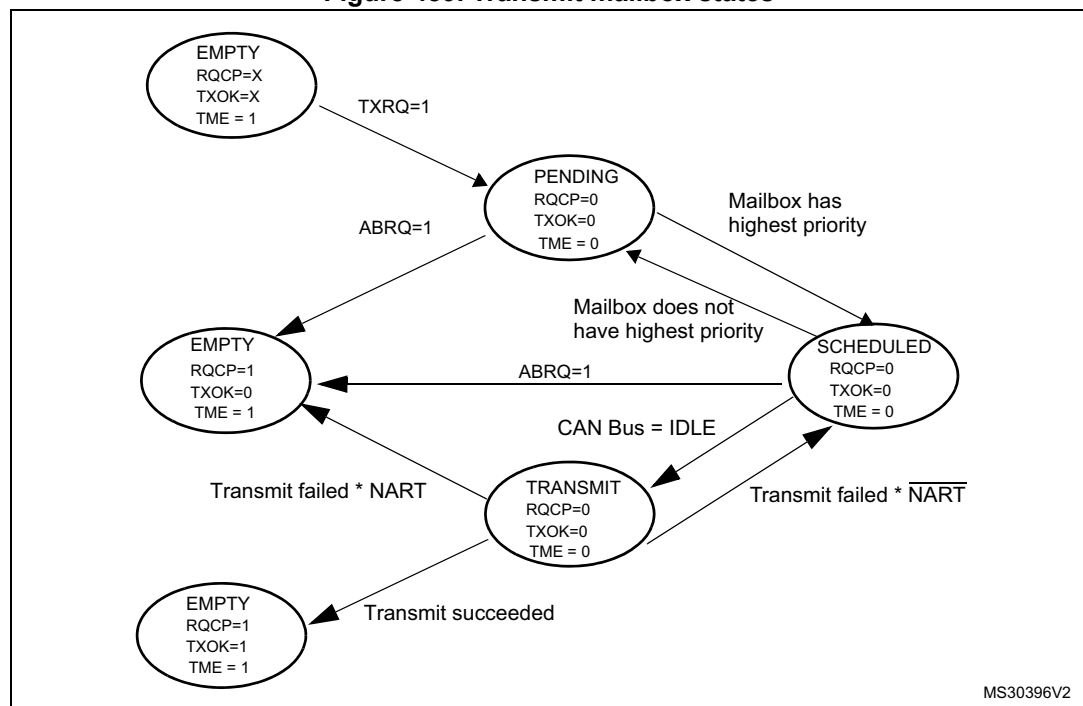
Figure 489. Transmit mailbox states
