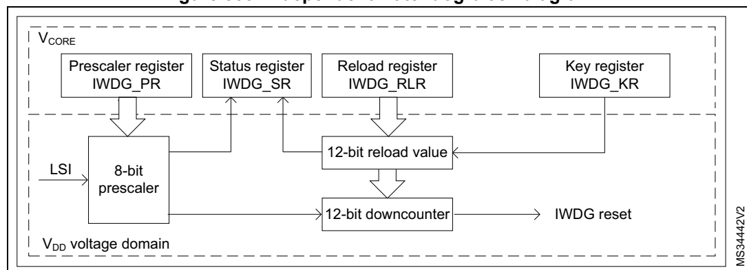
Figure 353. Independent watchdog block diagram
