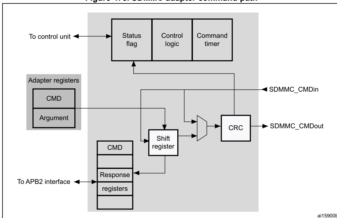
Figure 478. SDMMC adapter command path
