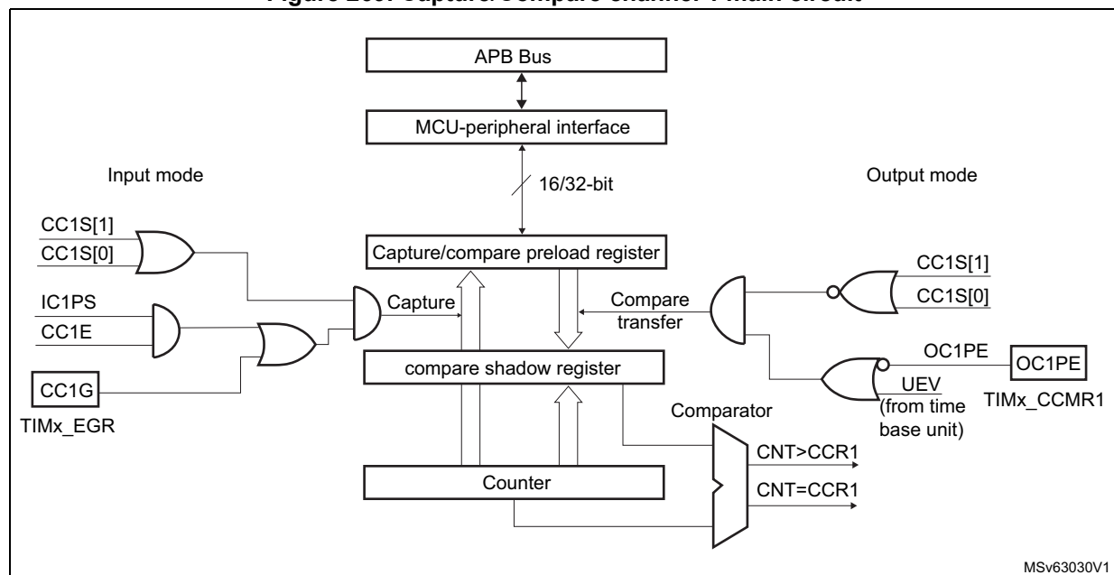
Figure 269. Capture/Compare channel 1 main circuit
