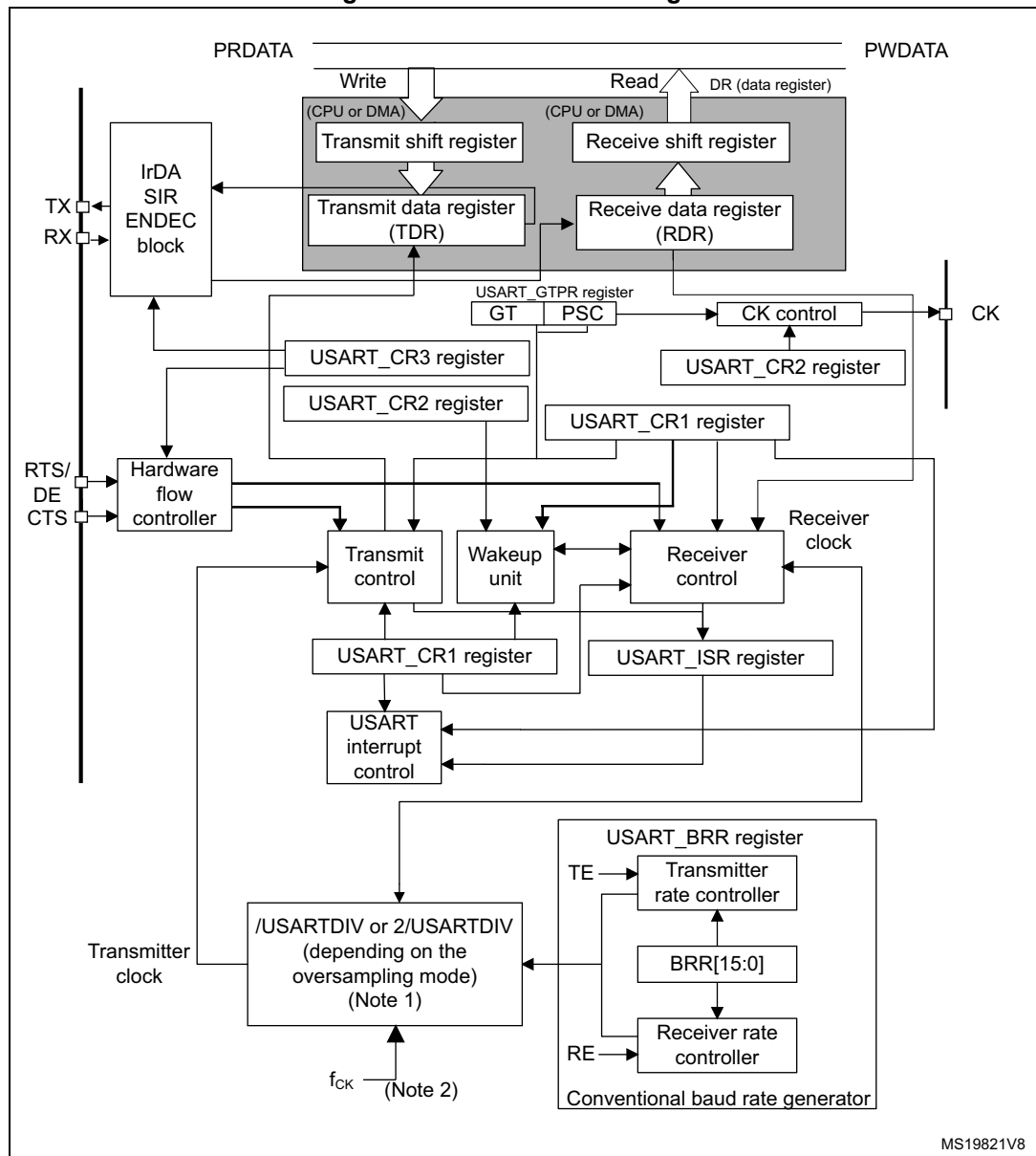
Figure 389. USART block diagram
