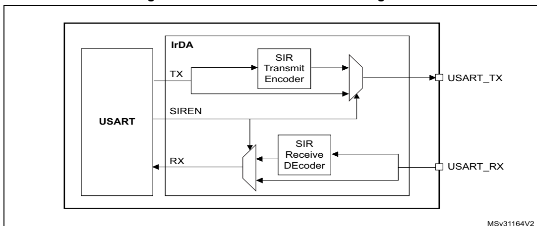
Figure 406. IrDA SIR ENDEC- block diagram
