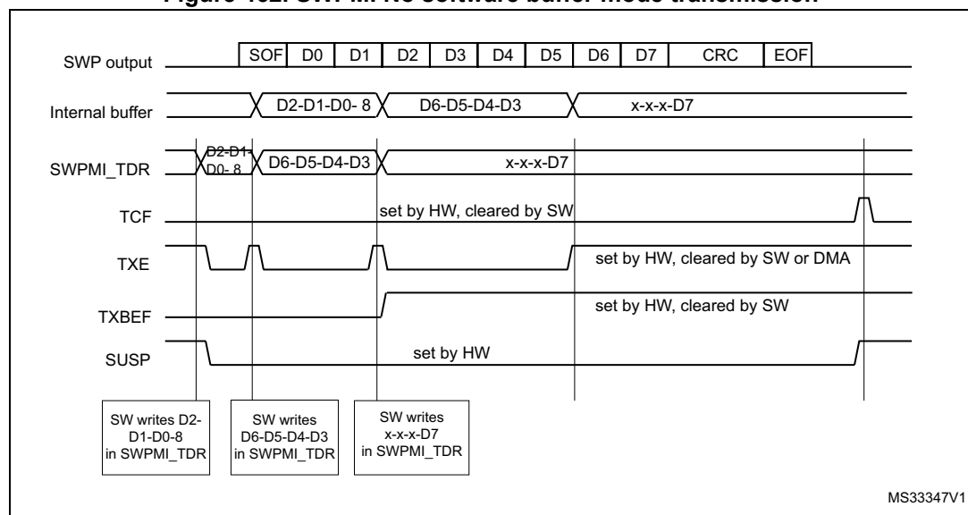
Figure 462. SWPMI No software buffer mode transmission
