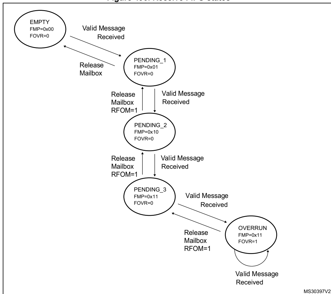
Figure 490. Receive FIFO states
