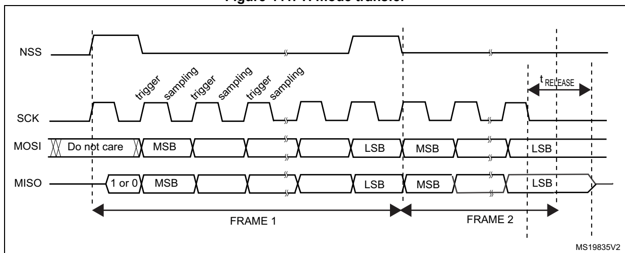
Figure 441. TI mode transfer
