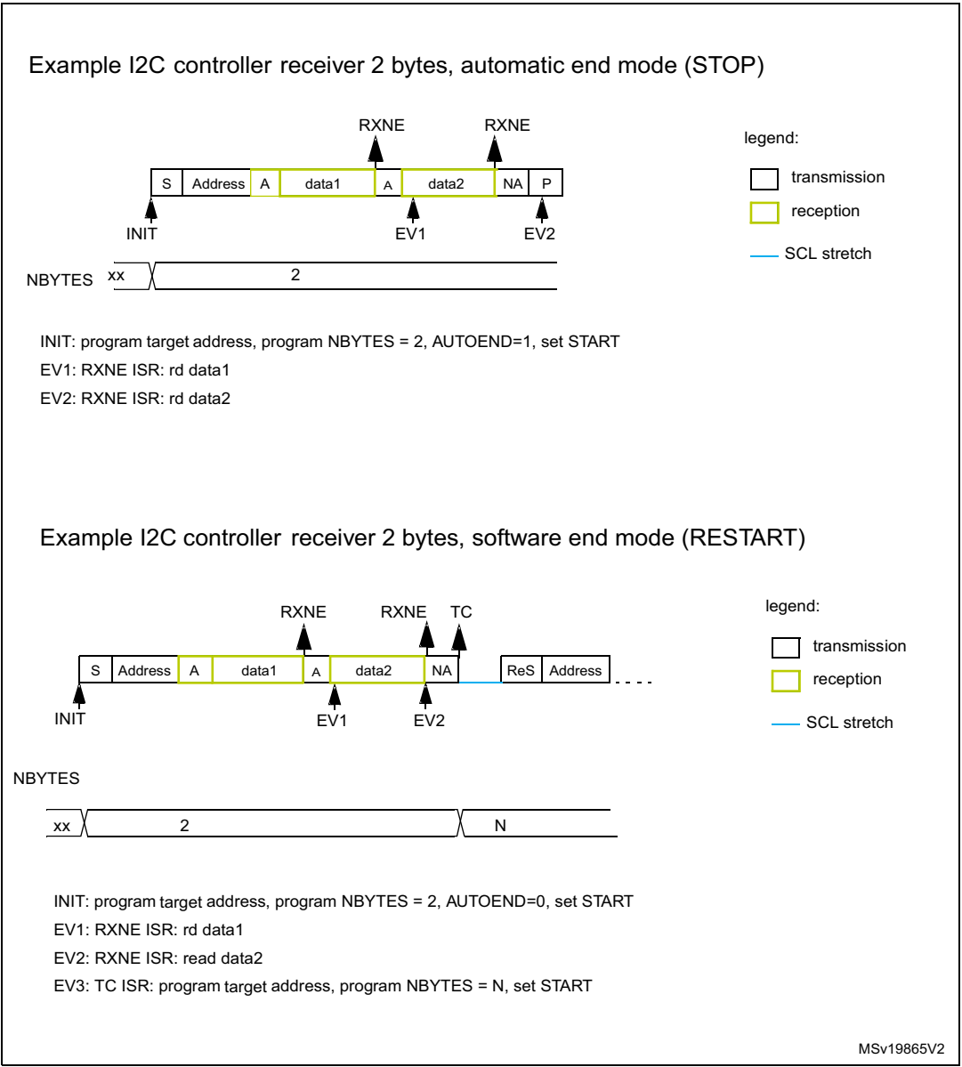
Figure 381. Transfer bus diagrams for I2C controller receiver (mandatory events only)
