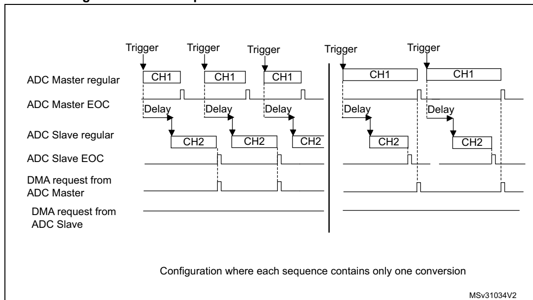
Figure 105. DMA requests in interleaved mode when MDMA = 10
