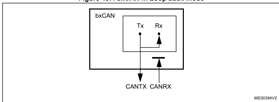
Figure 487. bxCAN in Loop back mode
