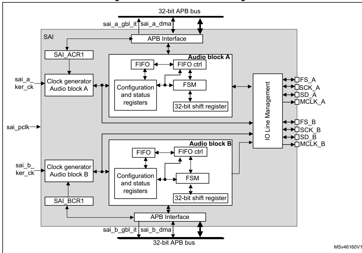
Figure 442. SAI functional block diagram
