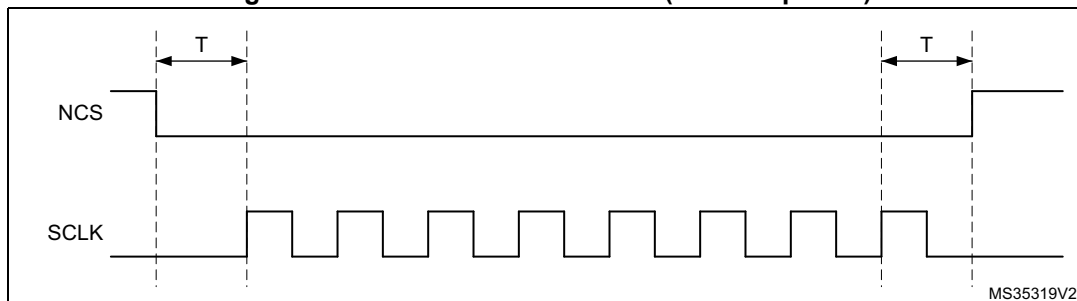
Figure 35. NCS when CKMODE = 0 (T = CLK period)
