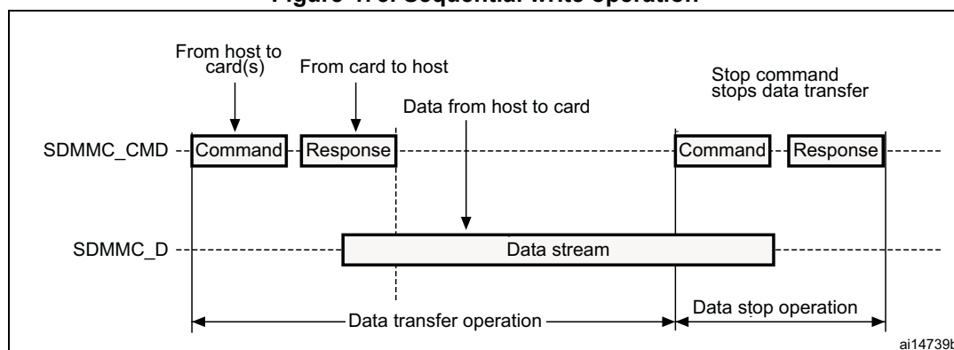
Figure 473. Sequential write operation
