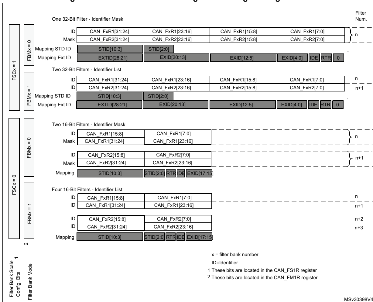
Figure 491. Filter bank scale configuration - Register organization
