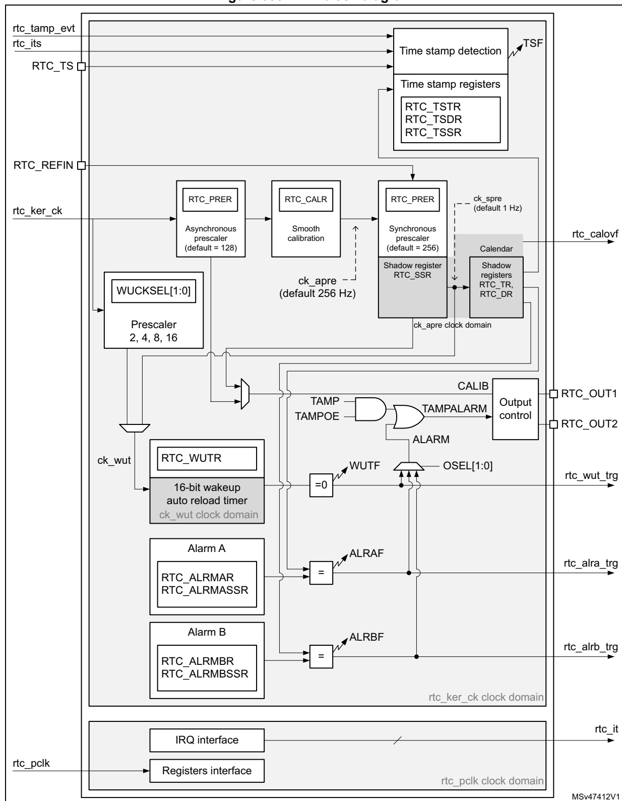
Figure 356. RTC block diagram
