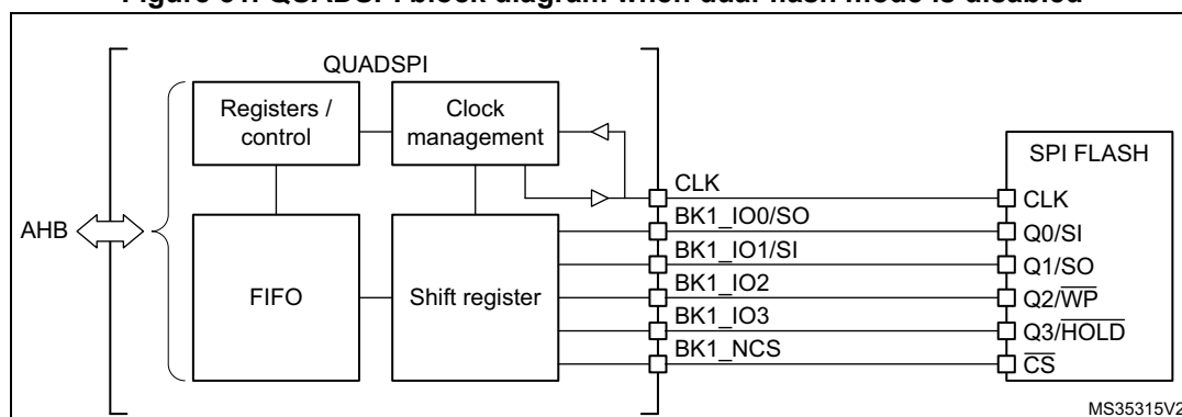
Figure 31. QUADSPI block diagram when dual-flash mode is disabled
