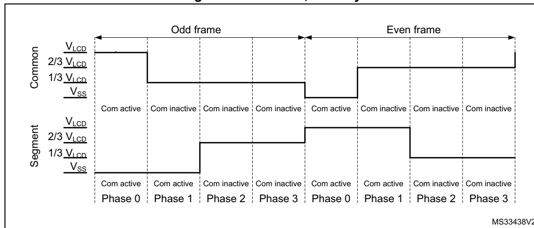
Figure 135. 1/3 bias, 1/4 duty
