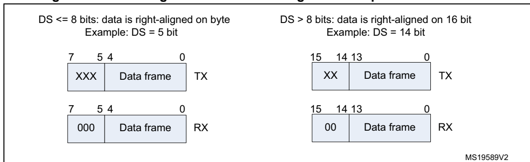
Figure 434. Data alignment when data length is not equal to 8-bit or 16-bit
