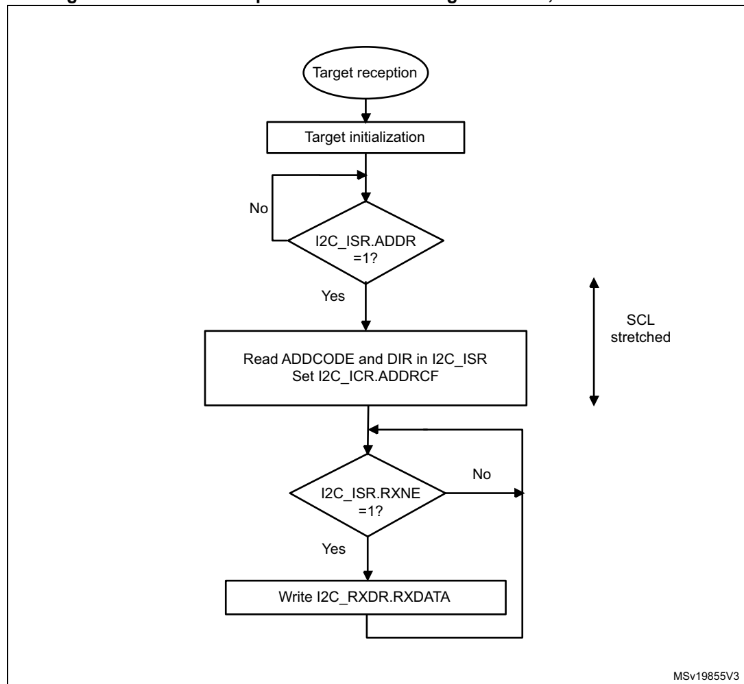
Figure 369. Transfer sequence flow for I2C target receiver, NOSTRETCH = 0
