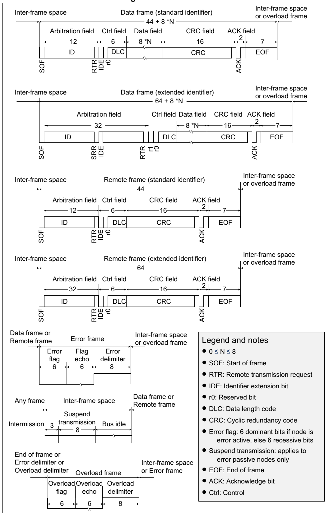
Figure 496. CAN frames
