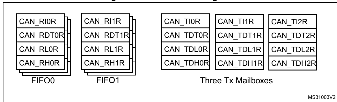
Figure 498. CAN mailbox registers
