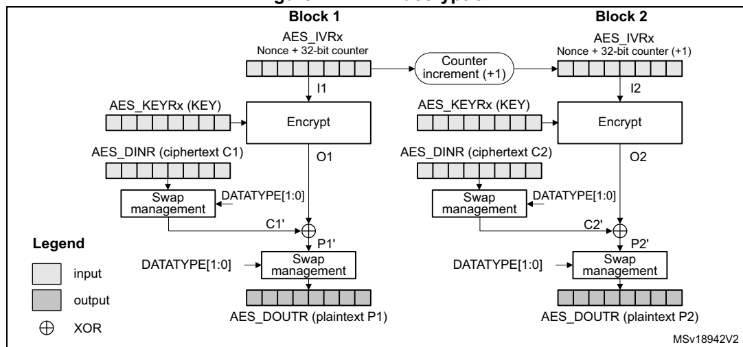
Figure 172. CTR decryption
