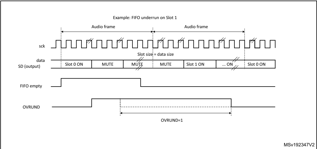
Figure 456. FIFO underrun event
