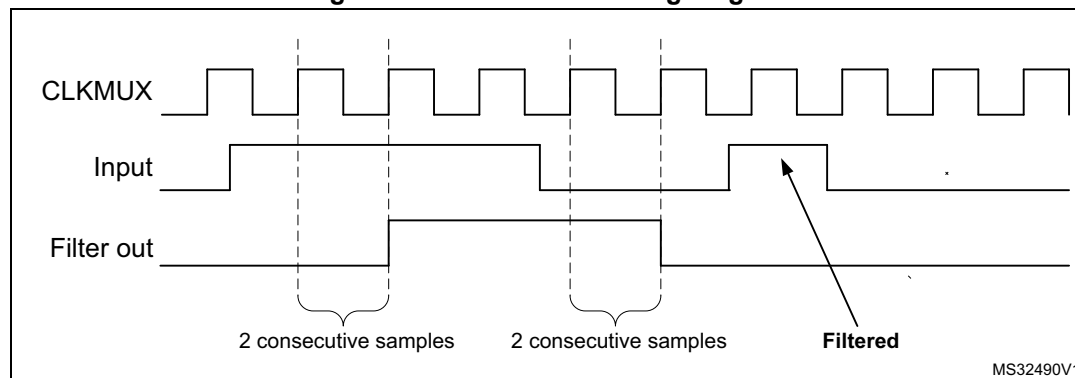
Figure 345. Glitch filter timing diagram
