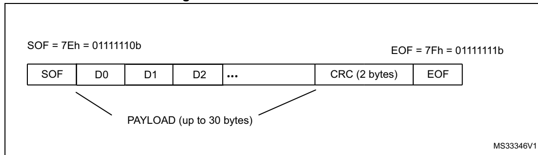
Figure 461. SWP frame structure
