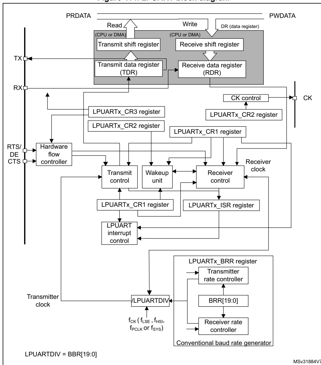
Figure 414. LPUART block diagram
