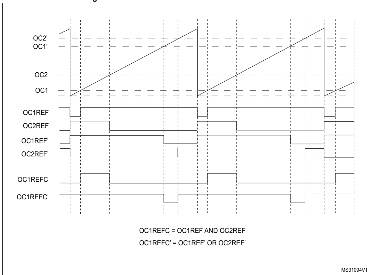
Figure 314. Combined PWM mode on channel 1 and 2
