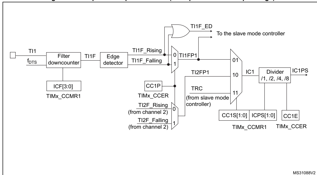
Figure 307. Capture/compare channel (example: channel 1 input stage)
