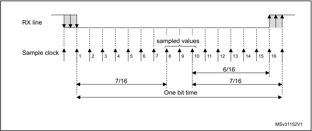
Figure 394. Data sampling when oversampling by 16
