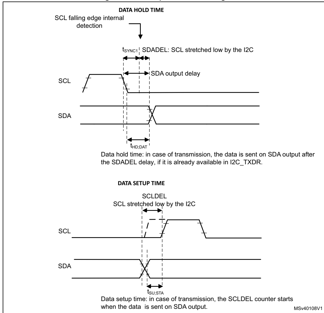
Figure 361. Setup and hold timings
