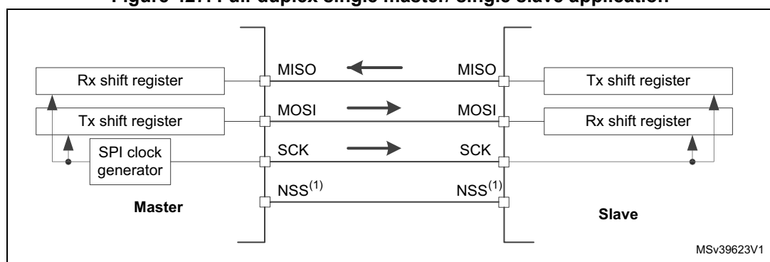
Figure 427. Full-duplex single master/ single slave application
