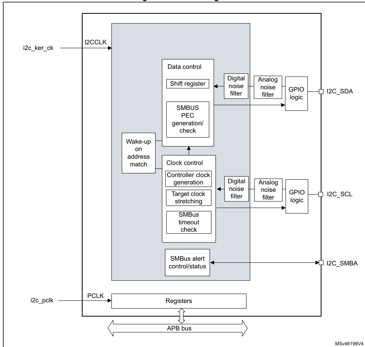
Figure 359. Block diagram
