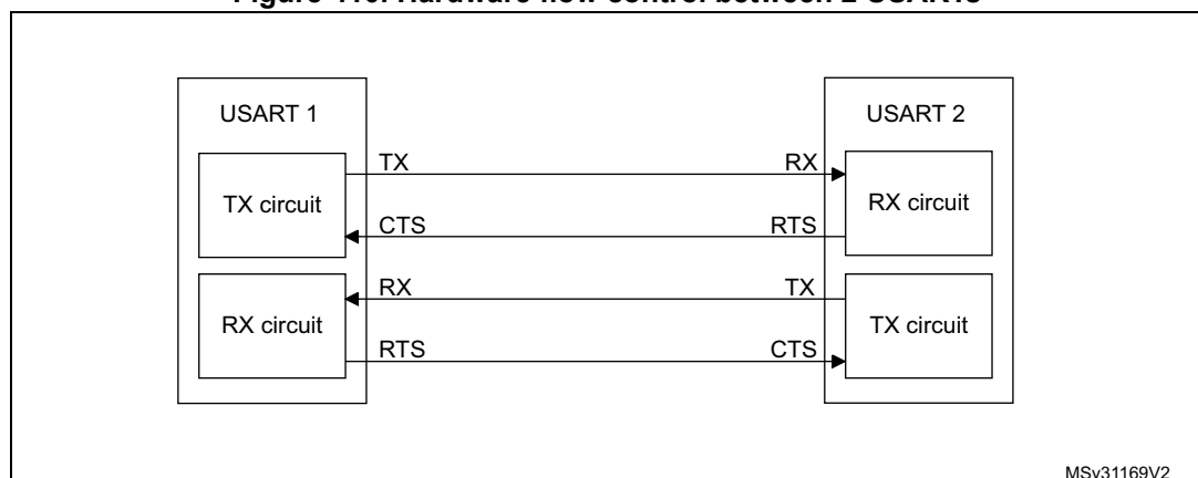
Figure 410. Hardware flow control between 2 USARTs
