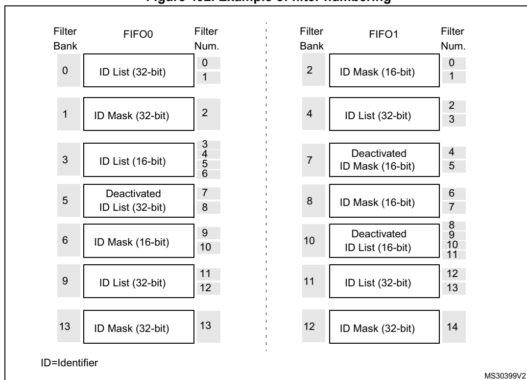
Figure 492. Example of filter numbering
