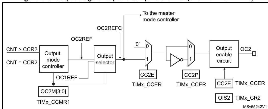
Figure 310. Output stage of capture/compare channel (channel 2 for TIM15)
