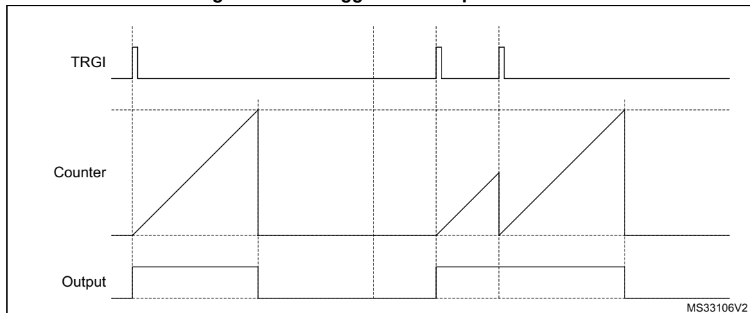
Figure 279. Retriggerable one-pulse mode
