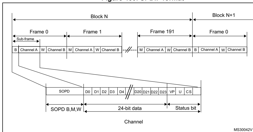
Figure 450. SPDIF format
