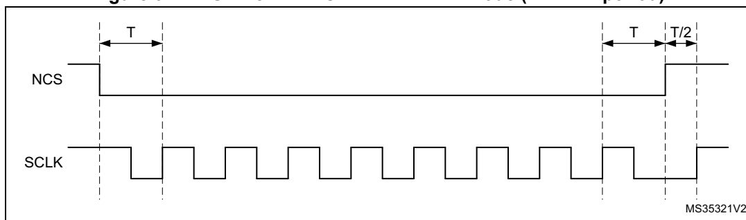
Figure 37. NCS when CKMODE = 1 in DDR mode ( T = \text{CLK period} )
