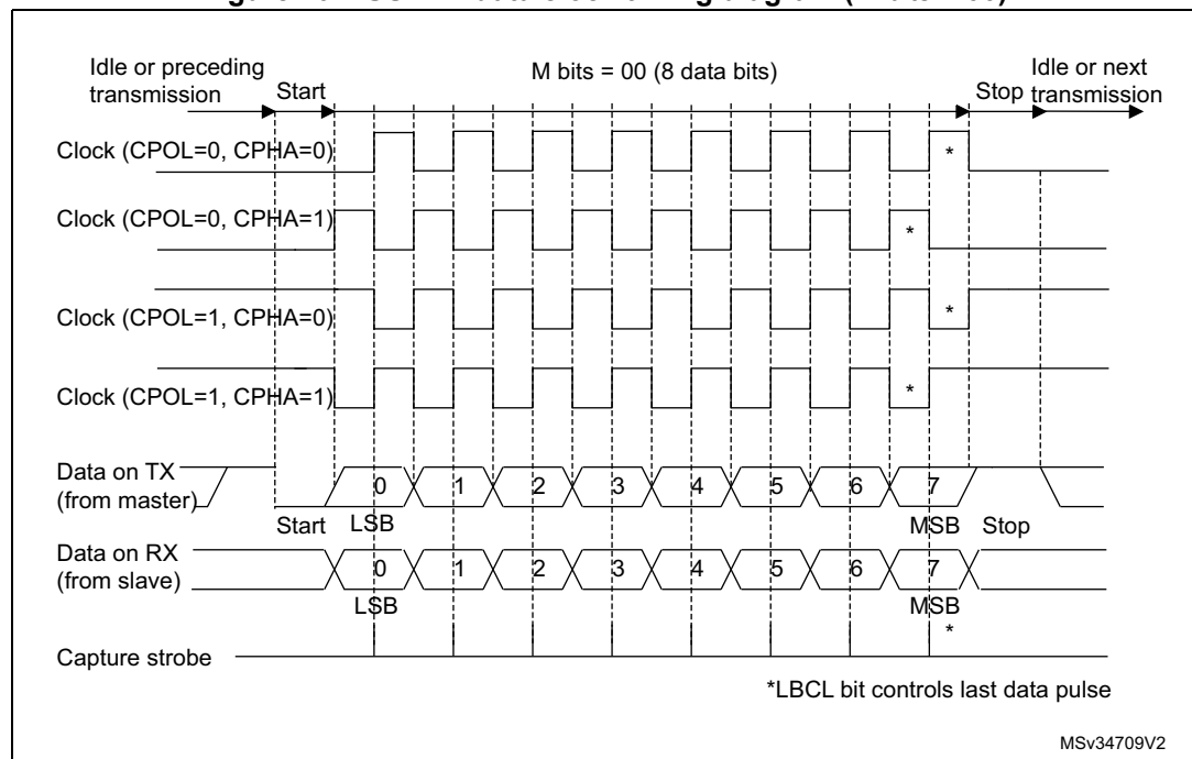
Figure 401. USART data clock timing diagram (M bits = 00)
