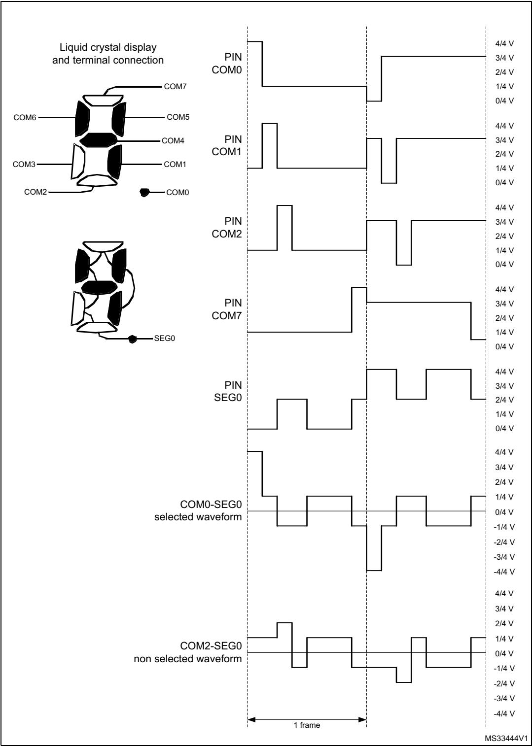
Figure 141. 1/8 duty, 1/4 bias
