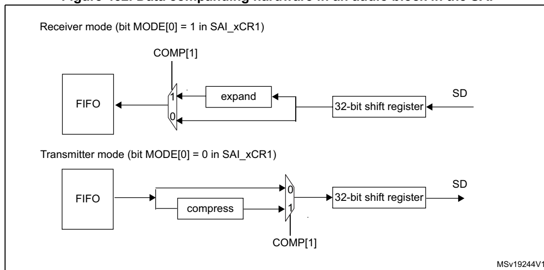
Figure 452. Data companding hardware in an audio block in the SAI
