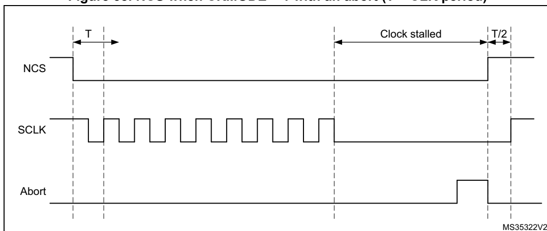
Figure 38. NCS when CKMODE = 1 with an abort ( T = \text{CLK period} )
