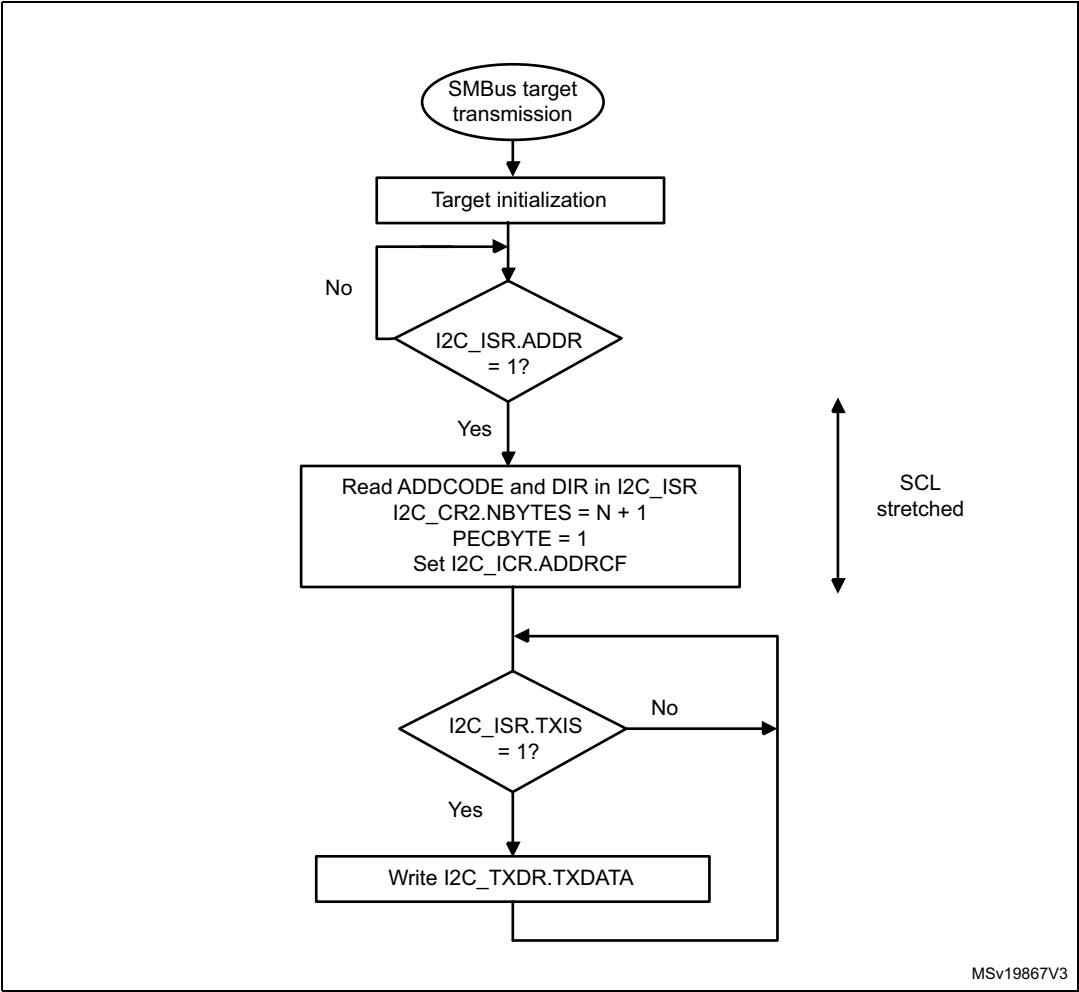
Figure 384. Transfer bus diagram for SMBus target transmitter (SBC = 1)
