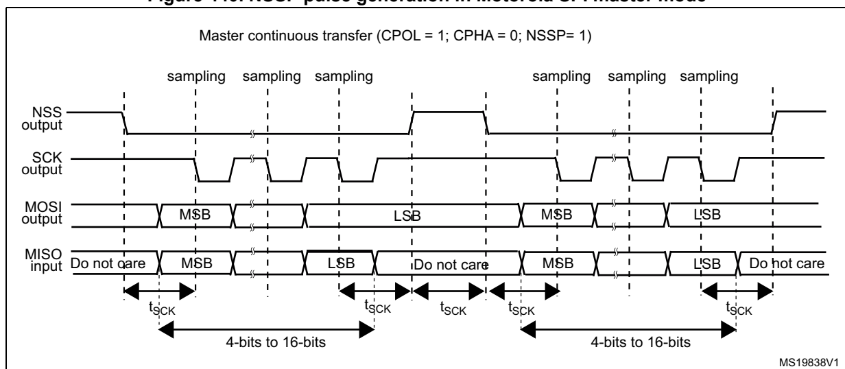
Figure 440. NSSP pulse generation in Motorola SPI master mode
