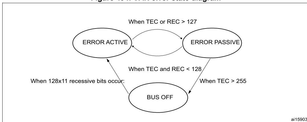
Figure 494. CAN error state diagram
