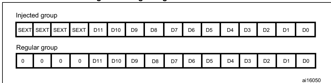
Figure 36. Right alignment of 12-bit data
