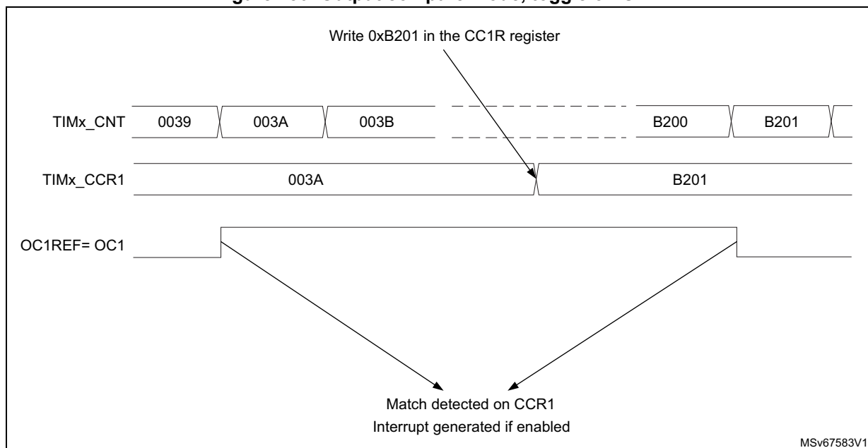
Figure 150. Output compare mode, toggle on OC1.
