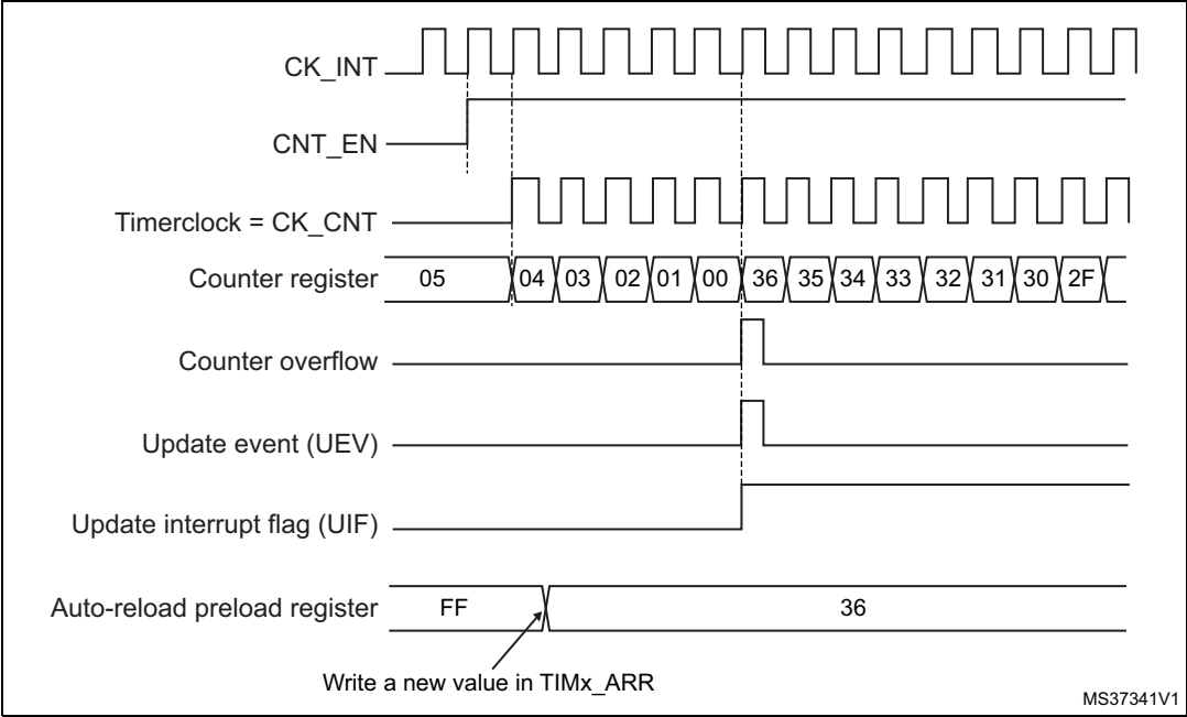
Figure 110. Counter timing diagram, Update event
