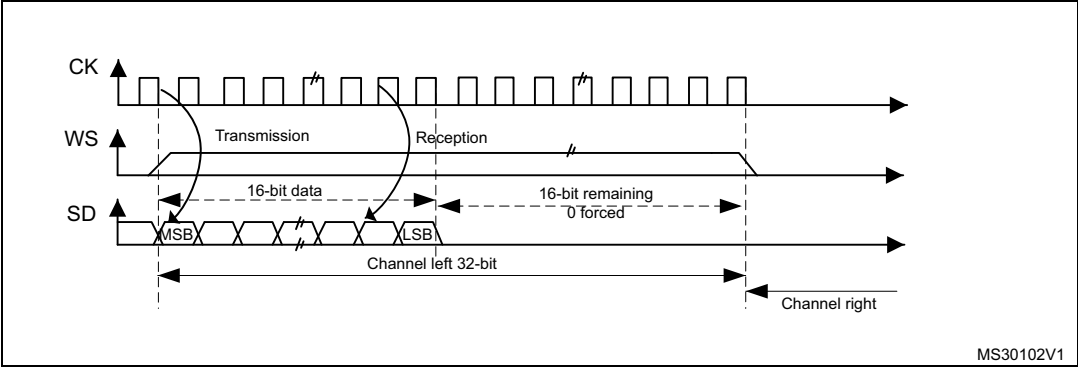
Figure 262. MSB justified 16-bit extended to 32-bit packet frame with CPOL = 0
