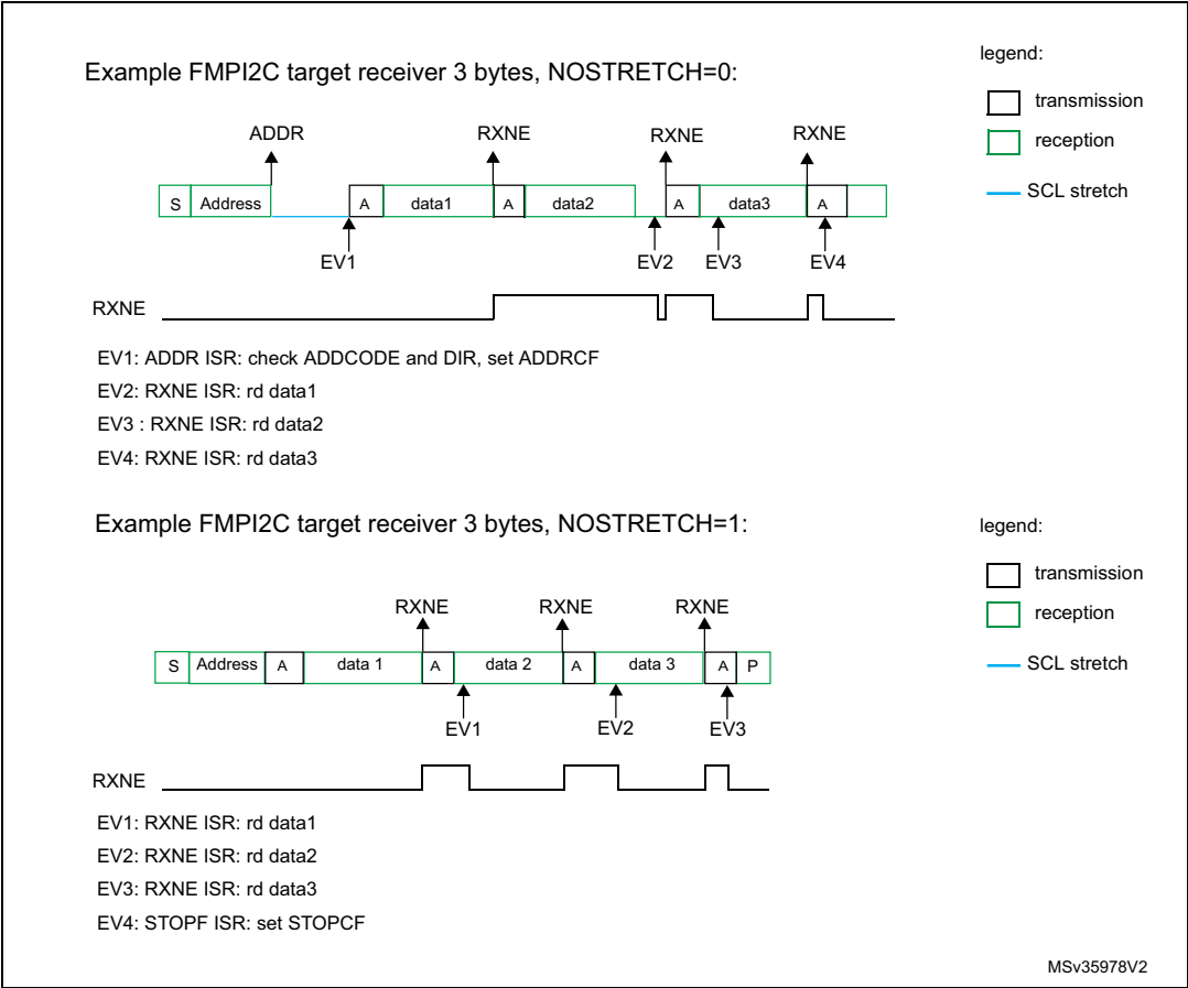
Figure 189. Transfer bus diagrams for FMPI2C target receiver (mandatory events only)
