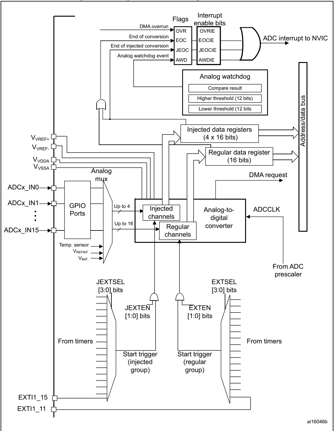
Figure 32. Single ADC block diagram
