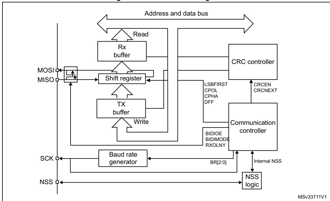
Figure 239. SPI block diagram
