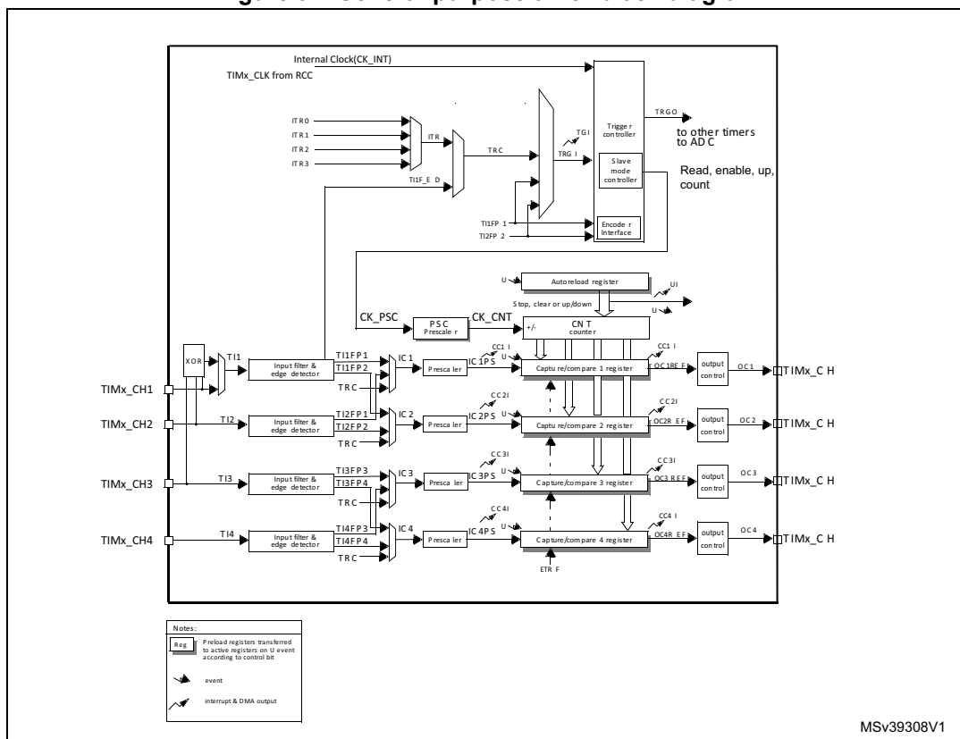
Figure 97. General-purpose timer block diagram
