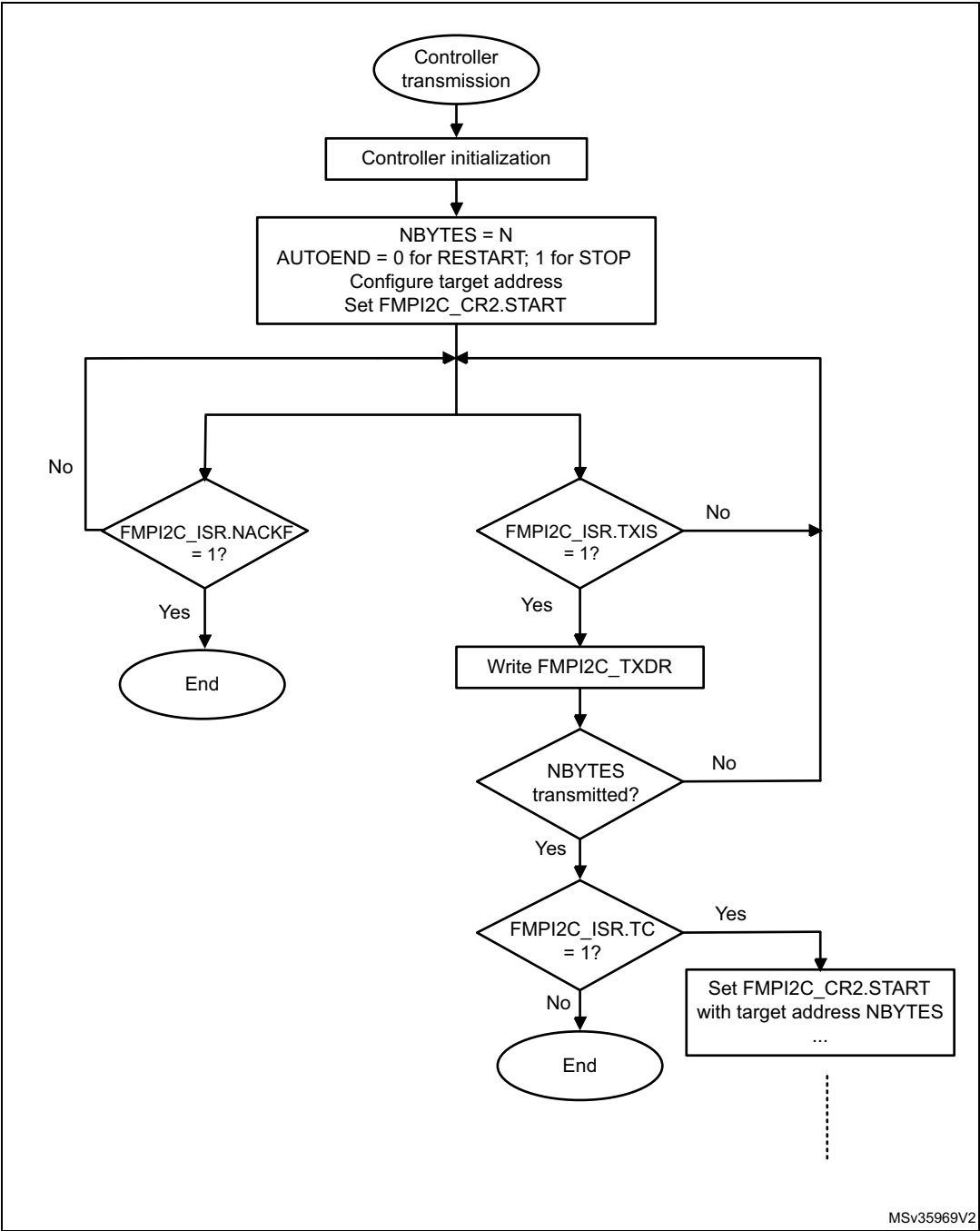
Figure 194. Transfer sequence flow for FMPI2C controller transmitter, N \leq 255 bytes
