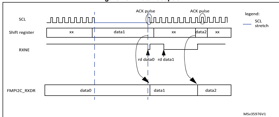
Figure 181. Data reception
