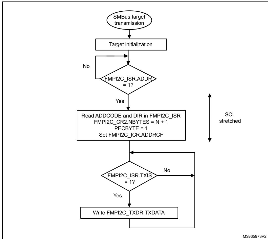
Figure 201. Transfer sequence flow for SMBus target transmitter N bytes + PEC
