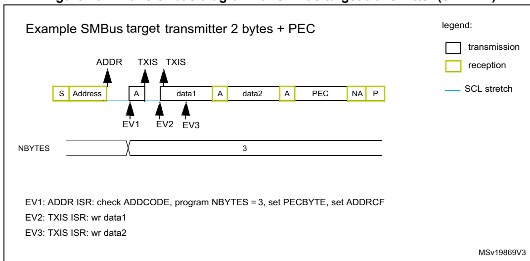
Figure 202. Transfer bus diagram for SMBus target transmitter (SBC = 1)
