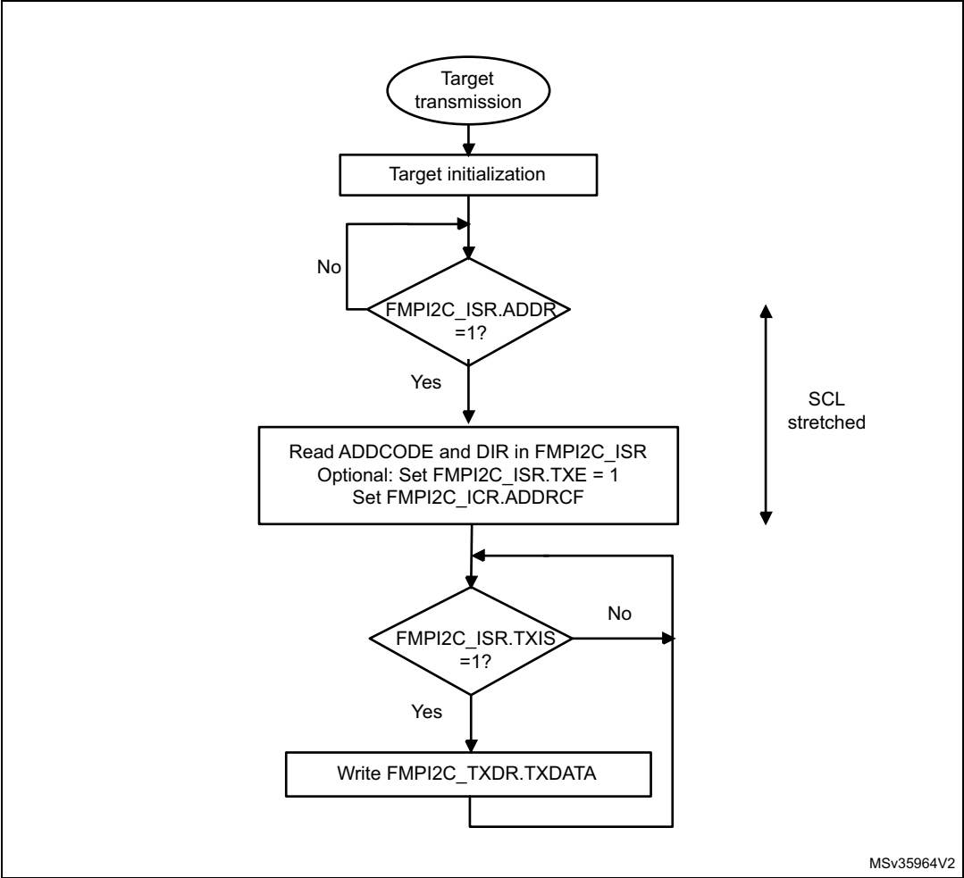
Figure 184. Transfer sequence flow for FMPI2C target transmitter, NOSTRETCH = 0
