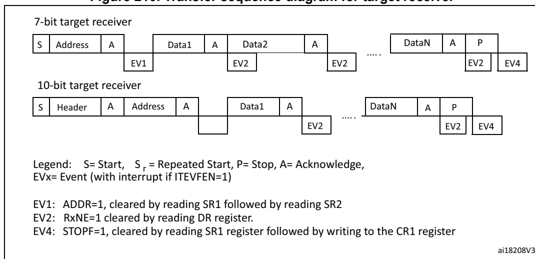
Figure 210. Transfer sequence diagram for target receiver
