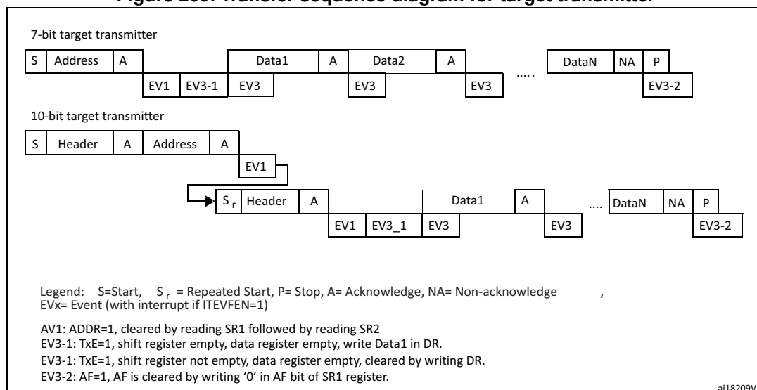
Figure 209. Transfer sequence diagram for target transmitter
