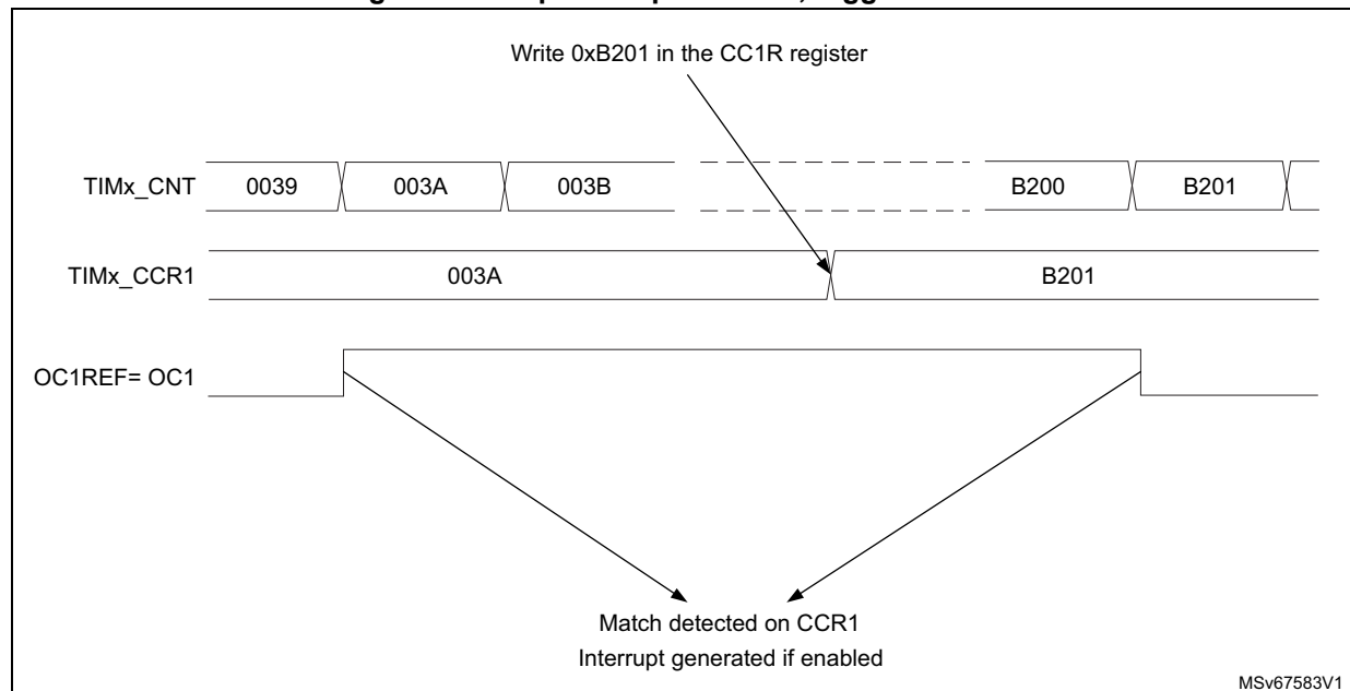
Figure 80. Output compare mode, toggle on OC1.
