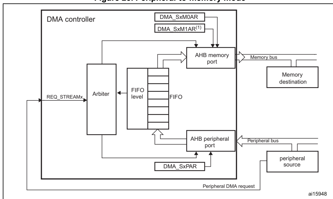
Figure 25. Peripheral-to-memory mode
