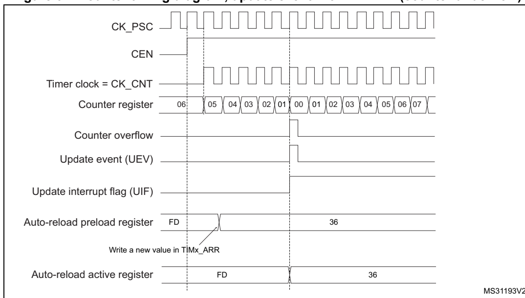
Figure 67. Counter timing diagram, update event with ARPE=1 (counter underflow)
