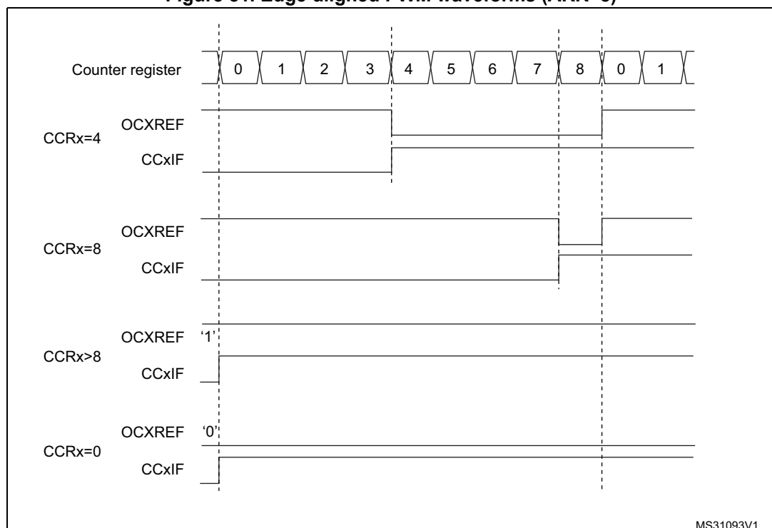
Figure 81. Edge-aligned PWM waveforms (ARR=8)
