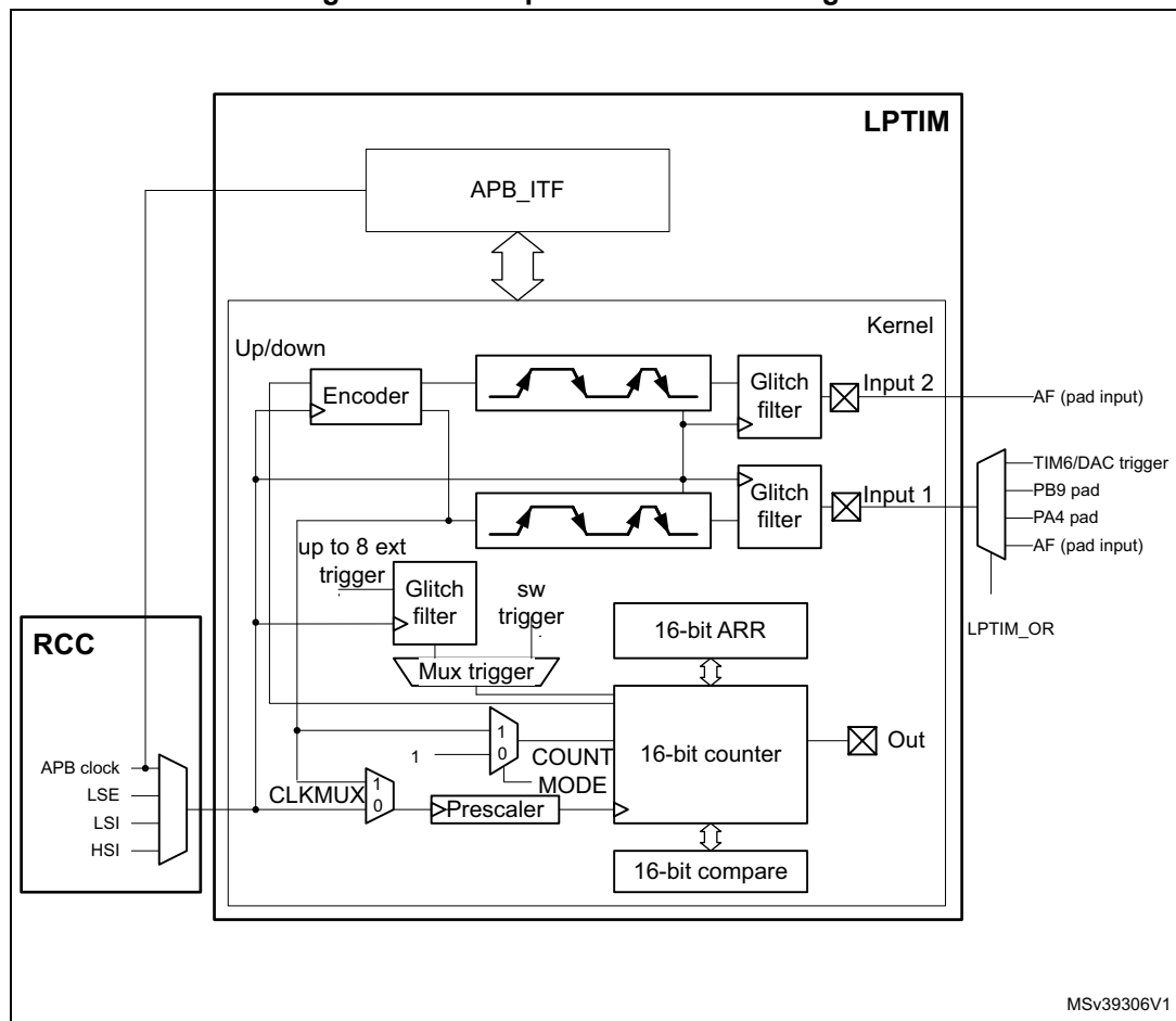
Figure 166. Low-power timer block diagram
