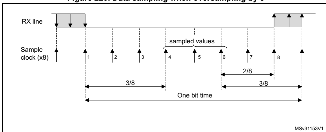
Figure 220. Data sampling when oversampling by 8
