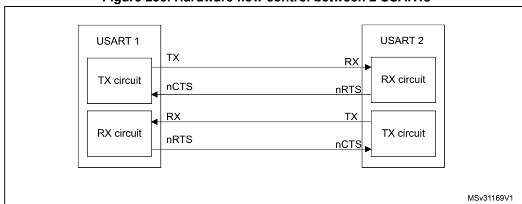
Figure 235. Hardware flow control between 2 USARTs
