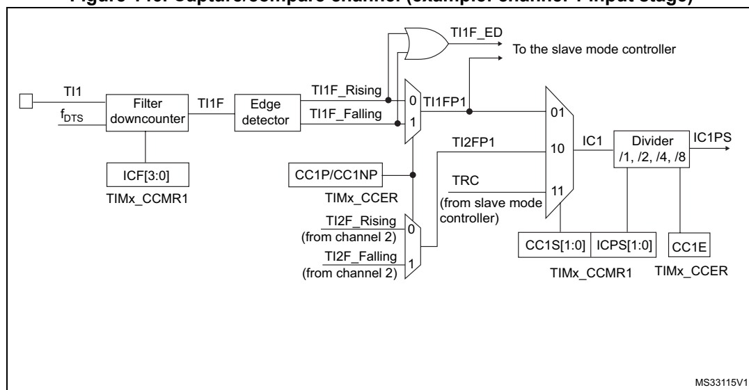
Figure 146. Capture/compare channel (example: channel 1 input stage)
