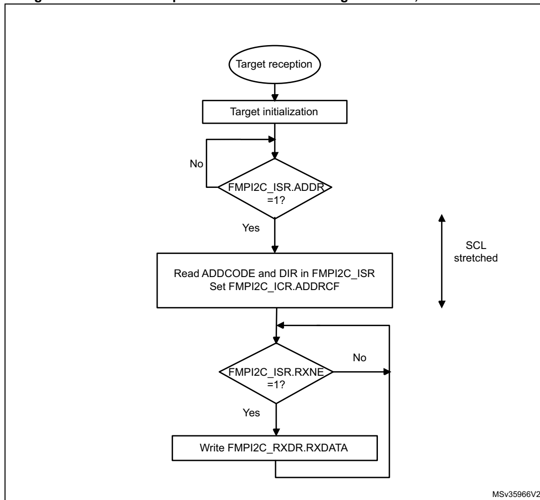
Figure 187. Transfer sequence flow for FMPI2C target receiver, NOSTRETCH = 0
