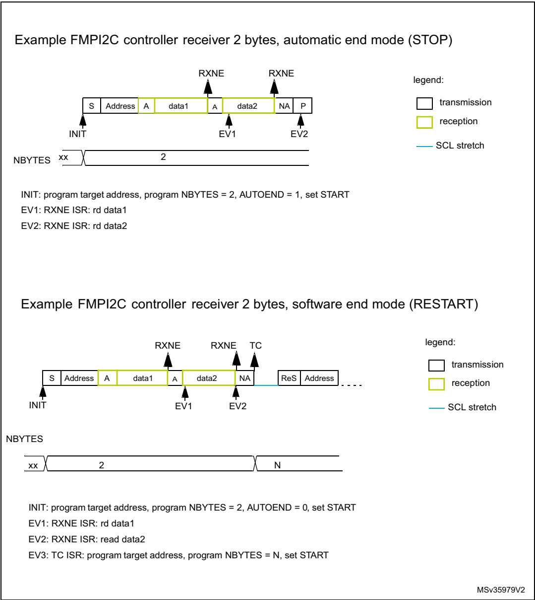
Figure 199. Transfer bus diagrams for FMPI2C controller receiver (mandatory events only)
