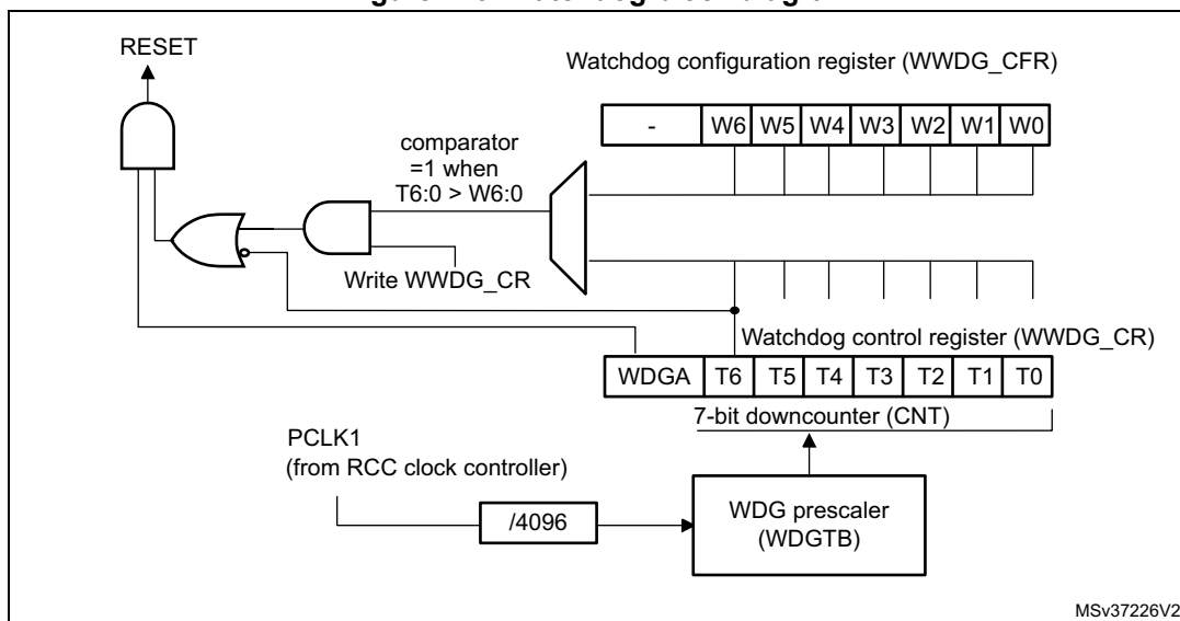
Figure 173. Watchdog block diagram
