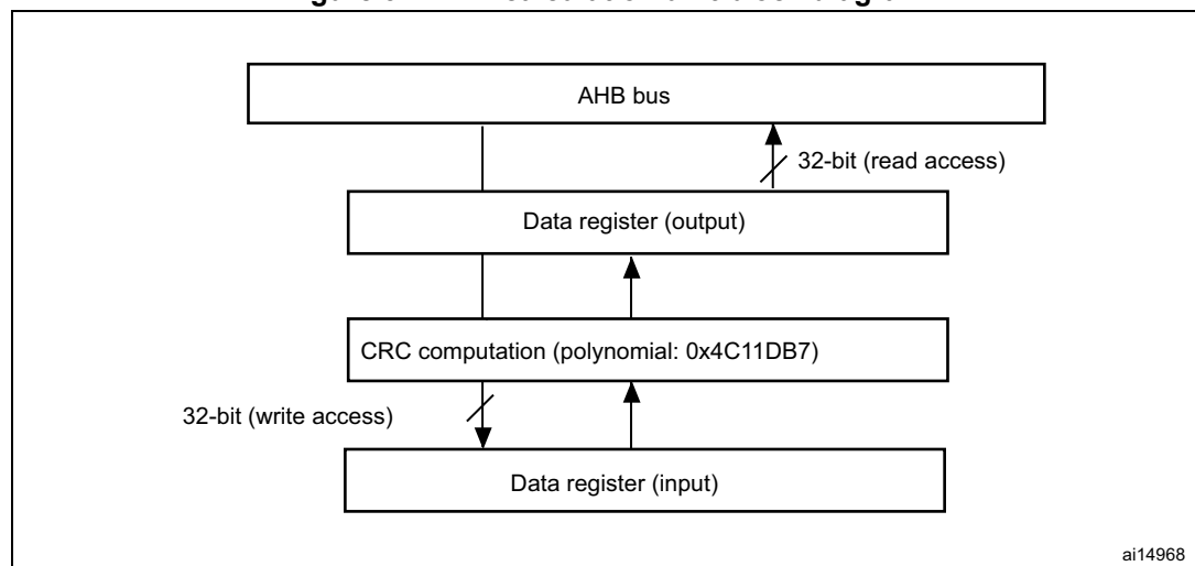
Figure 31. CRC calculation unit block diagram
