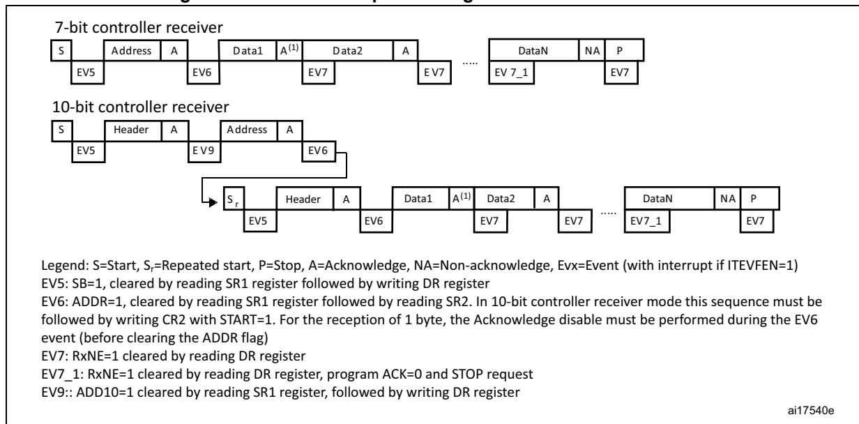
Figure 212. Transfer sequence diagram for controller receiver
