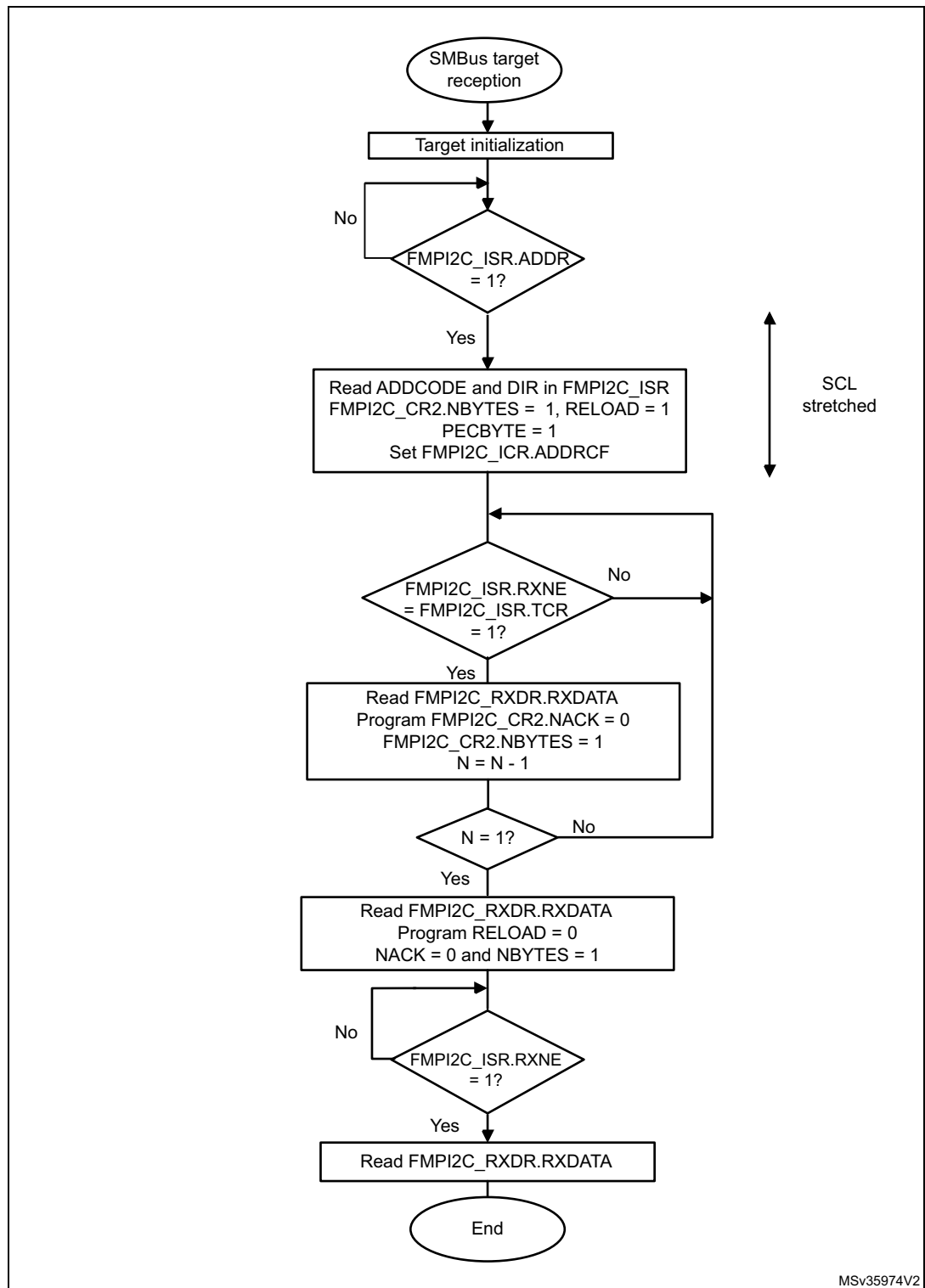
Figure 203. Transfer sequence flow for SMBus target receiver N bytes + PEC
