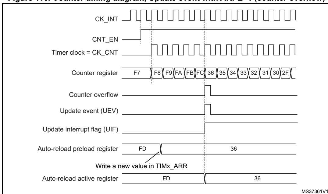
Figure 116. Counter timing diagram, Update event with ARPE=1 (counter overflow)
