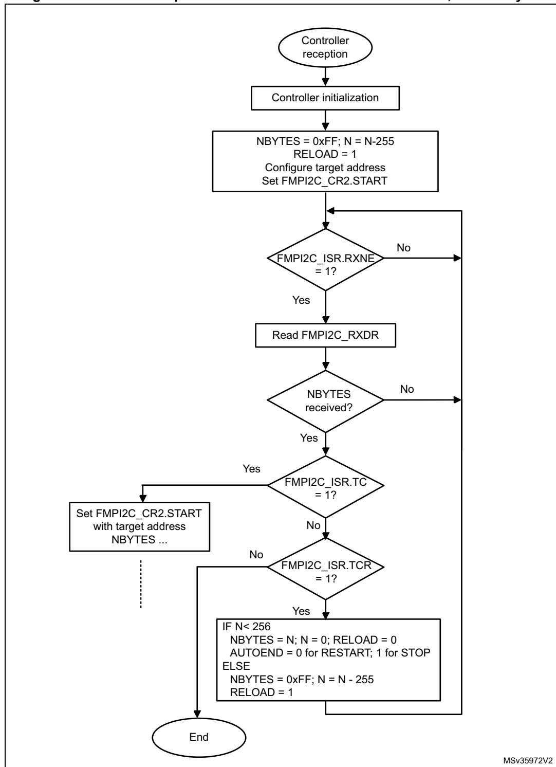
Figure 198. Transfer sequence flow for FMPI2C controller receiver, N > 255 bytes
