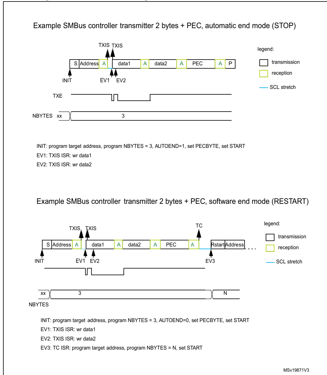
Figure 205. Bus transfer diagrams for SMBus controller transmitter
