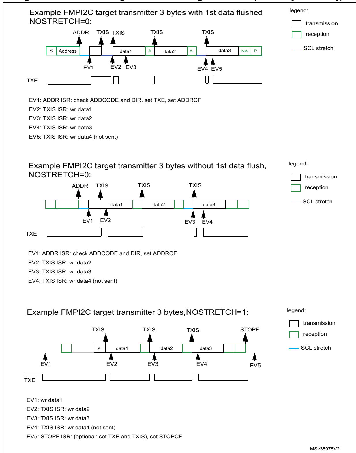
Figure 186. Transfer bus diagrams for FMPI2C target transmitter (mandatory events only)
