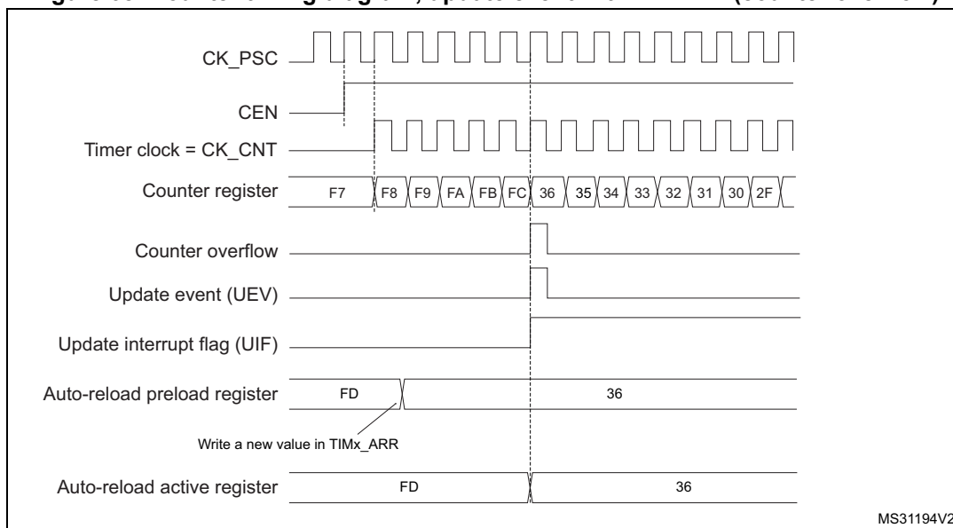
Figure 68. Counter timing diagram, update event with ARPE=1 (counter overflow)
