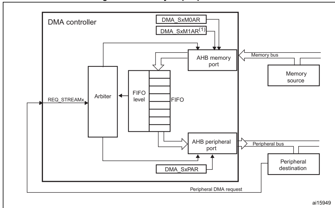
Figure 26. Memory-to-peripheral mode
