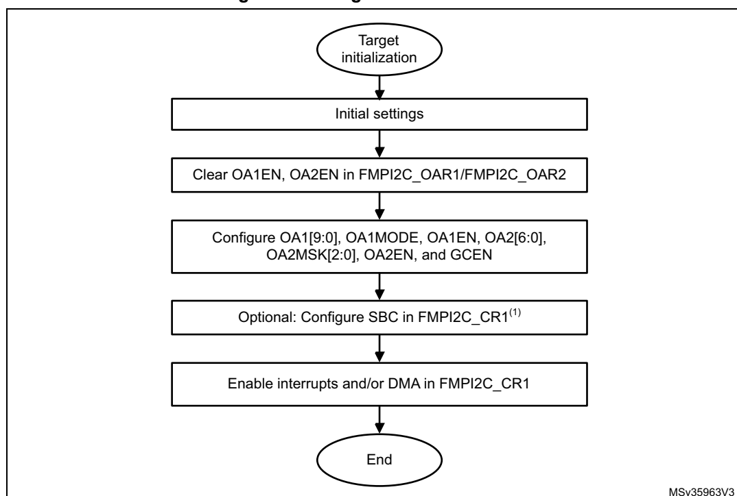
Figure 183. Target initialization flow
