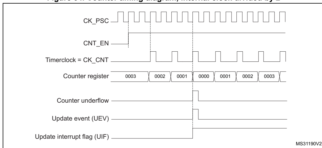
Figure 64. Counter timing diagram, internal clock divided by 2
