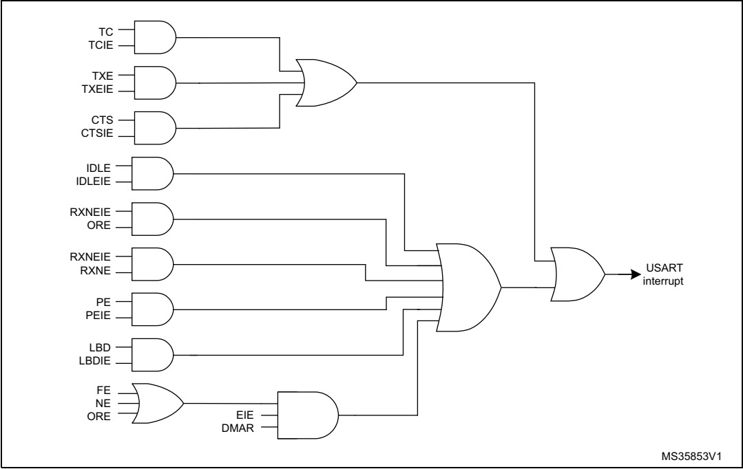
Figure 238. USART interrupt mapping diagram
