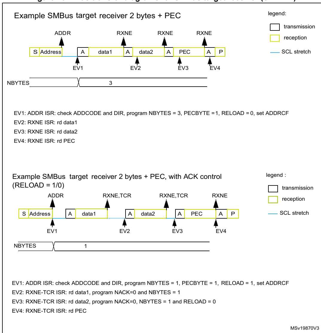
Figure 204. Bus transfer diagrams for SMBus target receiver (SBC = 1)
