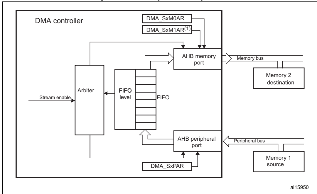
Figure 27. Memory-to-memory mode
