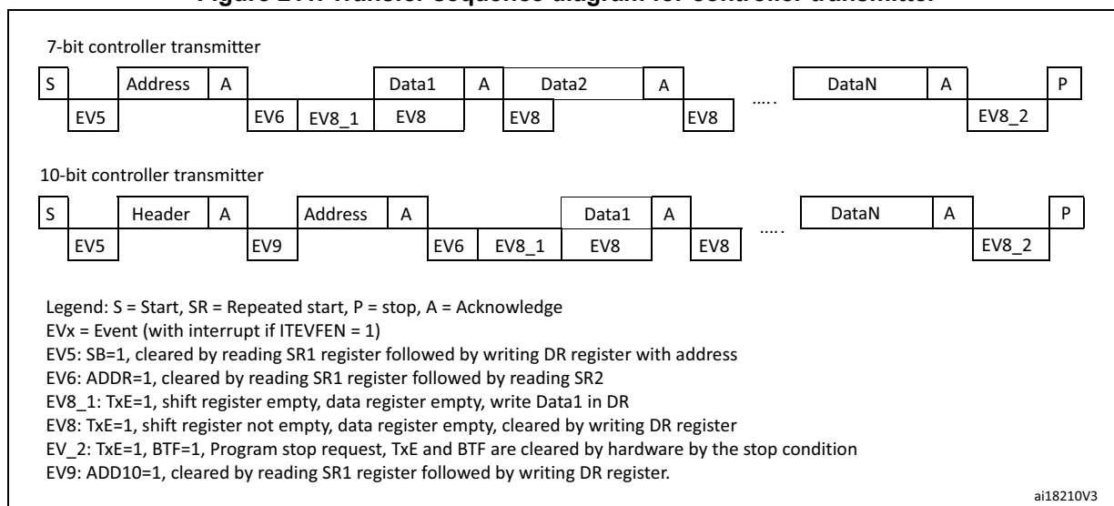
Figure 211. Transfer sequence diagram for controller transmitter
