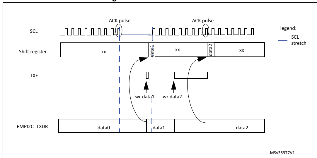
Figure 182. Data transmission
