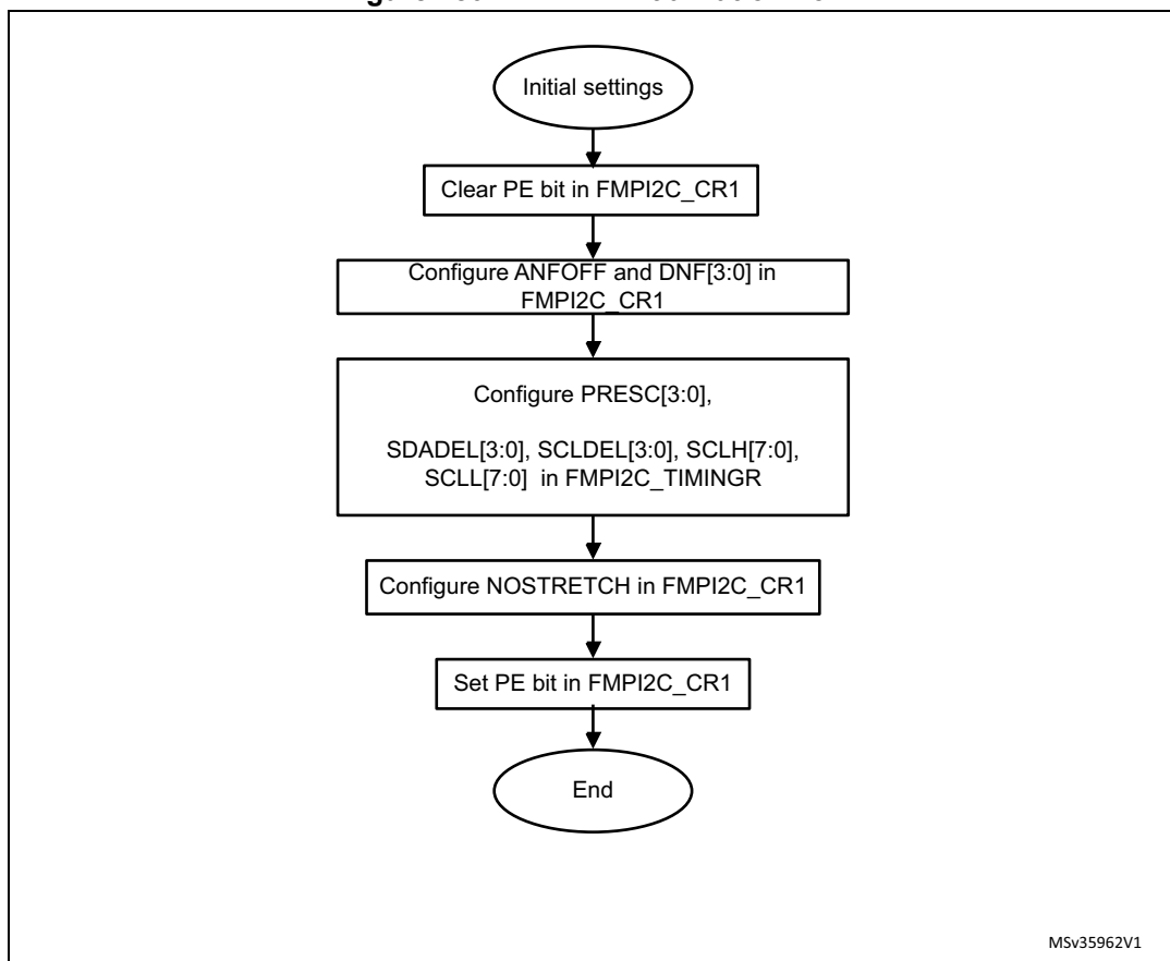
Figure 180. FMPI2C initialization flow
