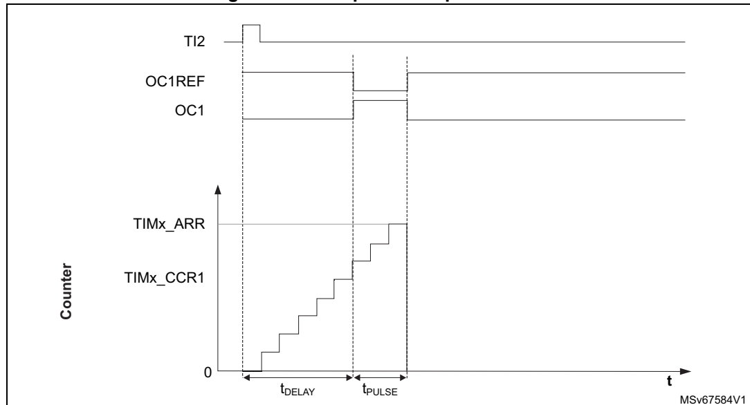
Figure 89. Example of one pulse mode
