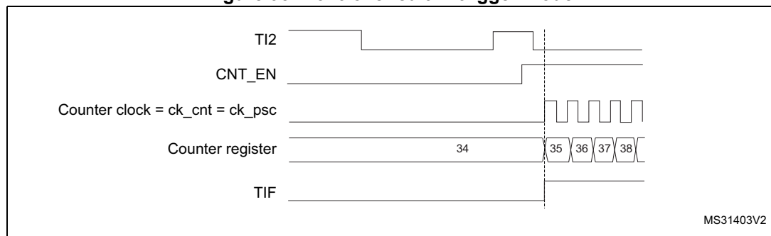
Figure 95. Control circuit in trigger mode
