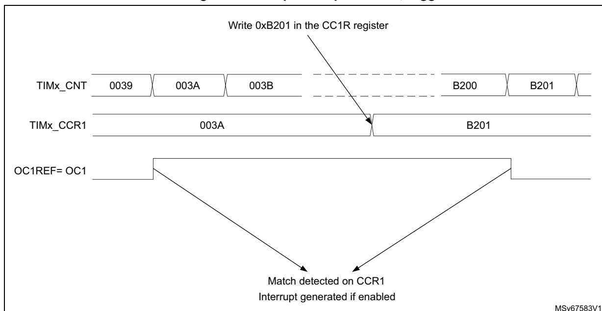
Figure 124. Output compare mode, toggle on OC1
