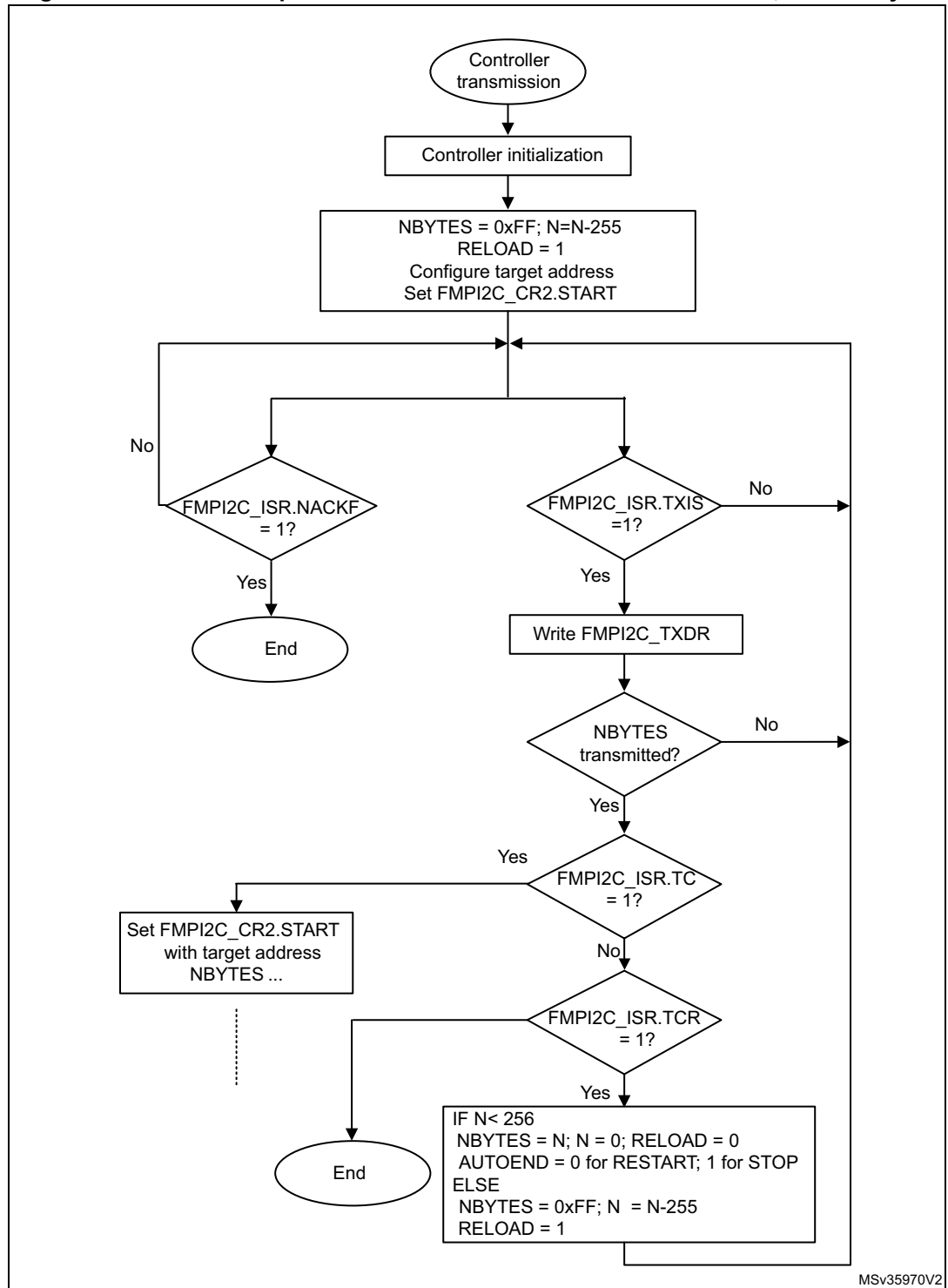
Figure 195. Transfer sequence flow for FMPI2C controller transmitter, N &gt; 255 bytes
