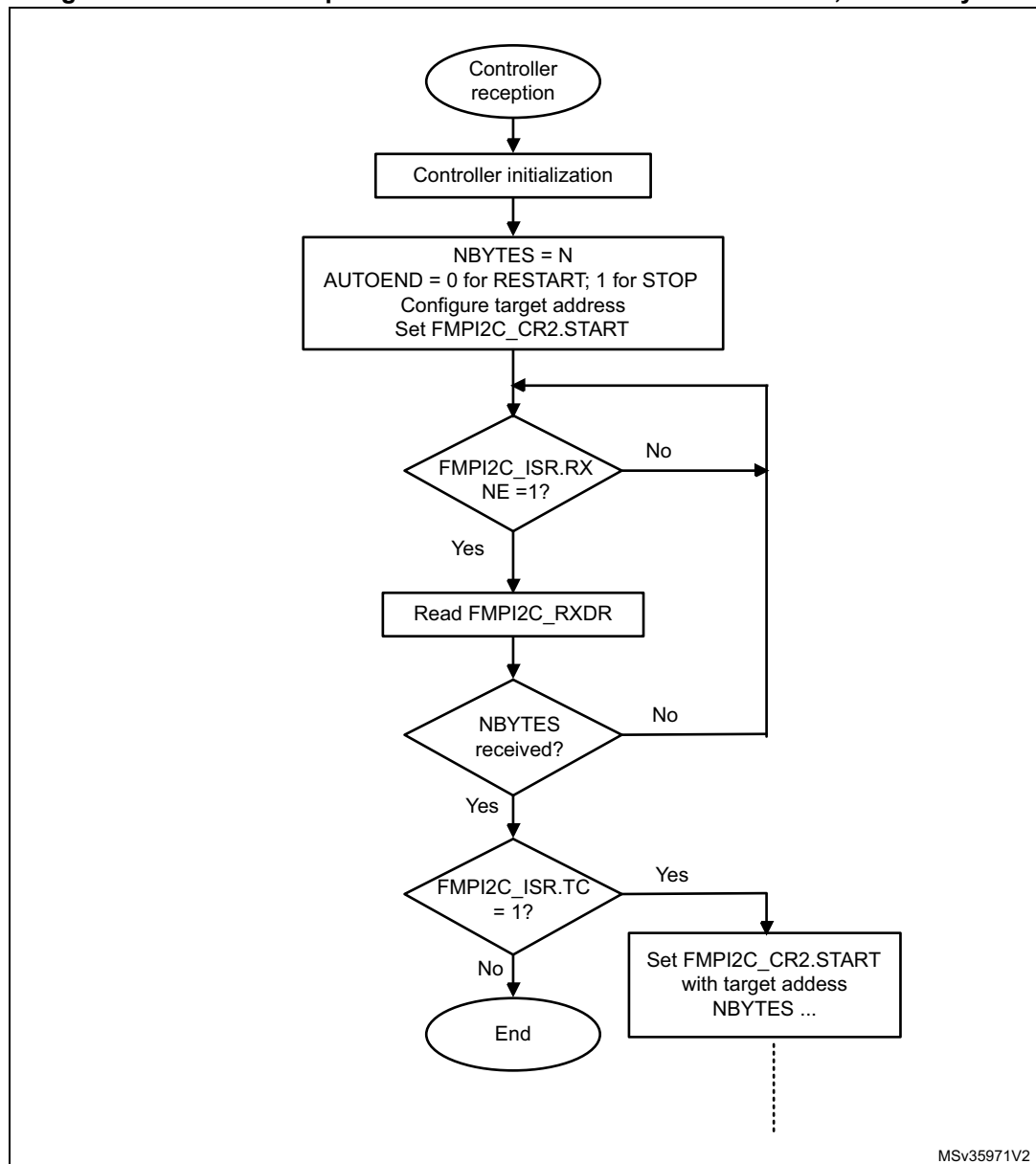
Figure 197. Transfer sequence flow for FMPI2C controller receiver, N \leq 255 bytes
