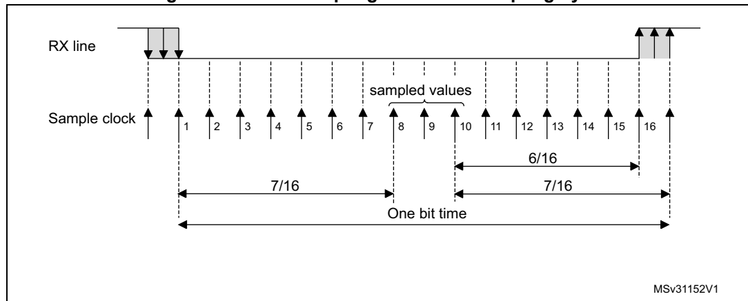
Figure 219. Data sampling when oversampling by 16
