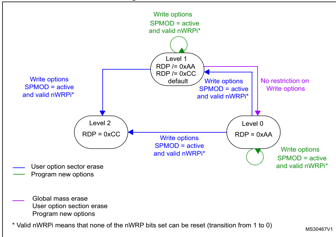
Figure 6. PCROP levels
