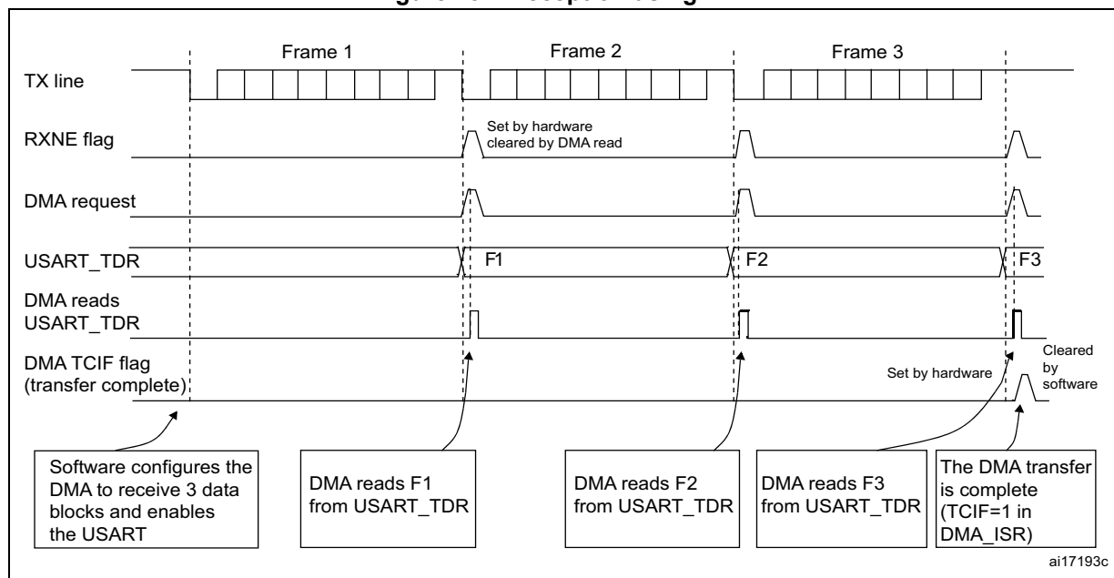
Figure 234. Reception using DMA
