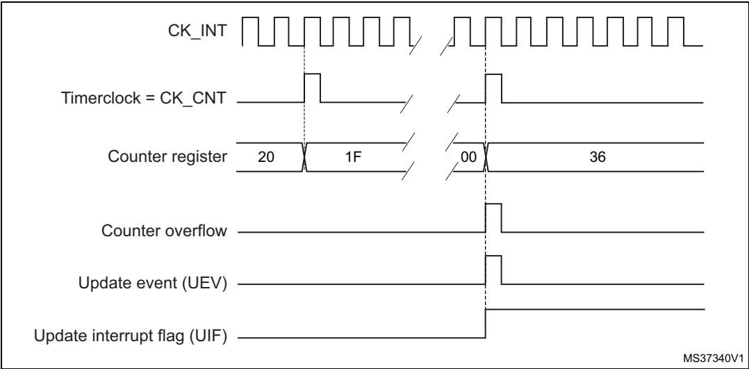
Figure 109. Counter timing diagram, internal clock divided by N
