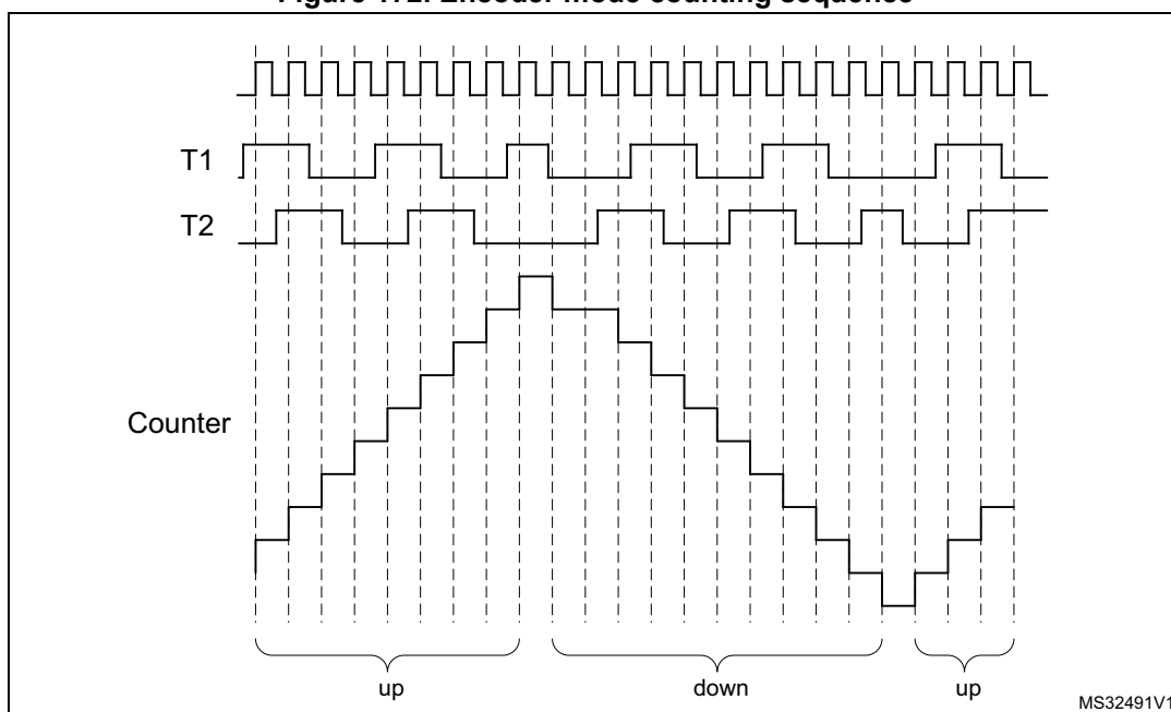
Figure 172. Encoder mode counting sequence
