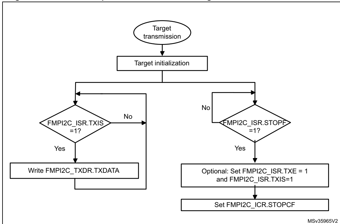
Figure 185. Transfer sequence flow for FMPI2C target transmitter, NOSTRETCH = 1
