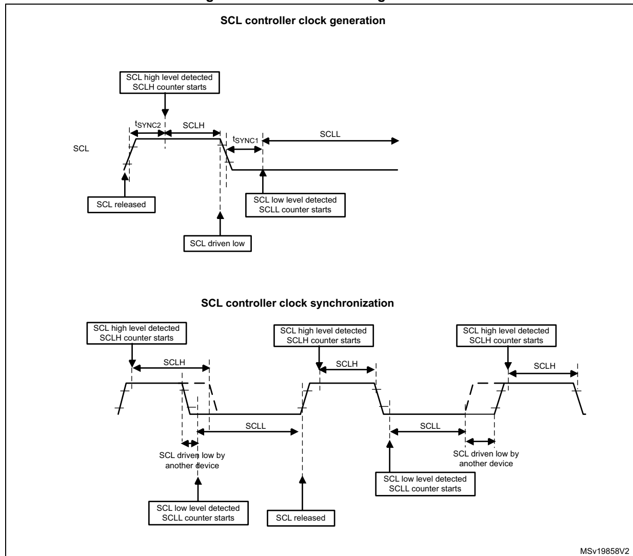
Figure 190. Controller clock generation
