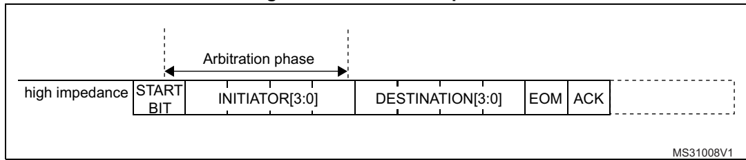
Figure 288. Arbitration phase
