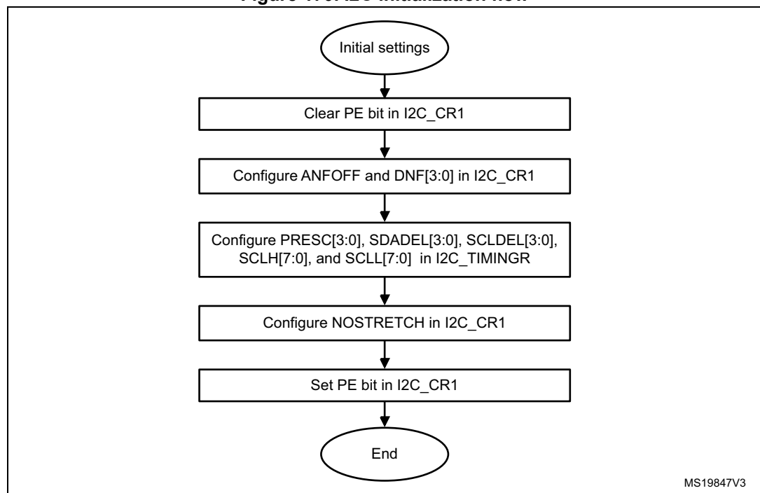
Figure 170. I2C initialization flow
