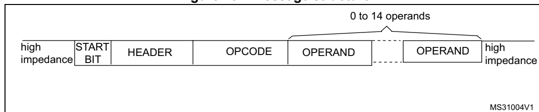
Figure 284. Message structure
