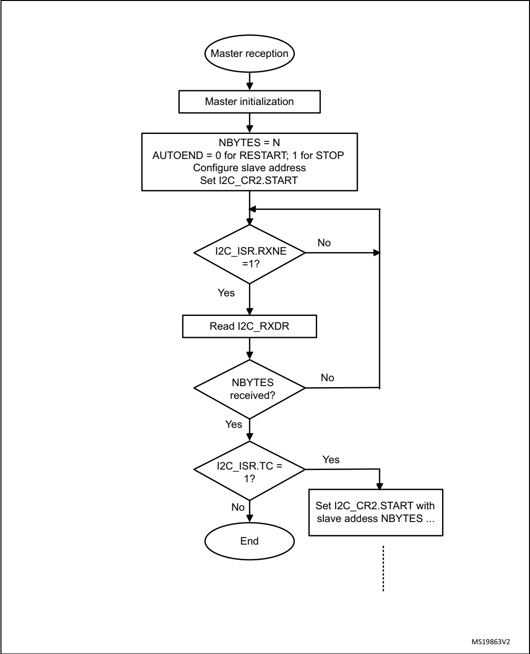
Figure 187. Transfer sequence flow for I2C master receiver for N \leq 255 bytes
