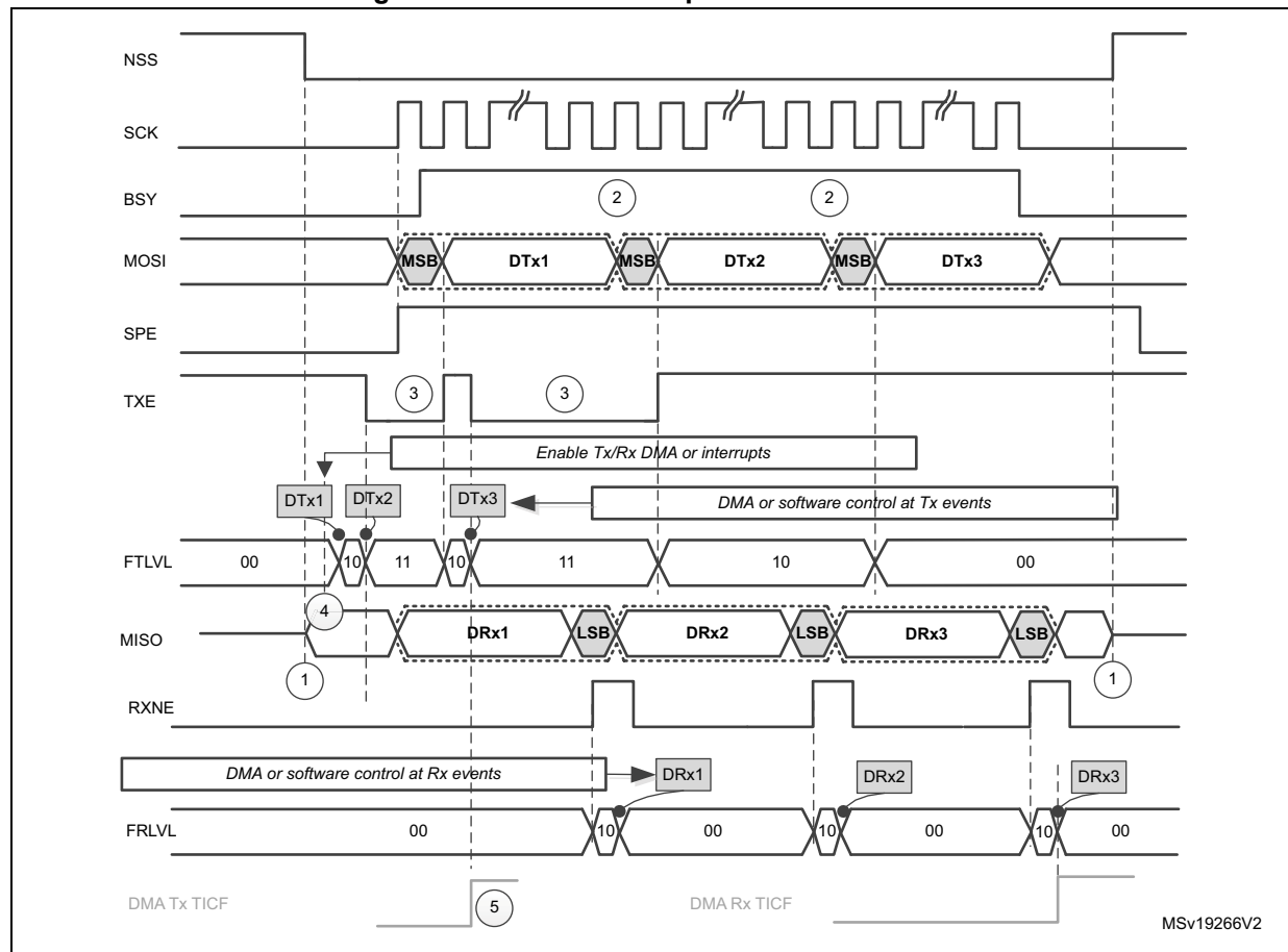
Figure 232. Master full-duplex communication
