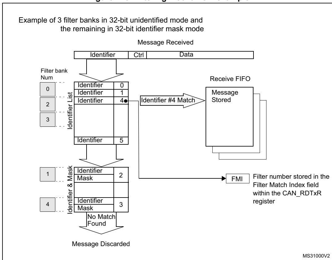
Figure 275. Filtering mechanism example
