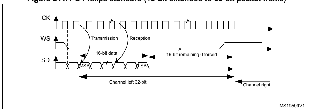
Figure 244. I 2 S Philips standard (16-bit extended to 32-bit packet frame)
