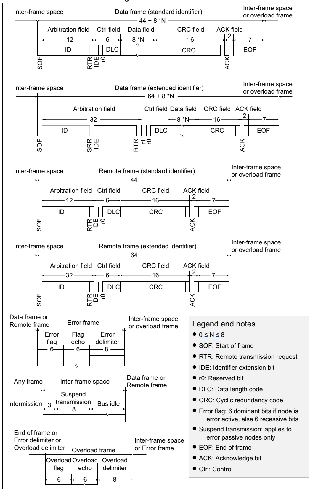
Figure 278. CAN frames
