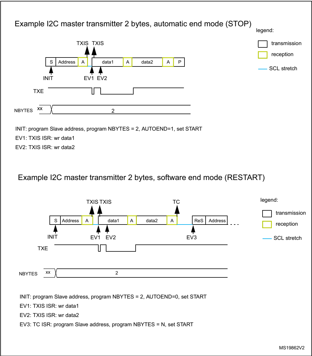
Figure 186. Transfer bus diagrams for I2C master transmitter (mandatory events only)
