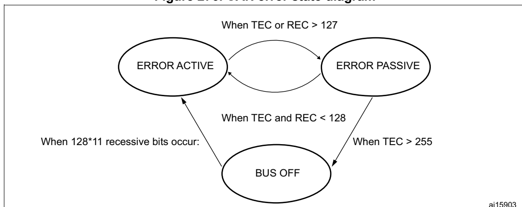
Figure 276. CAN error state diagram
