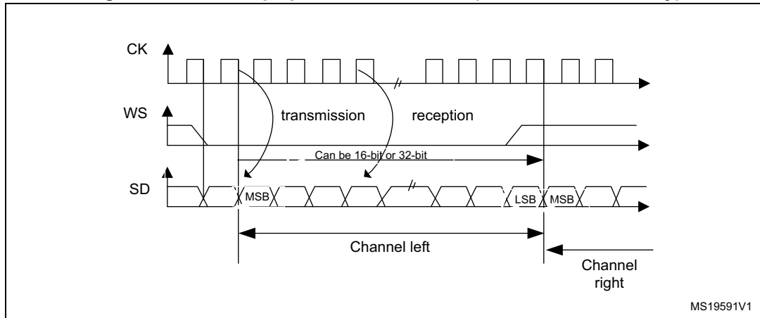
Figure 240. I 2 S Philips protocol waveforms (16/32-bit full accuracy)
