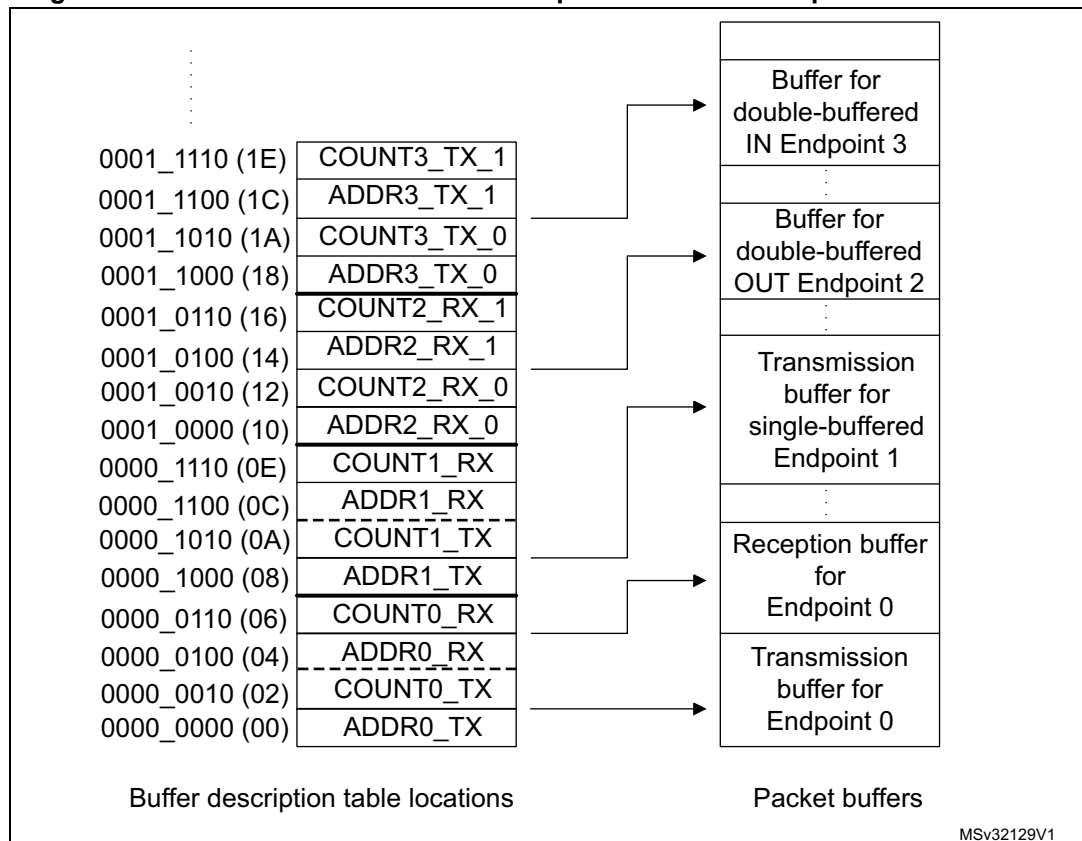
Figure 282. Packet buffer areas with examples of buffer description table locations
