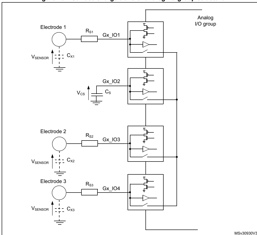
Figure 261. Surface charge transfer analog I/O group structure
