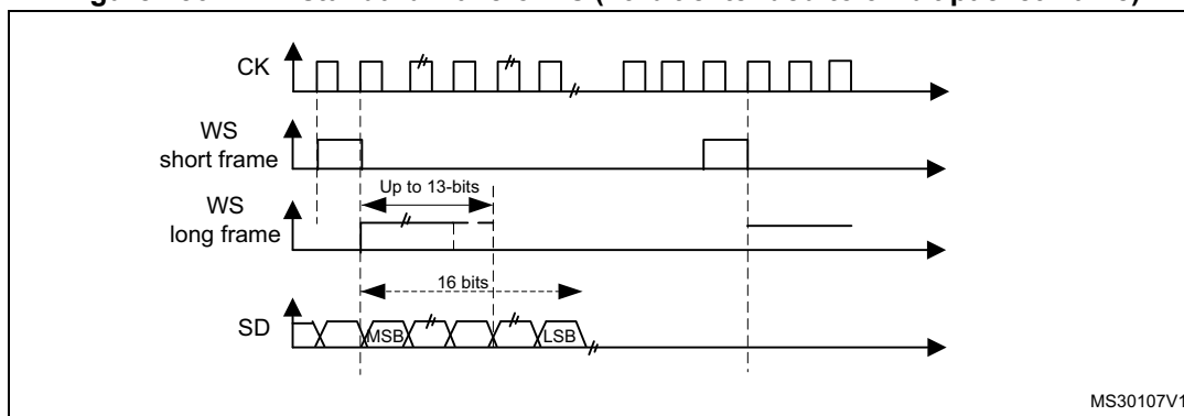
Figure 256. PCM standard waveforms (16-bit extended to 32-bit packet frame)
