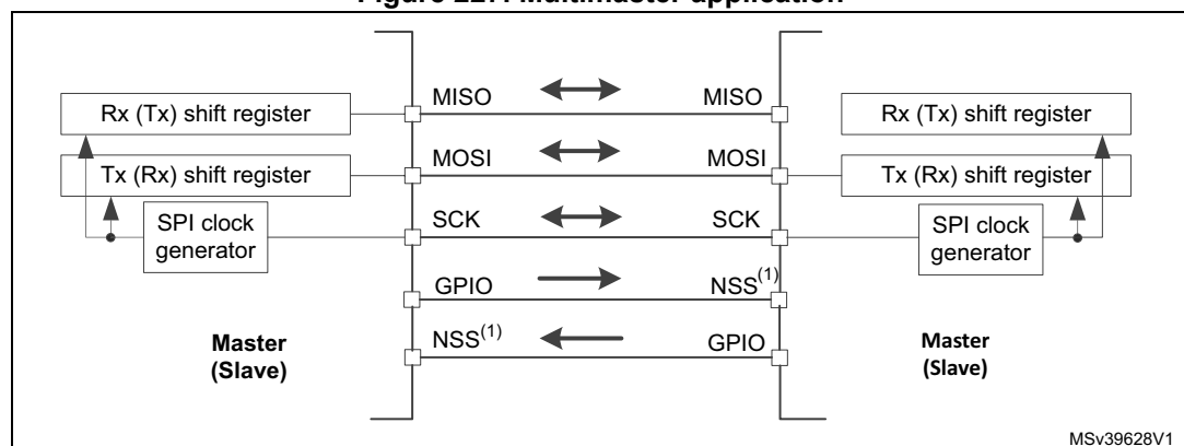
Figure 227. Multimaster application
