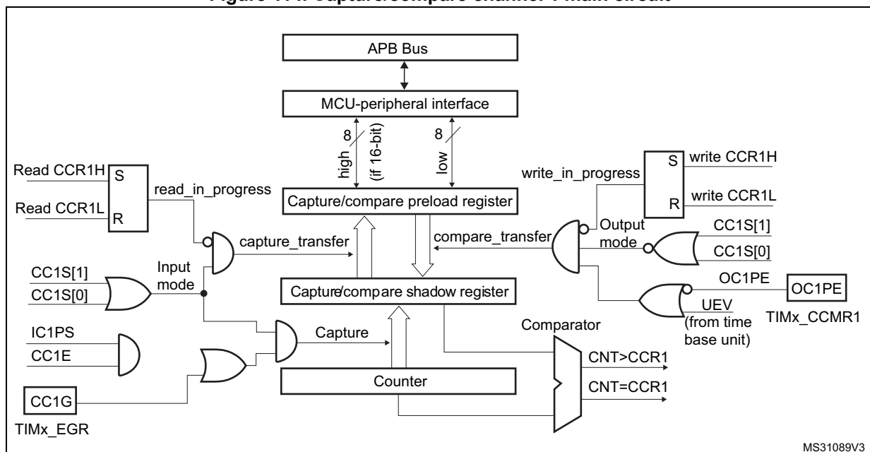
Figure 114. Capture/compare channel 1 main circuit
