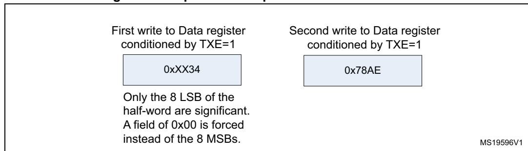
Figure 251. Operations required to transmit 0x3478AE
