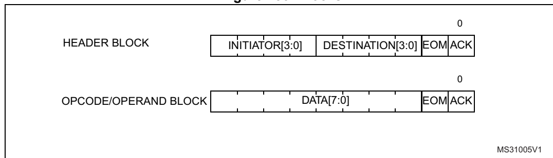
Figure 285. Blocks
