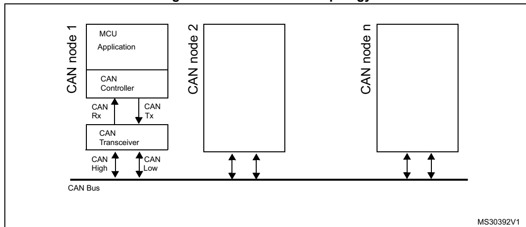
Figure 265. CAN network topology
