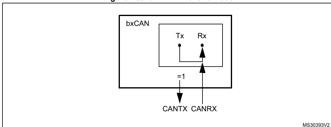
Figure 268. bxCAN in silent mode
