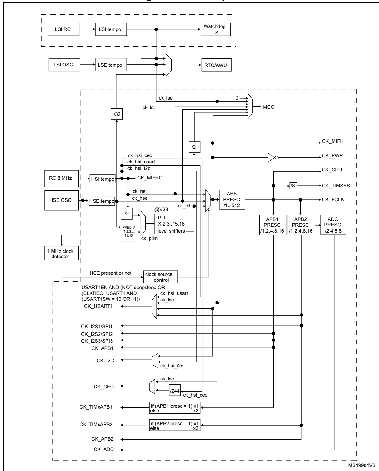
Figure 12. Clock tree part 1
