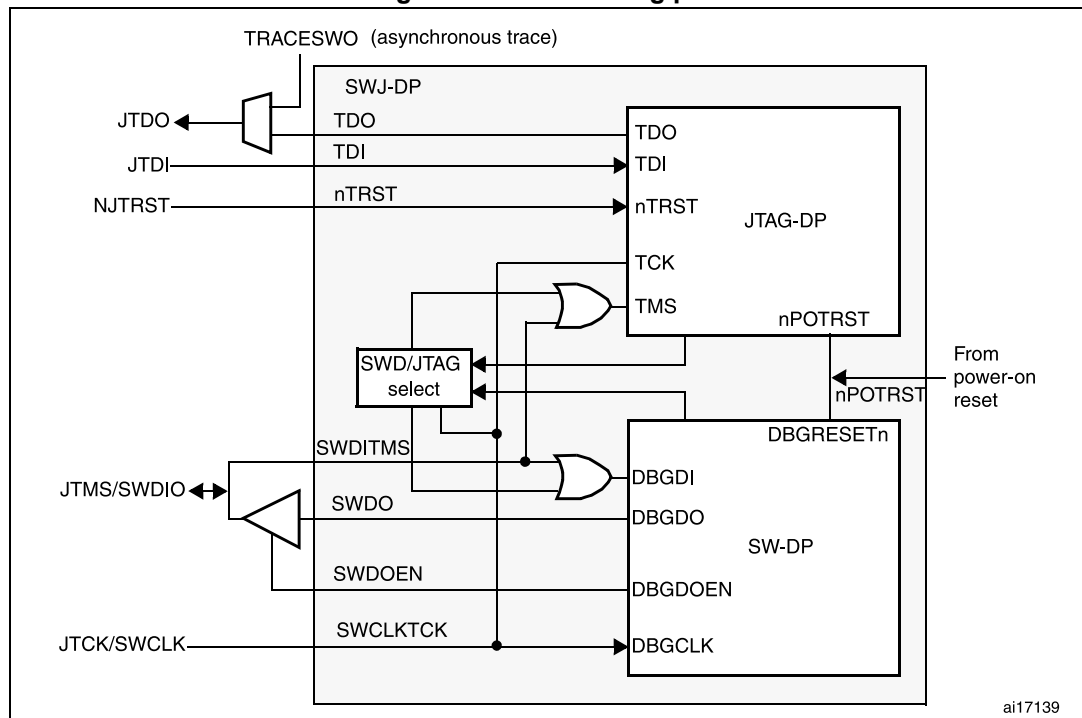
Figure 294. SWJ debug port
