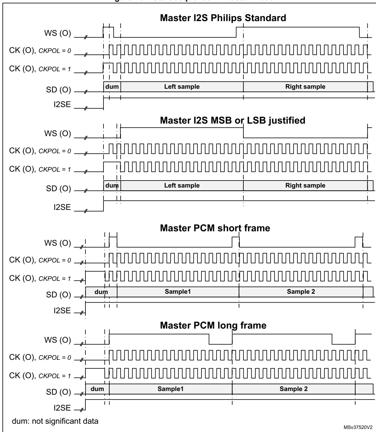
Figure 257. Start sequence in master mode
