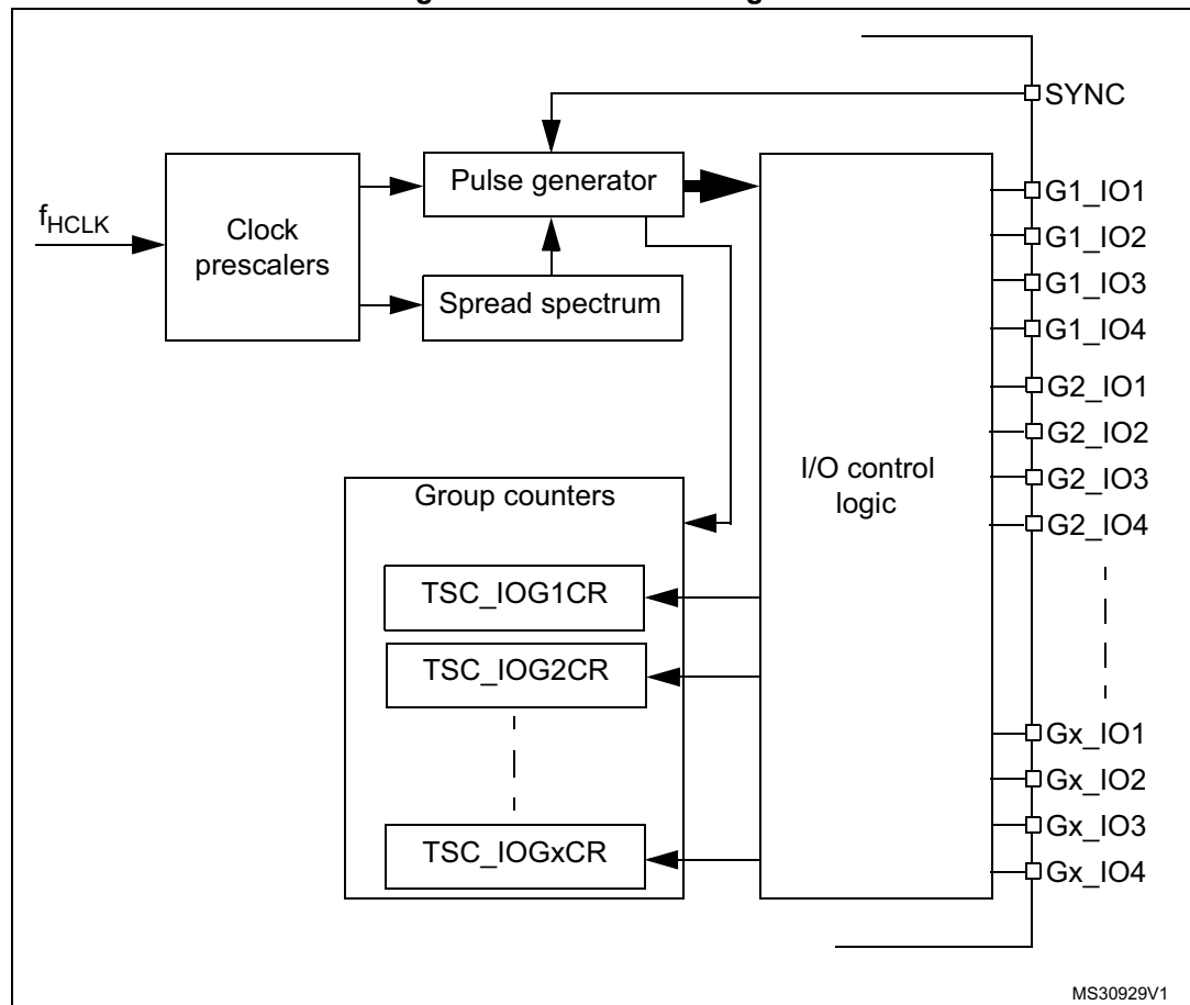
Figure 260. TSC block diagram
