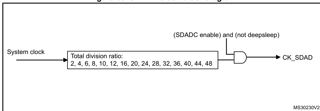
Figure 35. SDADC clock block diagram
