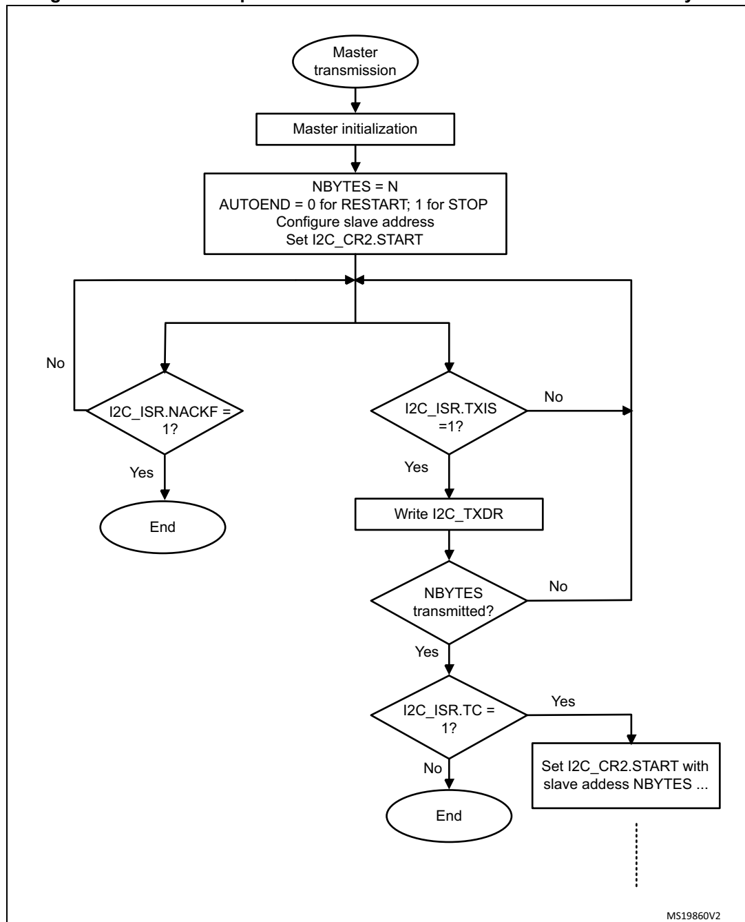
Figure 184. Transfer sequence flow for I2C master transmitter for N \leq 255 bytes
