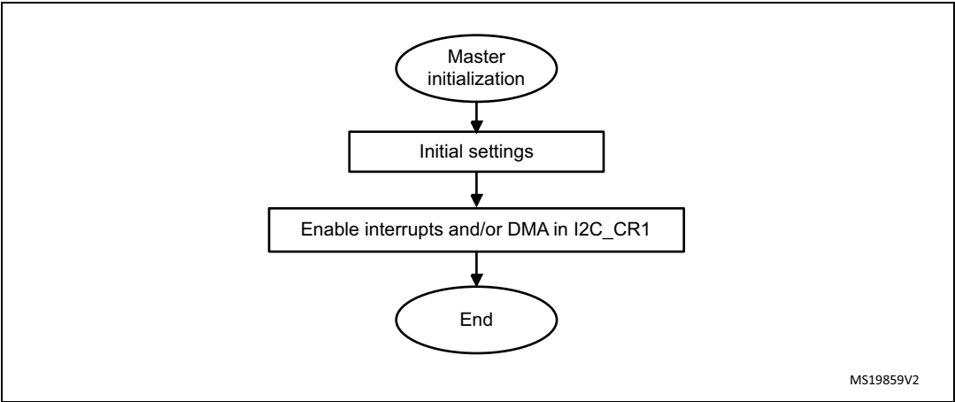
Figure 181. Master initialization flow
