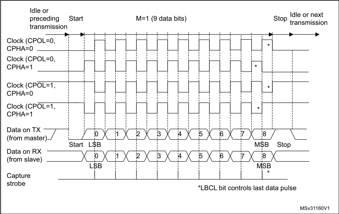
Figure 210. USART data clock timing diagram (M=1)
