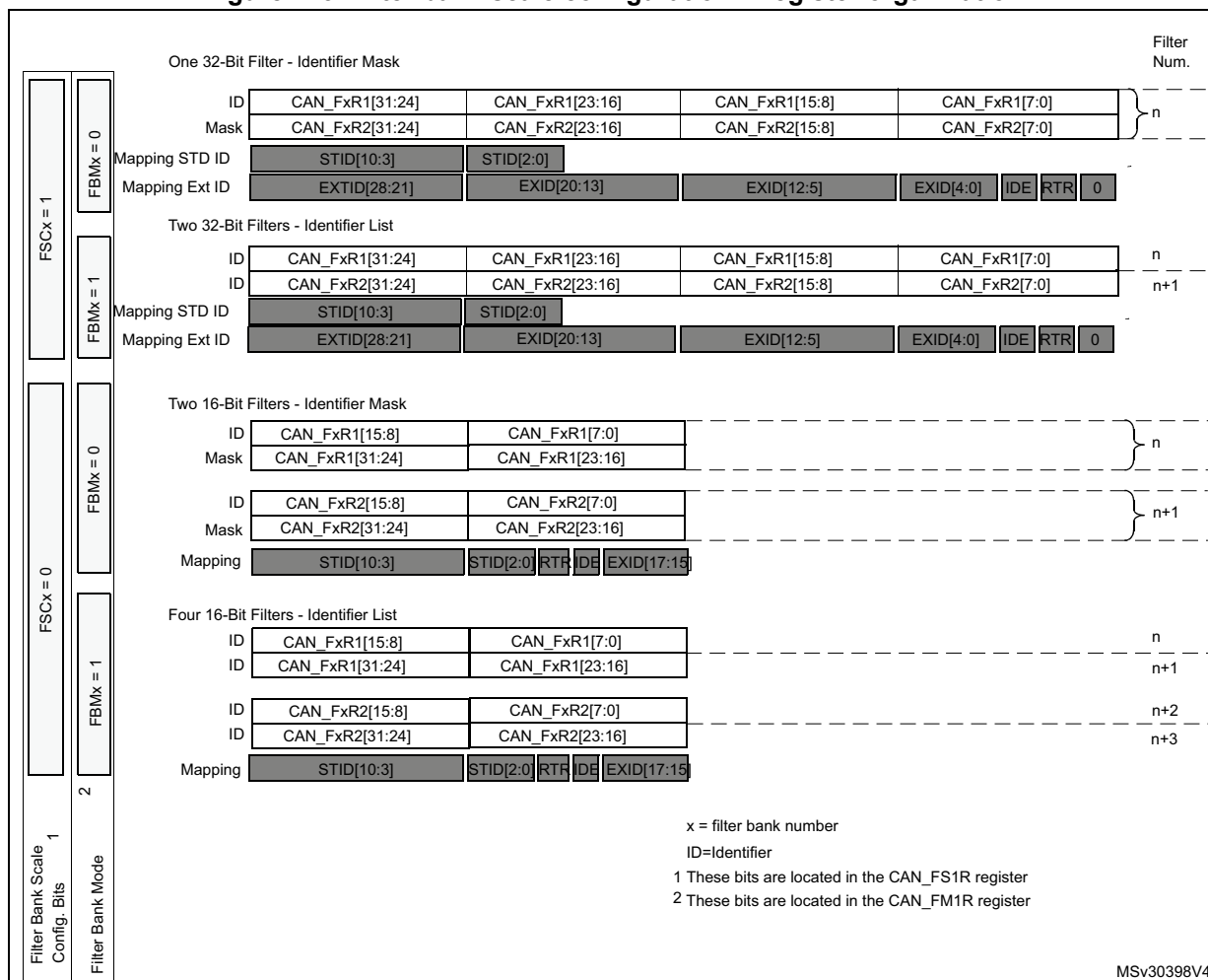
Figure 273. Filter bank scale configuration - Register organization
