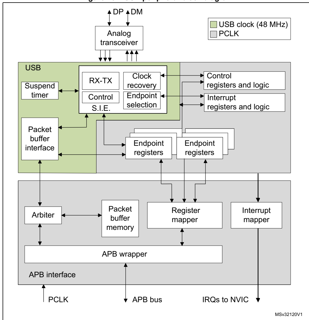
Figure 281. USB peripheral block diagram
