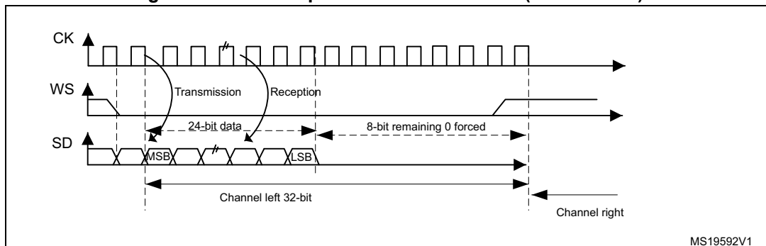
Figure 241. I 2 S Philips standard waveforms (24-bit frame)
