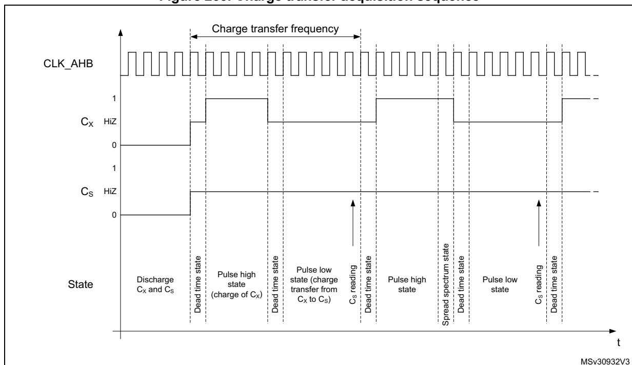
Figure 263. Charge transfer acquisition sequence
