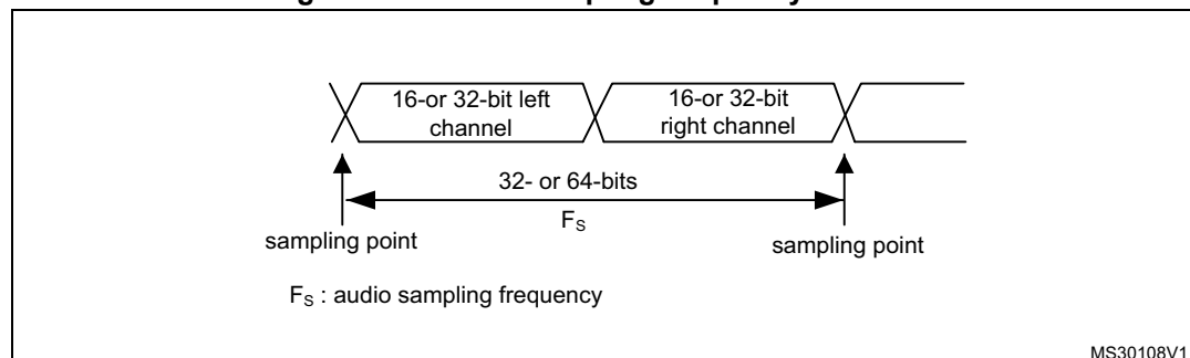
Figure 258. Audio sampling frequency definition
