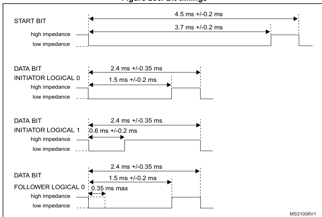
Figure 286. Bit timings
