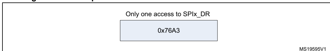
Figure 245. Example of 16-bit data frame extended to 32-bit channel frame
