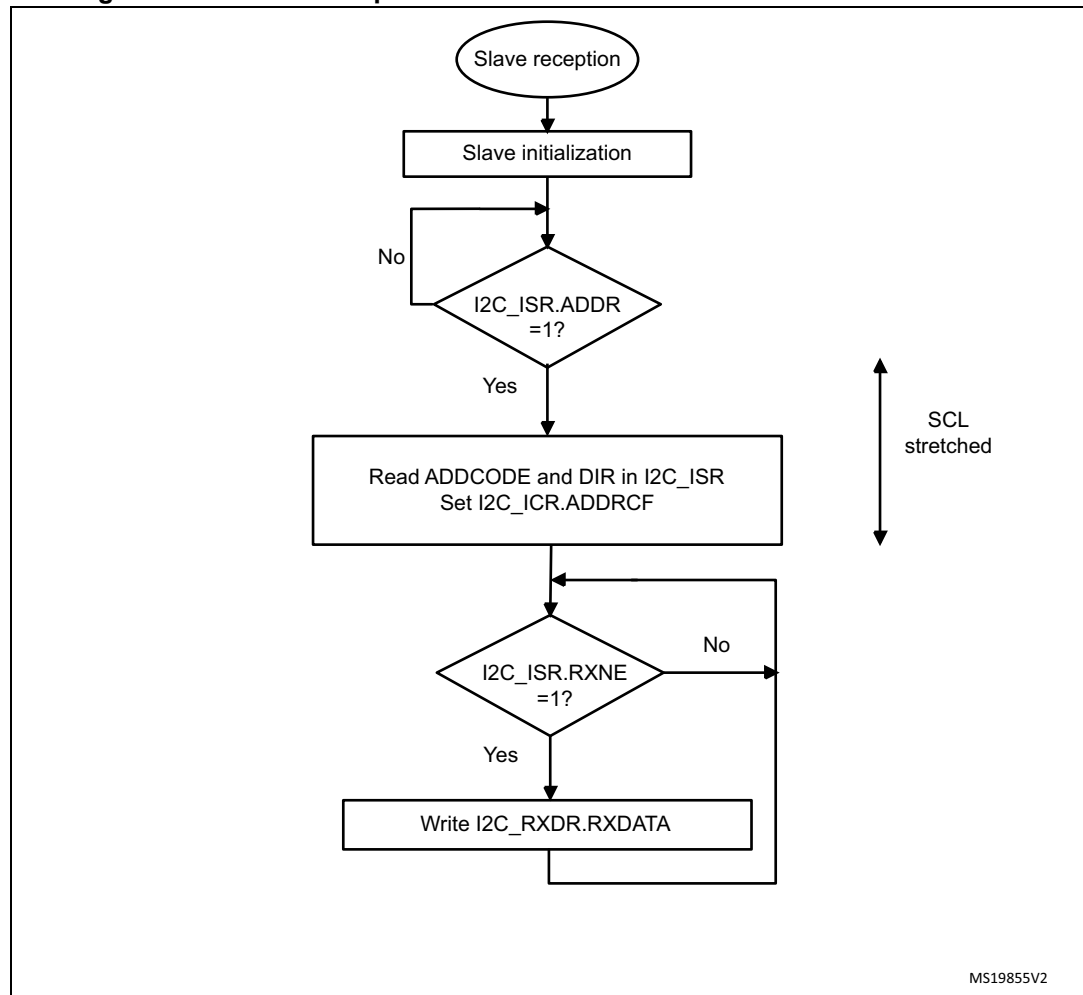
Figure 177. Transfer sequence flow for slave receiver with NOSTRETCH = 0
