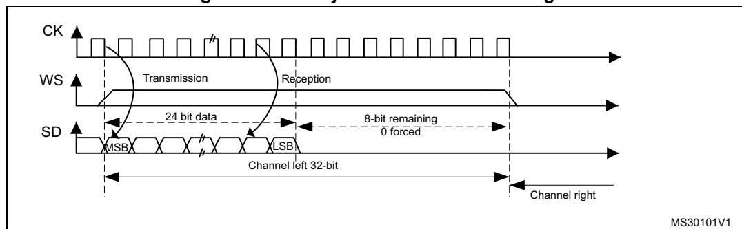
Figure 247. MSB justified 24-bit frame length
