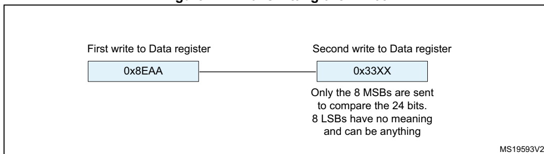
Figure 242. Transmitting 0x8EAA33
