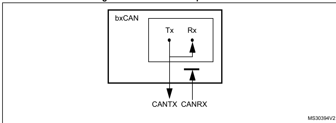
Figure 269. bxCAN in Loop back mode
