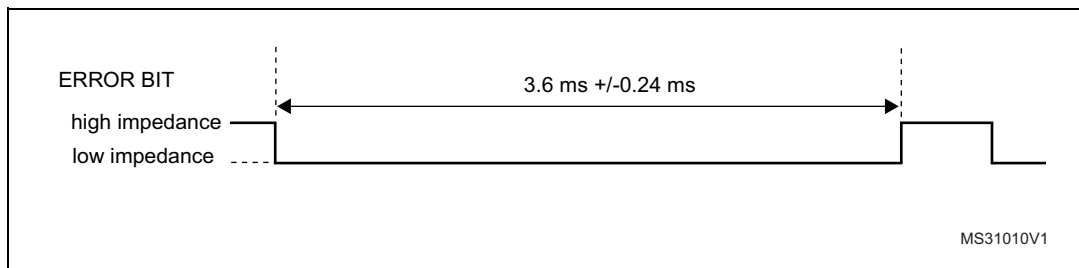
Figure 290. Error bit timing
