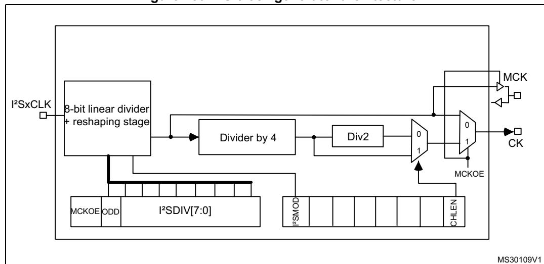
Figure 259. I 2 S clock generator architecture
