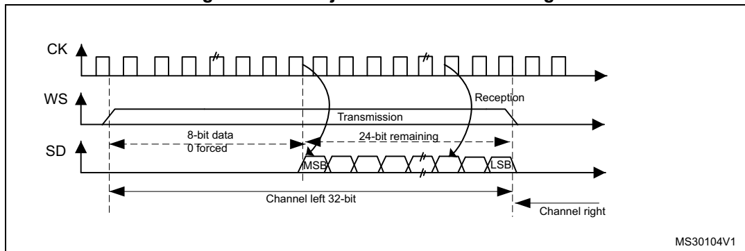
Figure 250. LSB justified 24-bit frame length
