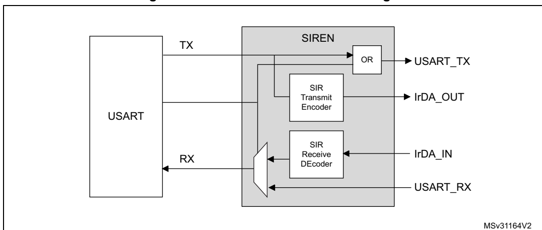
Figure 214. IrDA SIR ENDEC- block diagram
