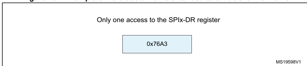
Figure 254. Example of 16-bit data frame extended to 32-bit channel frame
