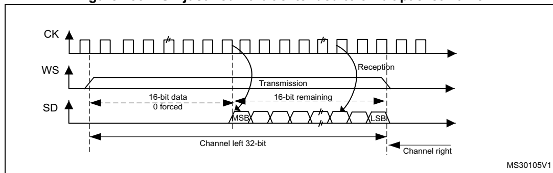
Figure 253. LSB justified 16-bit extended to 32-bit packet frame
