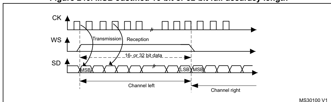
Figure 246. MSB Justified 16-bit or 32-bit full-accuracy length
