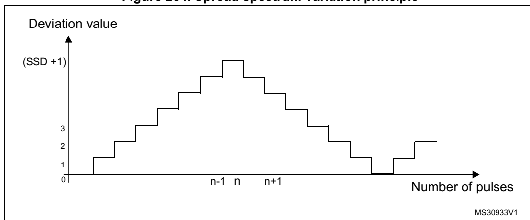
Figure 264. Spread spectrum variation principle
