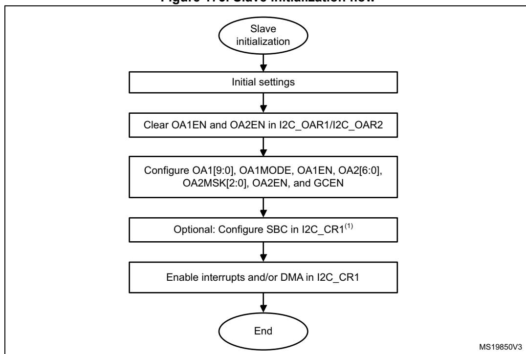
Figure 173. Slave initialization flow
