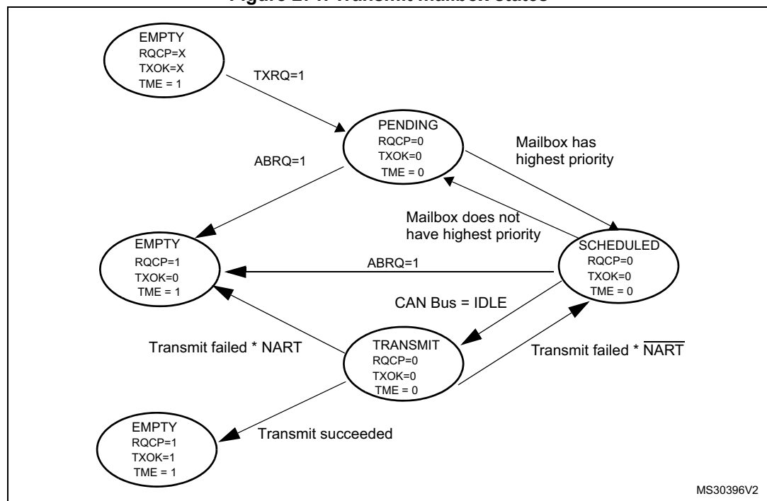
Figure 271. Transmit mailbox states
