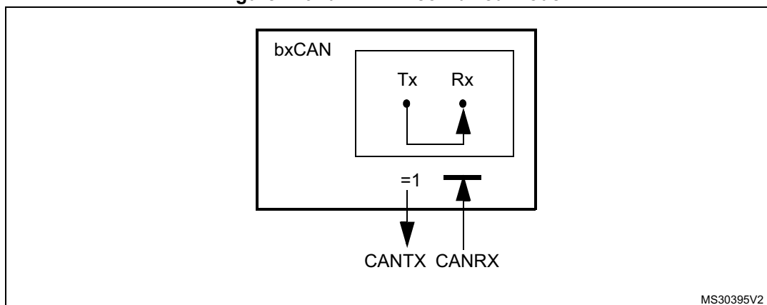
Figure 270. bxCAN in combined mode
