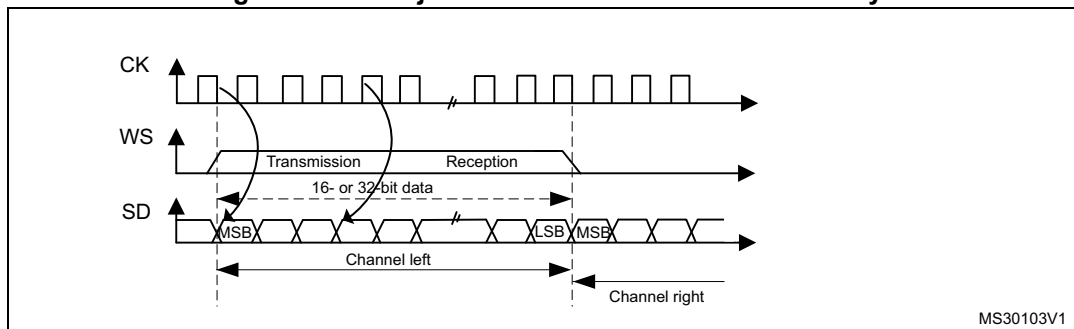
Figure 249. LSB justified 16-bit or 32-bit full-accuracy
