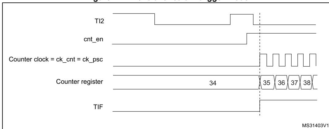
Figure 122. Control circuit in trigger mode
