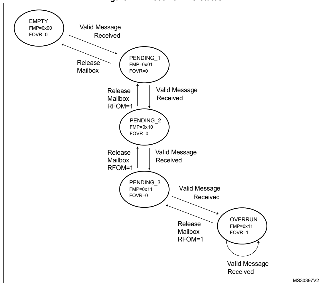
Figure 272. Receive FIFO states
