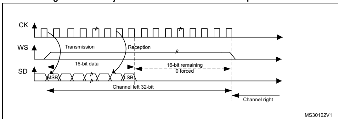
Figure 248. MSB justified 16-bit extended to 32-bit packet frame
