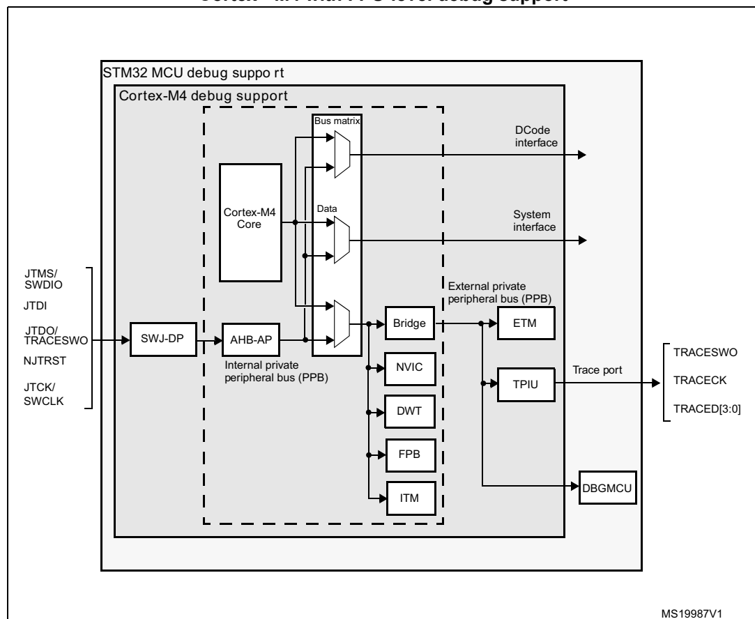
Figure 293. Block diagram of STM32F37xxx MCU and Cortex®-M4 with FPU-level debug support
