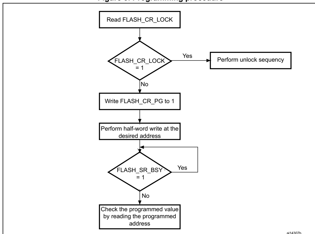
Figure 3. Programming procedure
