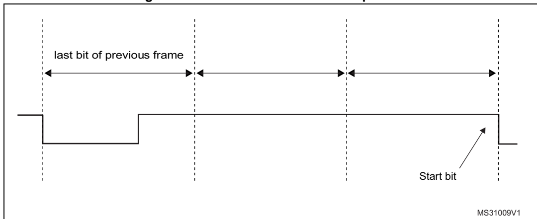
Figure 289. SFT of three nominal bit periods
