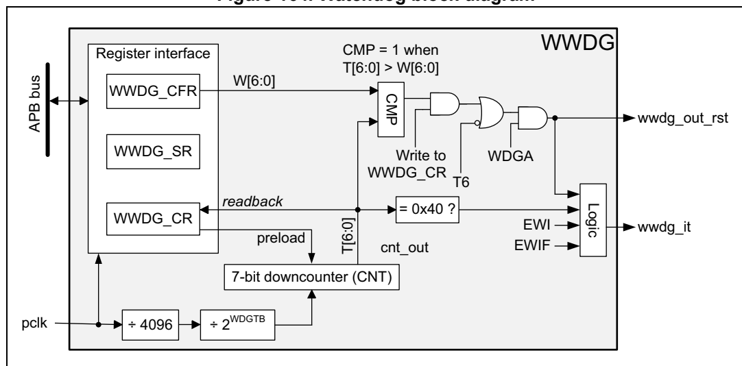
Figure 164. Watchdog block diagram
