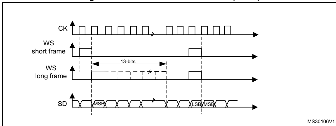
Figure 255. PCM standard waveforms (16-bit)
