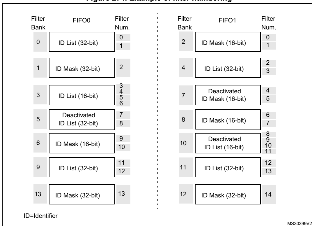
Figure 274. Example of filter numbering
