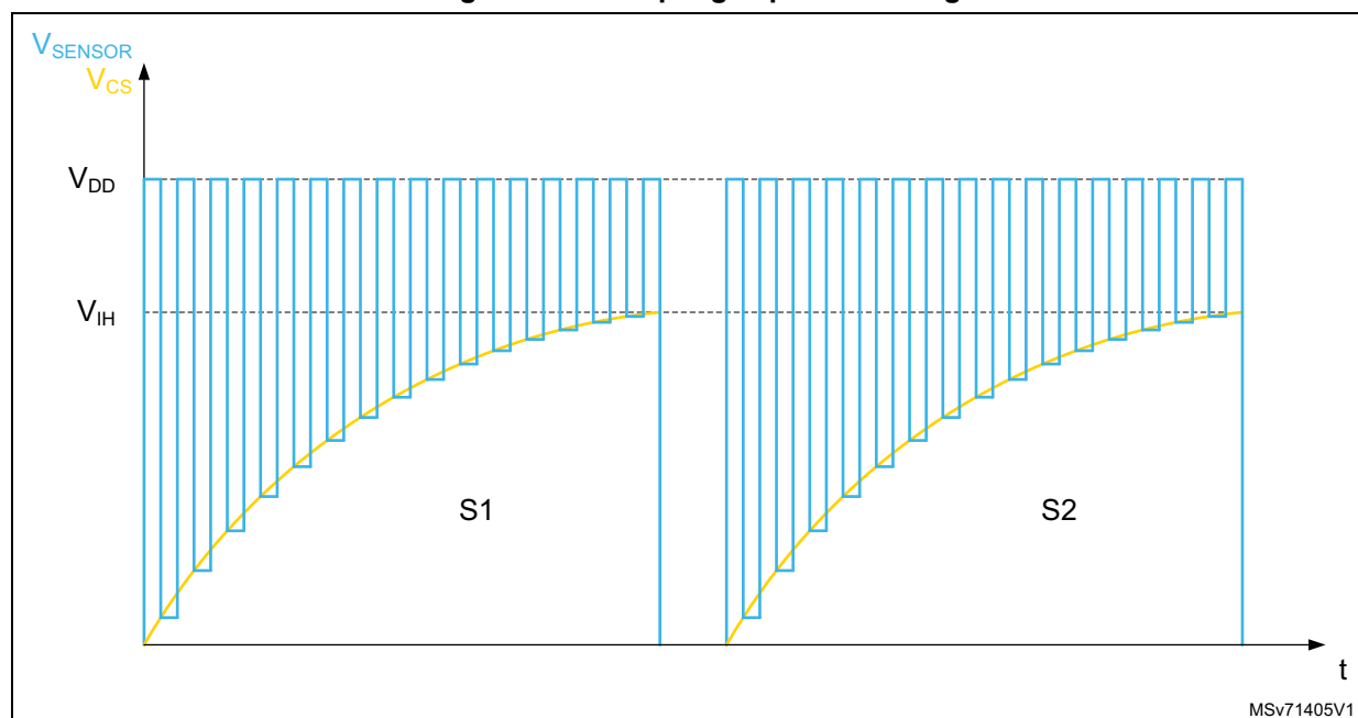
Figure 262. Sampling capacitor voltage variation
