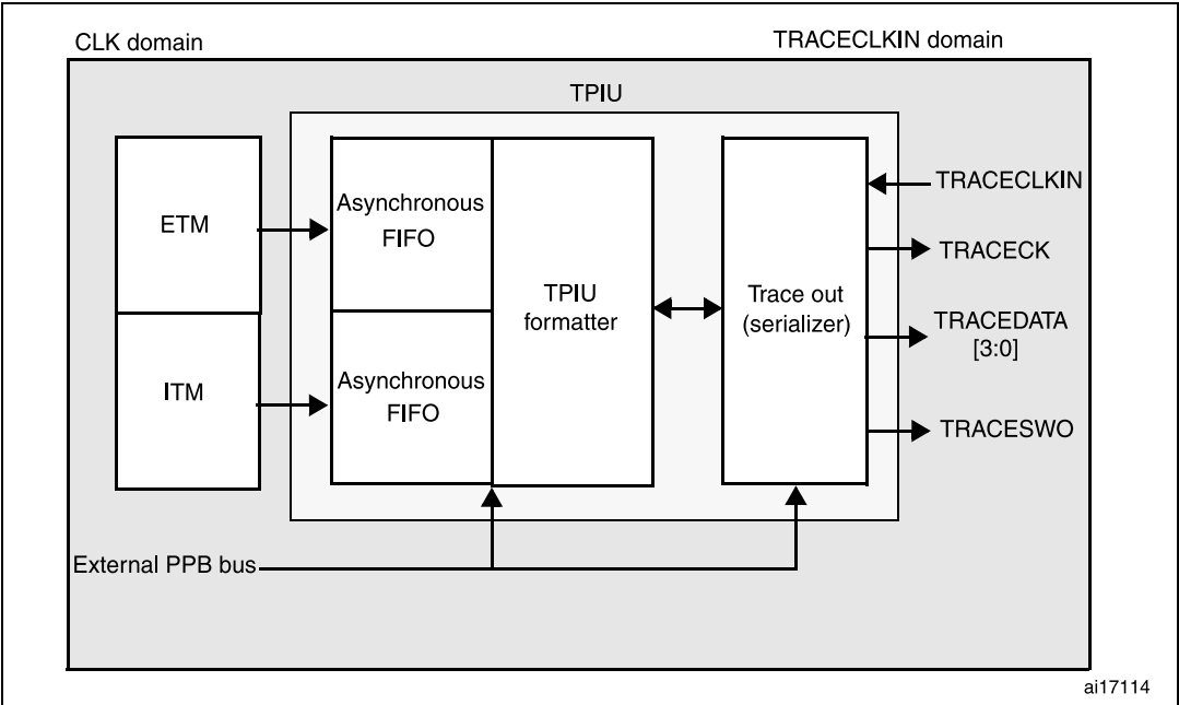
Figure 296. TPIU block diagram
