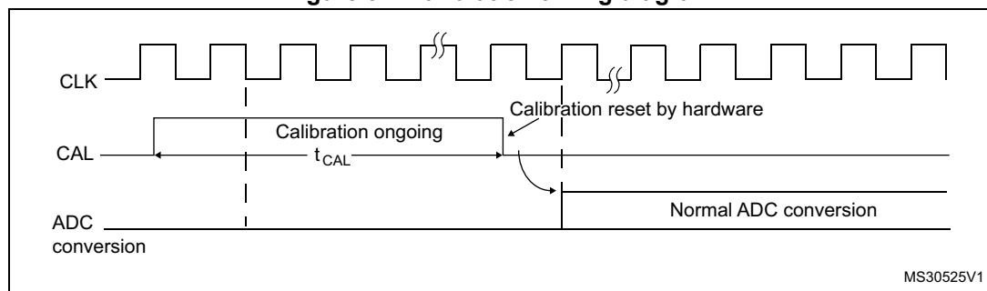
Figure 31. Calibration timing diagram
