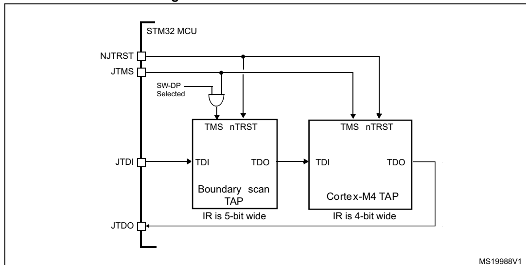
Figure 295. JTAG TAP connections
