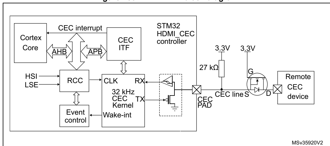
Figure 283. HDMI-CEC block diagram
