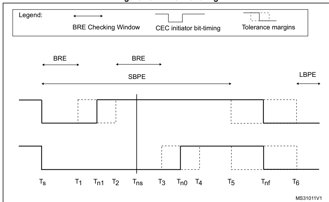
Figure 291. Error handling
