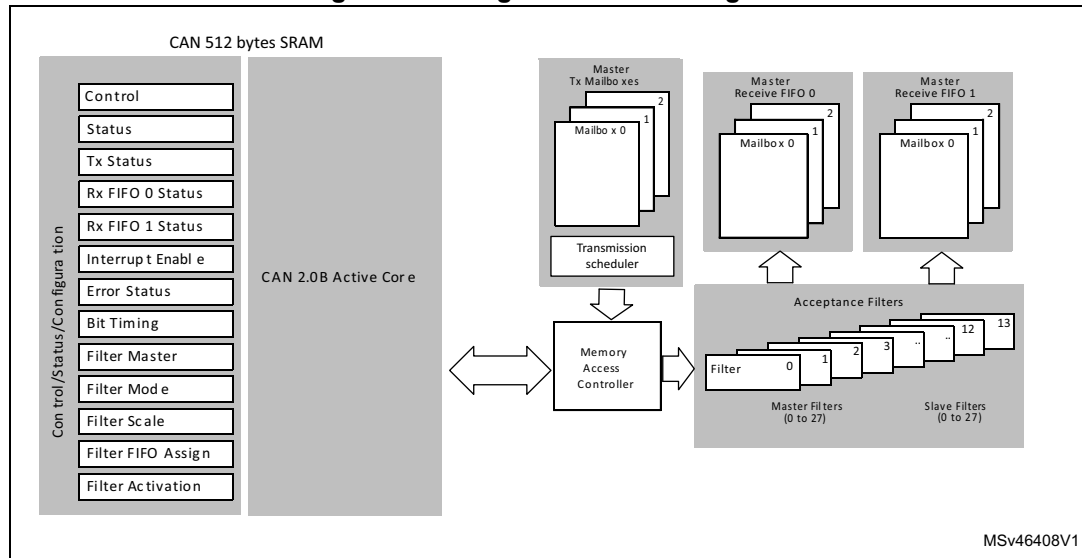
Figure 266. Single-CAN block diagram
