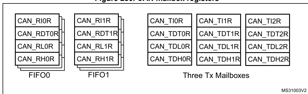
Figure 280. CAN mailbox registers
