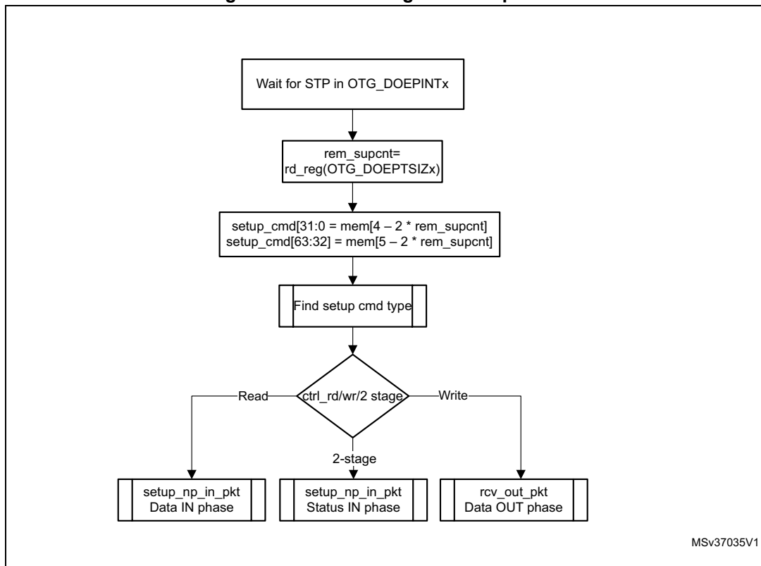
Figure 426. Processing a SETUP packet
