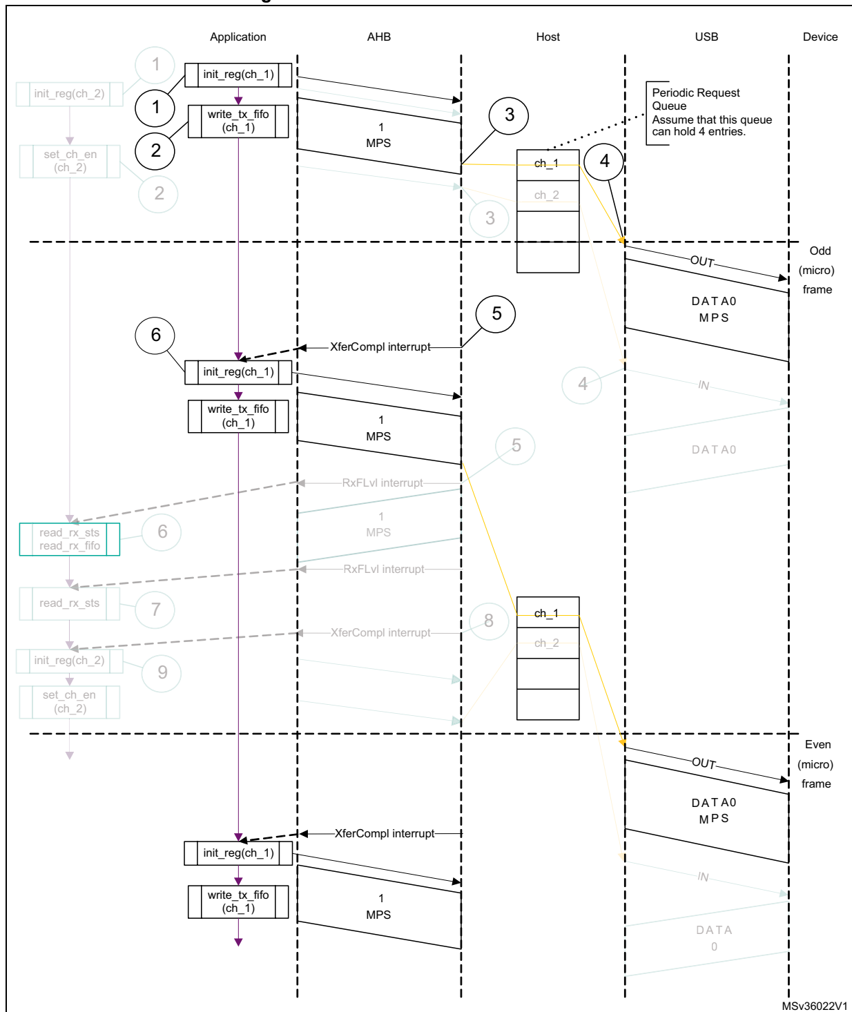
Figure 417. Isochronous OUT transactions
