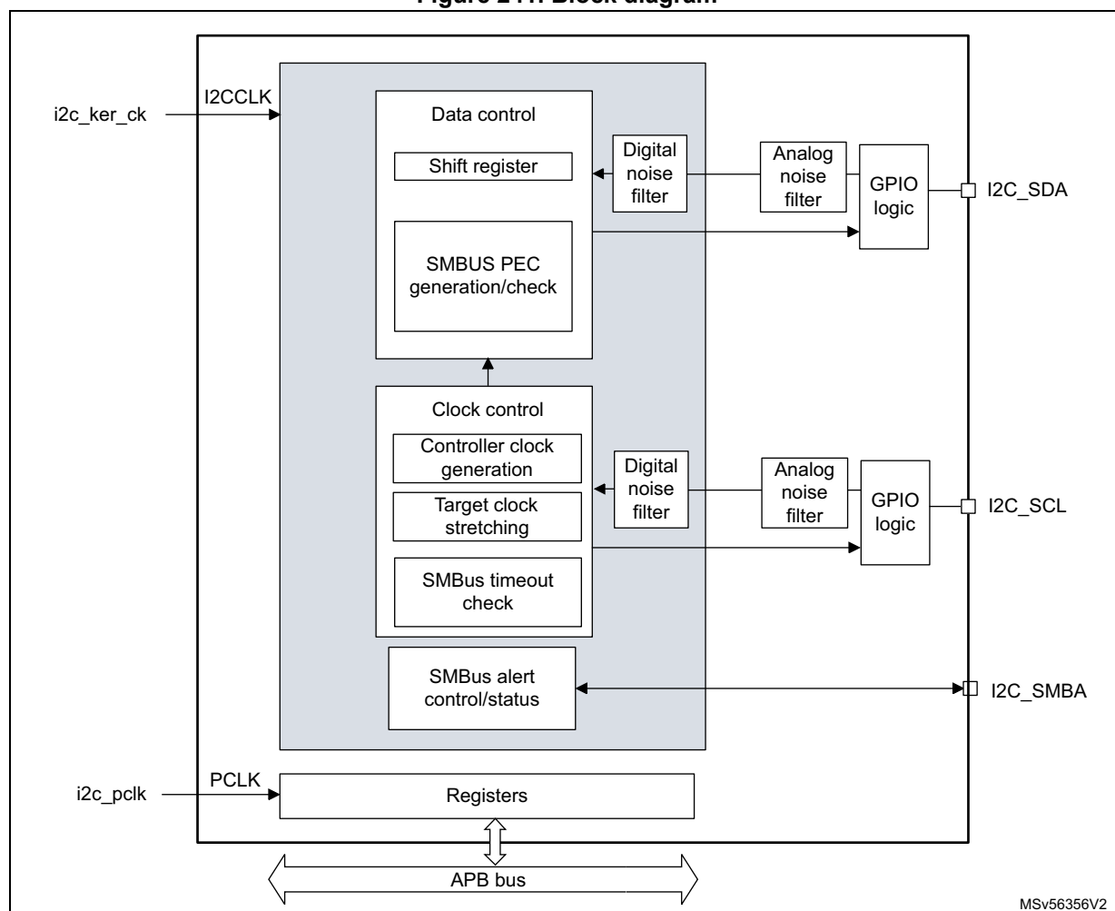
Figure 241. Block diagram
