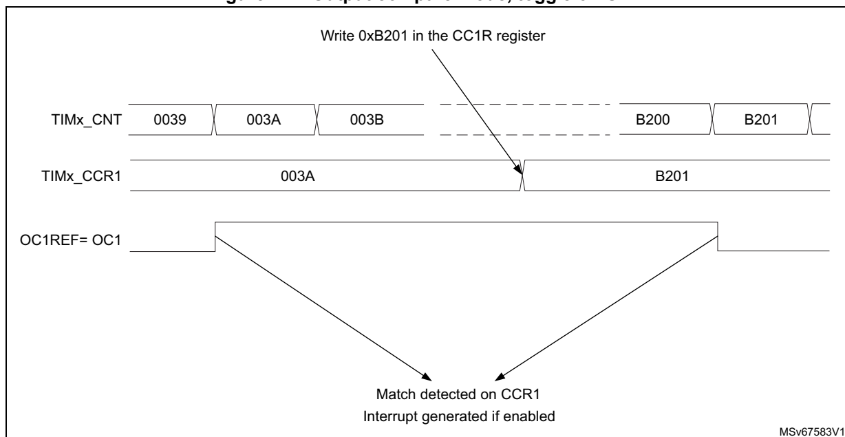
Figure 141. Output compare mode, toggle on OC1.
