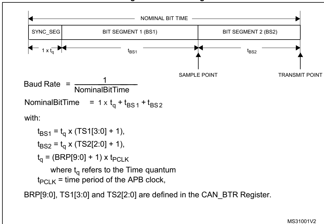
Figure 395. Bit timing
