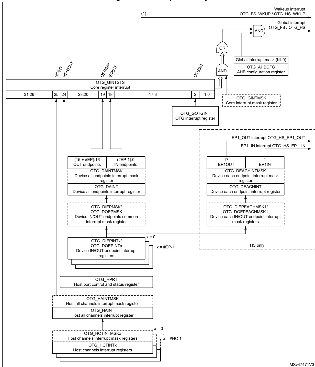
Figure 410. Interrupt hierarchy
