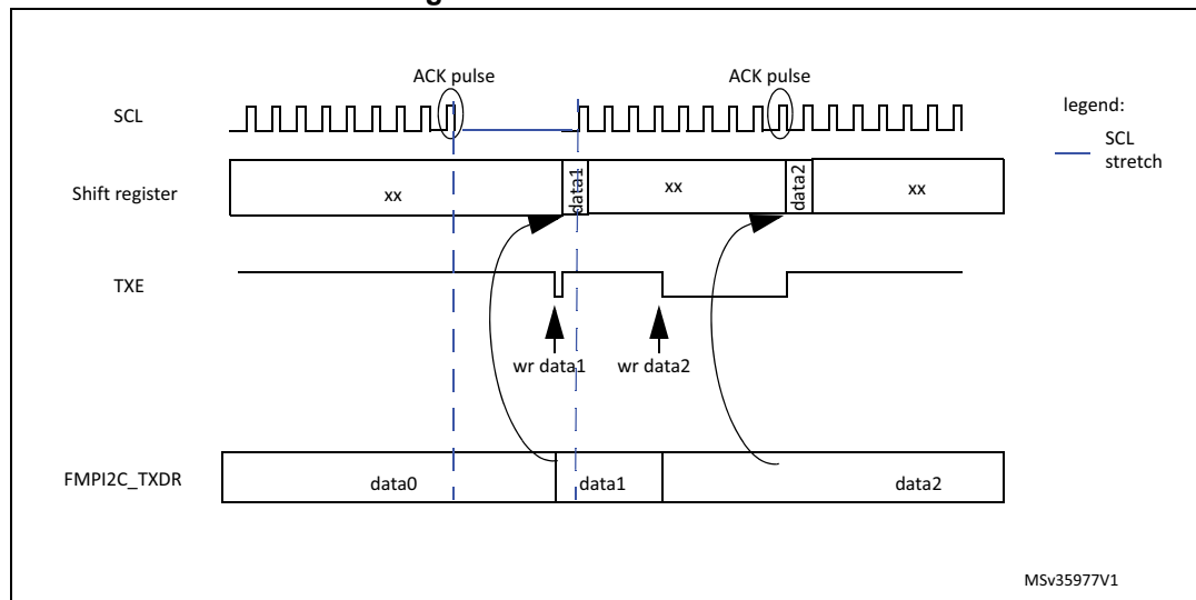
Figure 246. Data transmission
