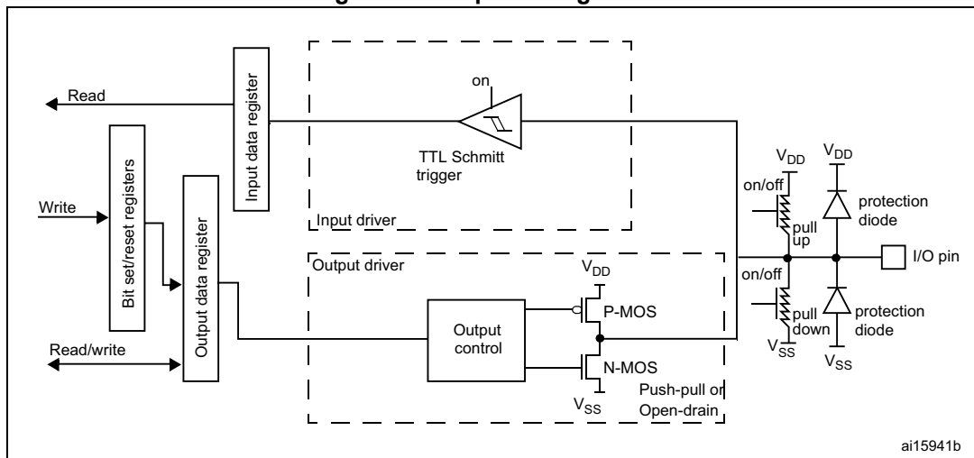
Figure 21. Output configuration
