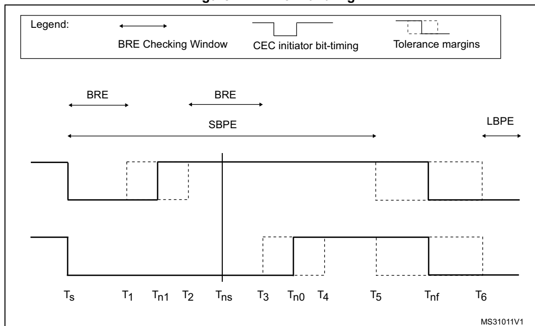
Figure 441. Error handling
