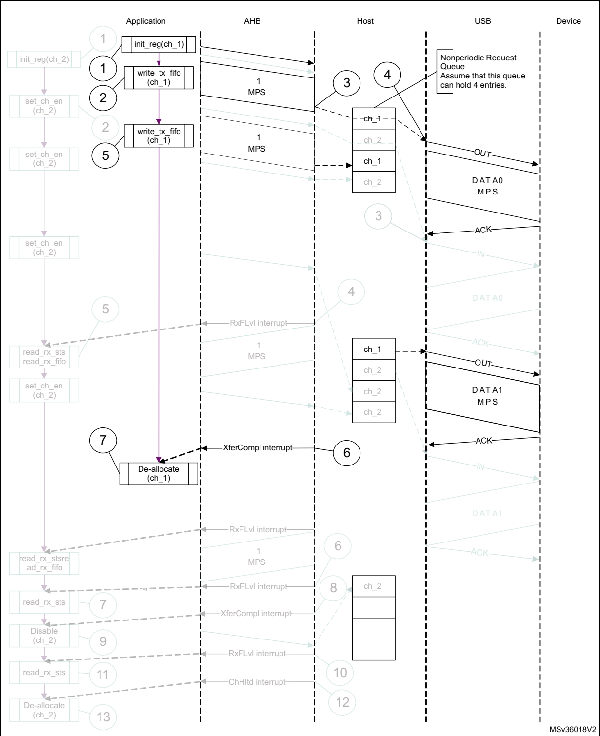
Figure 413. Normal bulk/control OUT/SETUP
