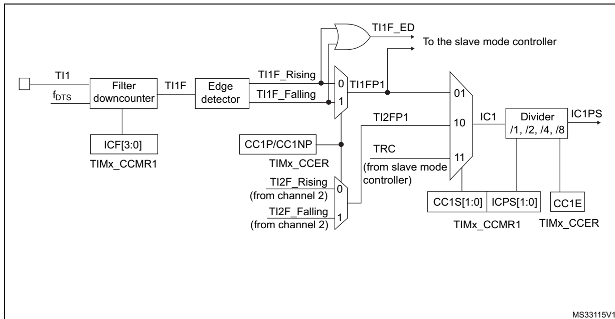
Figure 136. Capture/compare channel (example: channel 1 input stage)
