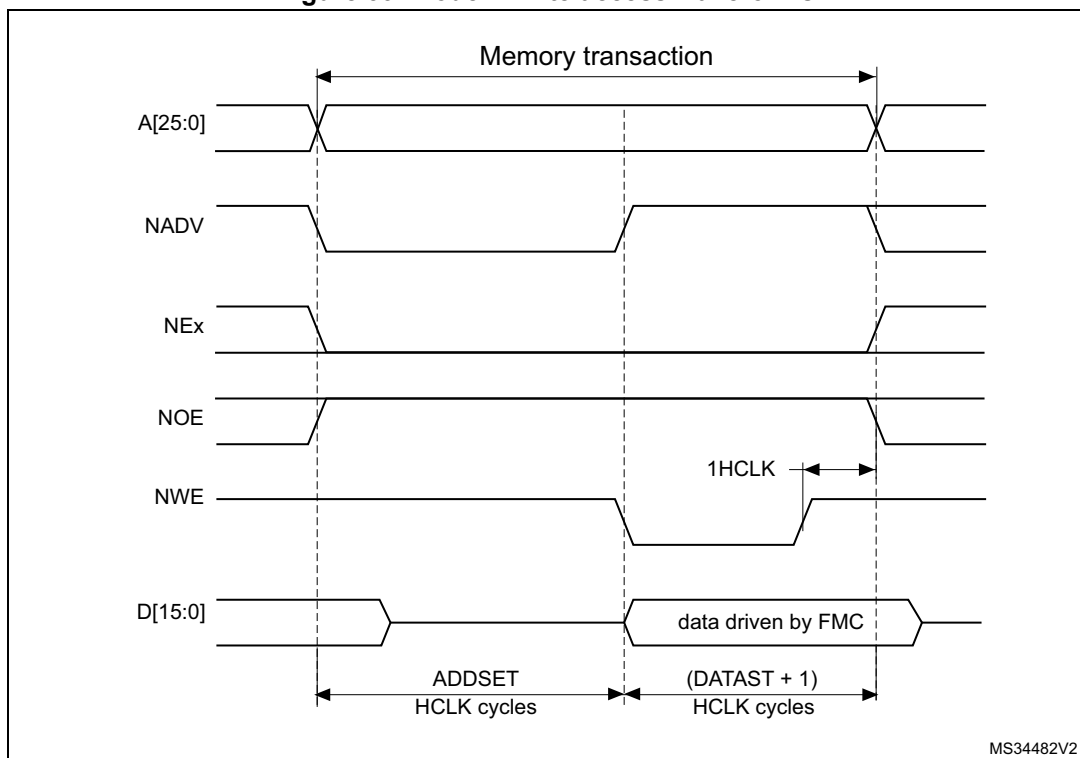
Figure 39. Mode 2 write access waveforms
