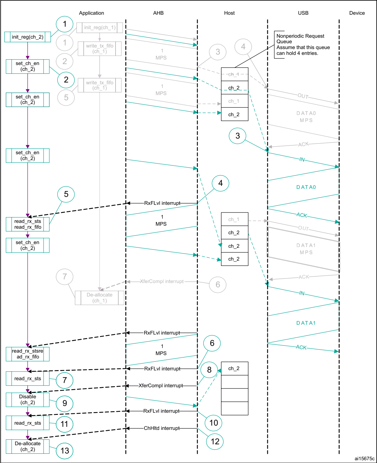
Figure 414. Bulk/control IN transactions
