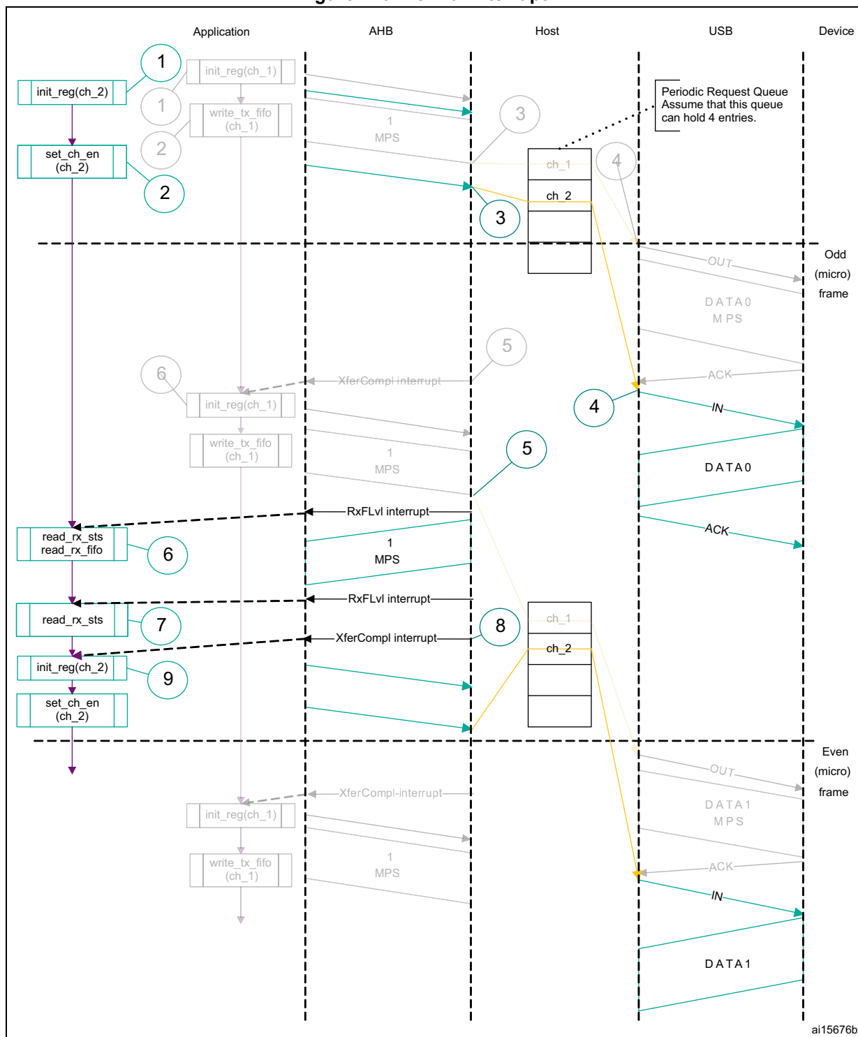
Figure 416. Normal interrupt IN
