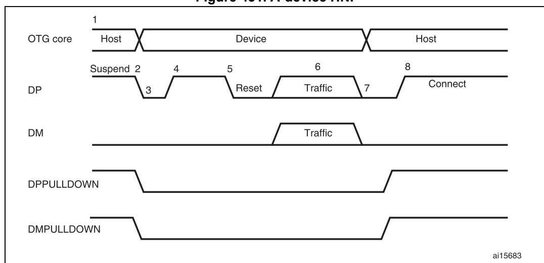
Figure 431. A-device HNP
