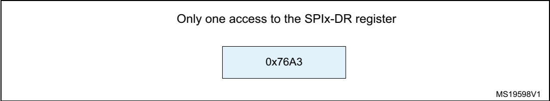
Figure 332. Example of 16-bit data frame extended to 32-bit channel frame
