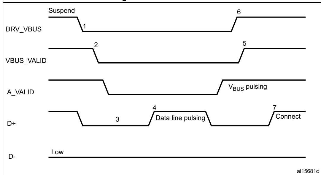
Figure 429. A-device SRP
