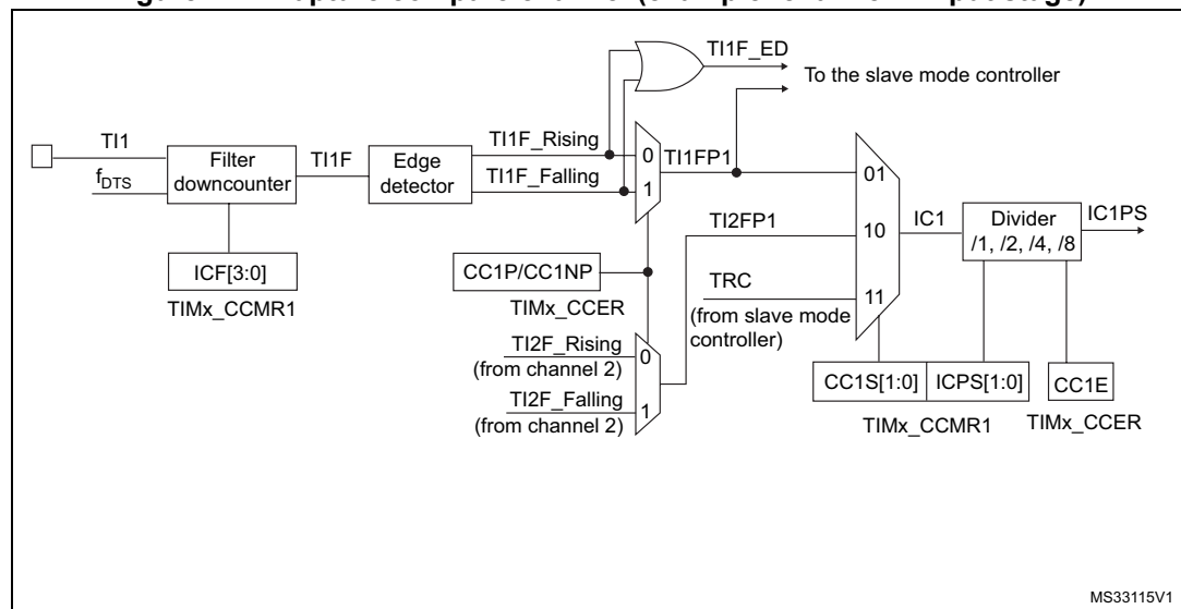
Figure 217. Capture/compare channel (example: channel 1 input stage)
