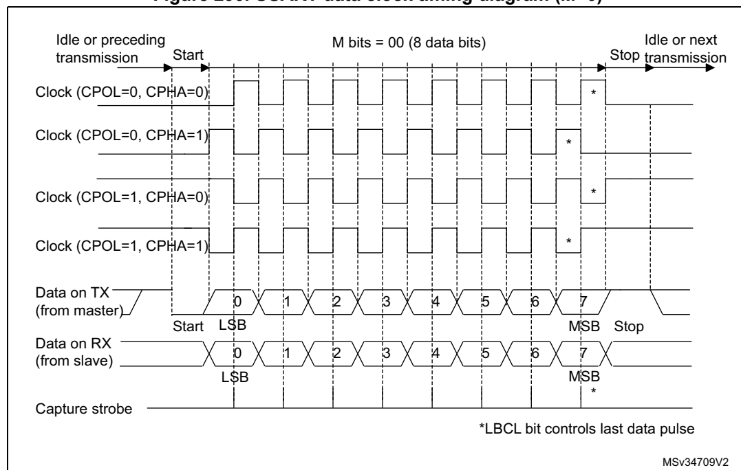
Figure 290. USART data clock timing diagram (M=0)
