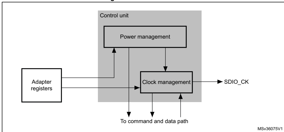
Figure 376. Control unit
