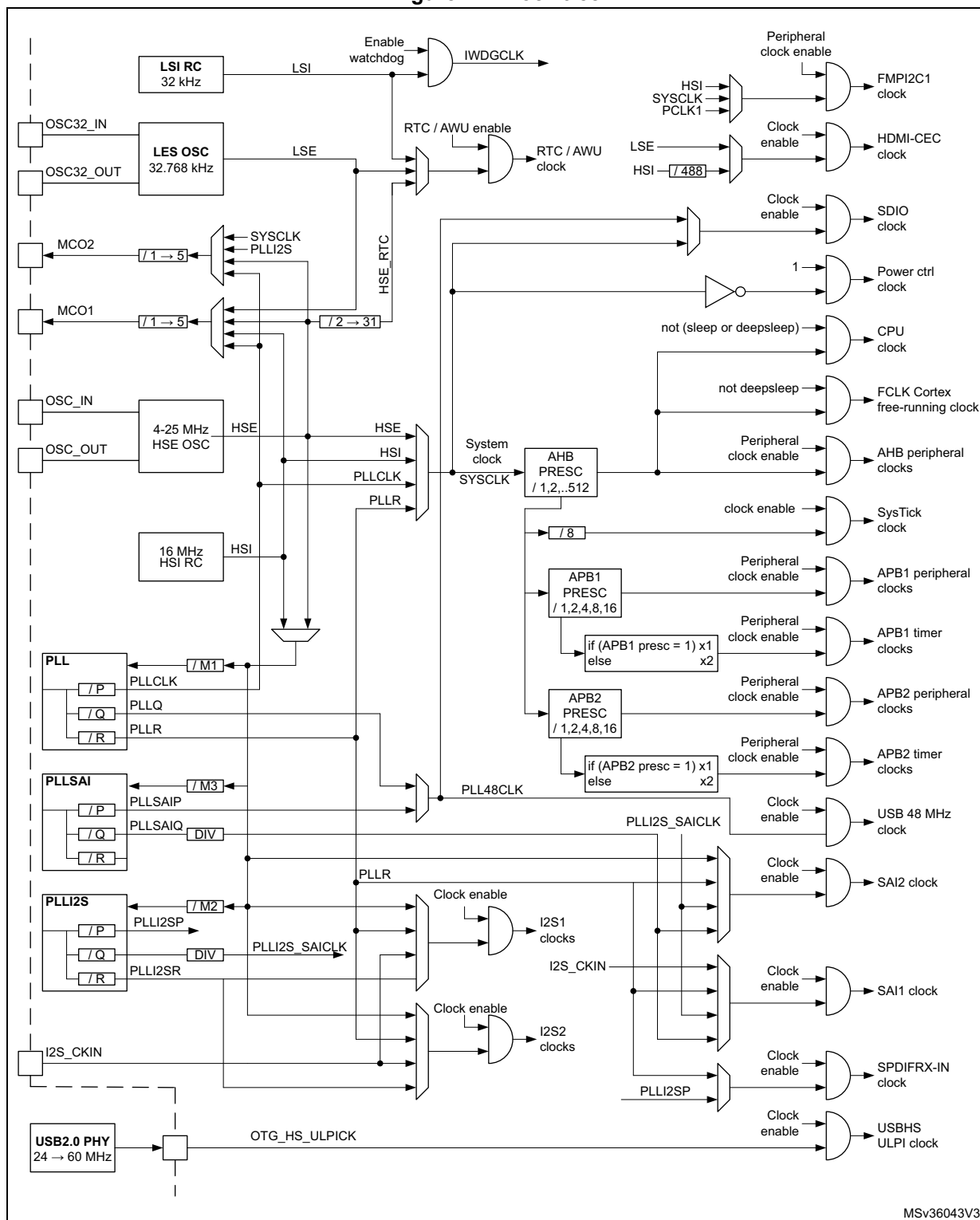
Figure 14. Clock tree
