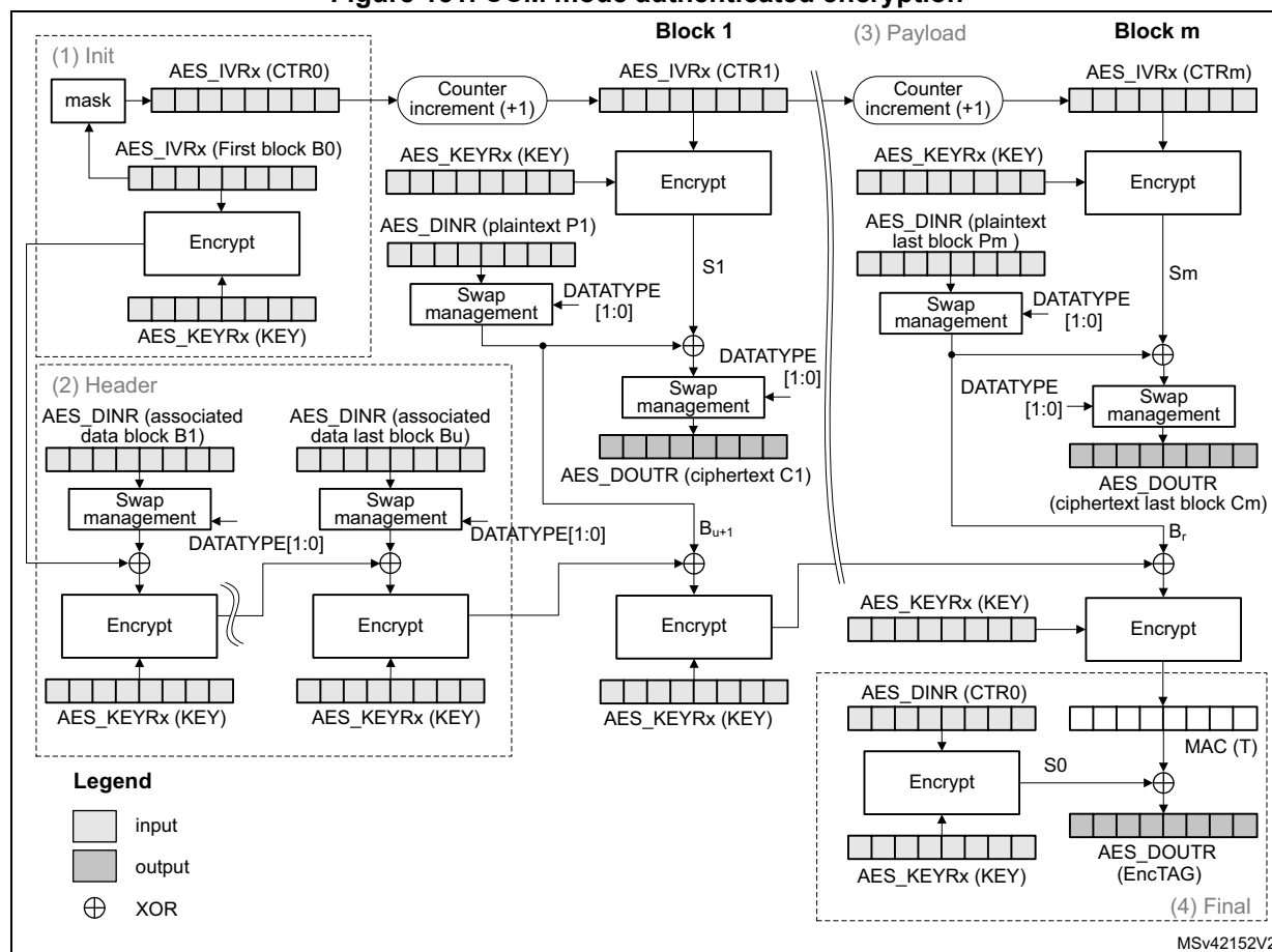
Figure 151. CCM mode authenticated encryption
