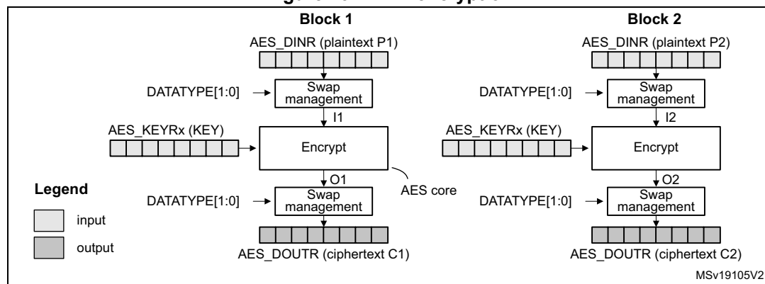
Figure 137. ECB encryption
