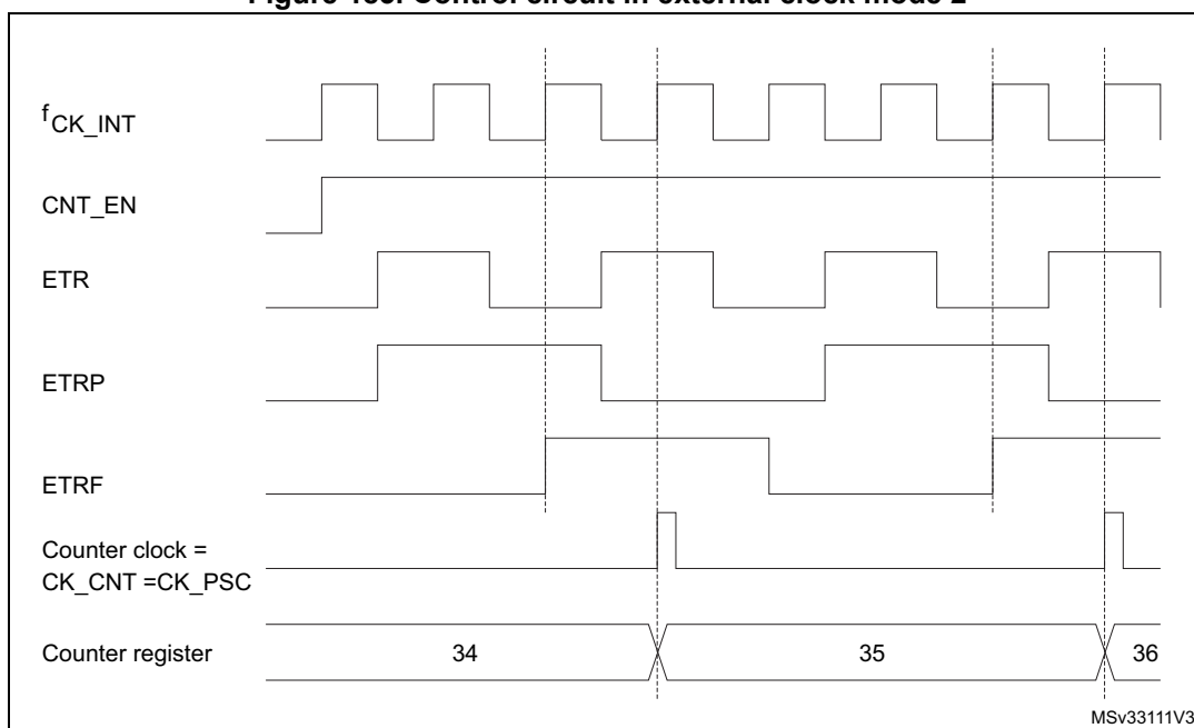
Figure 183. Control circuit in external clock mode 2
