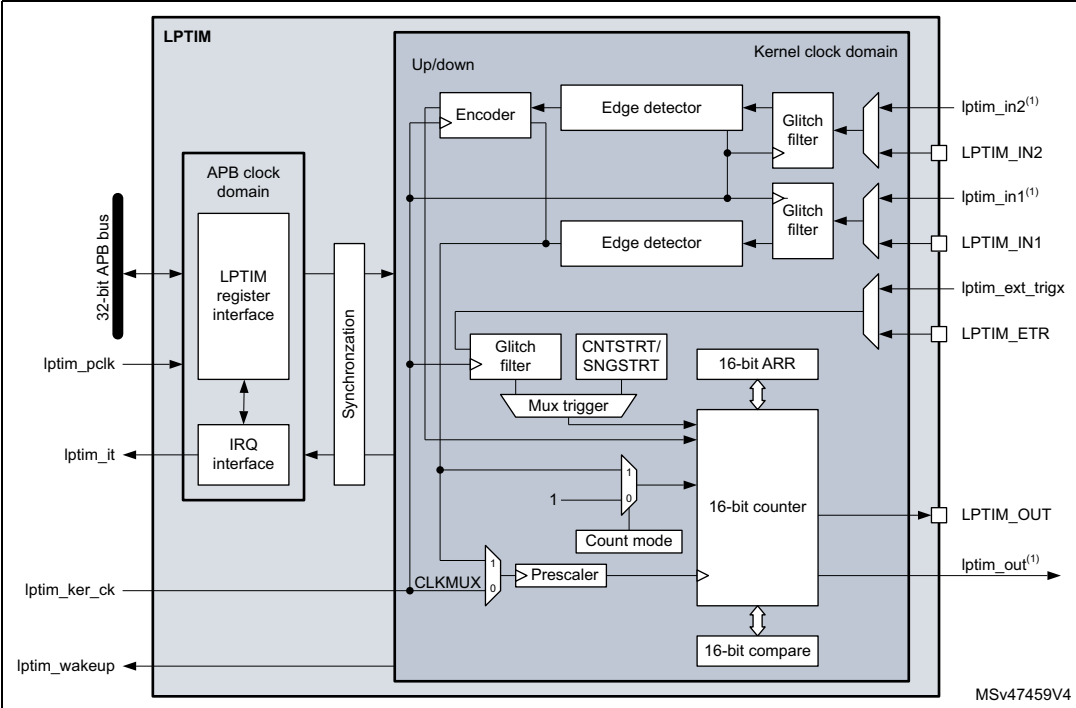
Figure 290. Low-power timer block diagram
