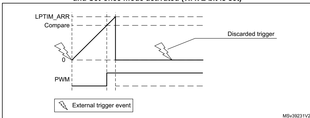
Figure 293. LPTIM output waveform, Single counting mode configuration and Set-once mode activated (WAVE bit is set)
