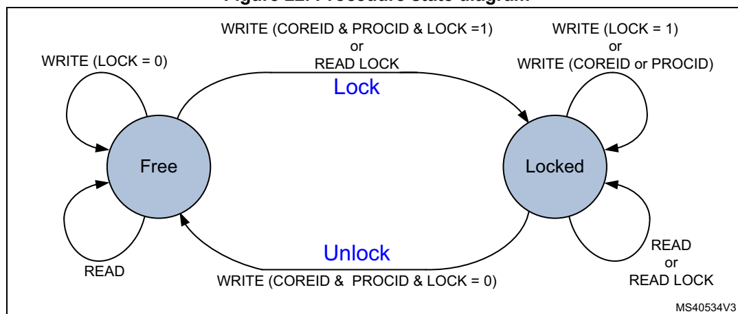
Figure 22. Procedure state diagram
