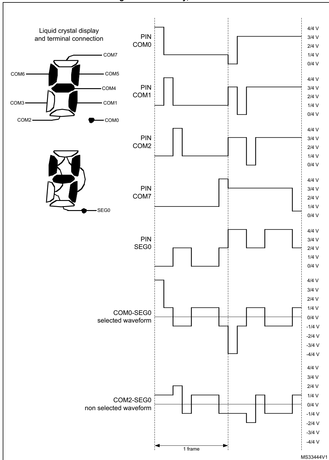
Figure 115. 1/8 duty, 1/4 bias
