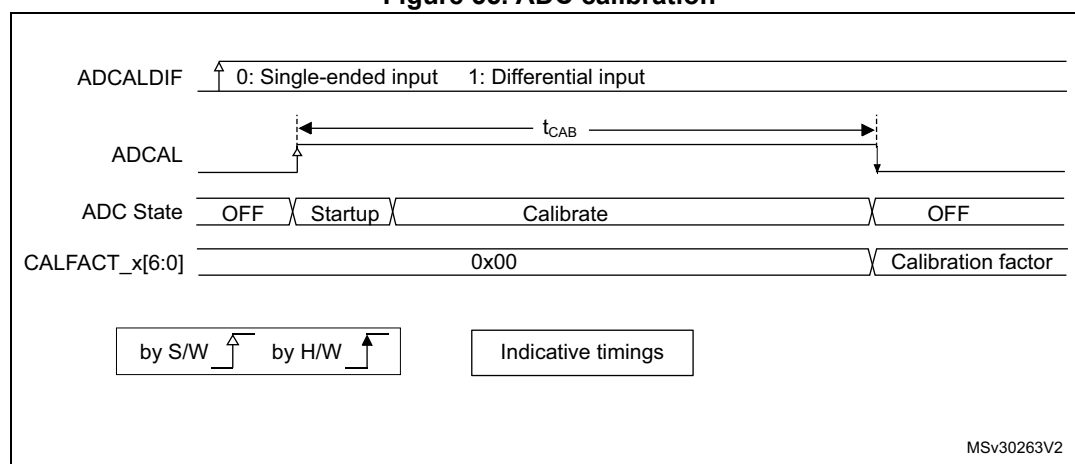
Figure 55. ADC calibration
