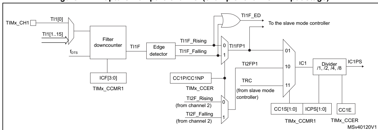
Figure 241. Capture/Compare channel (example: channel 1 input stage)
