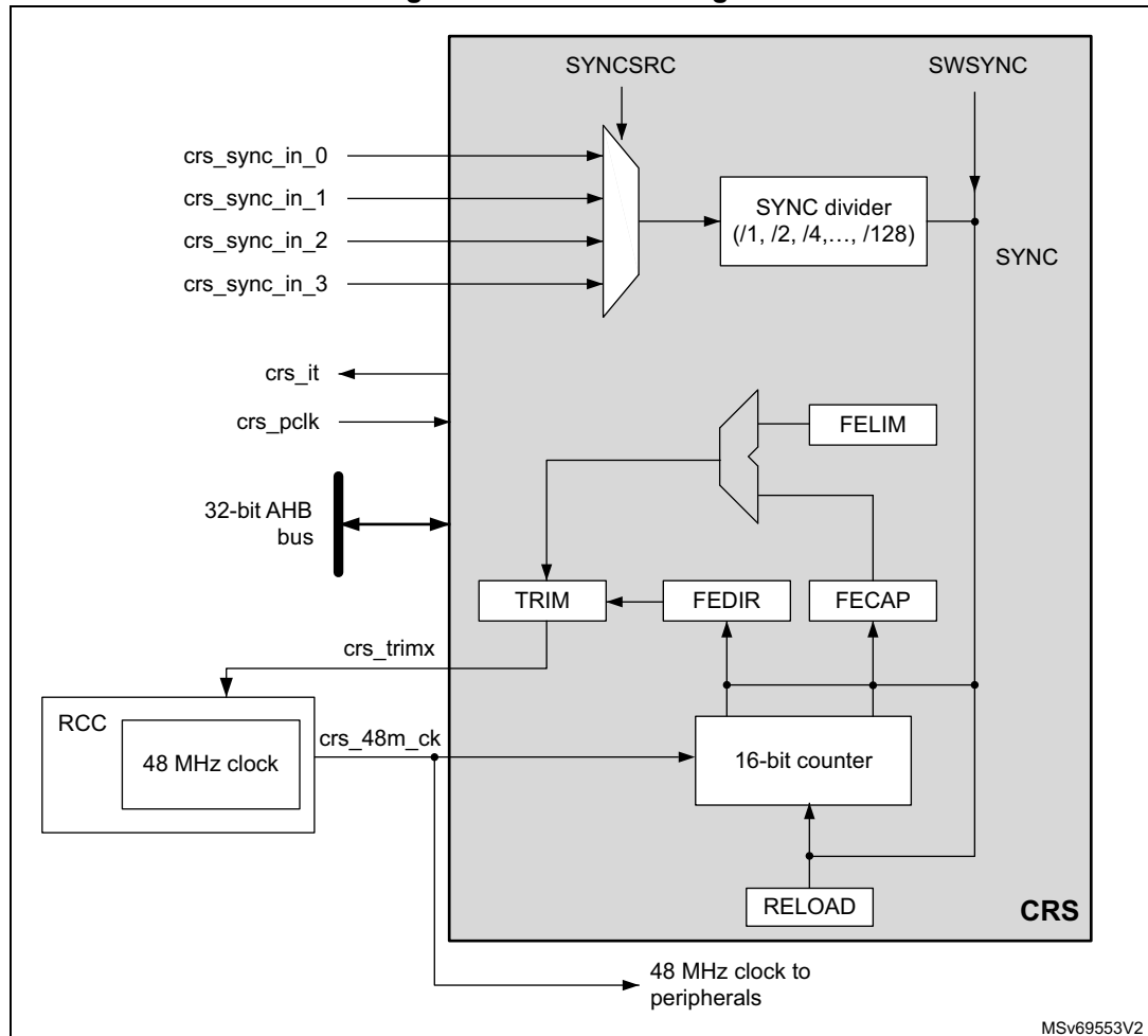
Figure 19. CRS block diagram
