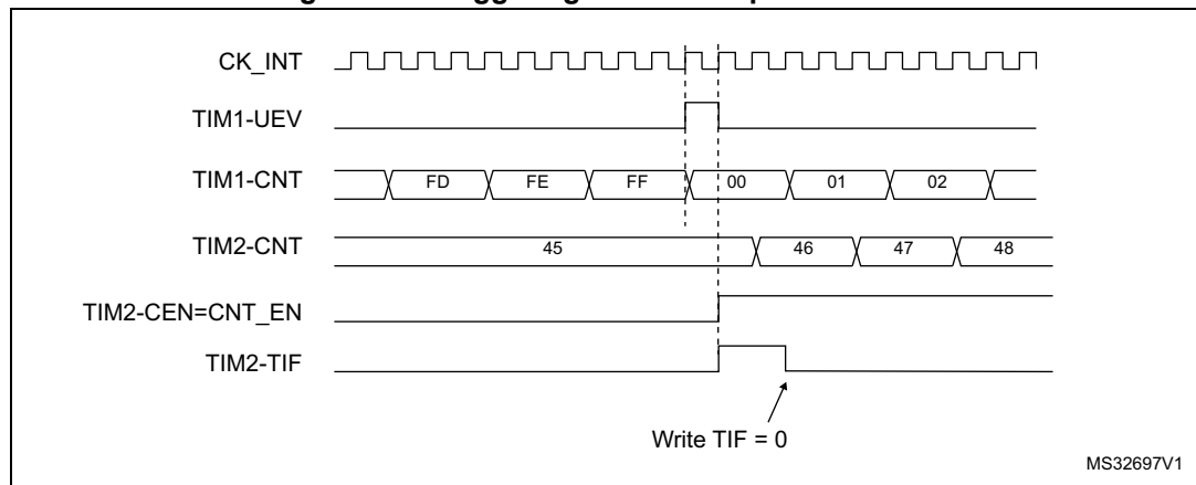
Figure 263. Triggering TIM2 with update of TIM1
