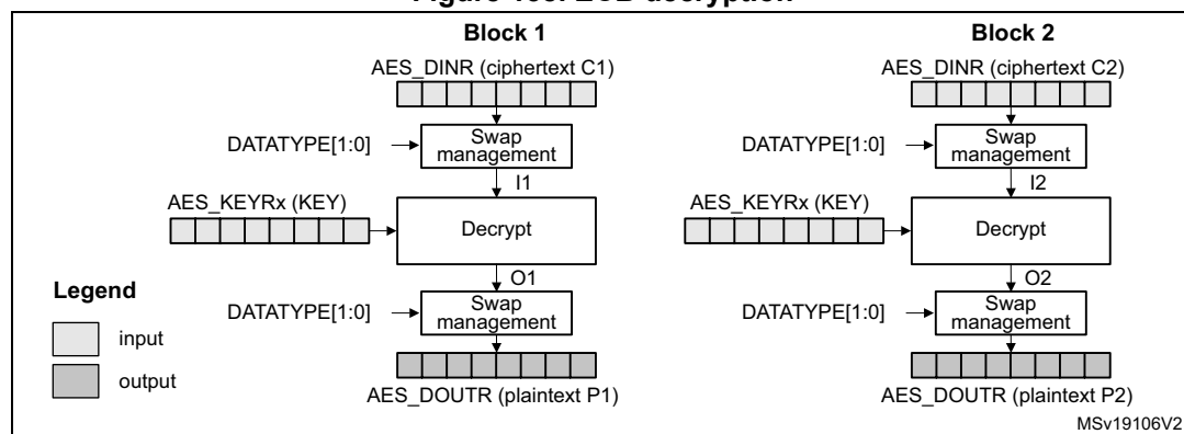
Figure 138. ECB decryption
