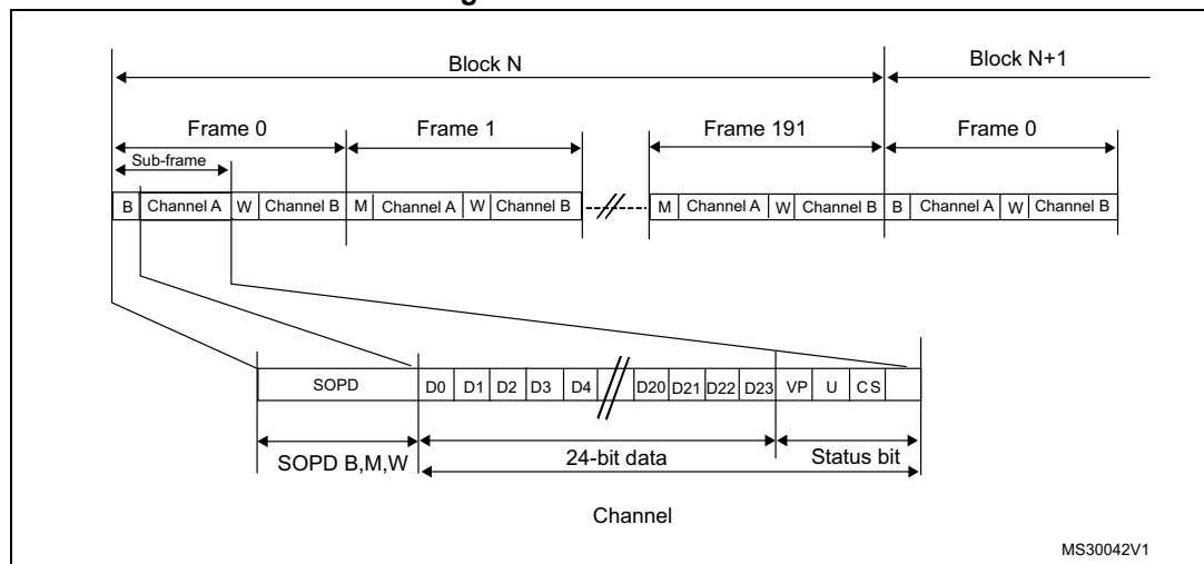
Figure 403. SPDIF format
