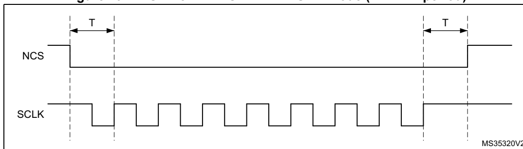
Figure 49. NCS when CKMODE = 1 in SDR mode ( T = \text{CLK period} )
