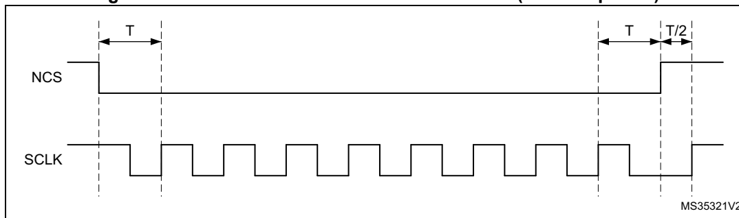
Figure 50. NCS when CKMODE = 1 in DDR mode ( T = \text{CLK period} )
