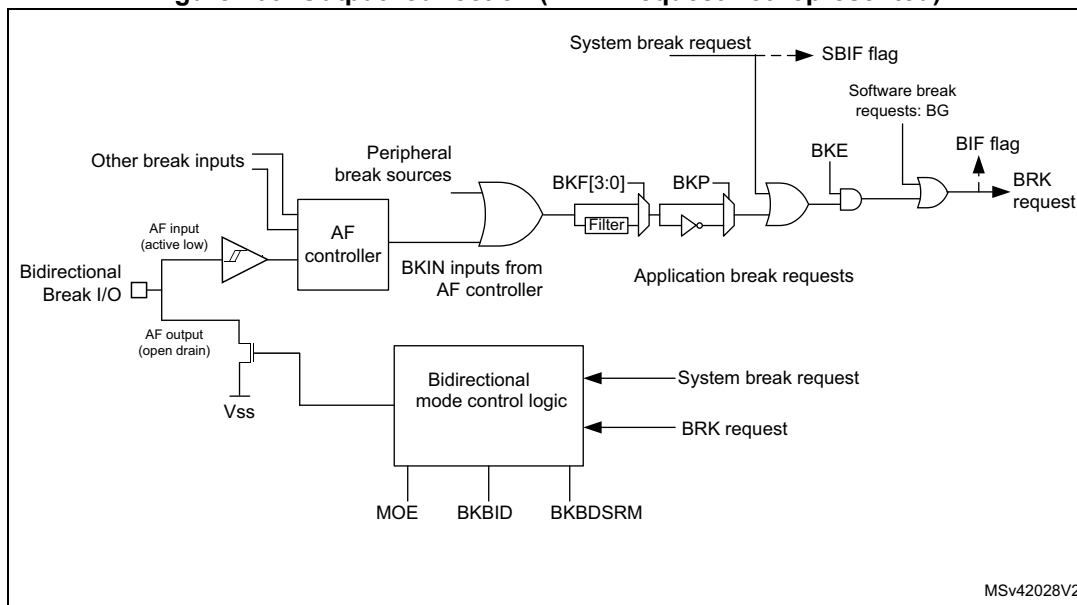
Figure 203. Output redirection (BRK2 request not represented)
