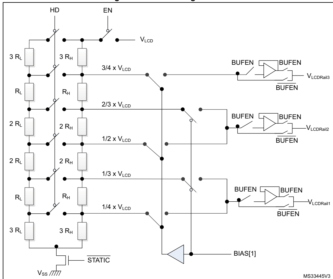
Figure 116. LCD voltage control
