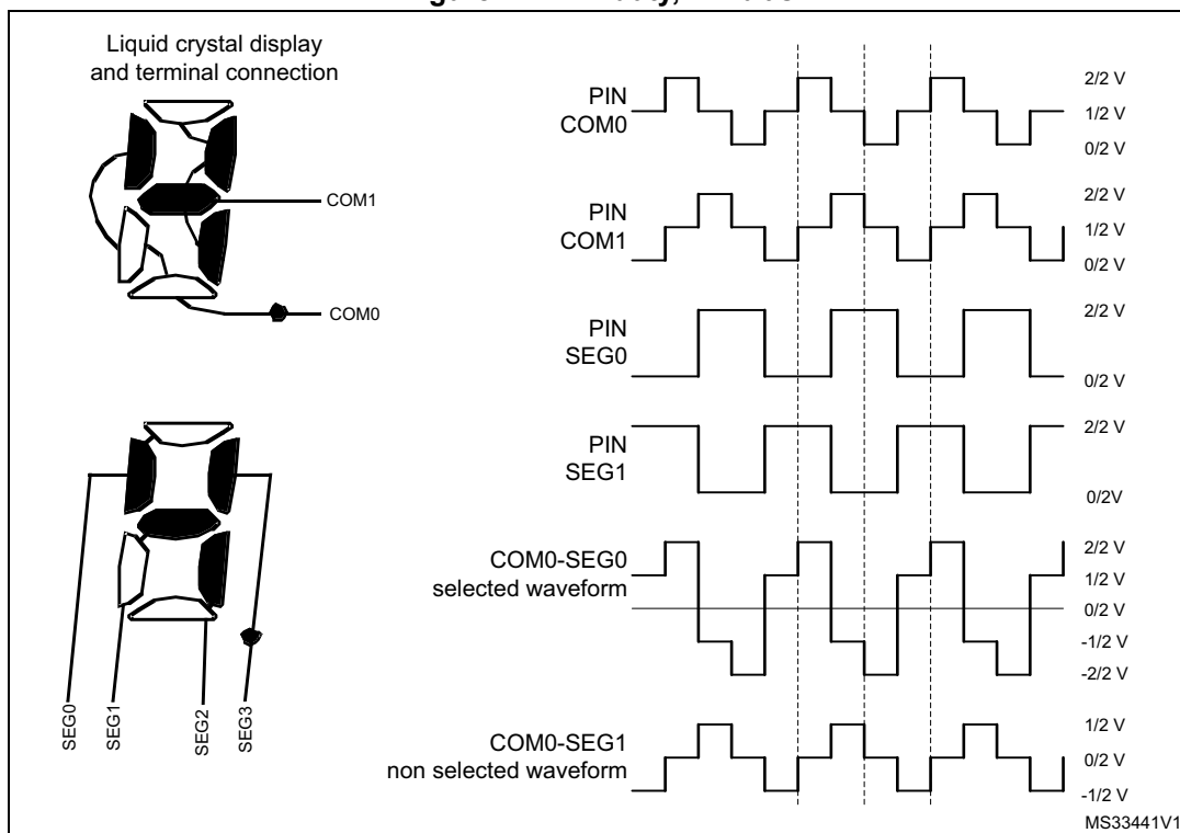
Figure 112. 1/2 duty, 1/2 bias
