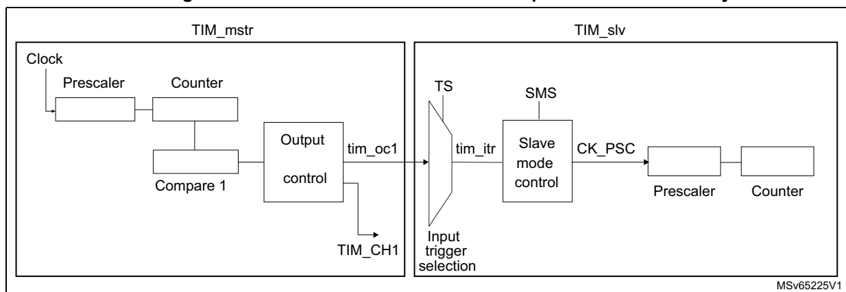
Figure 260. Master/slave connection example with 1 channel only timers
