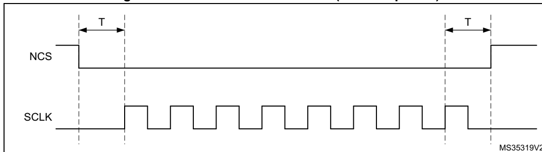
Figure 48. NCS when CKMODE = 0 ( T = \text{CLK period} )
