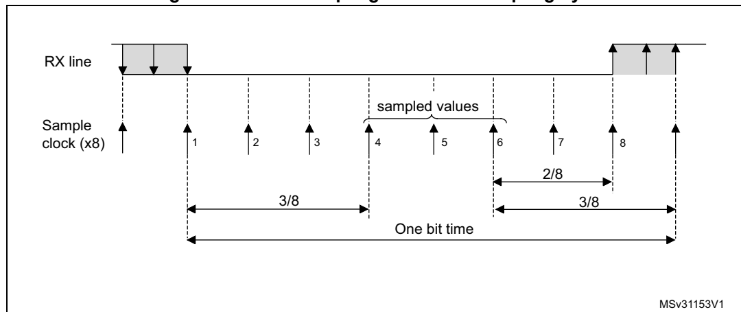
Figure 339. Data sampling when oversampling by 8
