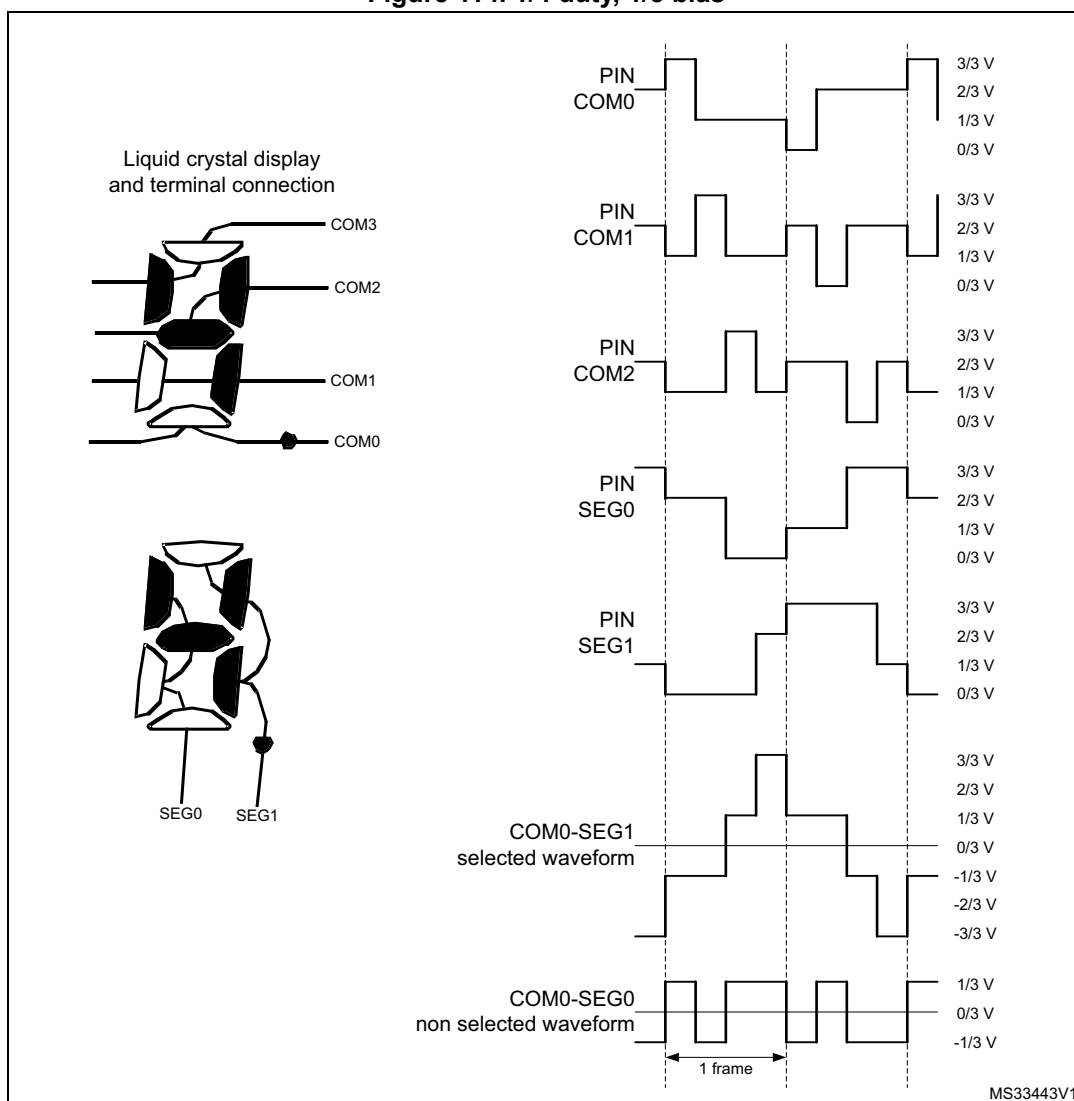
Figure 114. 1/4 duty, 1/3 bias
