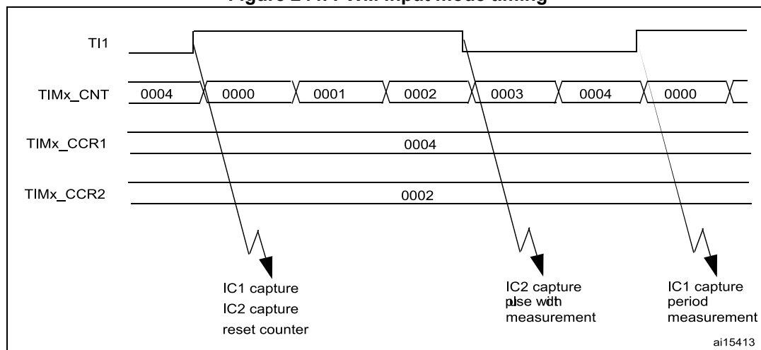
Figure 244. PWM input mode timing
