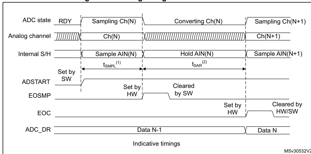
Figure 59. Analog-to-digital conversion time
