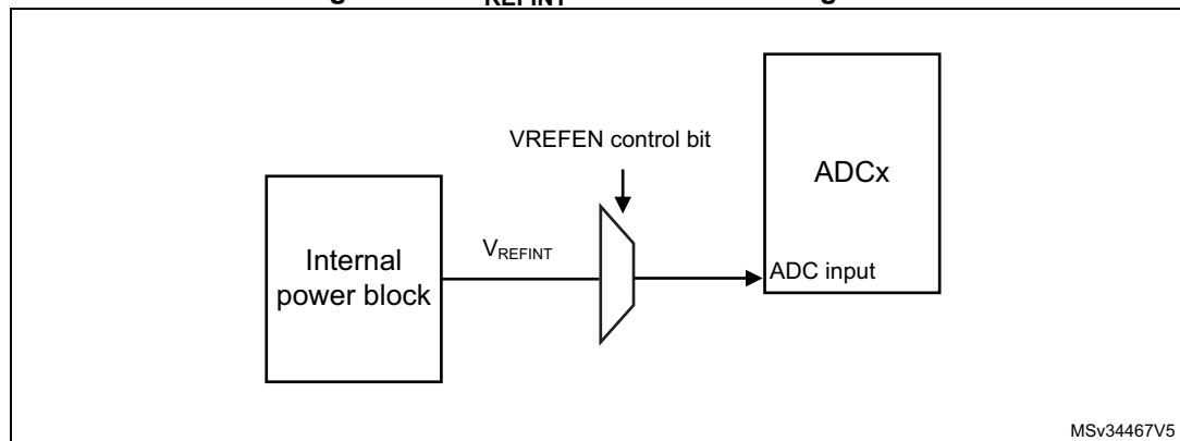
Figure 103. V_{REFINT} channel block diagram
