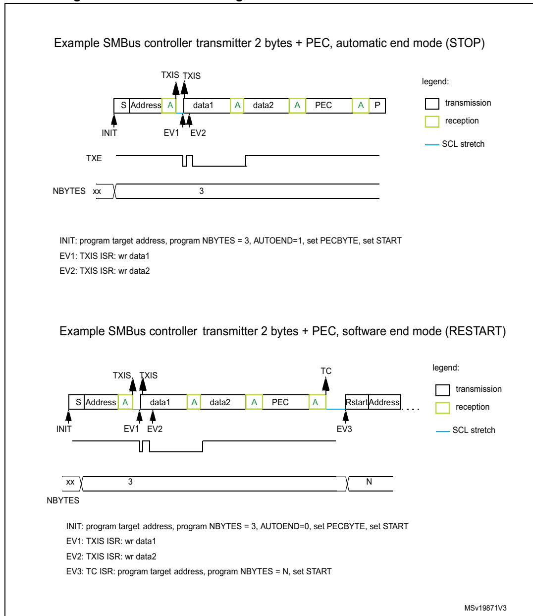
Figure 330. Bus transfer diagrams for SMBus controller transmitter
