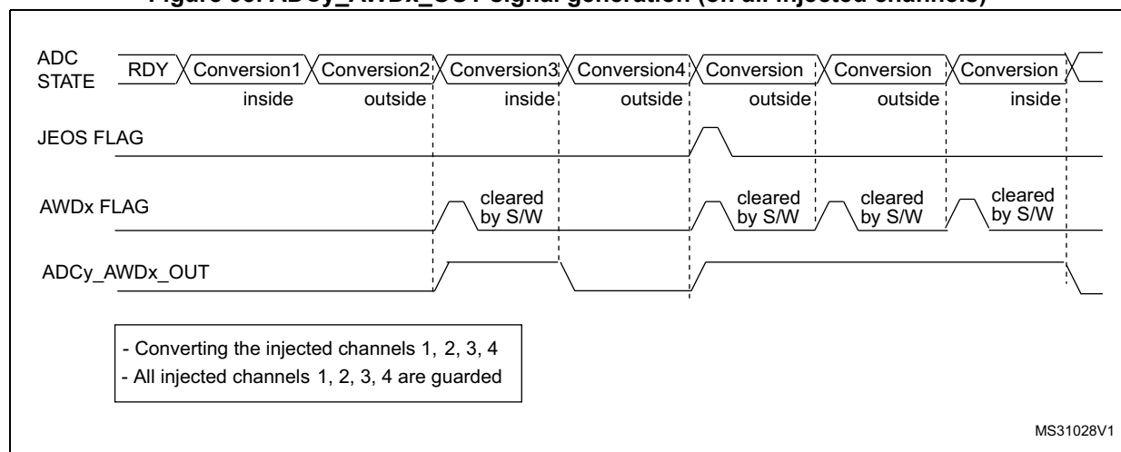
Figure 93. ADCy_AWDx_OUT signal generation (on all injected channels)
