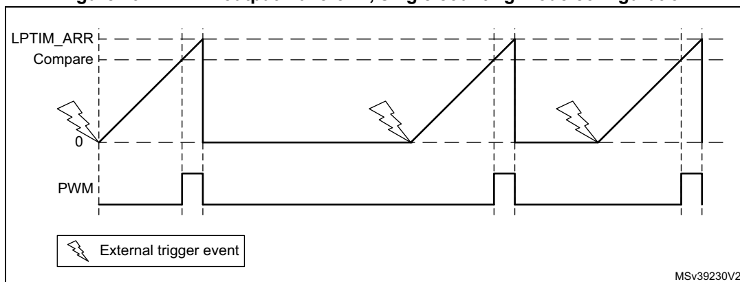
Figure 292. LPTIM output waveform, single counting mode configuration
