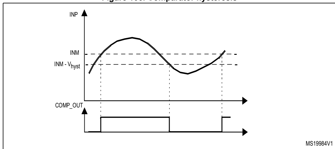
Figure 106. Comparator hysteresis
