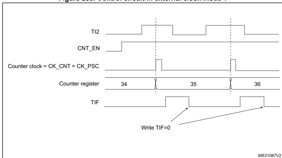
Figure 238. Control circuit in external clock mode 1
