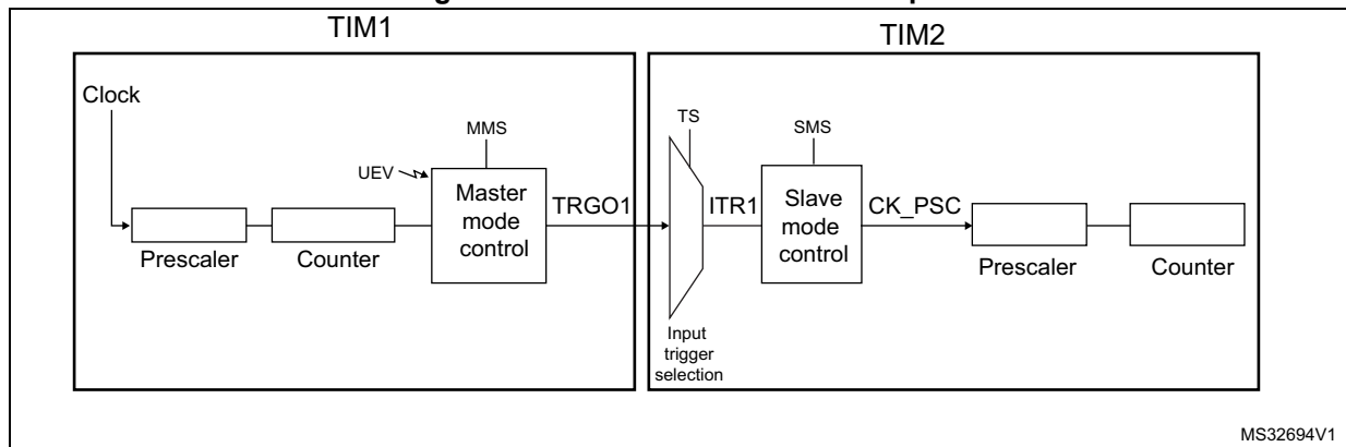
Figure 259. Master/Slave timer example
