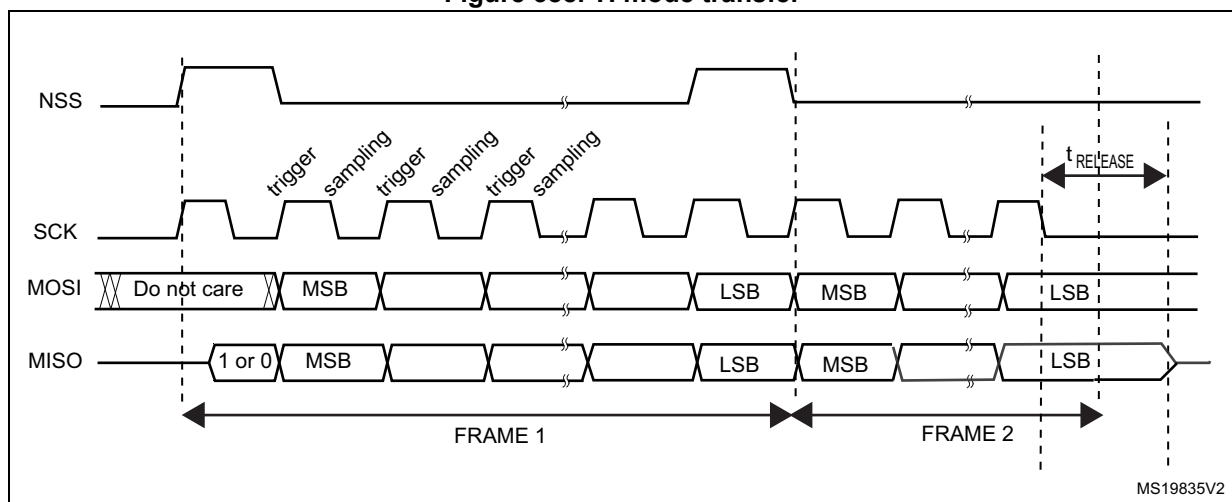
Figure 388. TI mode transfer
