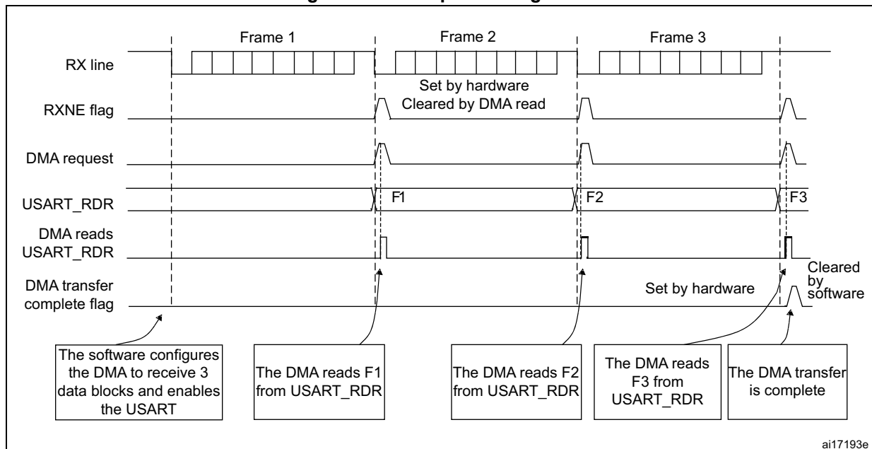
Figure 353. Reception using DMA
