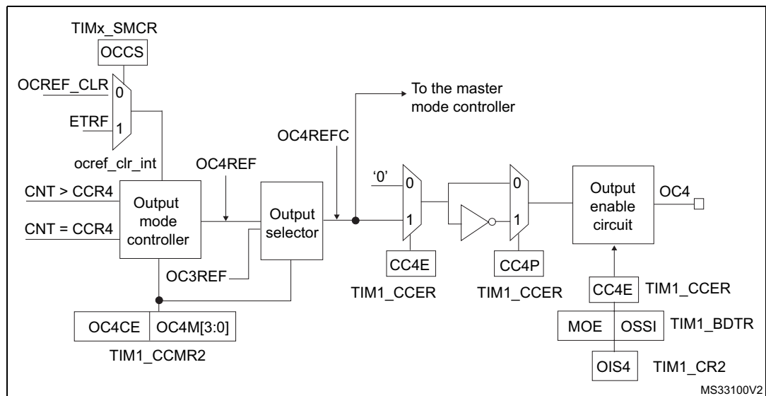
Figure 187. Output stage of capture/compare channel (channel 4)
