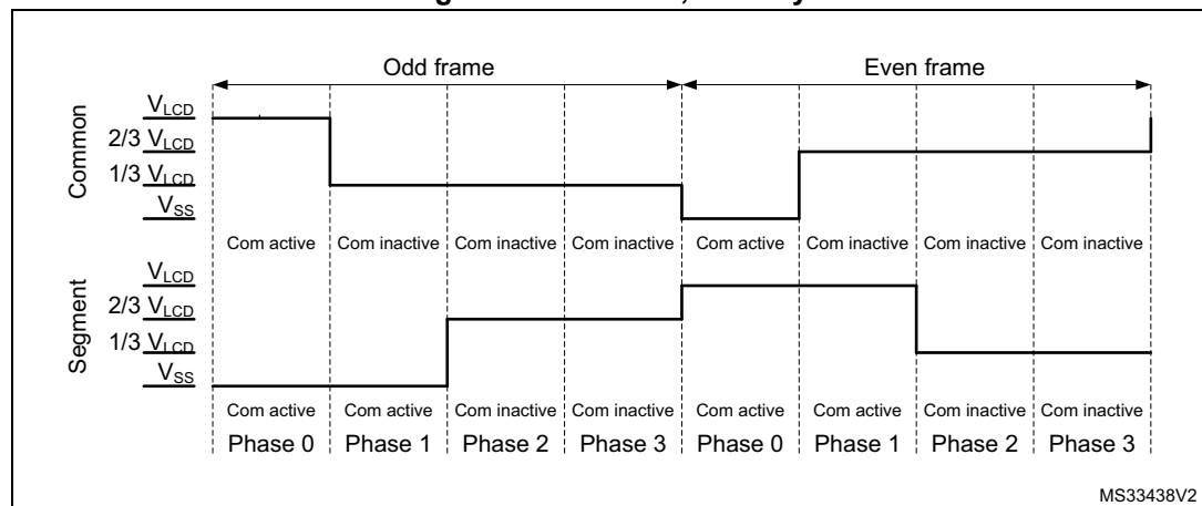
Figure 109. 1/3 bias, 1/4 duty
