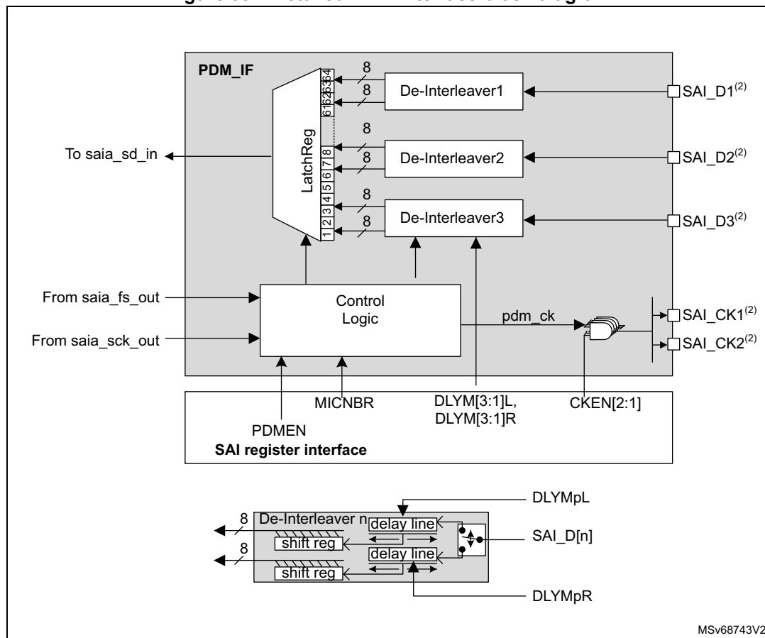
Figure 397. Detailed PDM interface block diagram
