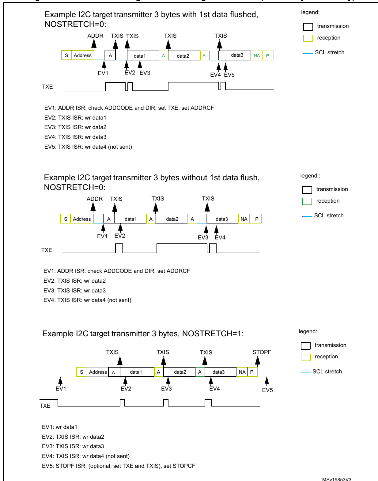
Figure 311. Transfer bus diagrams for I2C target transmitter (mandatory events only)
