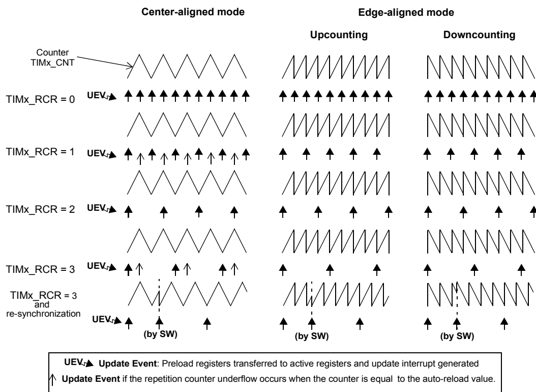
Figure 48. Update rate examples depending on mode and TIMx_RCR register settings
