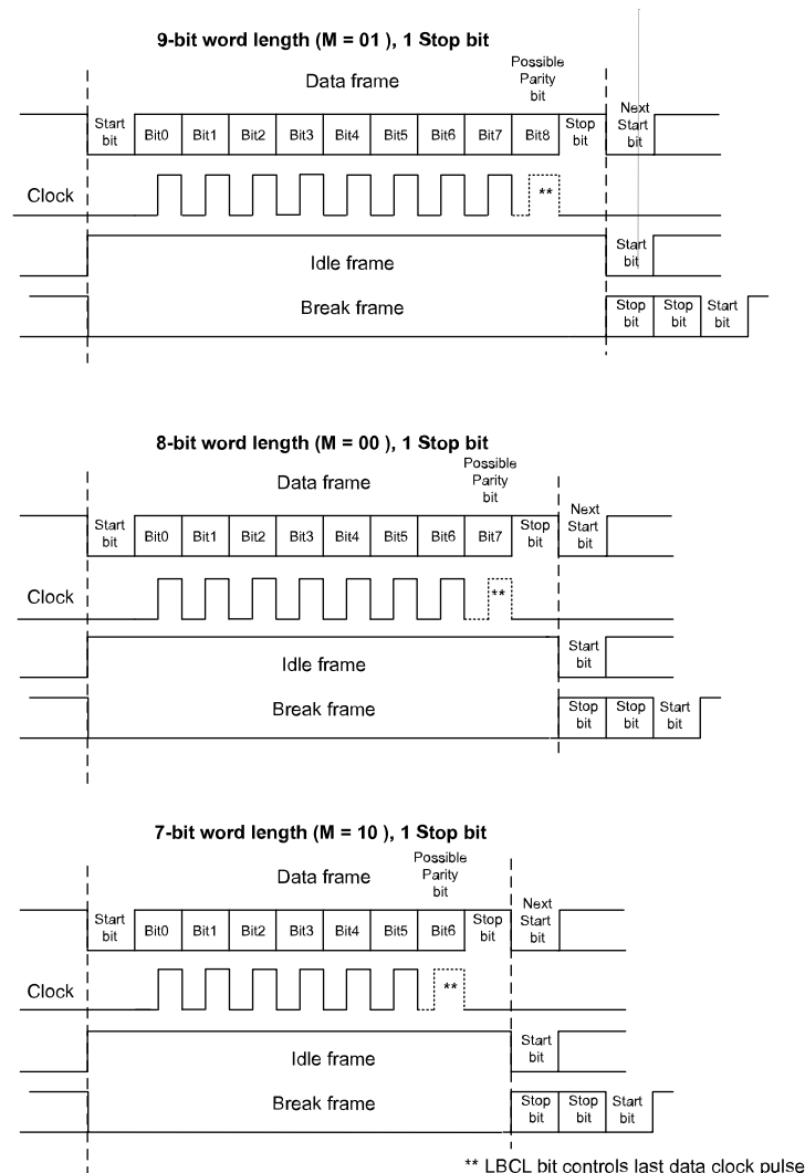
Figure 114. Word length programming
