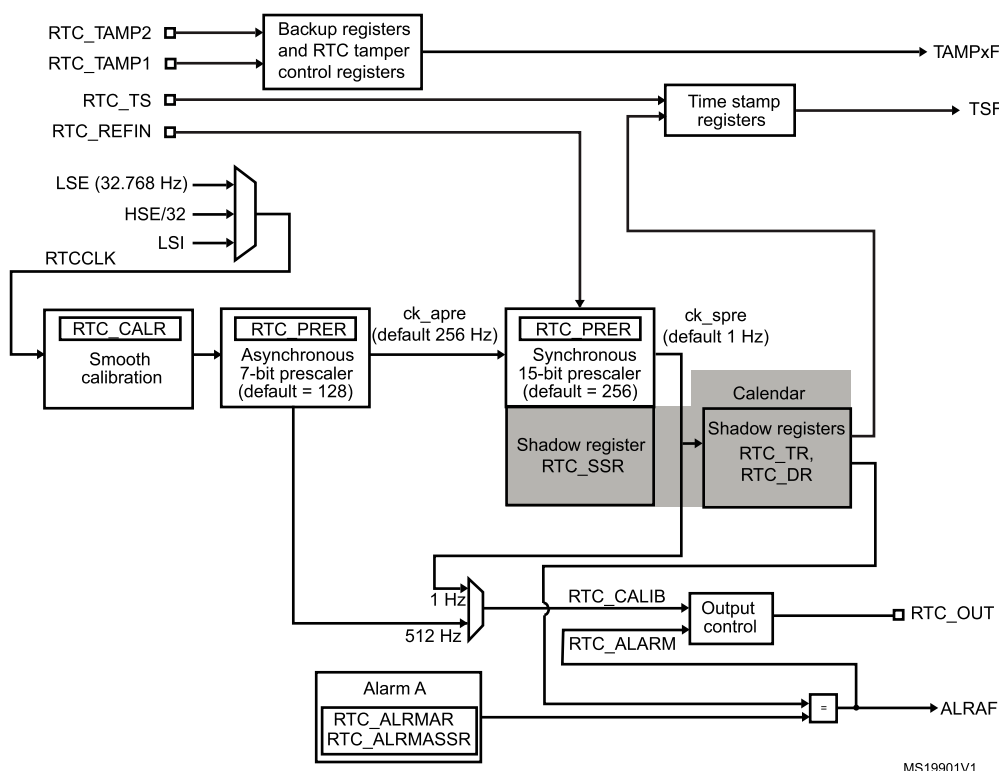
Figure 81. RTC block diagram
