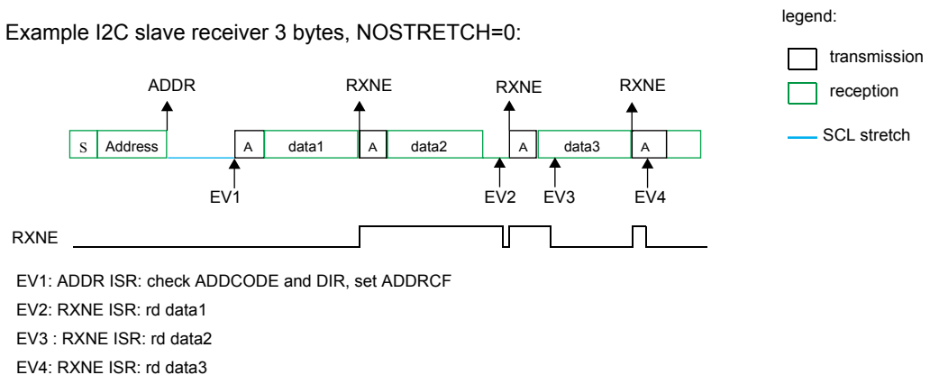
Figure 95. Transfer bus diagrams for I2C slave receiver
