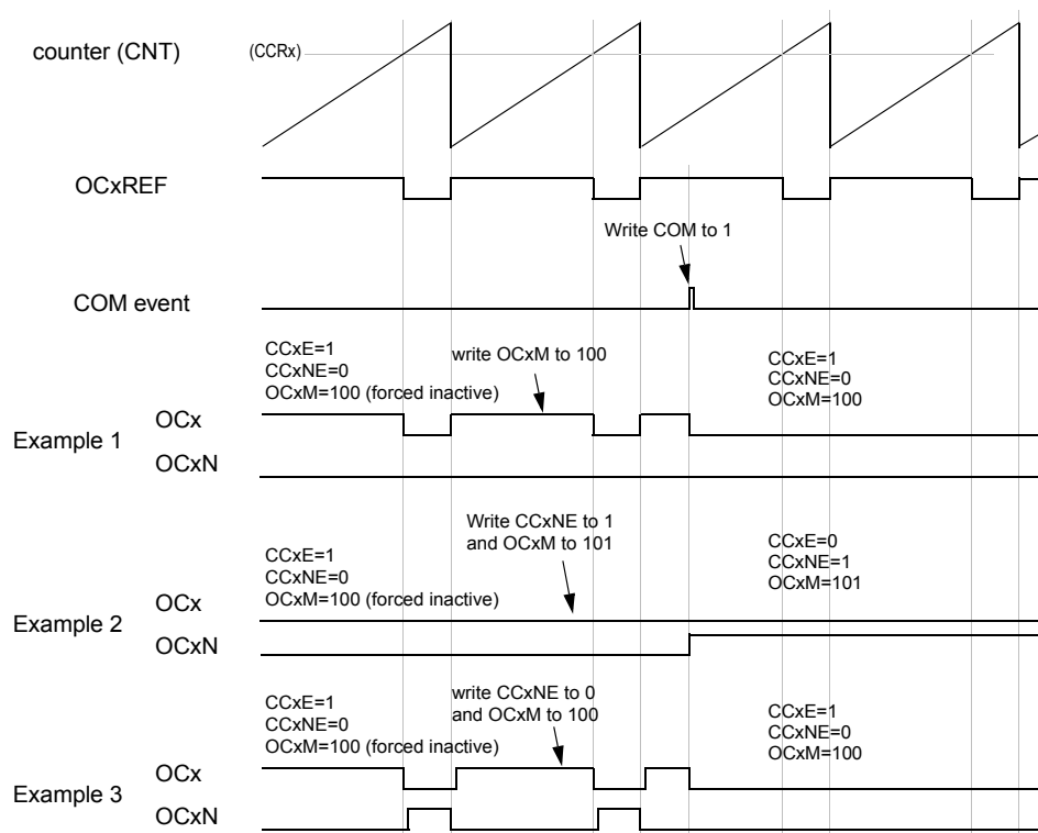
Figure 75. 6-step generation, COM example (OSSR=1)
