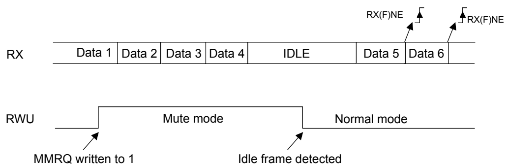
Figure 121. Mute mode using Idle line detection
