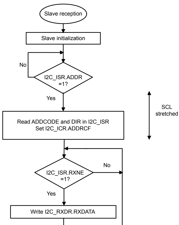
Figure 93. Transfer sequence flowchart for slave receiver with NOSTRETCH=0
