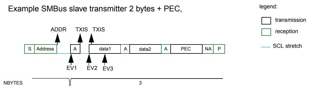
Figure 107. Transfer bus diagrams for SMBus slave transmitter (SBC=1)
