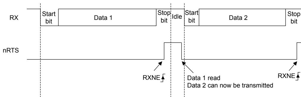
Figure 136. RS232 RTS flow control
