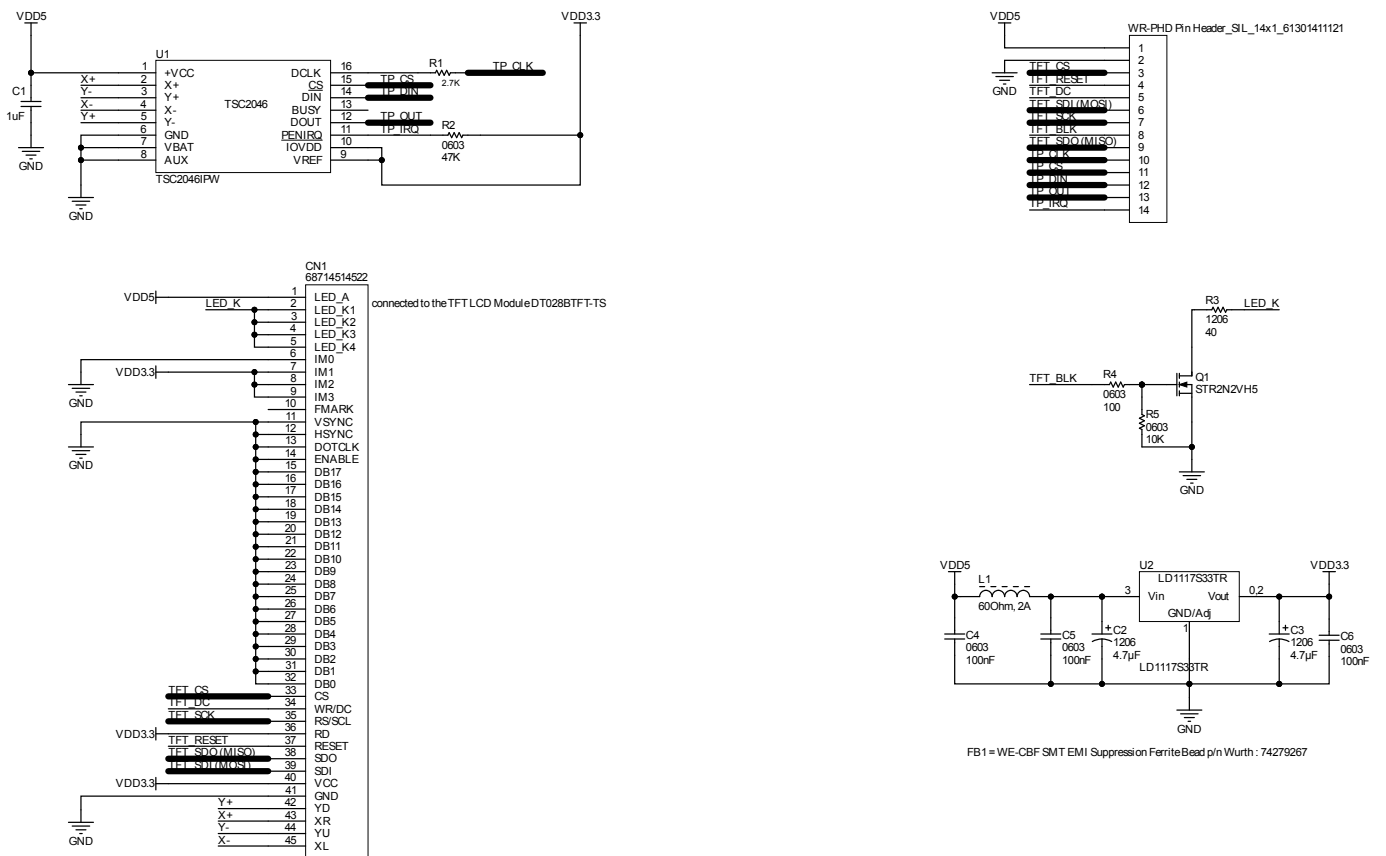
Figure 1. AEK-LCD-DT028V1 circuit schematic
