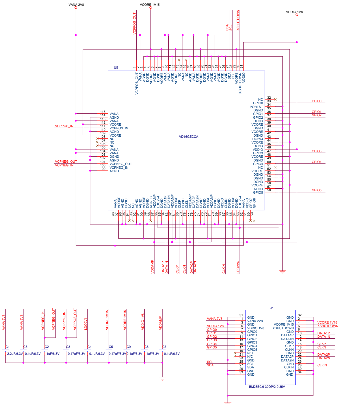
Figure 1. Circuit schematic
