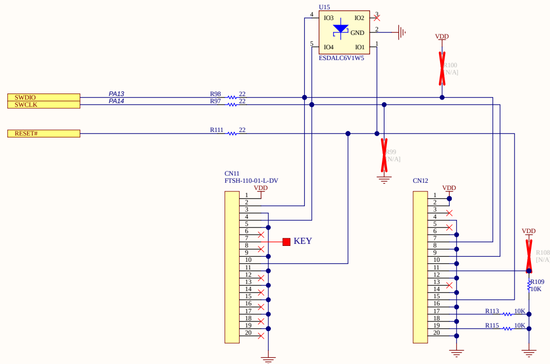
SWD connectors
