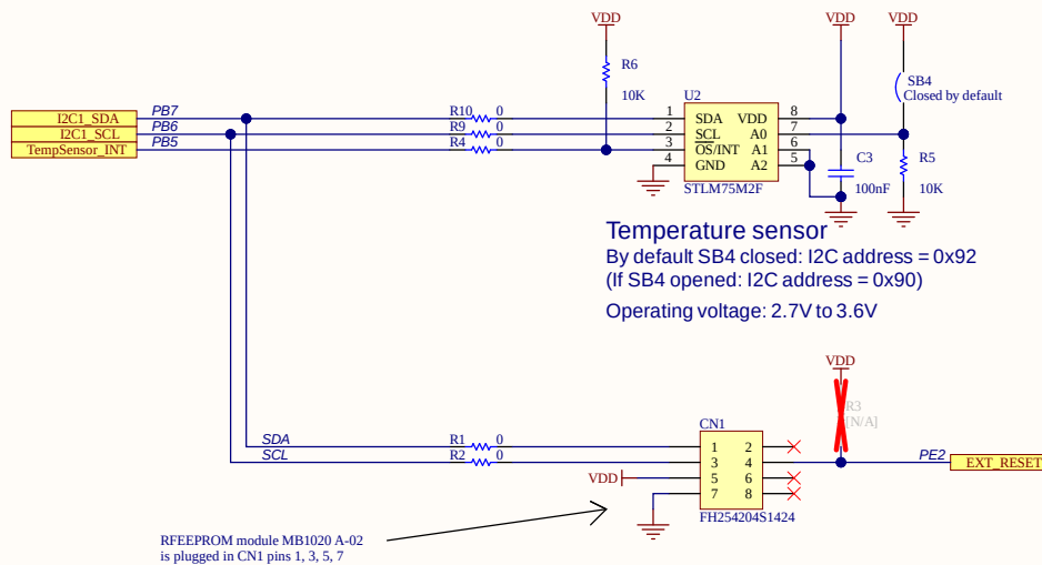
RFEEPROM & Extension Connector RF EEPROM MB1020 A-02 I2C address=0xA6
