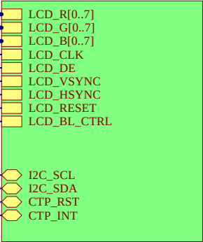
U_LCD_CTP_FLEX_CONNECTORS LCD_CTP_FLEX_CONNECTORS.SchDoc
