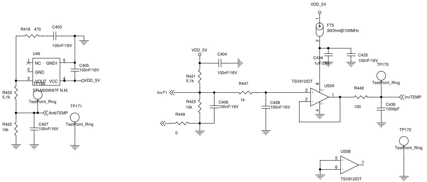
Figure 15. STDES-50KWPVWR main power board - circuit schematic (13 of 13)
