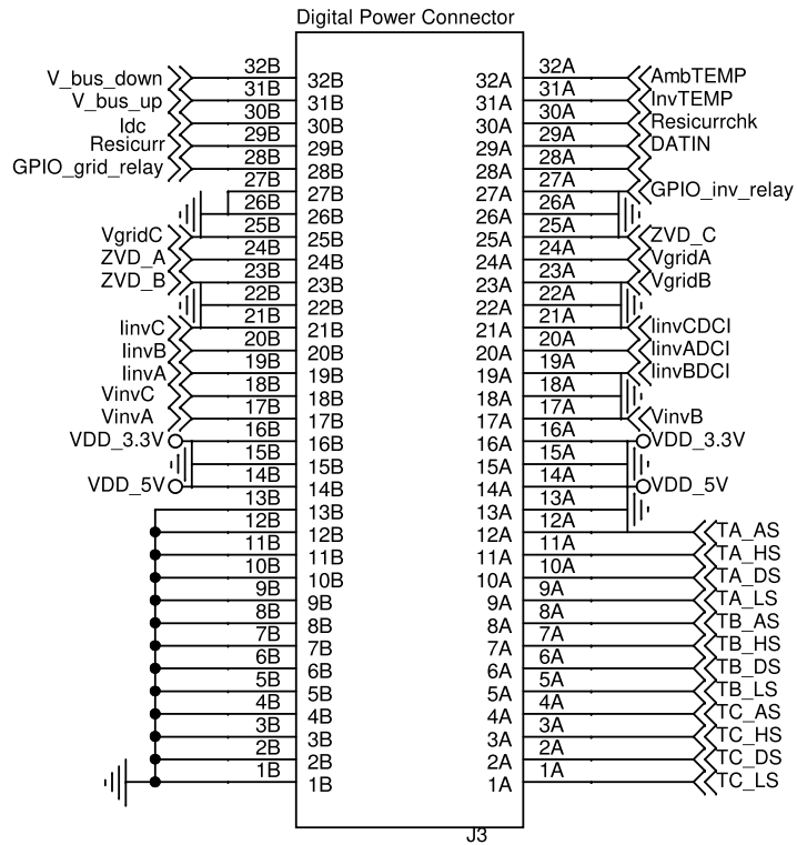
Figure 6. STDES-50KWPVPR main power board - circuit schematic (4 of 13)
