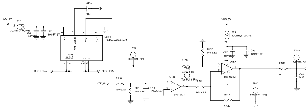
Figure 7. STDES-50KWPVPR main power board - circuit schematic (5 of 13)
