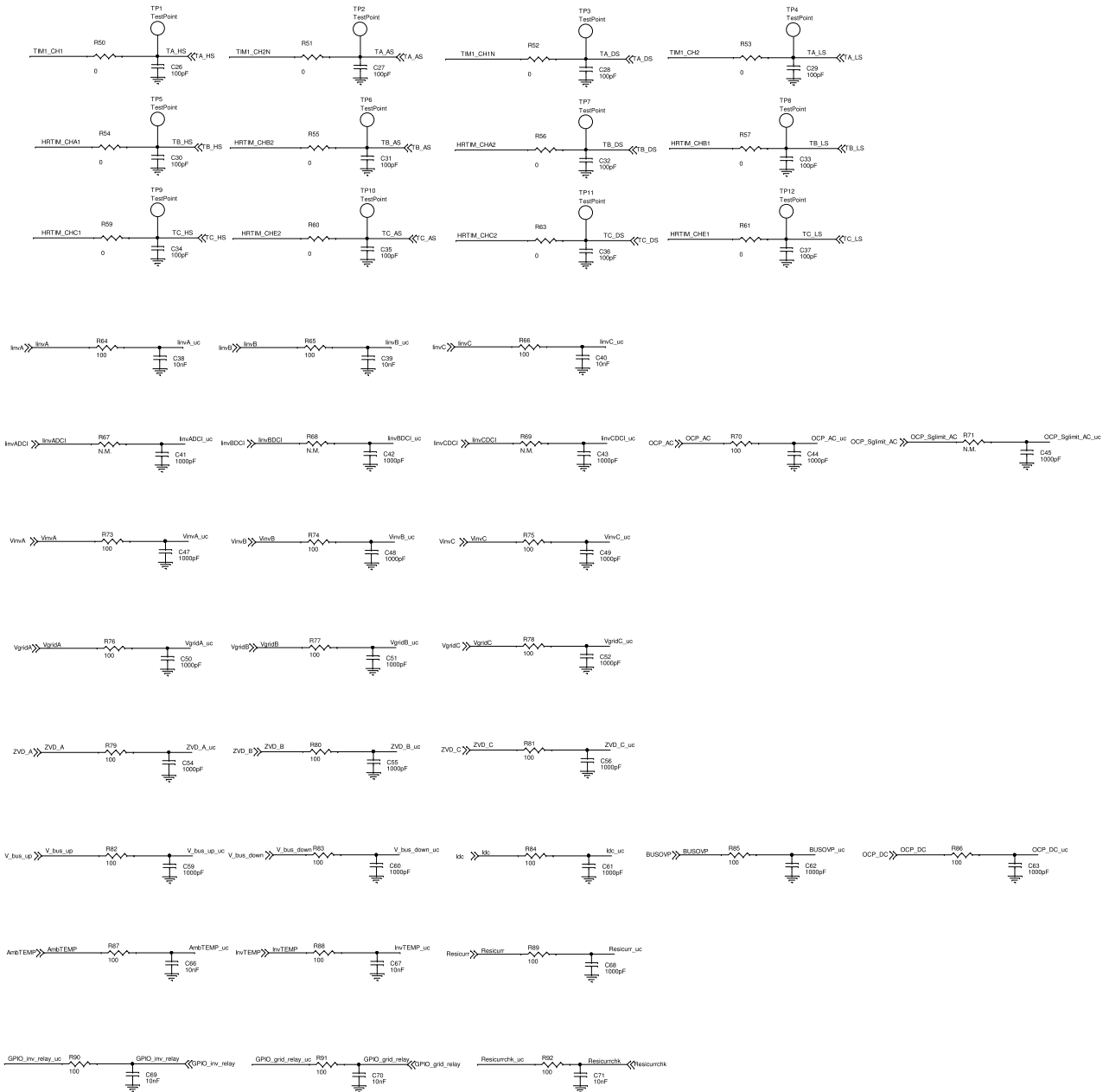
Figure 19. STDES-H743CTRL control board - circuit schematic (4 of 5)
