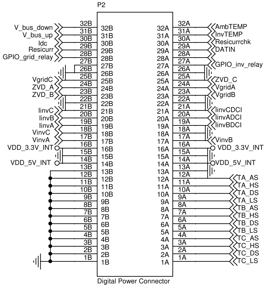
Figure 16. STDES-H743CTRL control board - circuit schematic (1 of 5)
