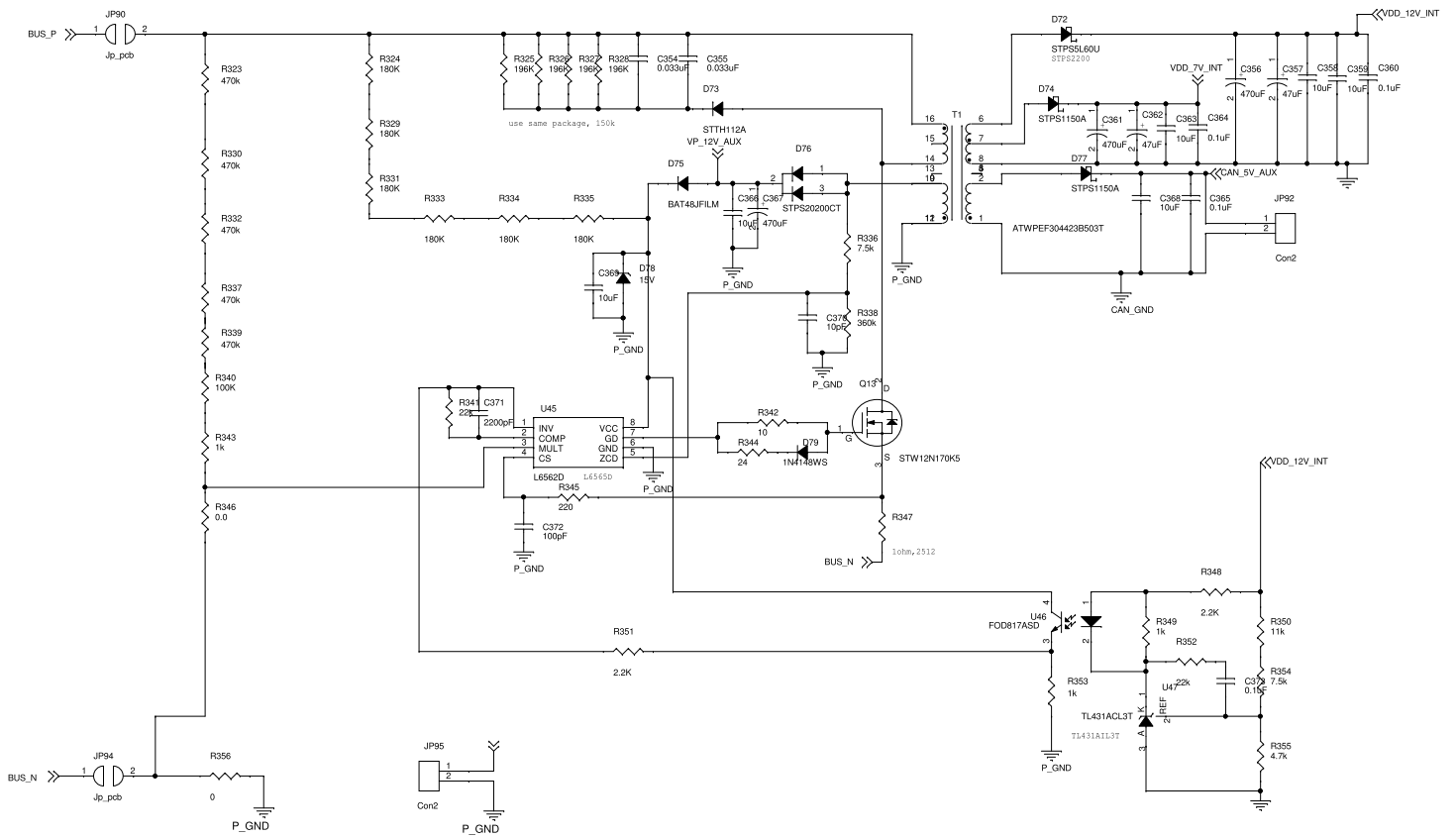
Figure 11. STDES-50KWPVWR main power board - circuit schematic (9 of 13)
