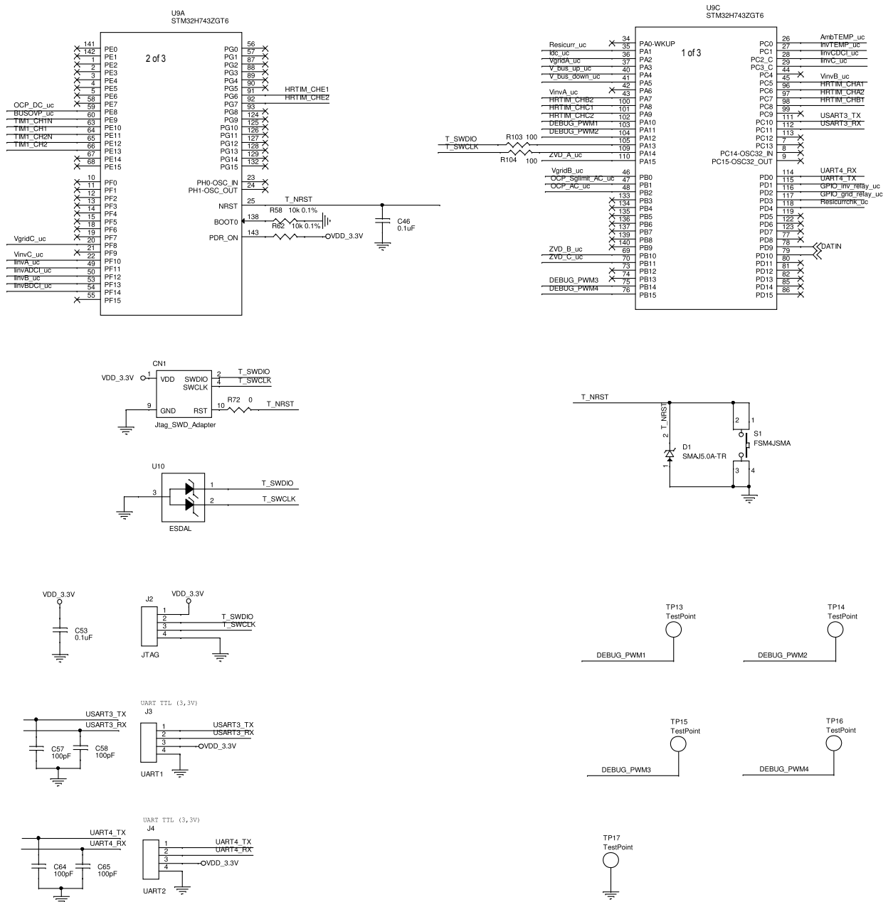
Figure 18. STDES-H743CTRL control board - circuit schematic (3 of 5)
