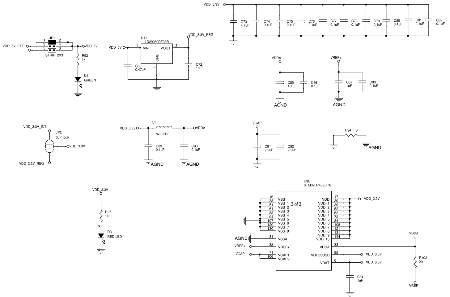
Figure 20. STDES-H743CTRL control board - circuit schematic (5 of 5)
