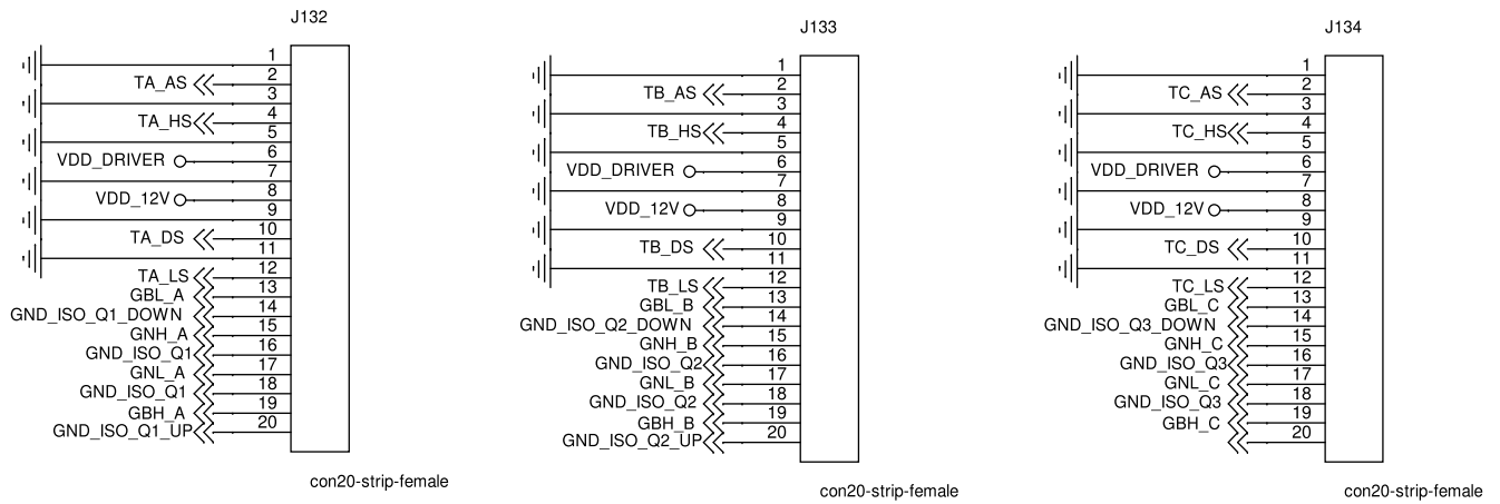
Figure 9. STDES-50KWPVPWR main power board - circuit schematic (7 of 13)
