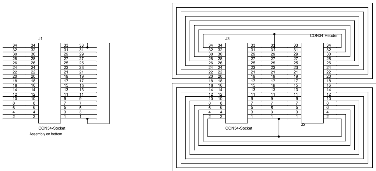
Figure 2. STEVAL-C34KAT2 circuit schematic: STEVAL-FLTCB02
