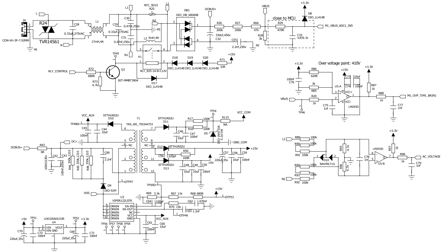
Figure 2. STEVAL-CTM014A circuit schematic (2 of 3)
