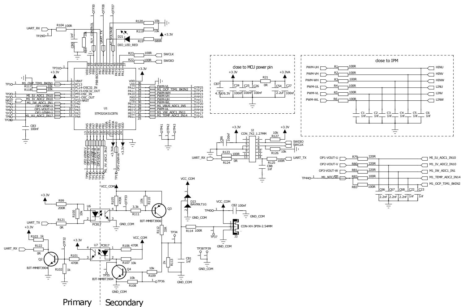
Figure 1. STEVAL-CTM014A circuit schematic (1 of 3)
