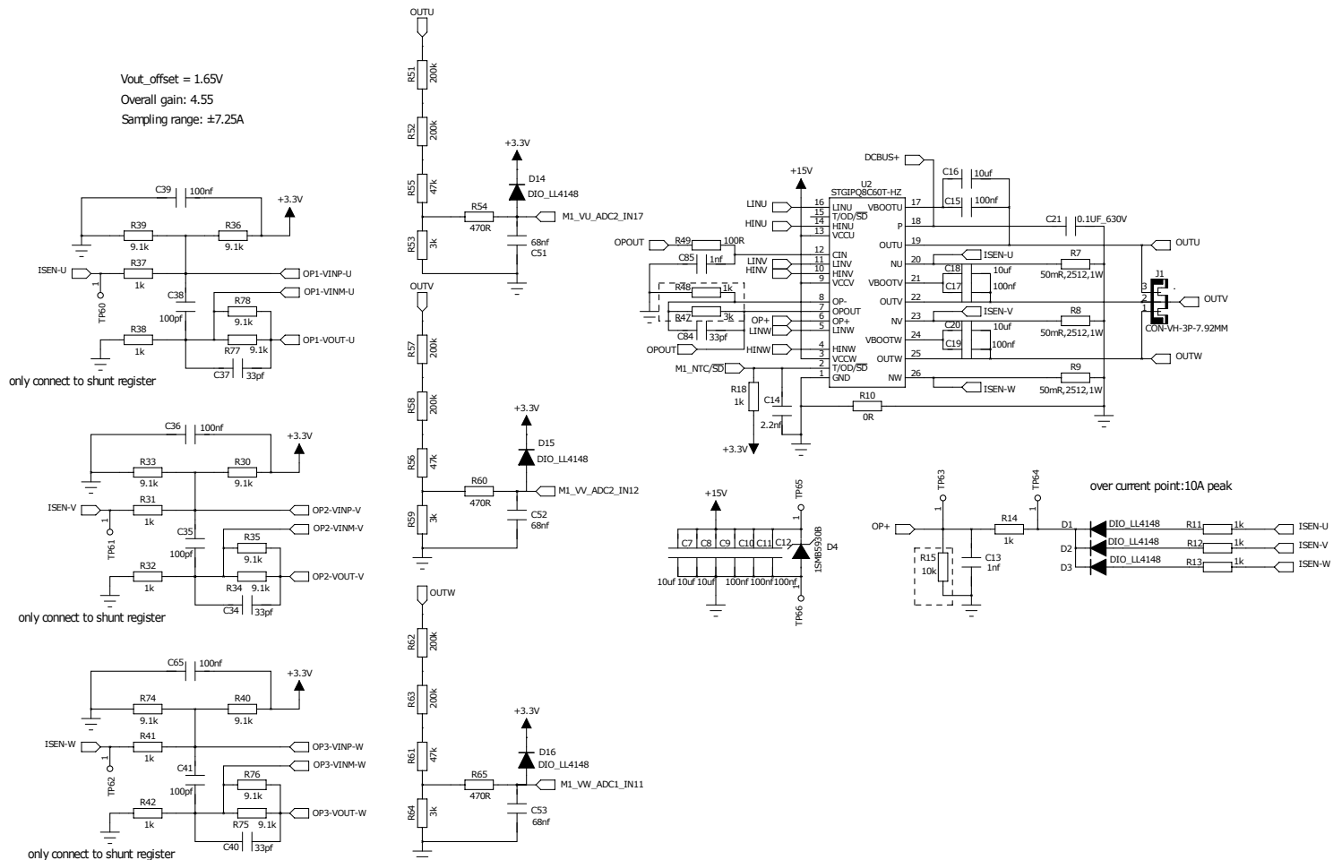
Figure 3. STEVAL-CTM014A circuit schematic (3 of 3)
