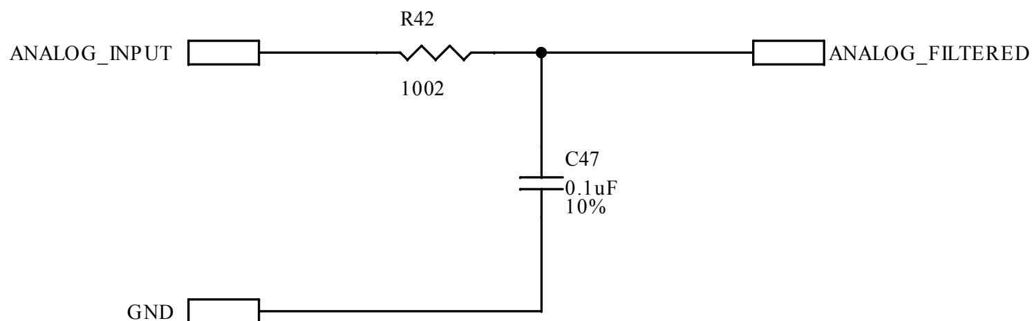
Figure 25. STEVAL-CTM020A circuit schematic (25 of 26)
