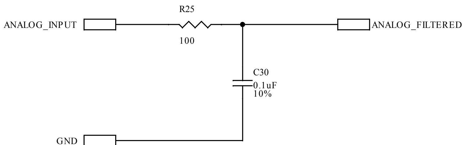
Figure 15. STEVAL-CTM020A circuit schematic (15 of 26) RC filter close to MCU pin
