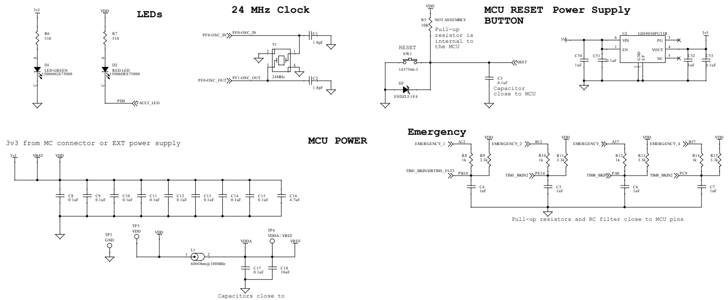
Figure 5. STEVAL-CTM020A circuit schematic (5 of 26)
