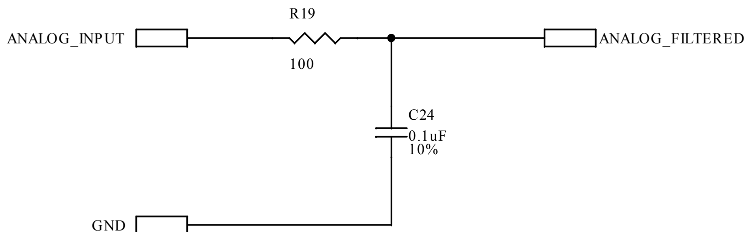
Figure 9. STEVAL-CTM020A circuit schematic (9 of 26)
