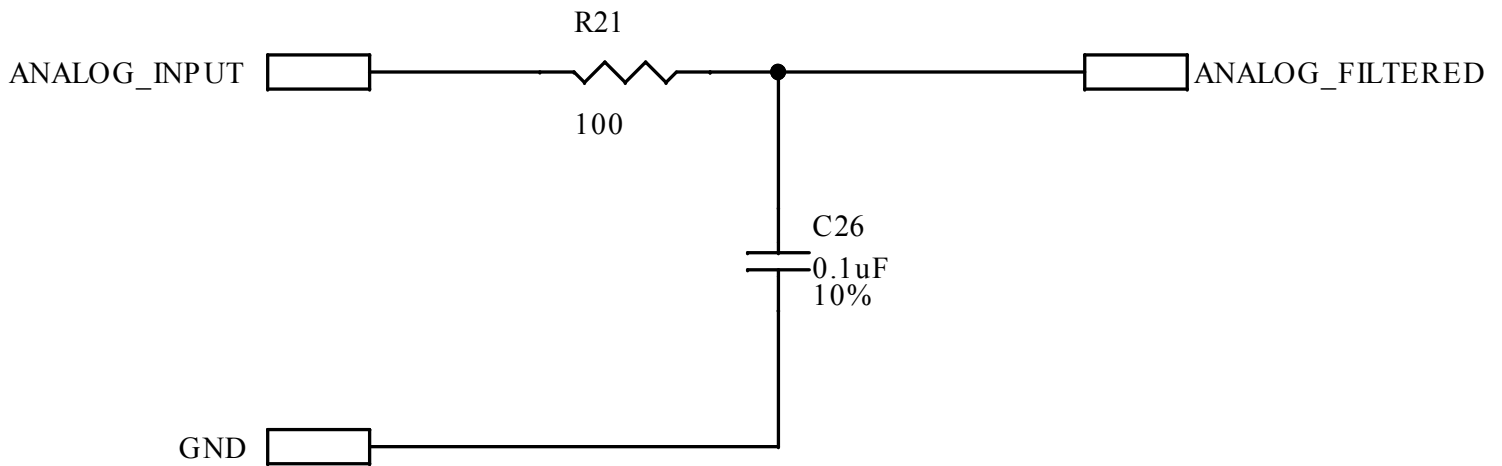
Figure 11. STEVAL-CTM020A circuit schematic (11 of 26) RC filter close to MCU pin
