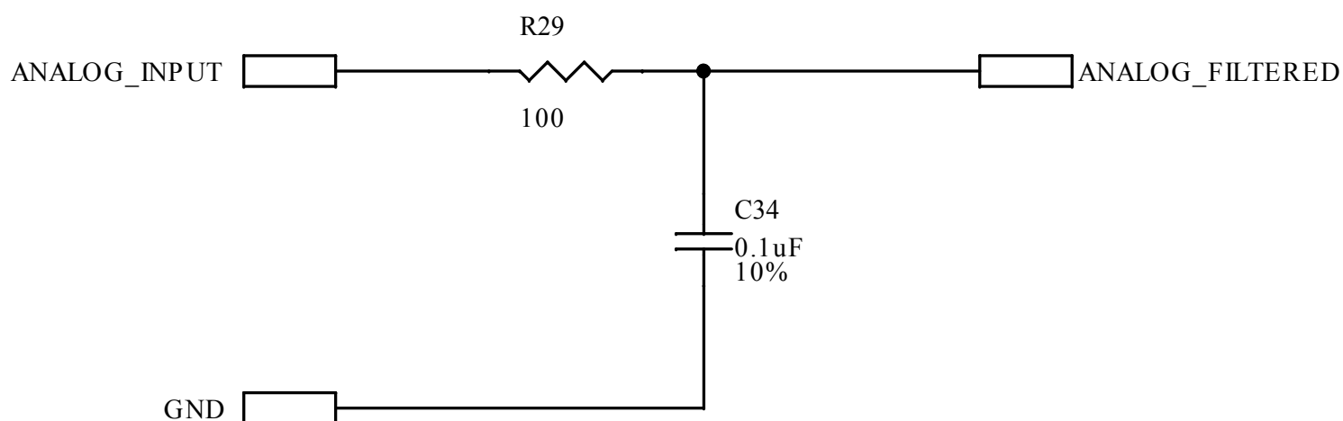
Figure 19. STEVAL-CTM020A circuit schematic (19 of 26) RC filter close to MCU pin
