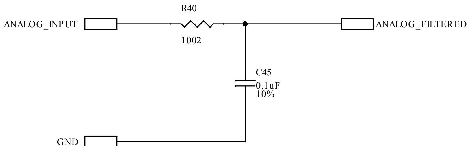
Figure 23. STEVAL-CTM020A circuit schematic (23 of 26)
