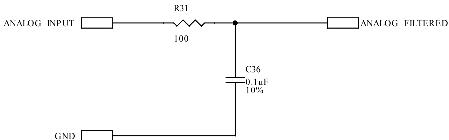
Figure 21. STEVAL-CTM020A circuit schematic (21 of 26)
