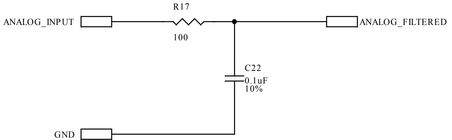
Figure 7. STEVAL-CTM020A circuit schematic (7 of 26)
