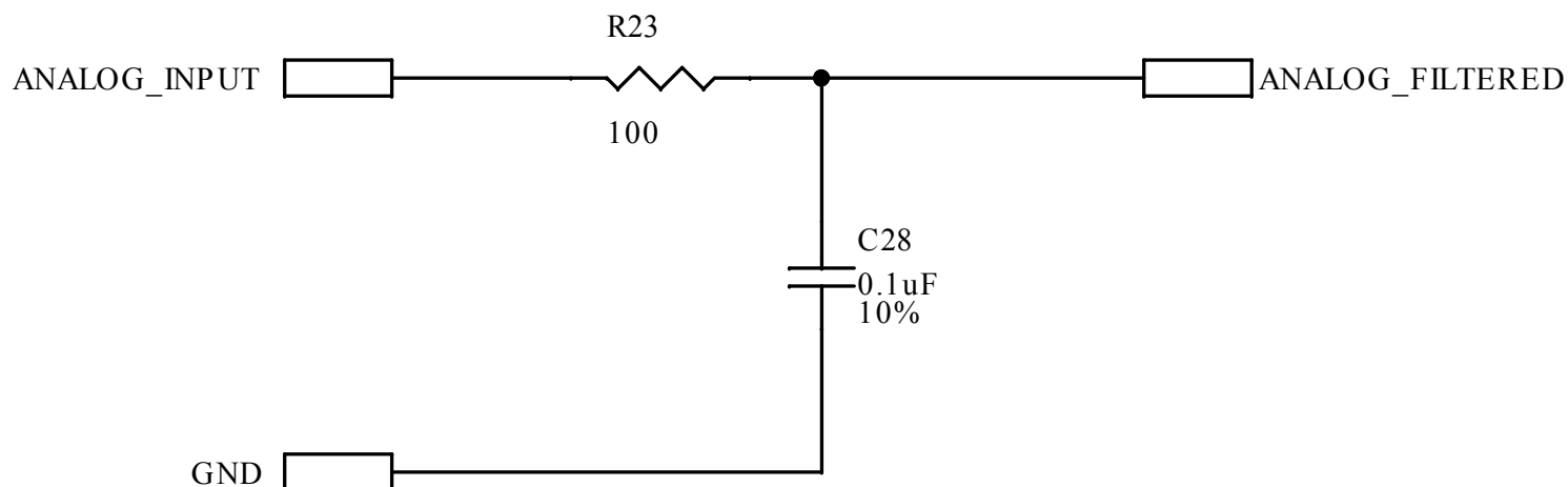
Figure 13. STEVAL-CTM020A circuit schematic (13 of 26) RC filter close to MCU pin
