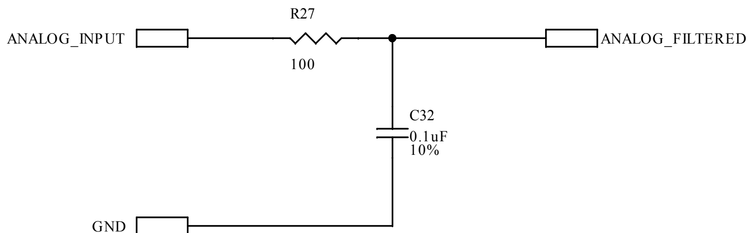
Figure 17. STEVAL-CTM020A circuit schematic (17 of 26)
