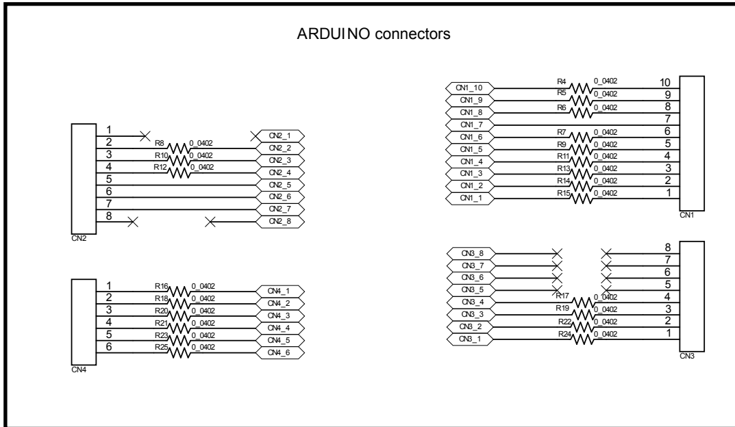
Figure 3. STEVAL-IDB013V1 circuit schematic (3 of 7)
