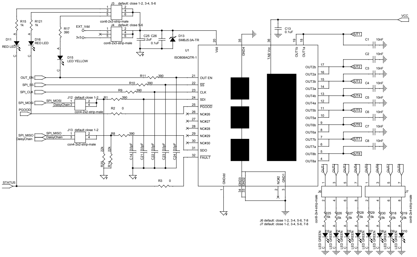
Figure 2. STEVAL-IFP048V1 circuit schematic (2 of 2)
