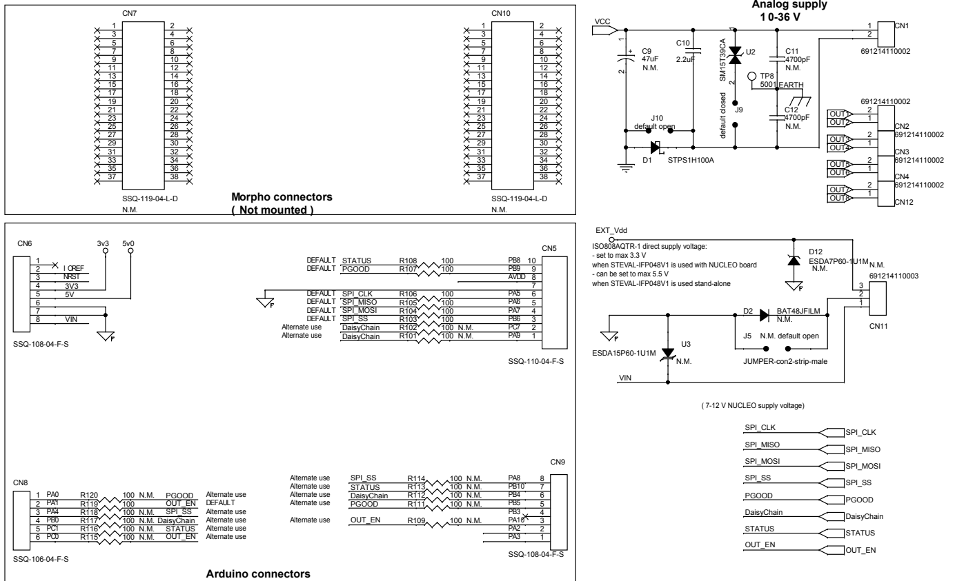
Figure 1. STEVAL-IFP048V1 circuit schematic (1 of 2)
