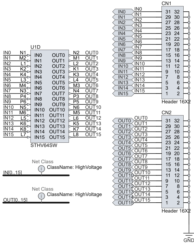
Figure 2: STEVAL-IME015V1 board schematic (2 of 6)
