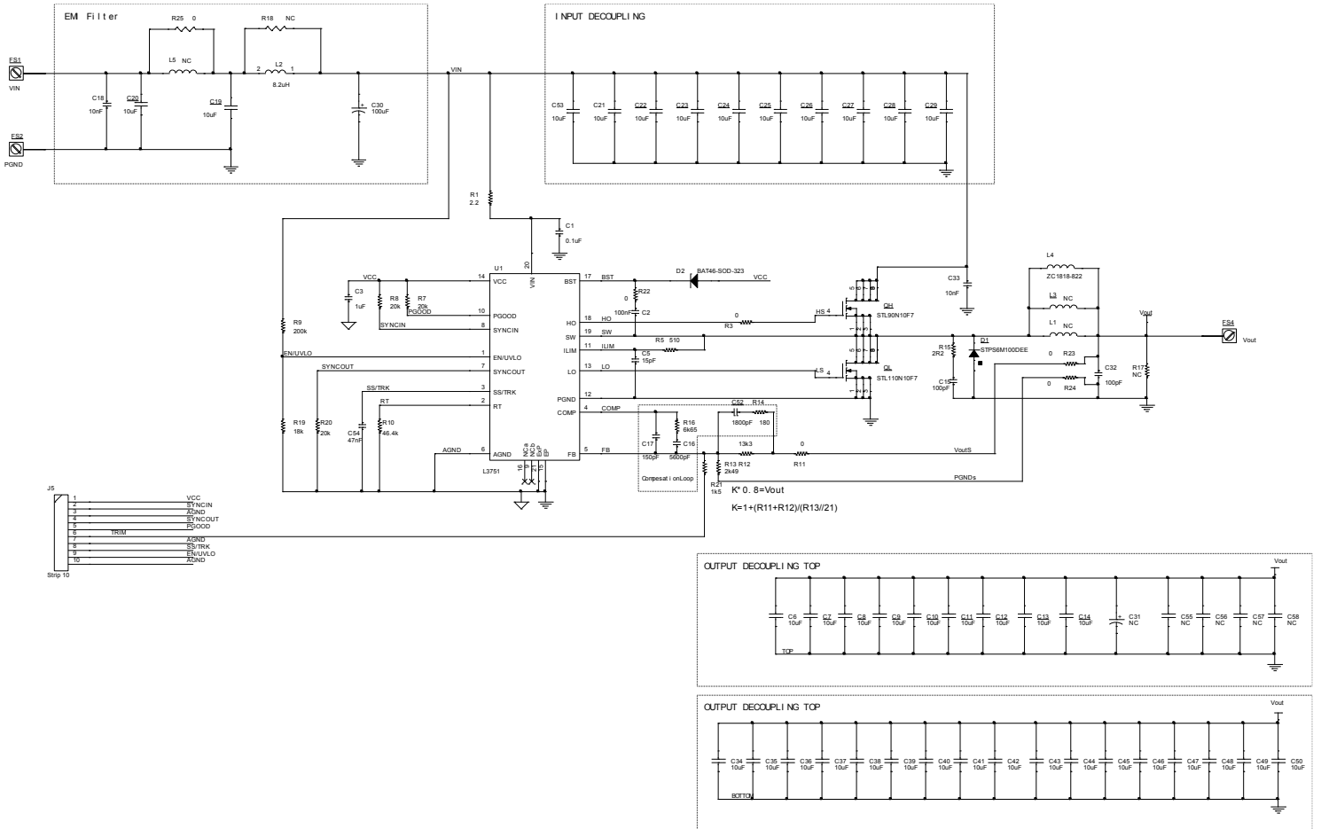
Figure 1. STEVAL-L3751V12 circuit schematic
