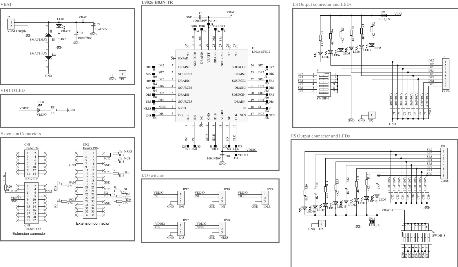
Figure 1. Evaluation board schematic
