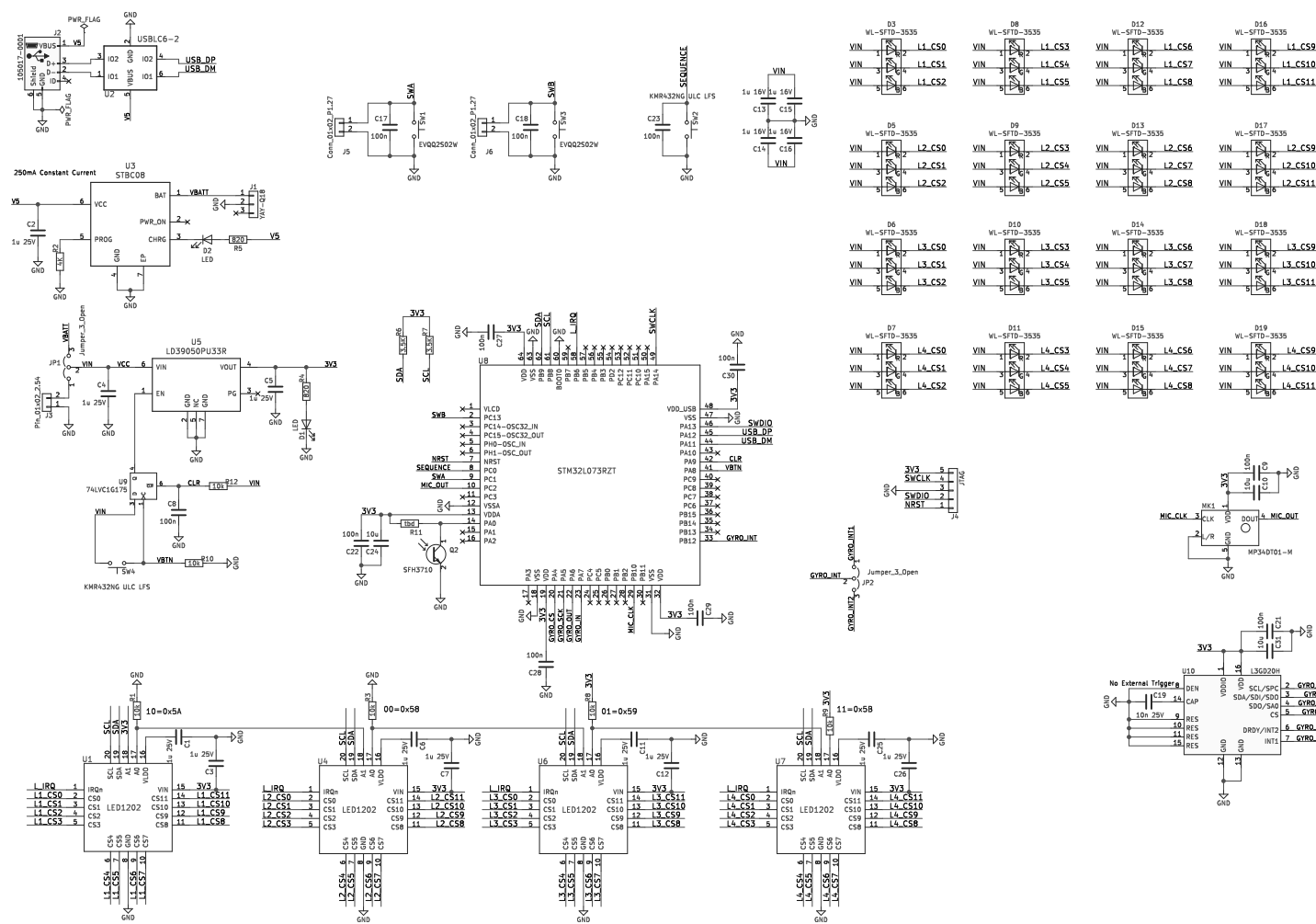
Figure 1: STEVAL-LLL011V1 schematic
