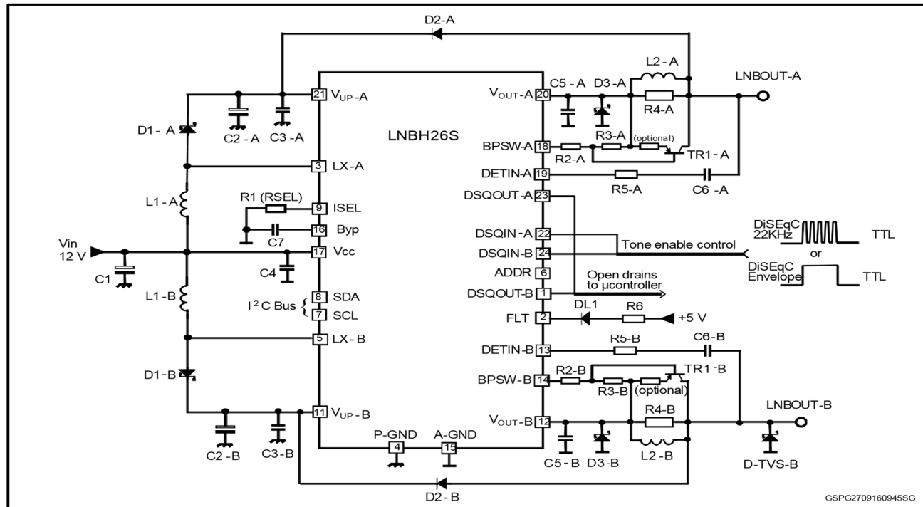
STEVAL-LNBH06 circuit schematic
