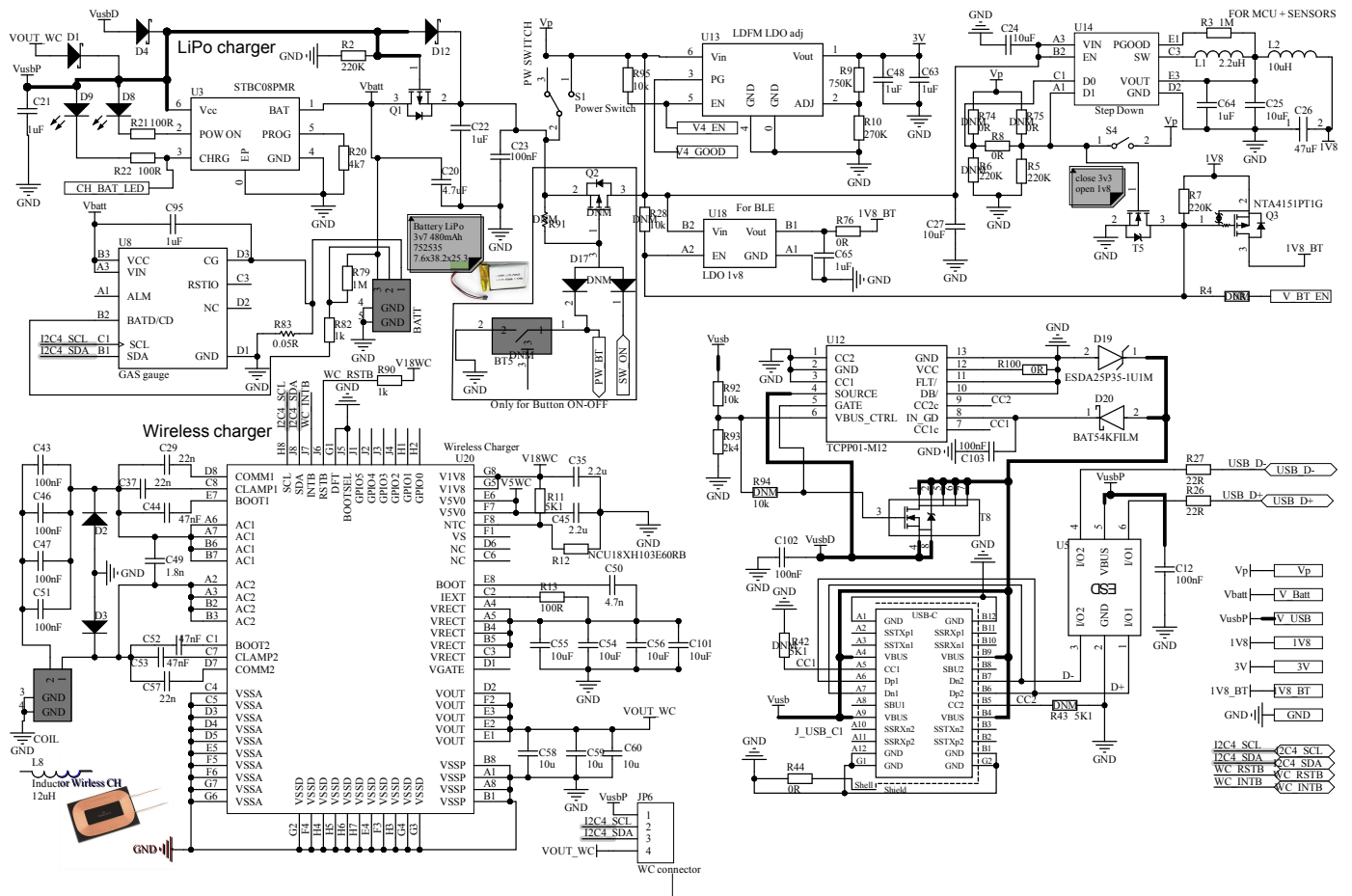
Figure 2. Sensortilebox_pro_Power
