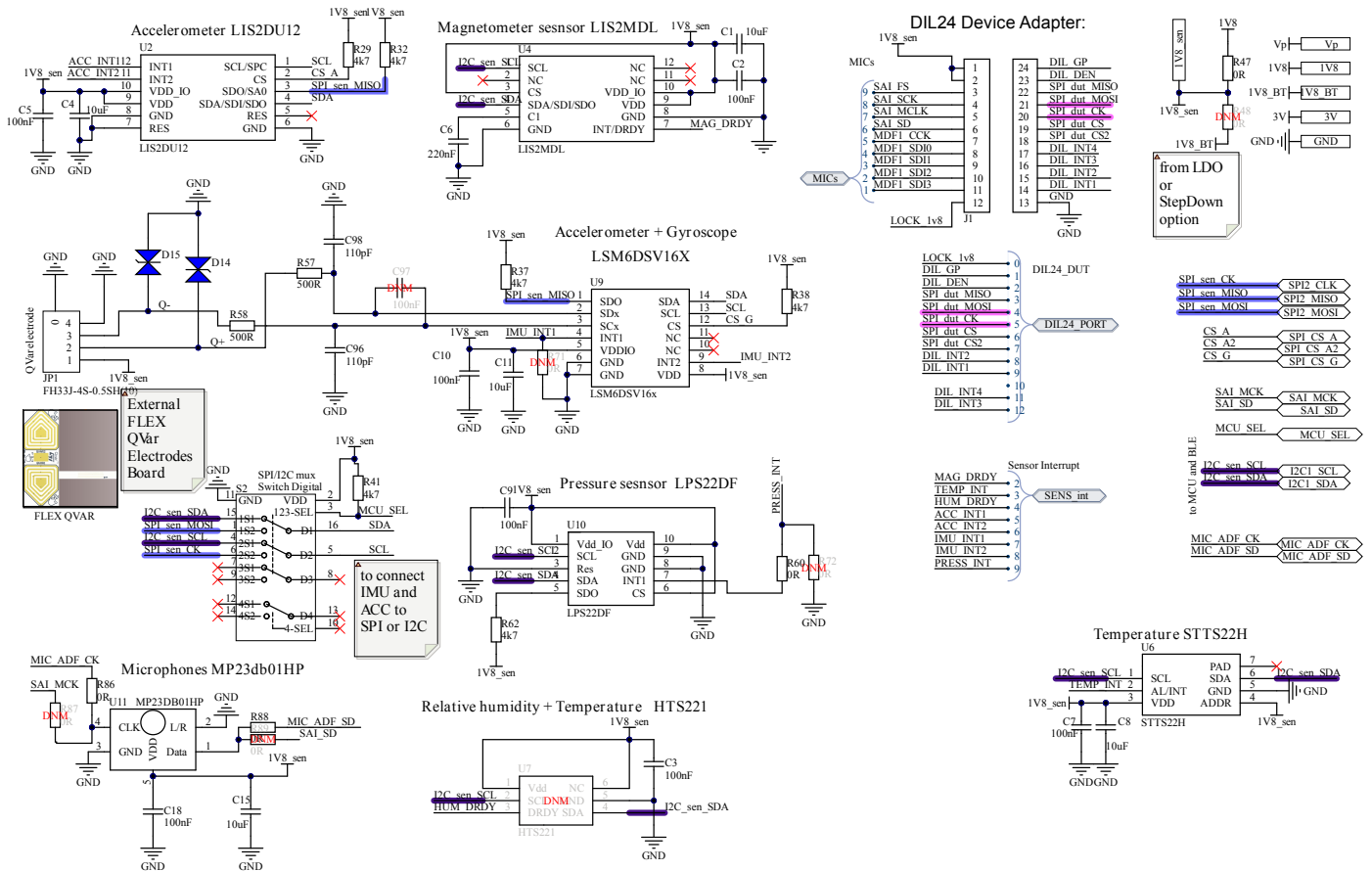
Figure 4. Sensortilebox_pro_sensors
