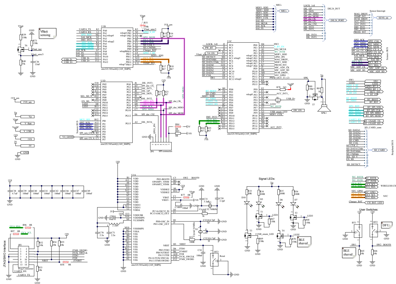
Figure 3. Sensortilebox_pro_MCU
