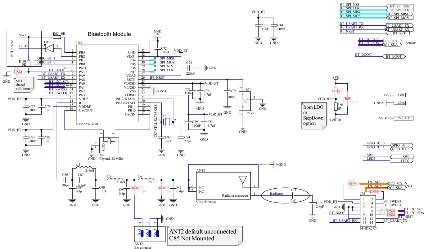
Figure 5. Sensortilebox_pro_BLE
