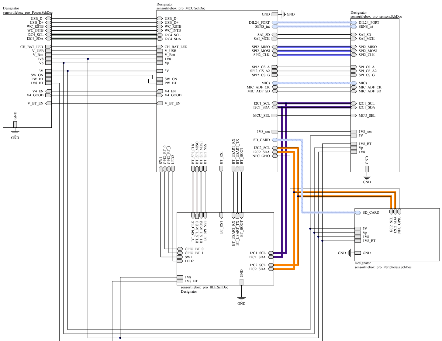
Figure 1. Sensortilebox_pro_main
