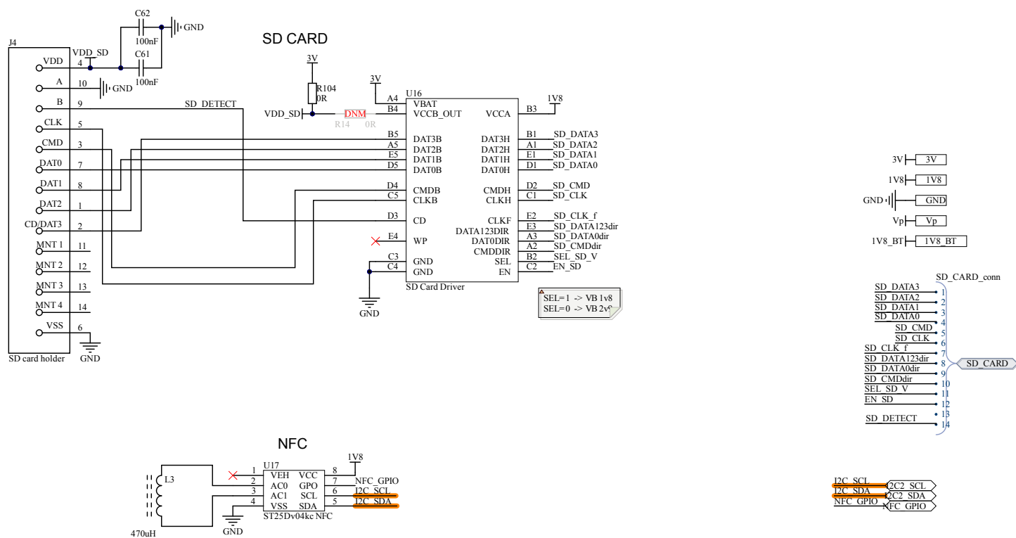
Figure 6. Sensortilebox_pro_Peripherals
