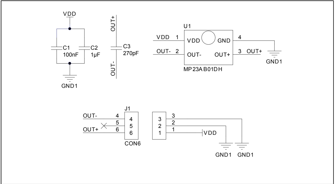
Figure 1: STEVAL-MKI139V5 circuit schematic
