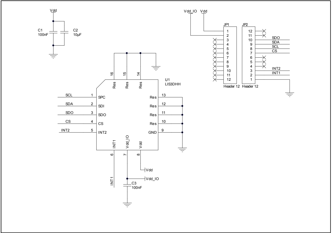
Figure 1: STEVAL-MKI180V1 circuit schematic
