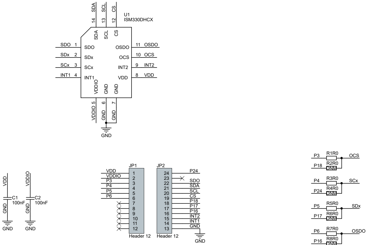
Figure 1: STEVAL-MKI207V1 circuit schematic
