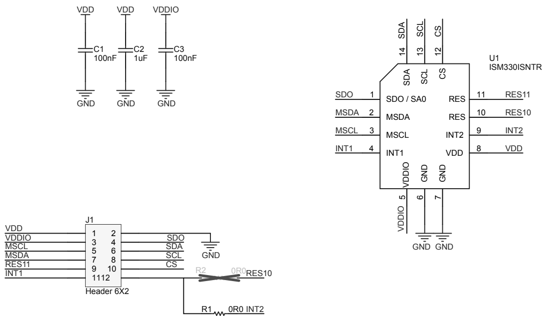
Figure 2. STEVAL-MKI233A circuit schematic
