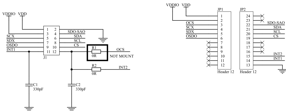
Figure 1. STEVAL-MKIGIBV5 circuit schematic
