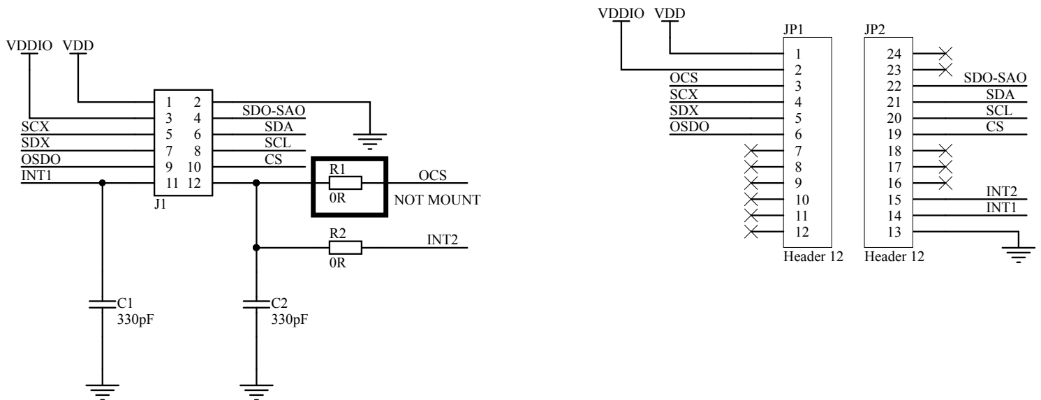
Figure 1. STEVAL-MKIGIBV5 circuit schematic
