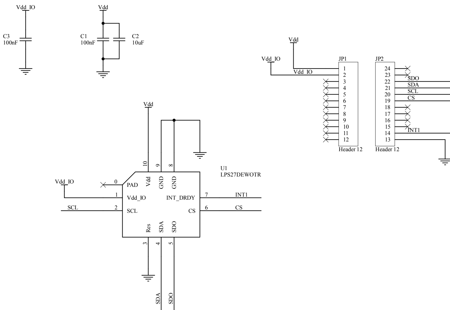
Figure 1. STEVAL-MKI256A schematic
