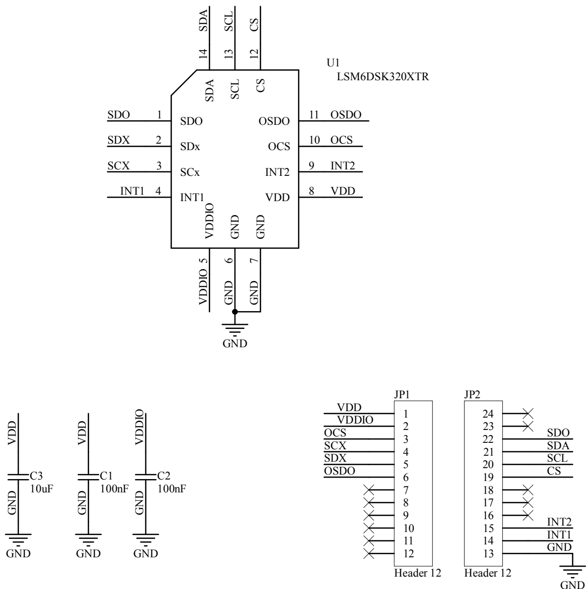
Figure 1. STEVAL-MKI257A schematic
