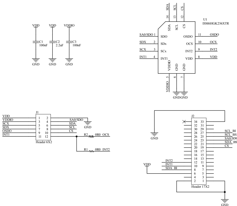
Figure 2. STEVAL-MKIGIBV5 circuit schematic
