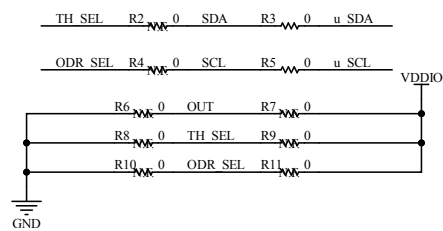
Figure 2. STEVAL-MKIGIBV5 circuit schematic
