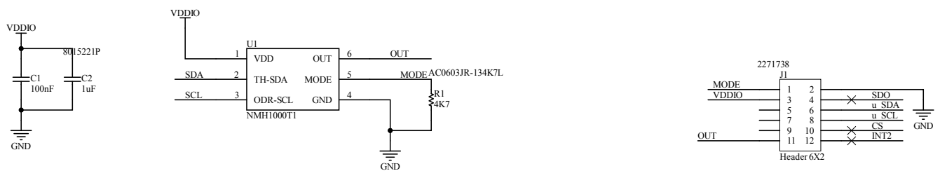
Figure 1. STEVAL-MKI259A circuit schematic
